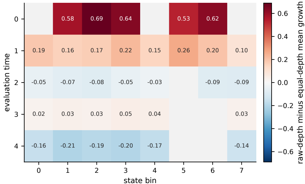
WFR-FM growth: raw minus equal-depth growth readout depends on mass convention
