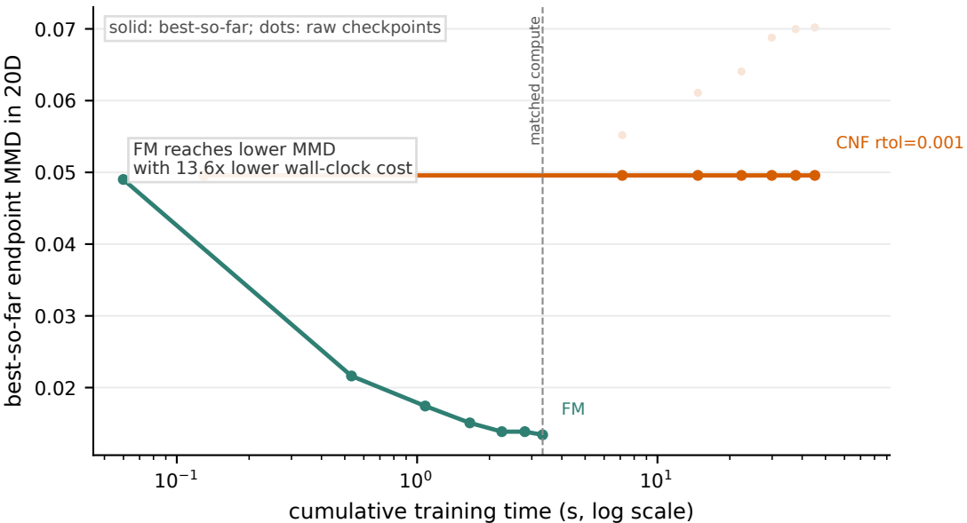
Training time vs endpoint quality
