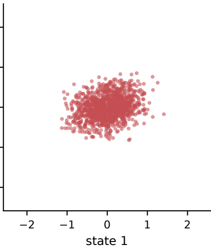
Target: rotated Gaussian
