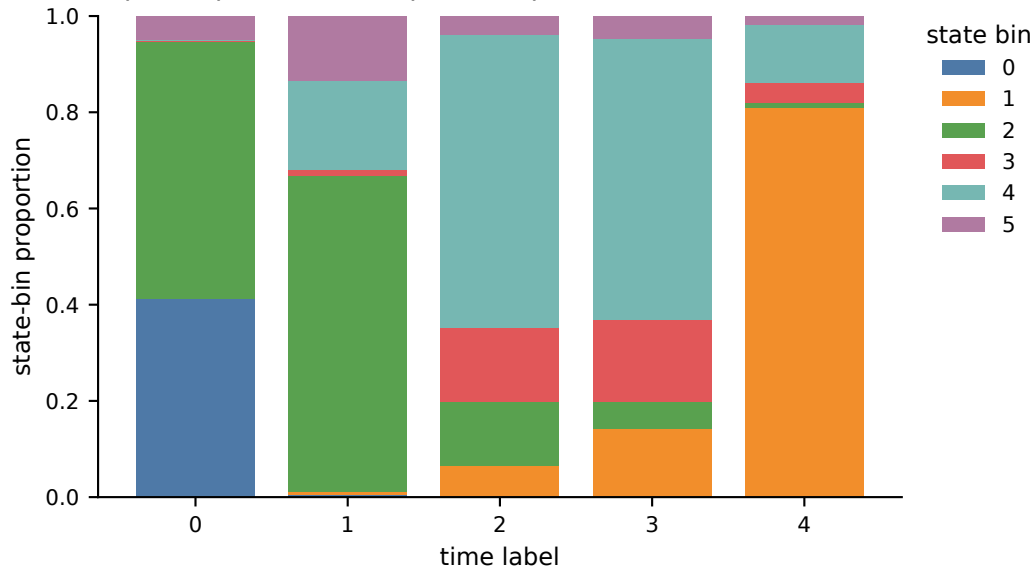
Equal-depth EB composition equal-depth: n = 2381 per time point
