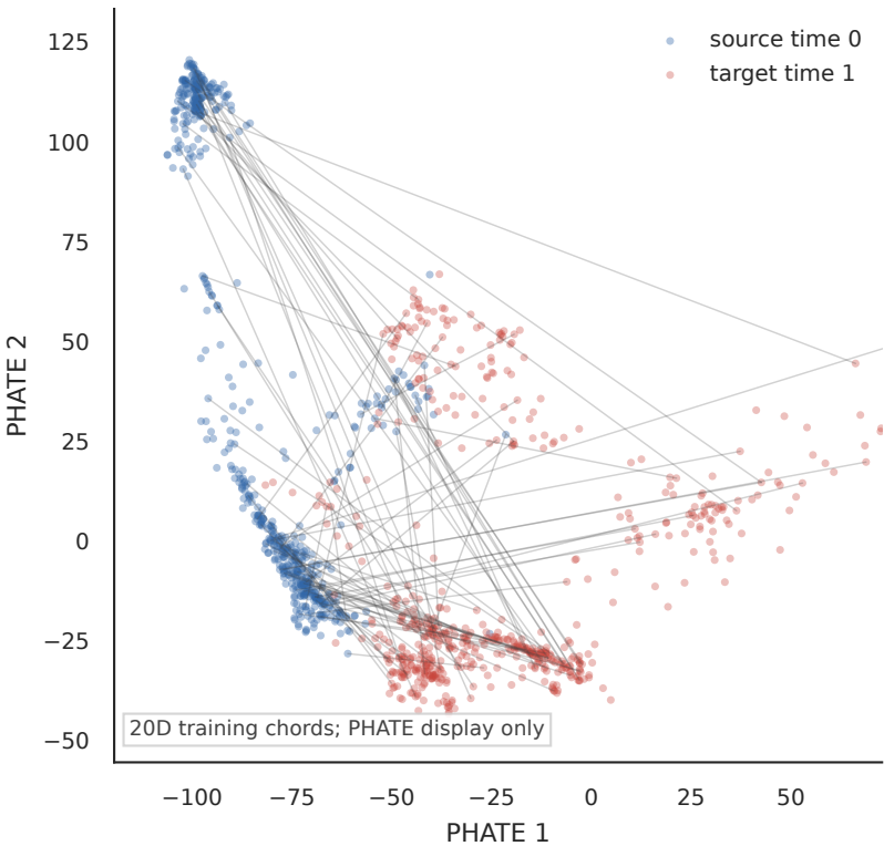
Sampled EB train endpoint pairs displayed in PHATE
