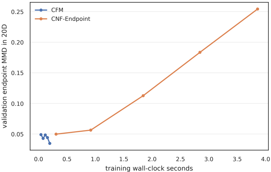
CFM local regression versus CNF-Endpoint adjoint training
