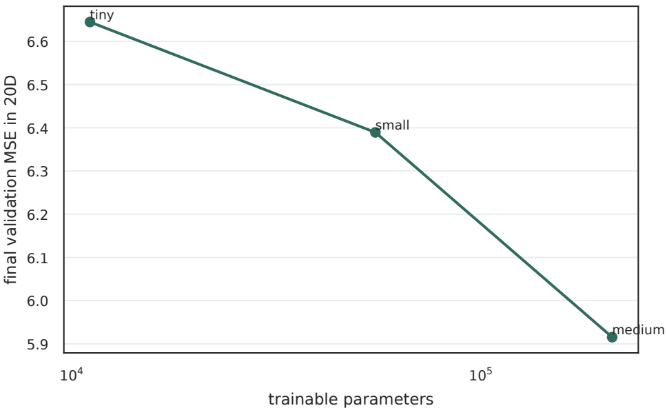
Capacity ablation: validation velocity-regression error
