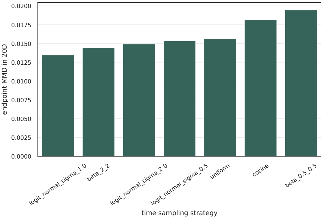
Final endpoint MMD after short CFM runs
