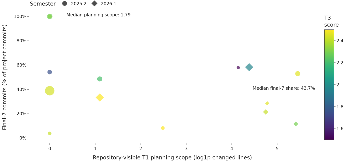
Fig. 3. Repository-visible planning scope versus final-seven-day commit concentration. Marker color reports T3 evaluator score and marker size reports absolute score change; quadrants are descriptive median splits.
