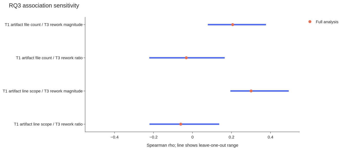
Fig. 17. RQ3 association sensitivity. Points show full-analysis Spearman values; horizontal segments show leave-one-out ranges. These ranges are descriptive diagnostics, not confidence intervals.
