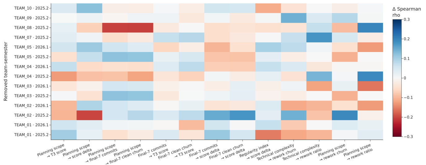
Leave-one-out influence map for directional associations
