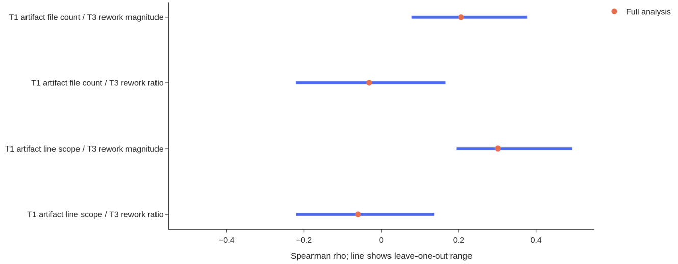
Fig. 7. RQ3 association sensitivity. Points show full-analysis Spearman values; horizontal segments show leave-one-out ranges. These ranges are descriptive diagnostics, not confidence intervals.
