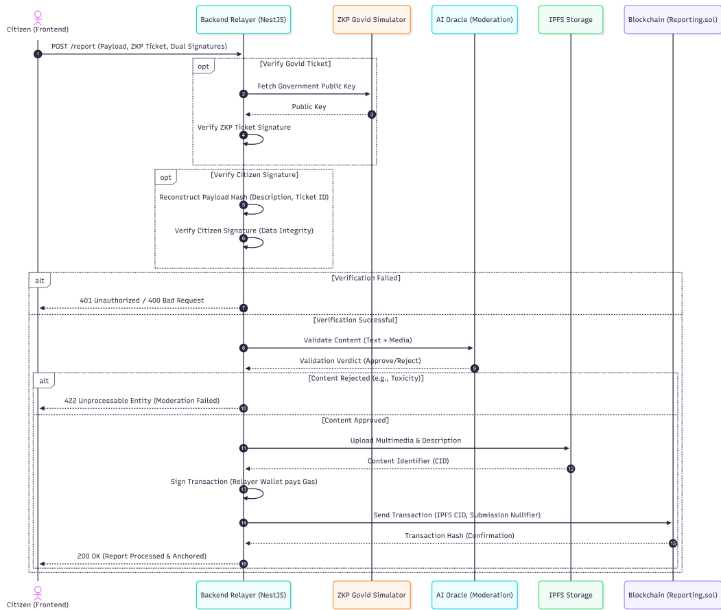
Figure 3.5: Backend relay workflow architecture.
