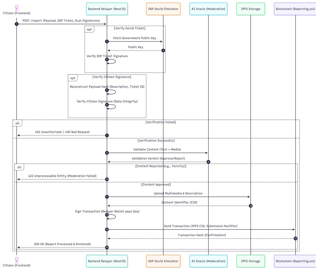
Figure 3.3: Backend relay workflow architecture.
