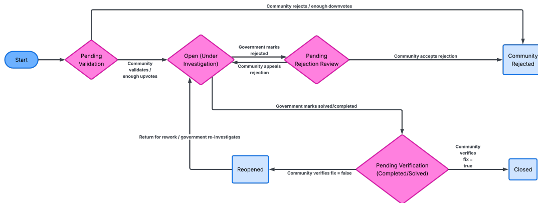
Figure 3.3: State transition diagram for the civic reporting system.
