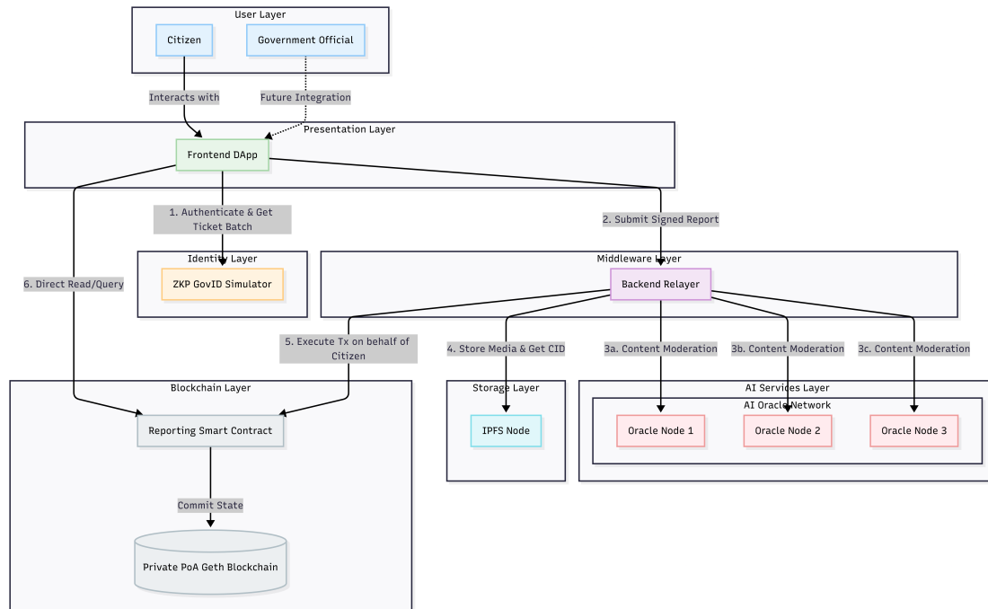
Figure 2.1: High-level architecture of the community-assisted reporting system.
