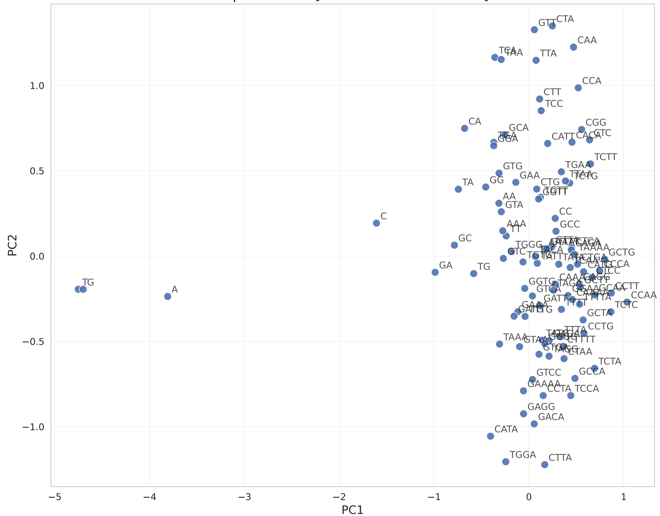
Explained Var: [0.07360279 0.02954664]
