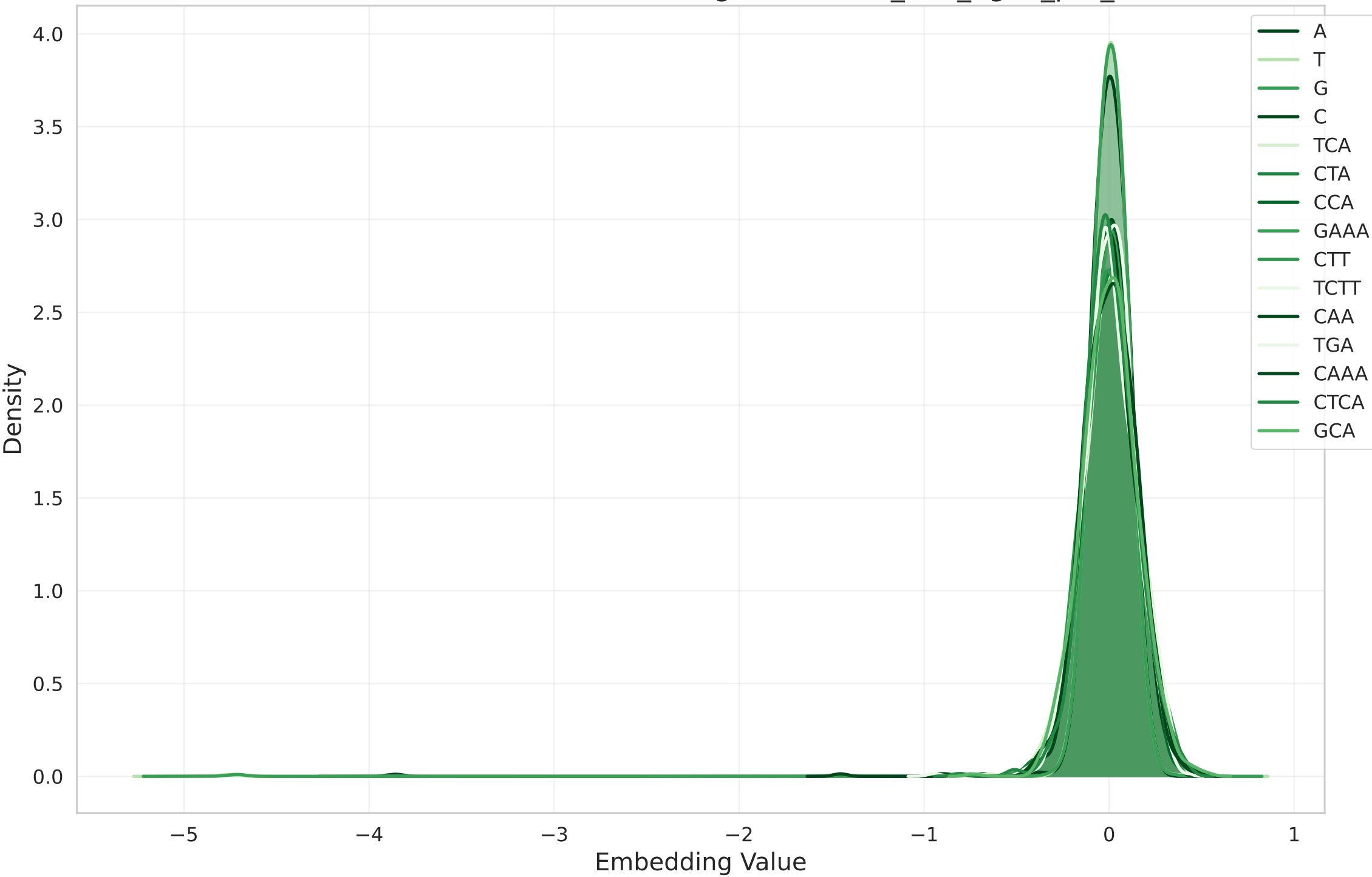
Distribution of Token Mean Embeddings (dnabert2_100_hg38_per_token)
