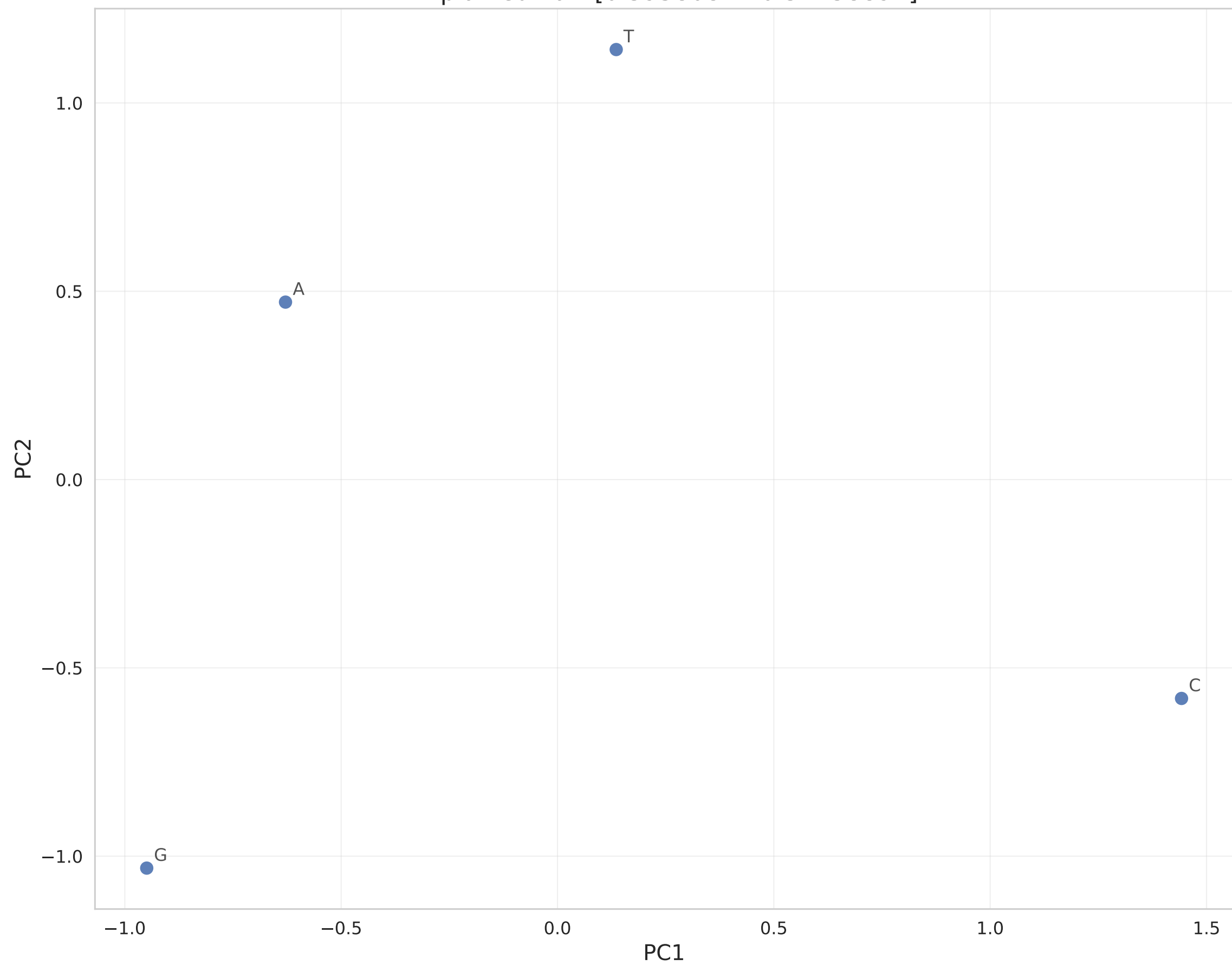
PCA of Token Embeddings (evo2_100_hg38_per_token) Explained Var: [0.39580822 0.34138897]
