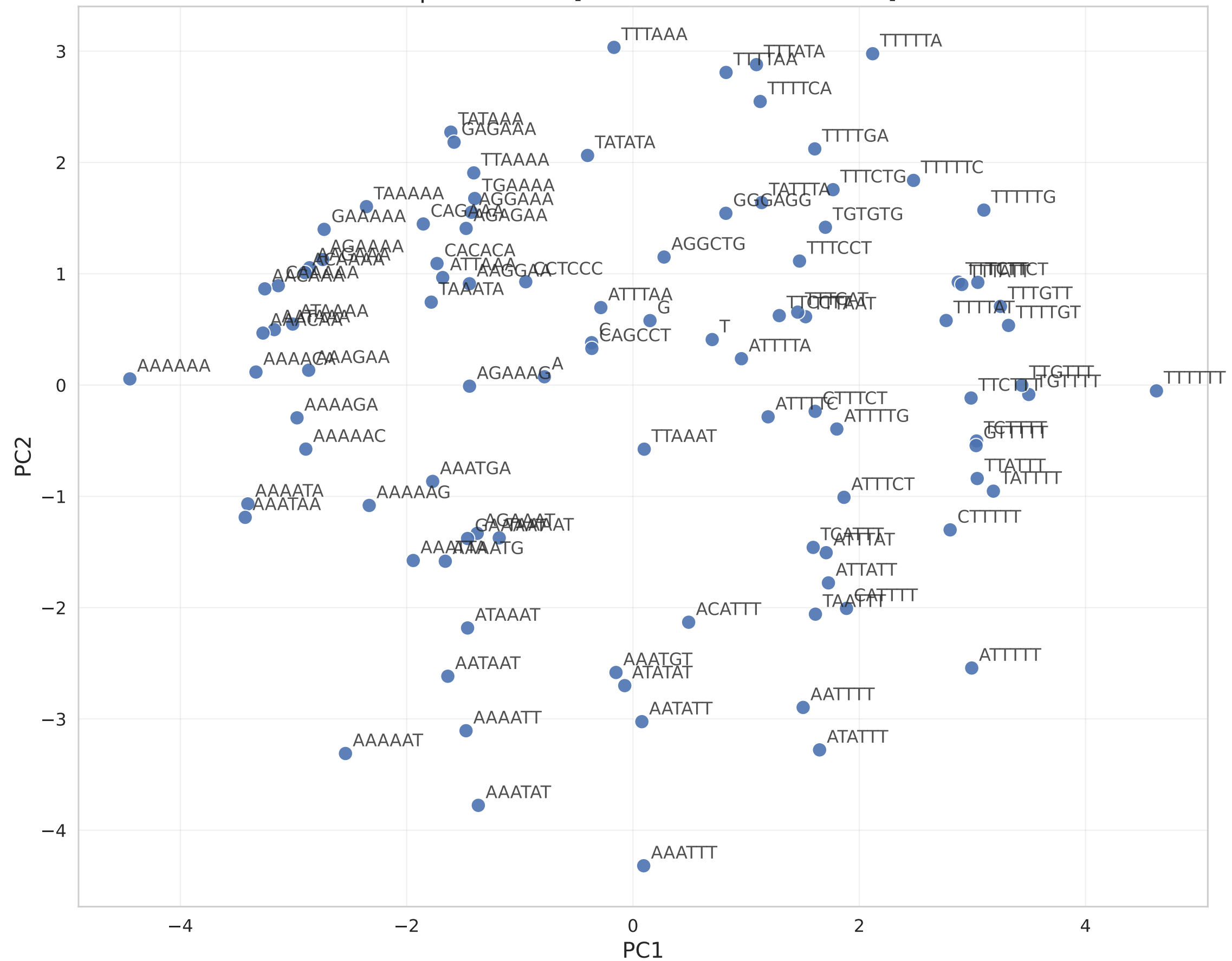
PCA of Token Embeddings (ntv2_100_hg38_per_token) Explained Var: [0.11175899 0.06301815]
