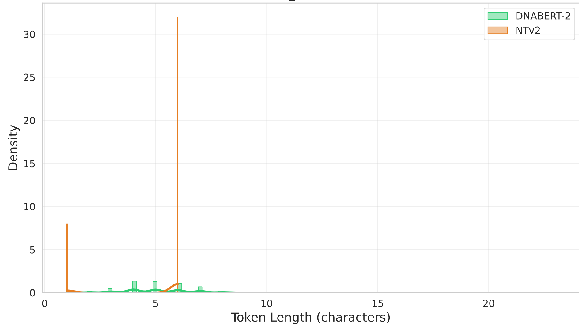
Token Length Distribution
