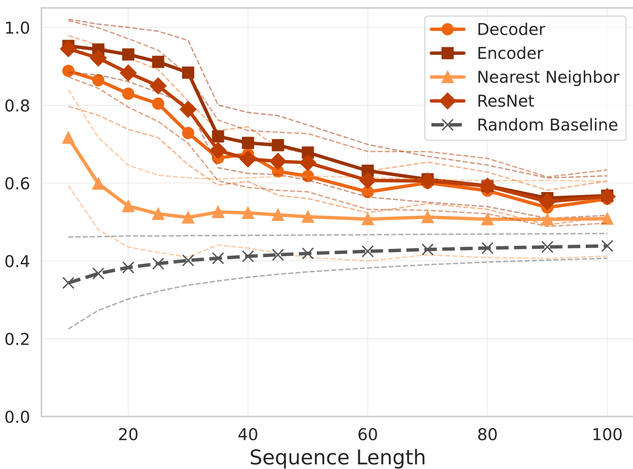
Levenshtein Similarity
