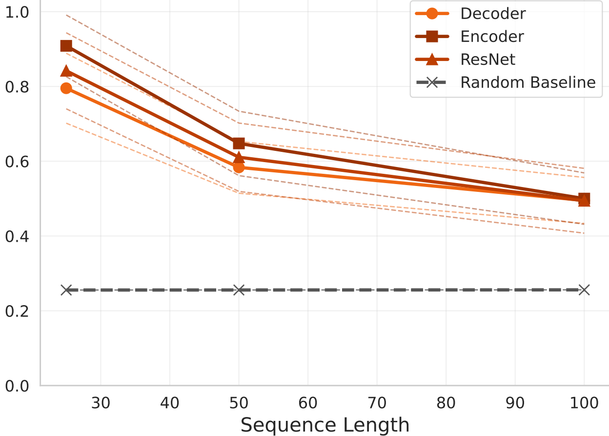
Nucleotide Accuracy
