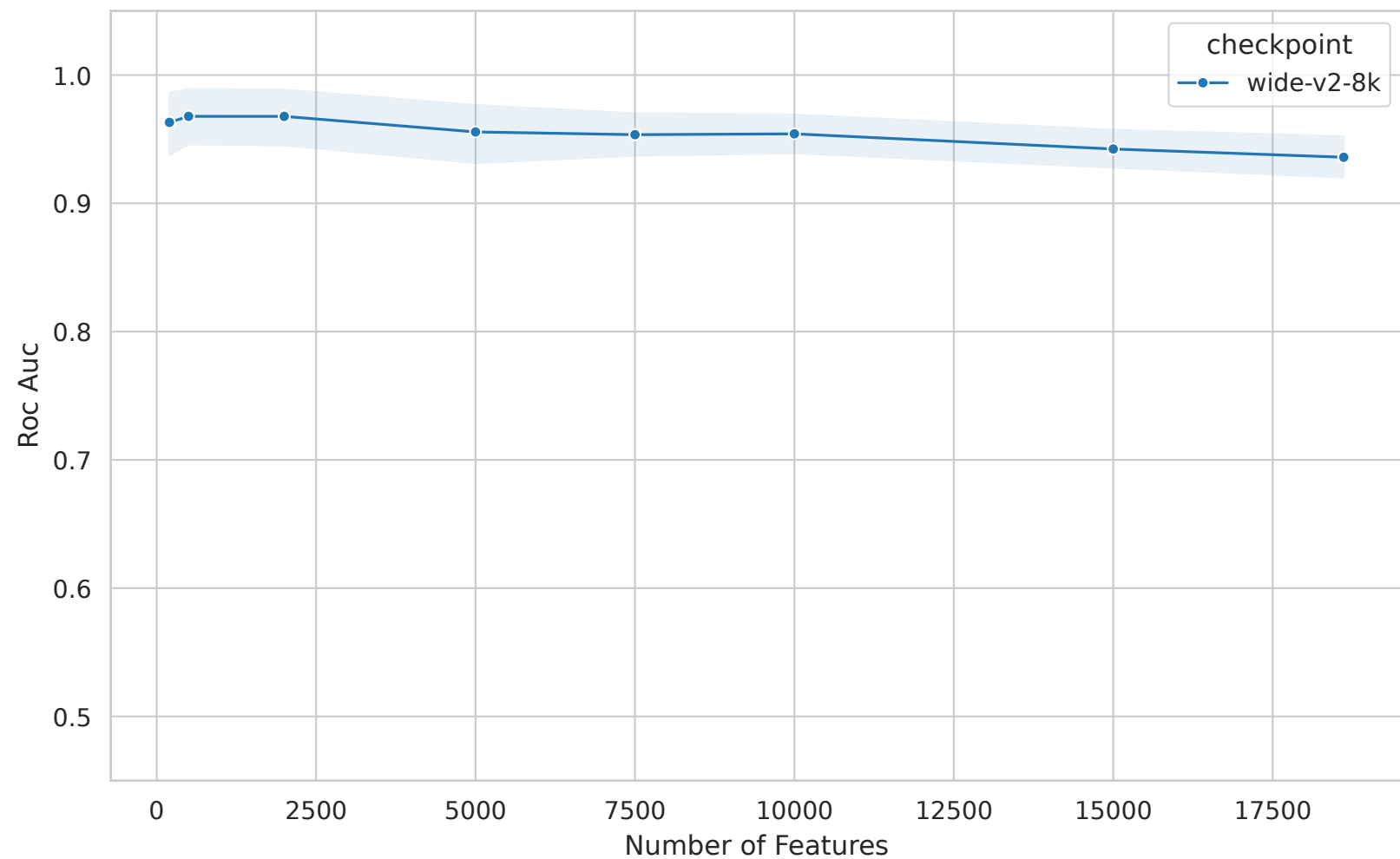
GBM - Roc Auc vs Feature Count
