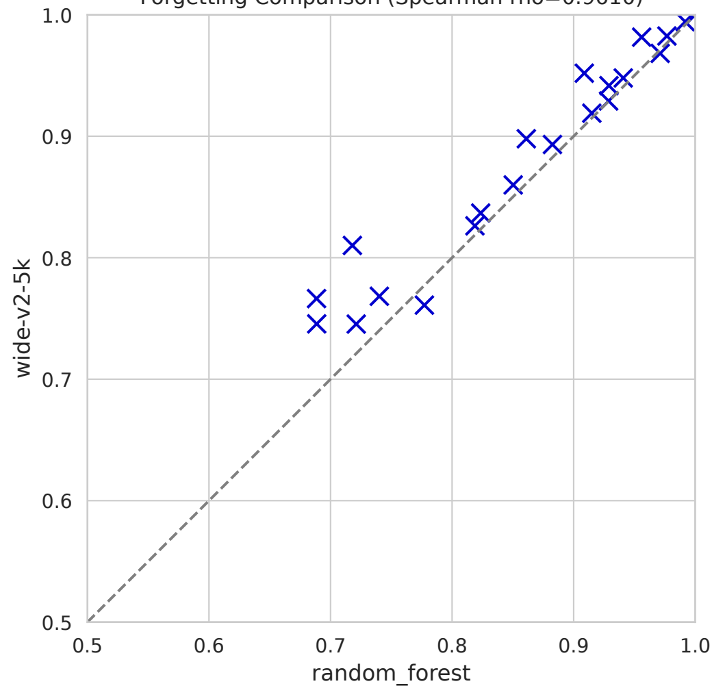
Forgetting Comparison (Spearman rho=0.9610)
