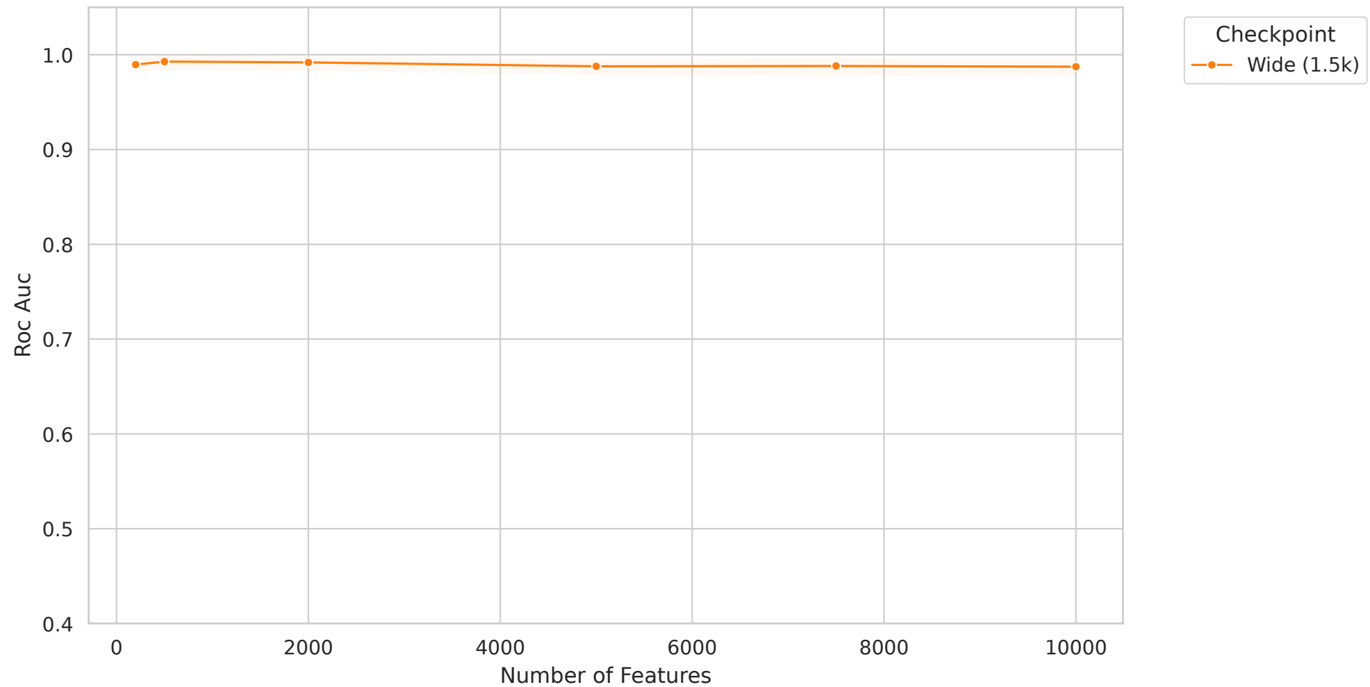
OV - Roc Auc vs Feature Count
