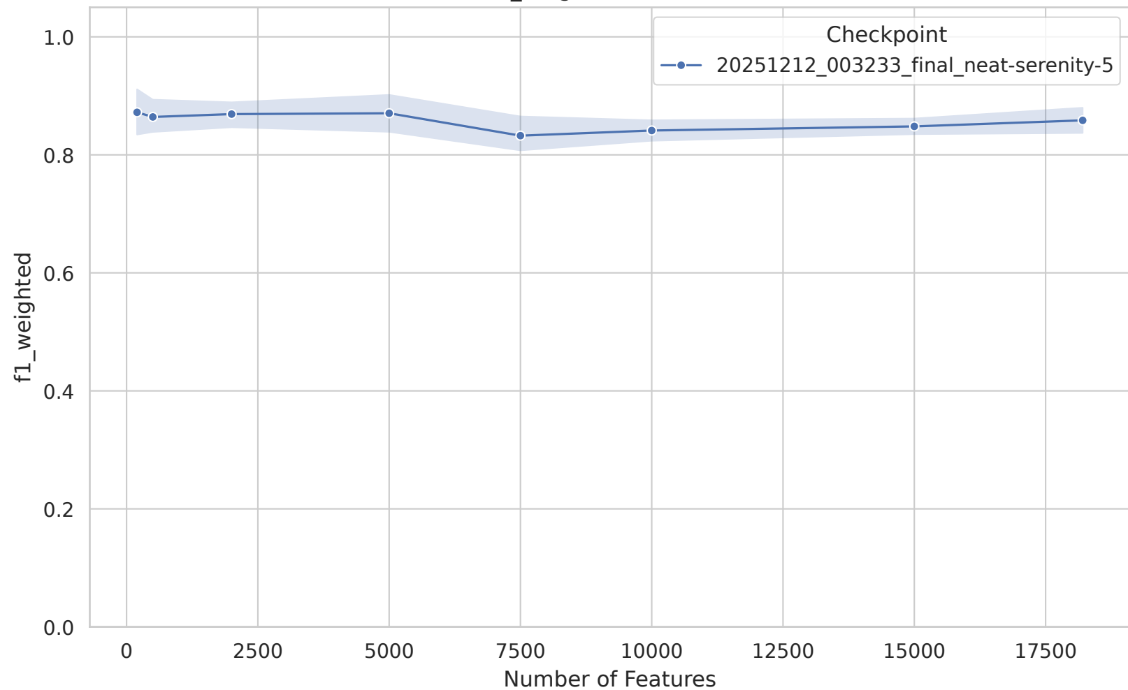
BRCA - f1_weighted vs Feature Count
