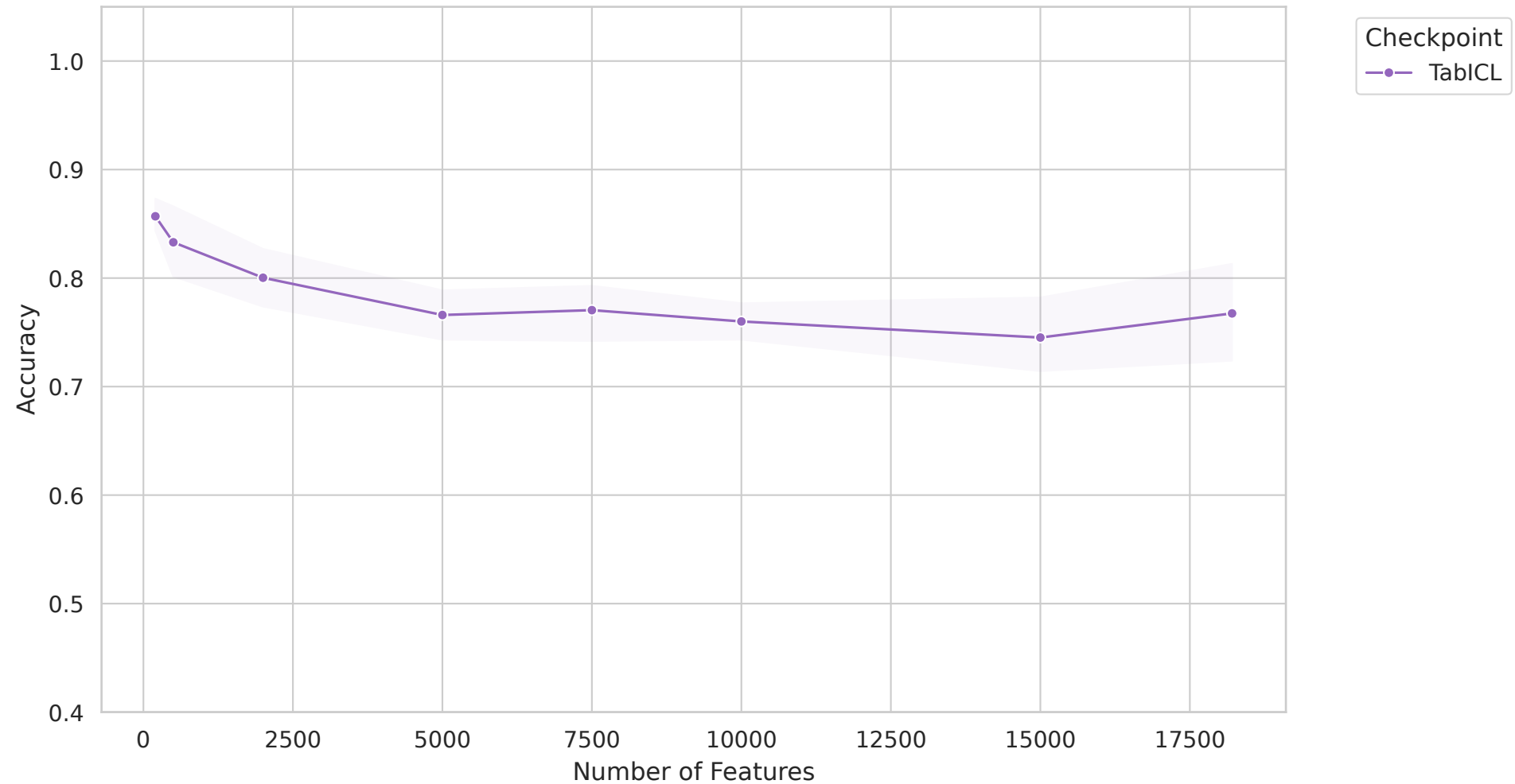
BRCA - Accuracy vs Feature Count
