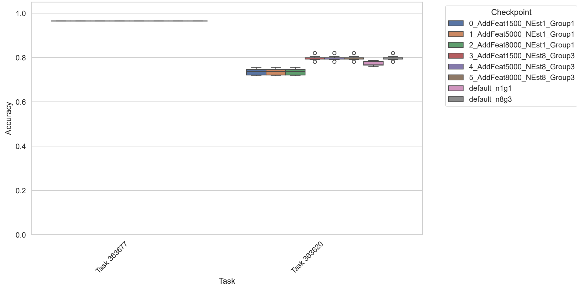
openml - accuracy per Task
