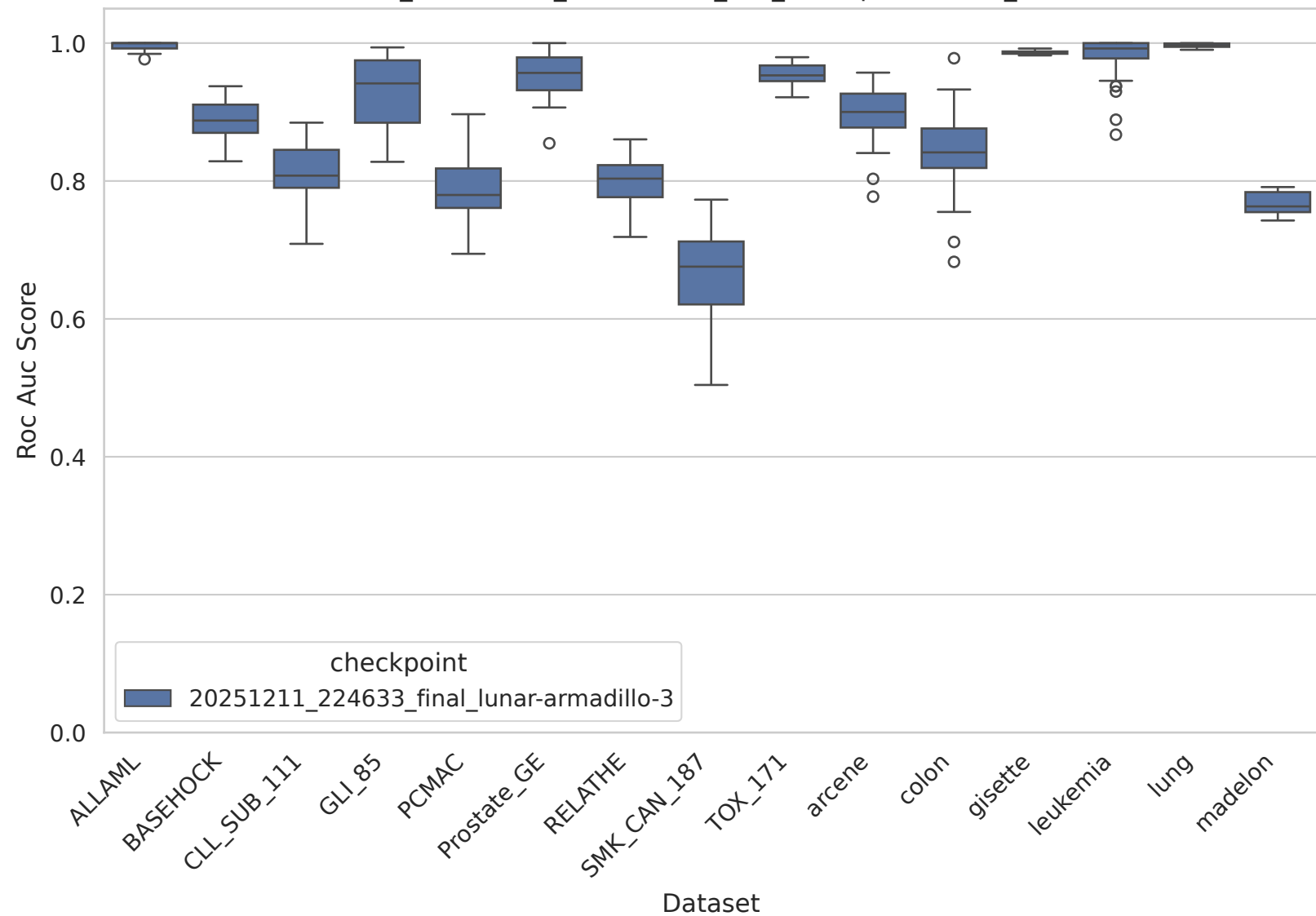
hdlss_benchmark_results - roc_auc_score per dataset_name
