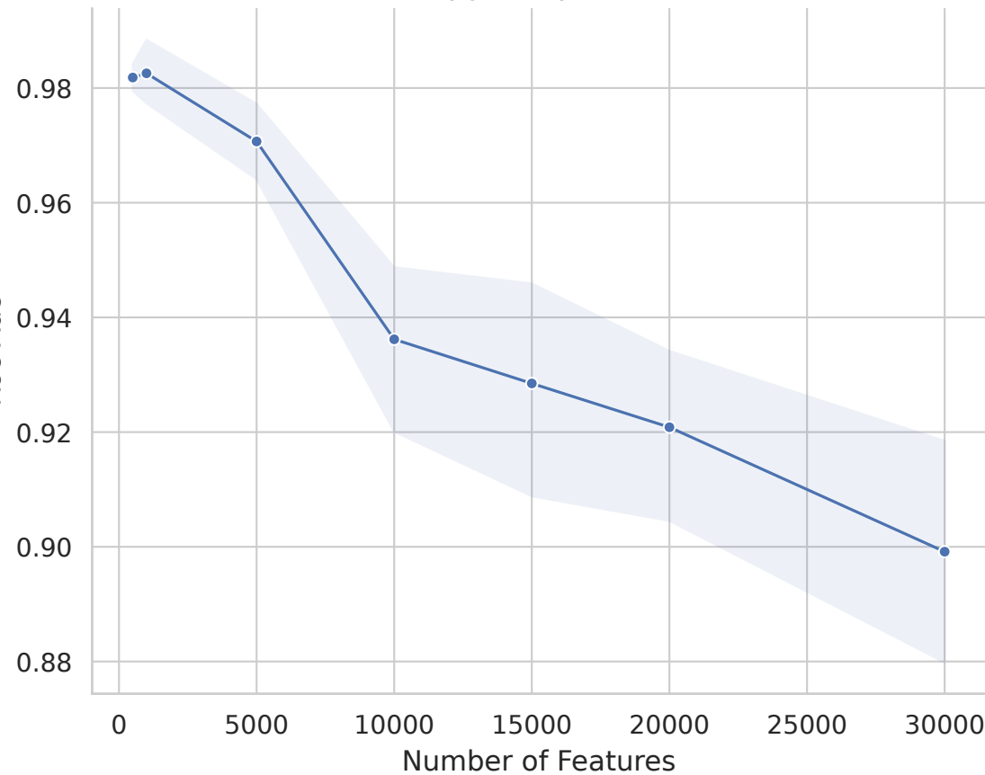
Polygenicity: 0.001
