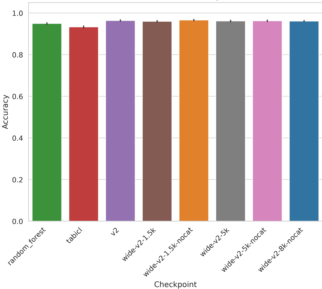
Task 363702 - Accuracy
