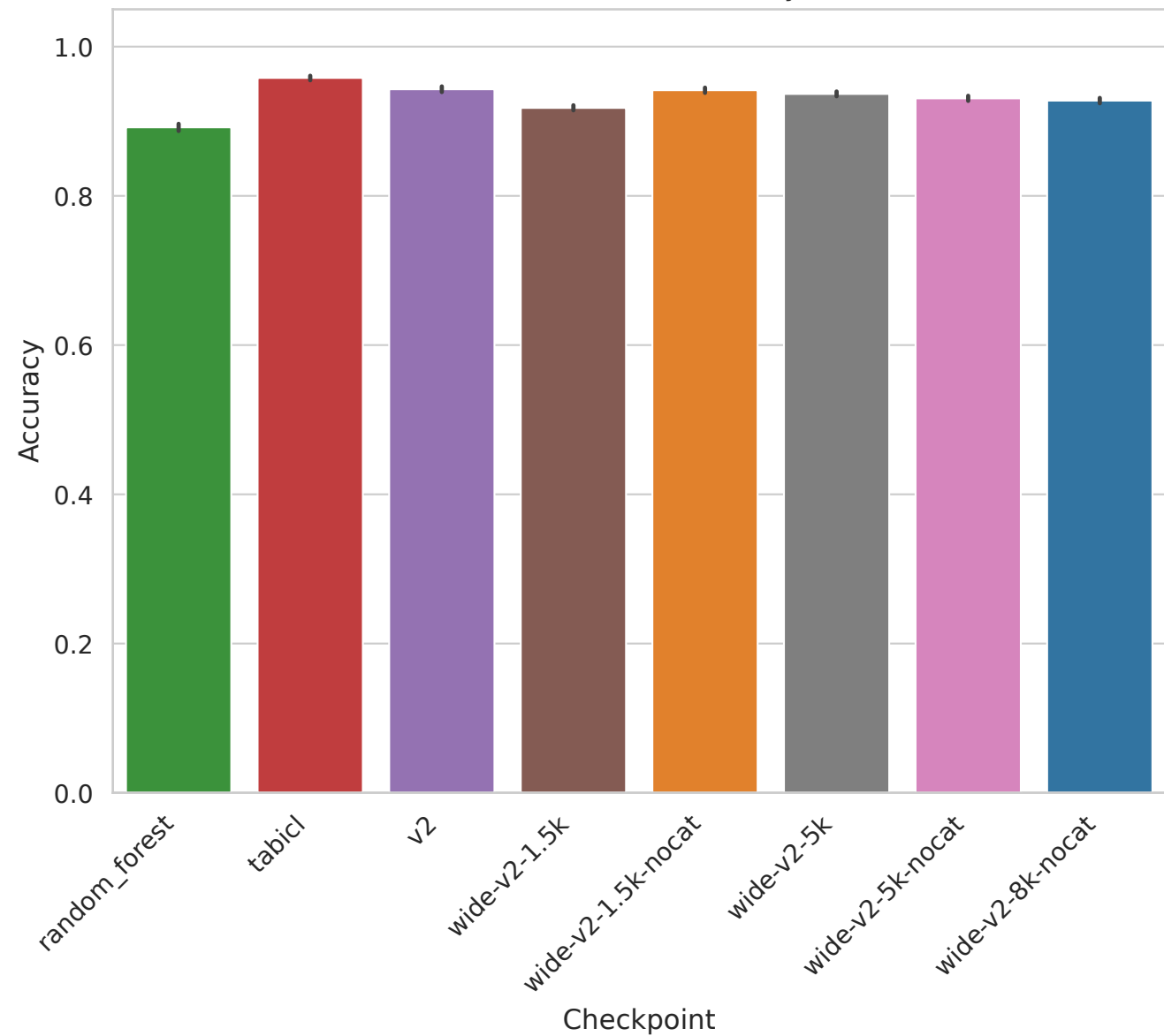
Task 363674 - Accuracy
