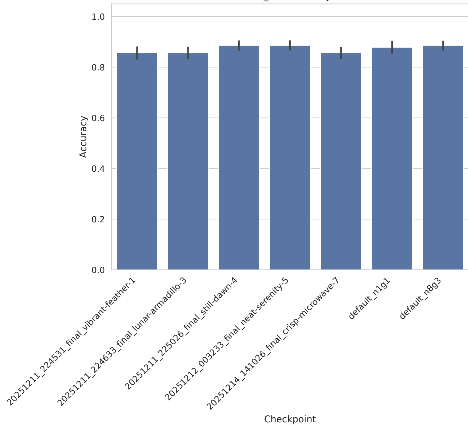
GLI_85 - Accuracy
