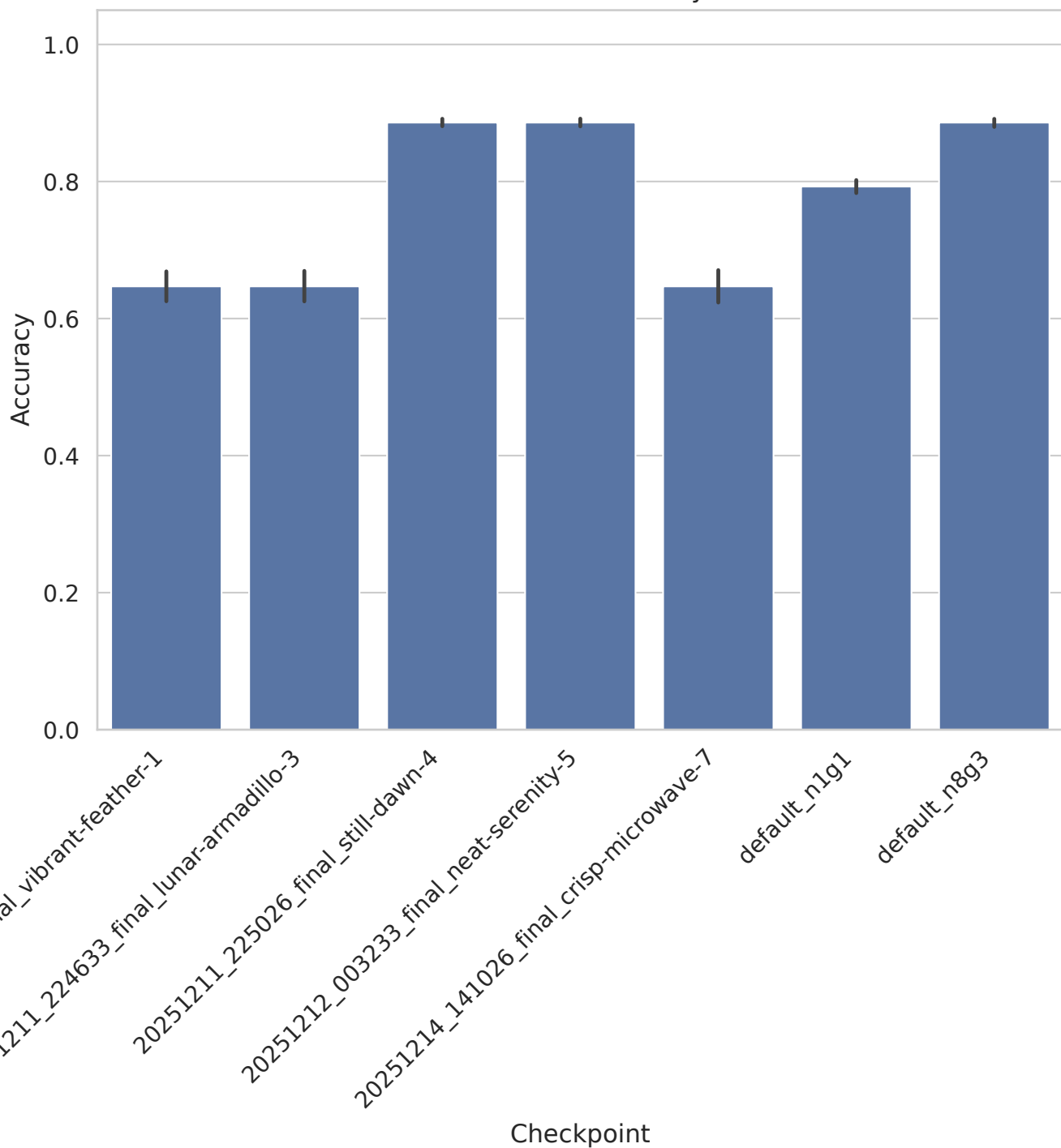
RELATHE - Accuracy
