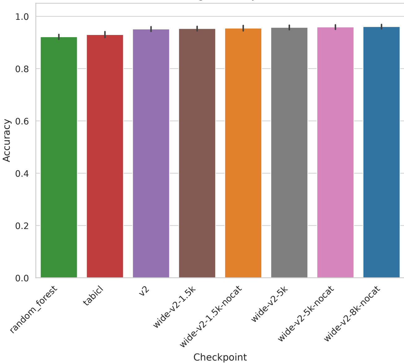
lung - Accuracy
