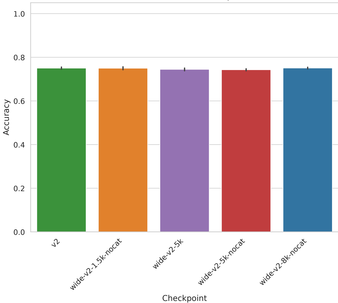
Task 363626 - Accuracy
