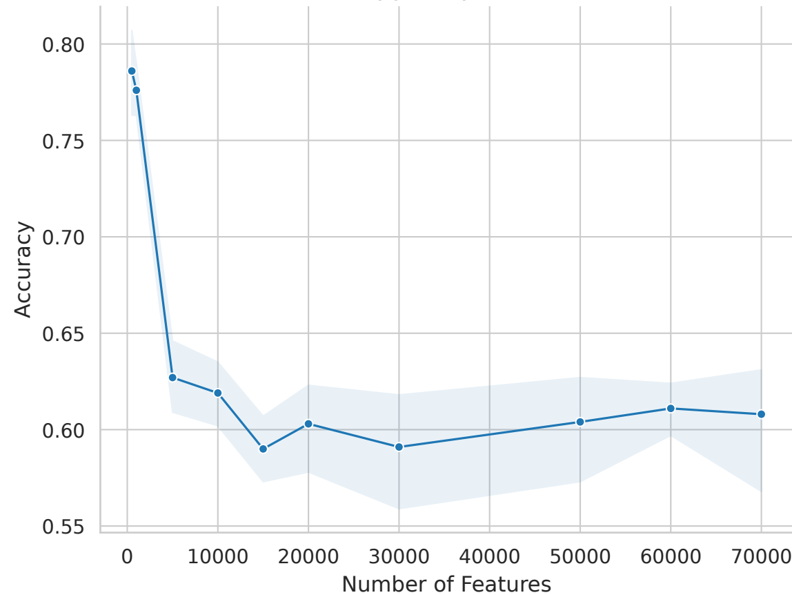
Polygenicity: 0.001
