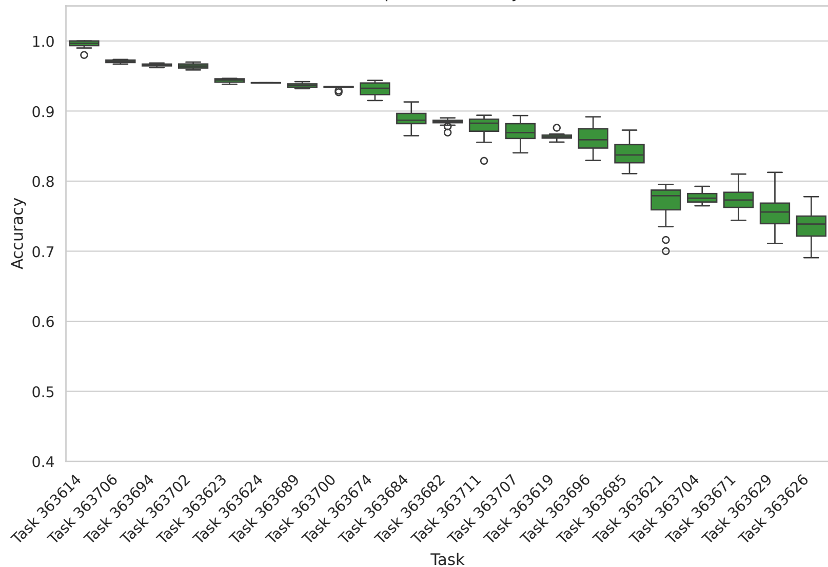
openml - accuracy
