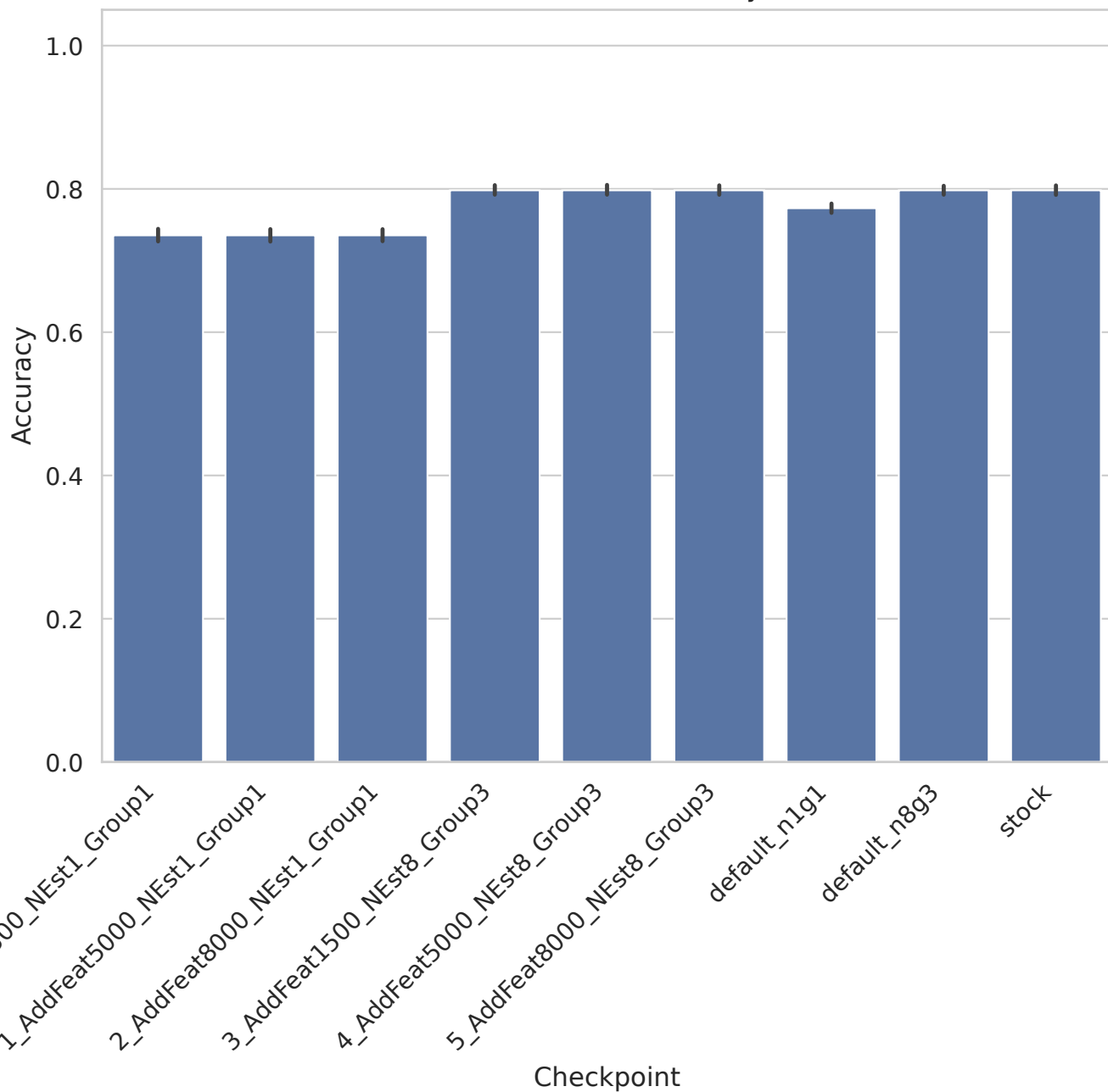
Task 363620 - Accuracy
