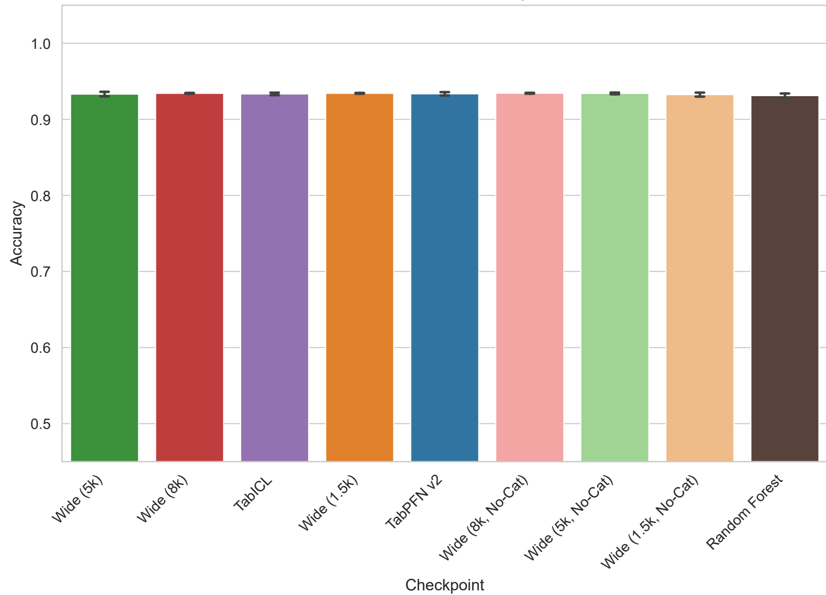
Task 363700 - Accuracy
