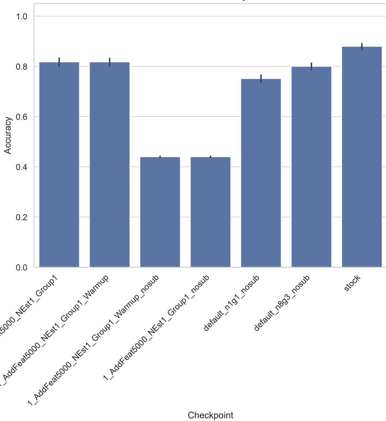
arcene - Accuracy
