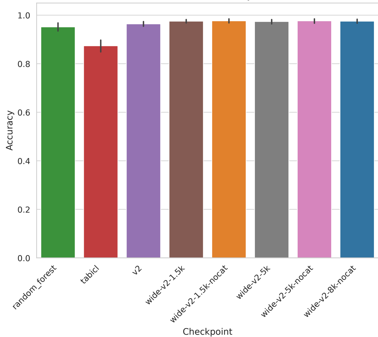
leukemia - Accuracy
