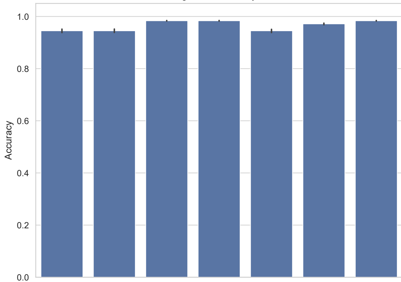
gisette - Accuracy
