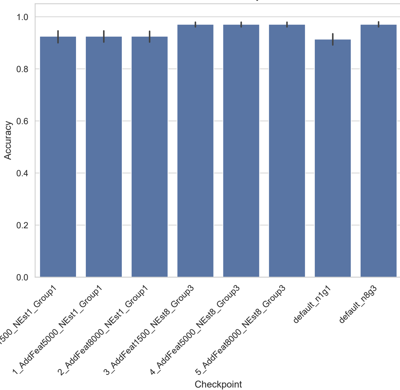
leukemia - Accuracy
