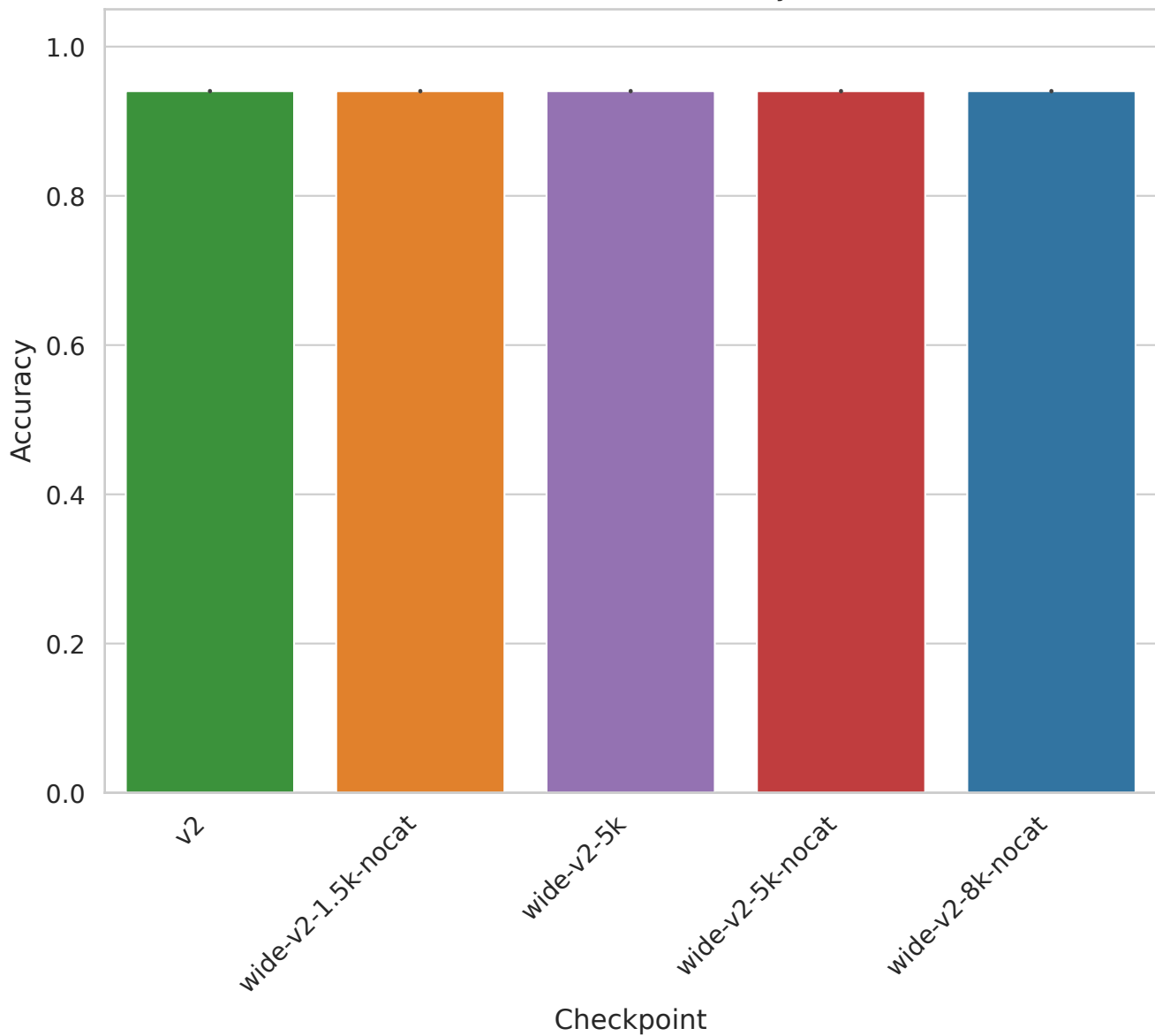
Task 363624 - Accuracy
