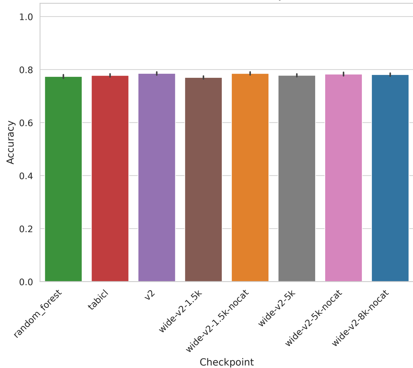
Task 363704 - Accuracy
