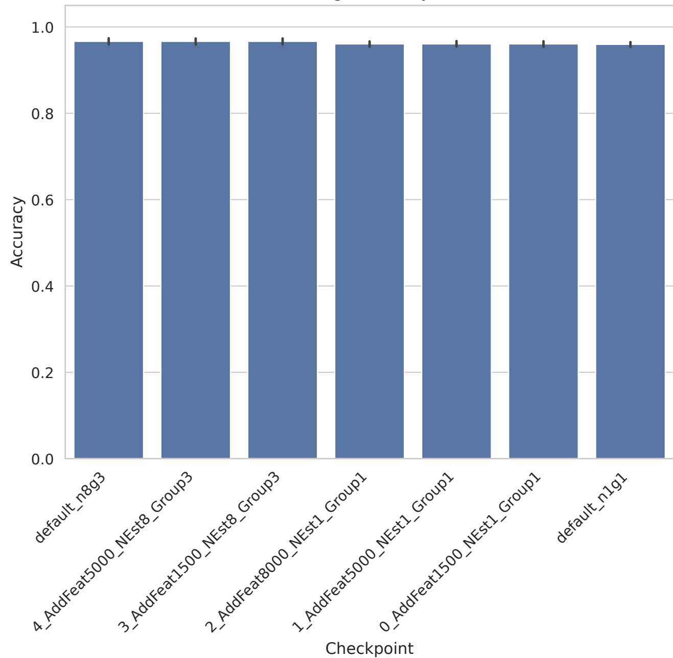
lung - Accuracy
