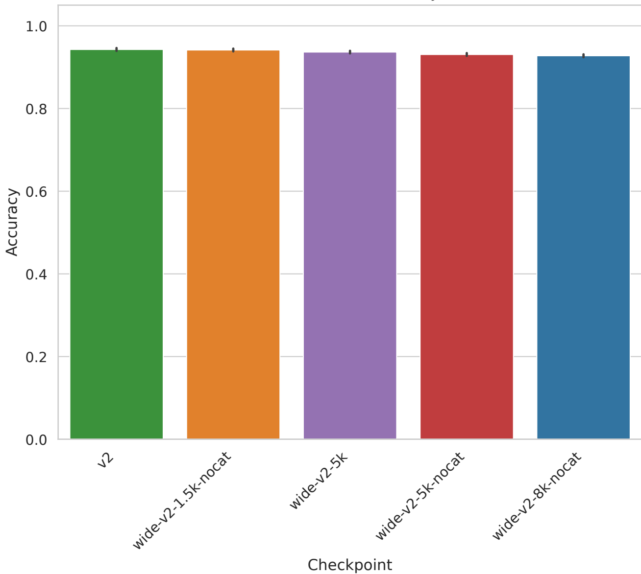
Task 363674 - Accuracy
