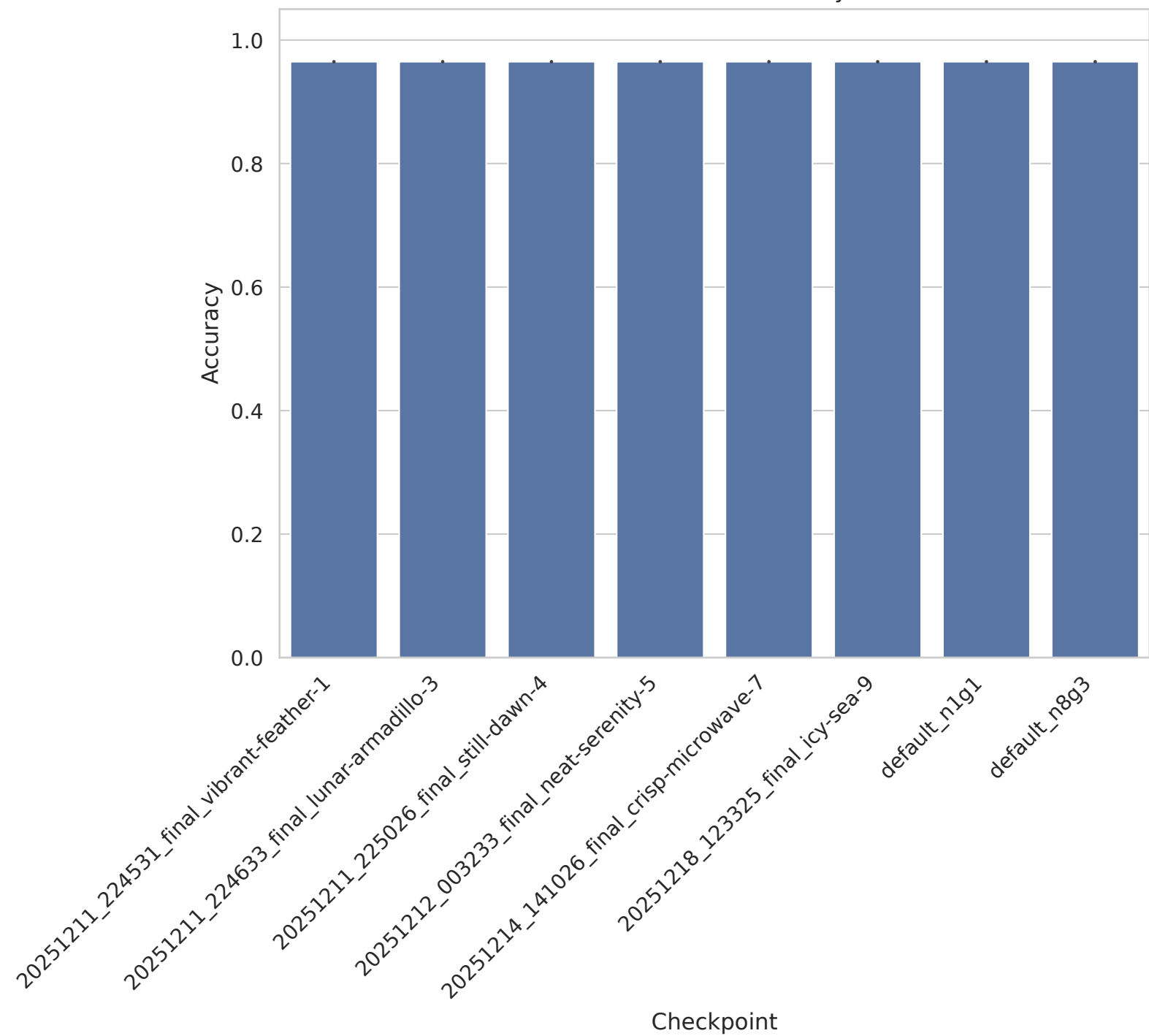
Task 363677 - Accuracy
