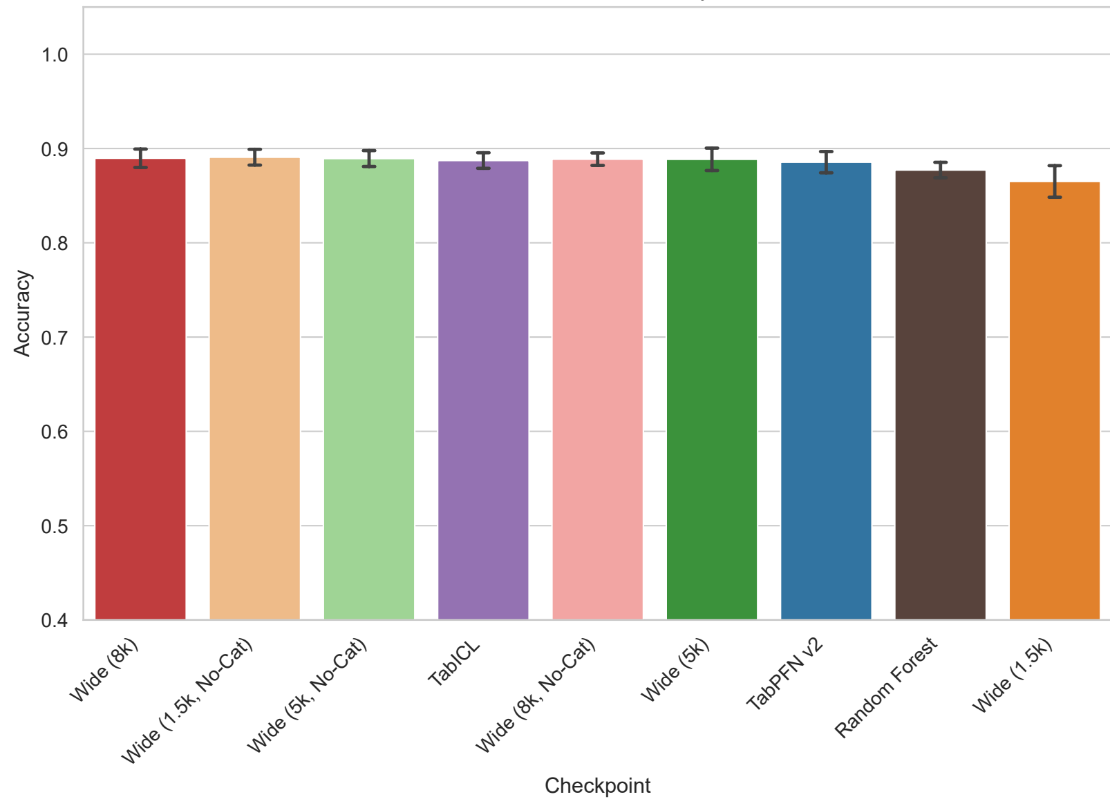
Task 363684 - Accuracy
