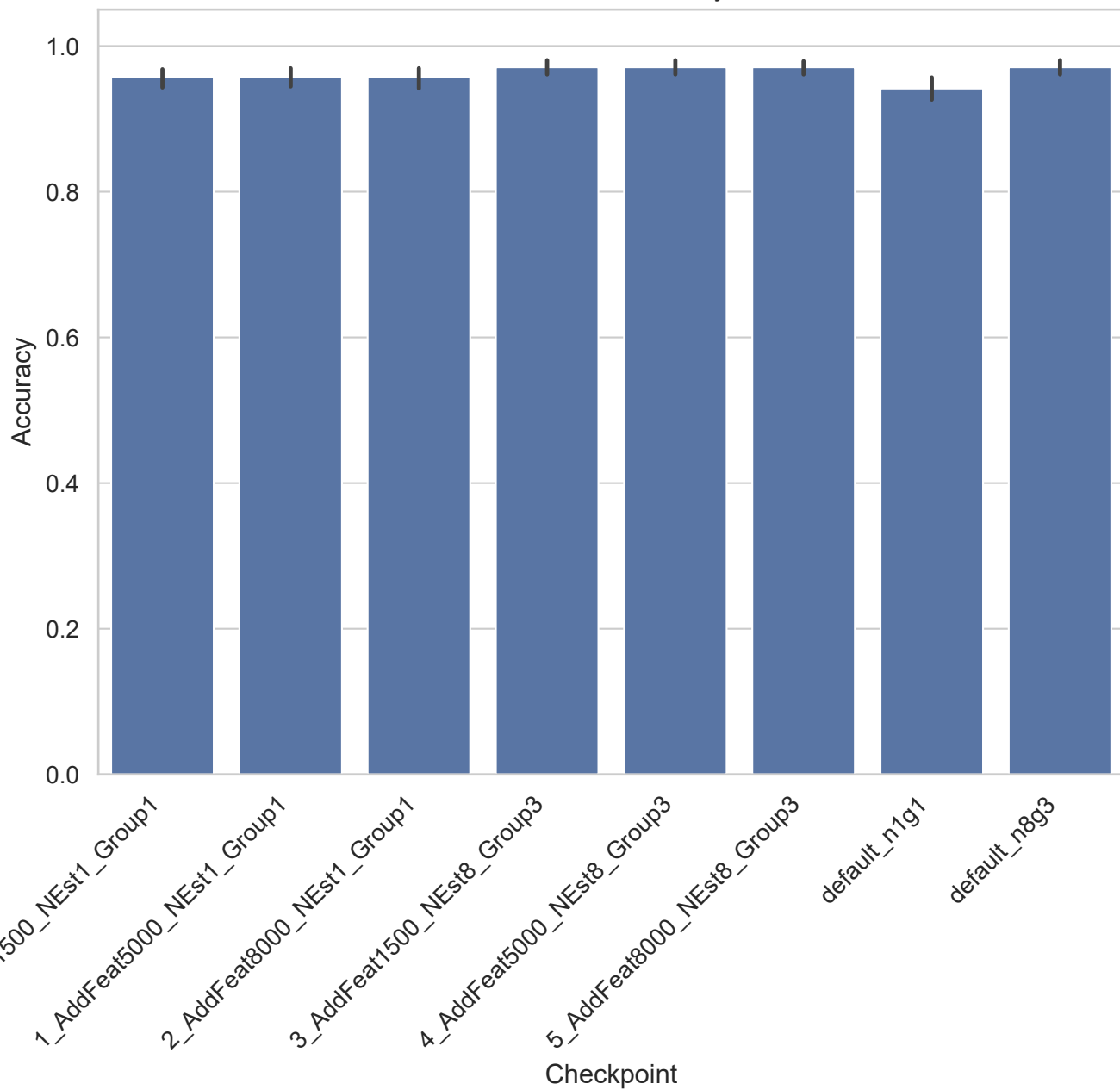
ALLAML - Accuracy
