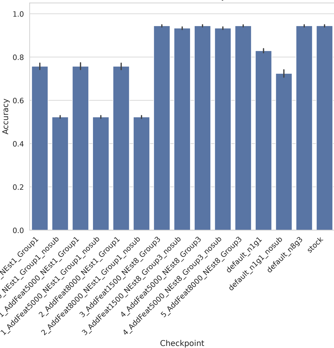
BASEHOCK - Accuracy
