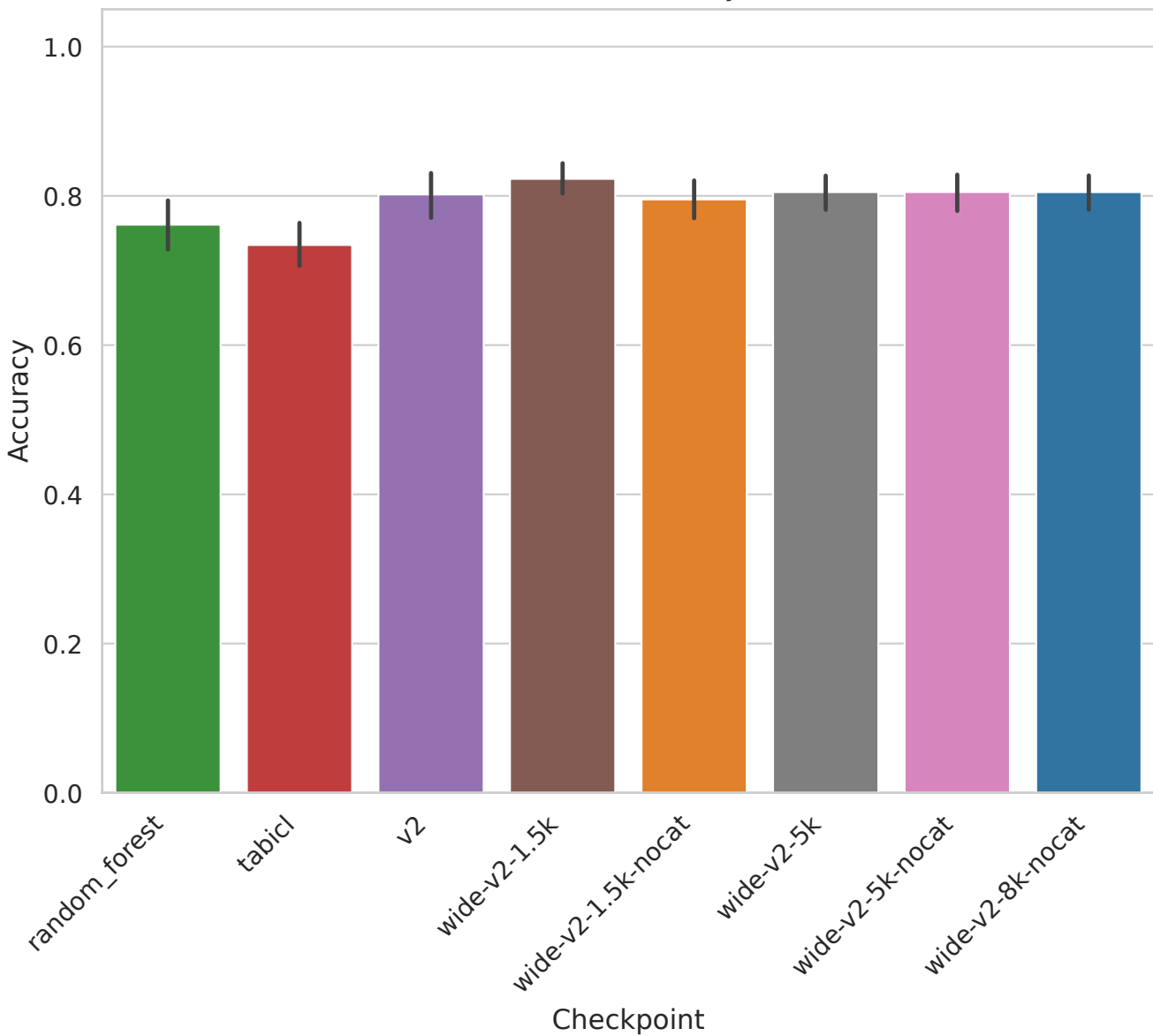
colon - Accuracy
