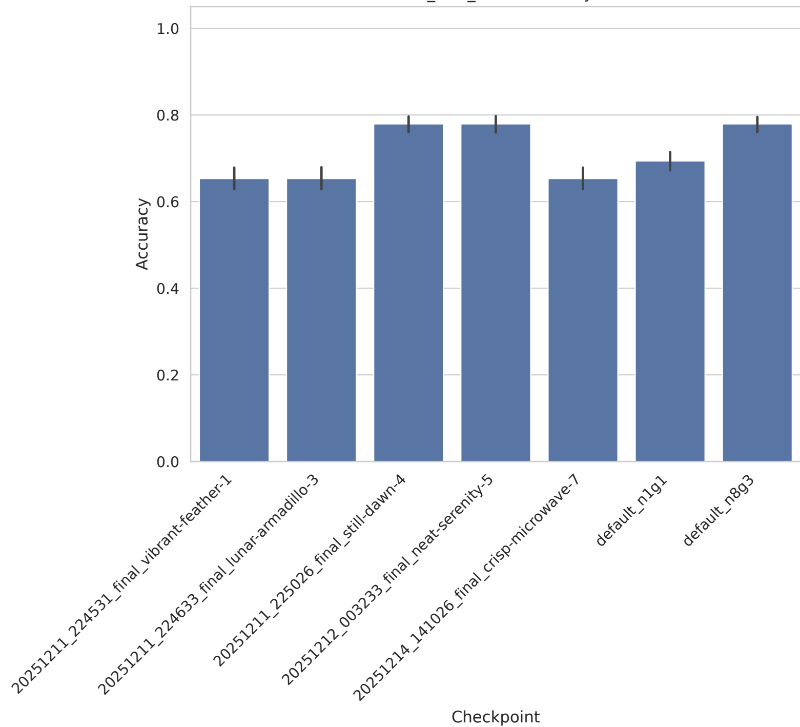
CLL_SUB_111 - Accuracy
