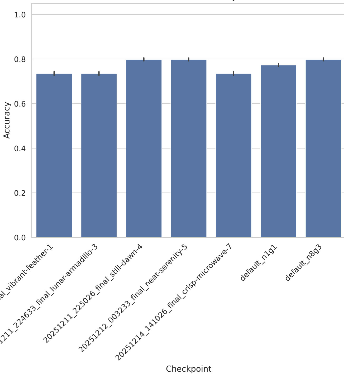
Task 363620 - Accuracy
