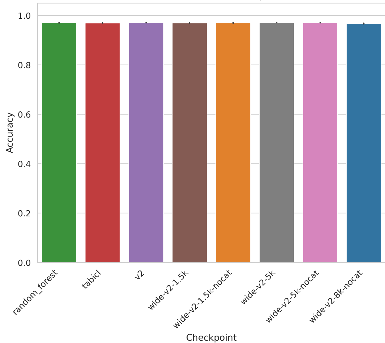
Task 363706 - Accuracy
