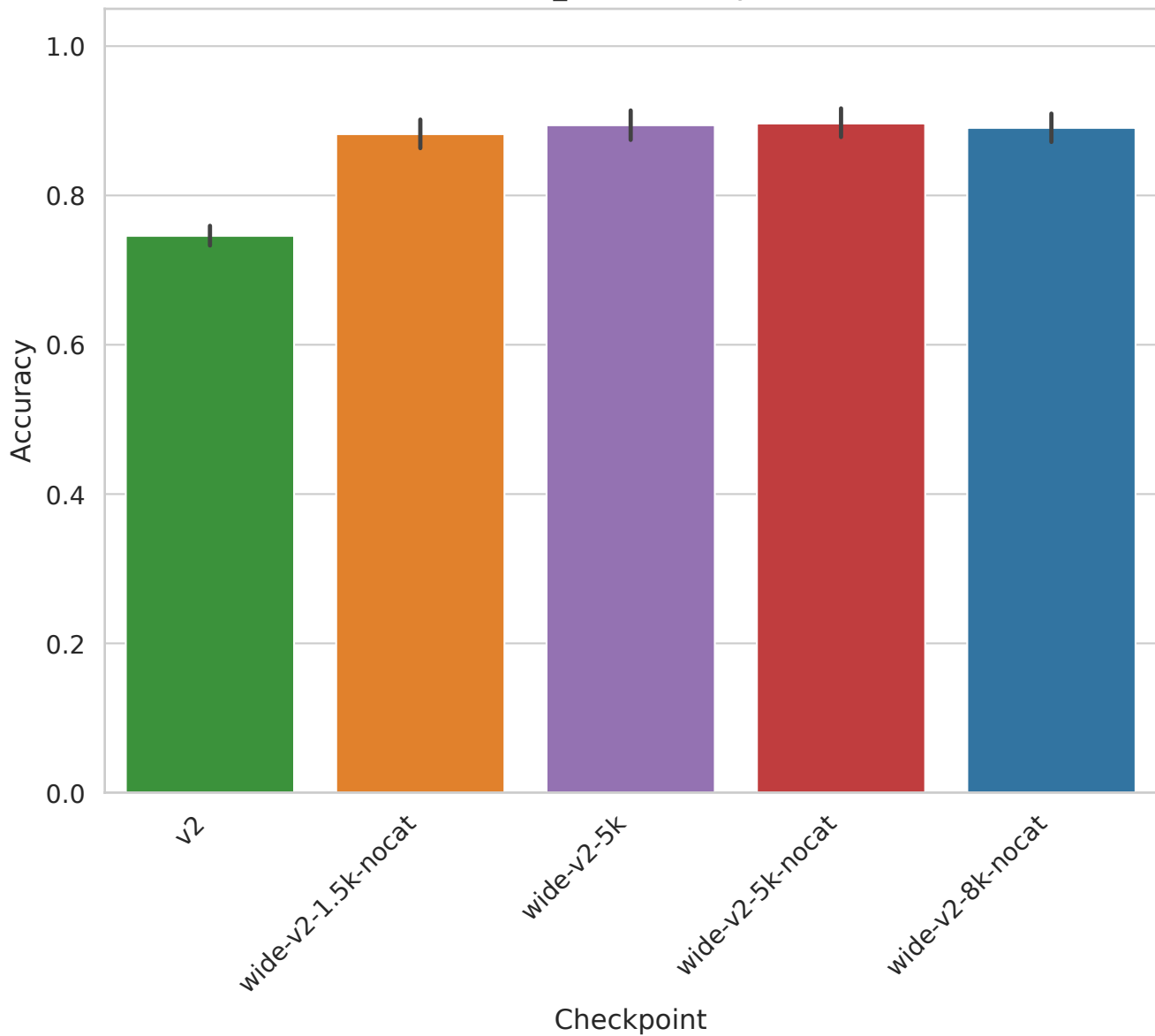
GLI_85 - Accuracy
