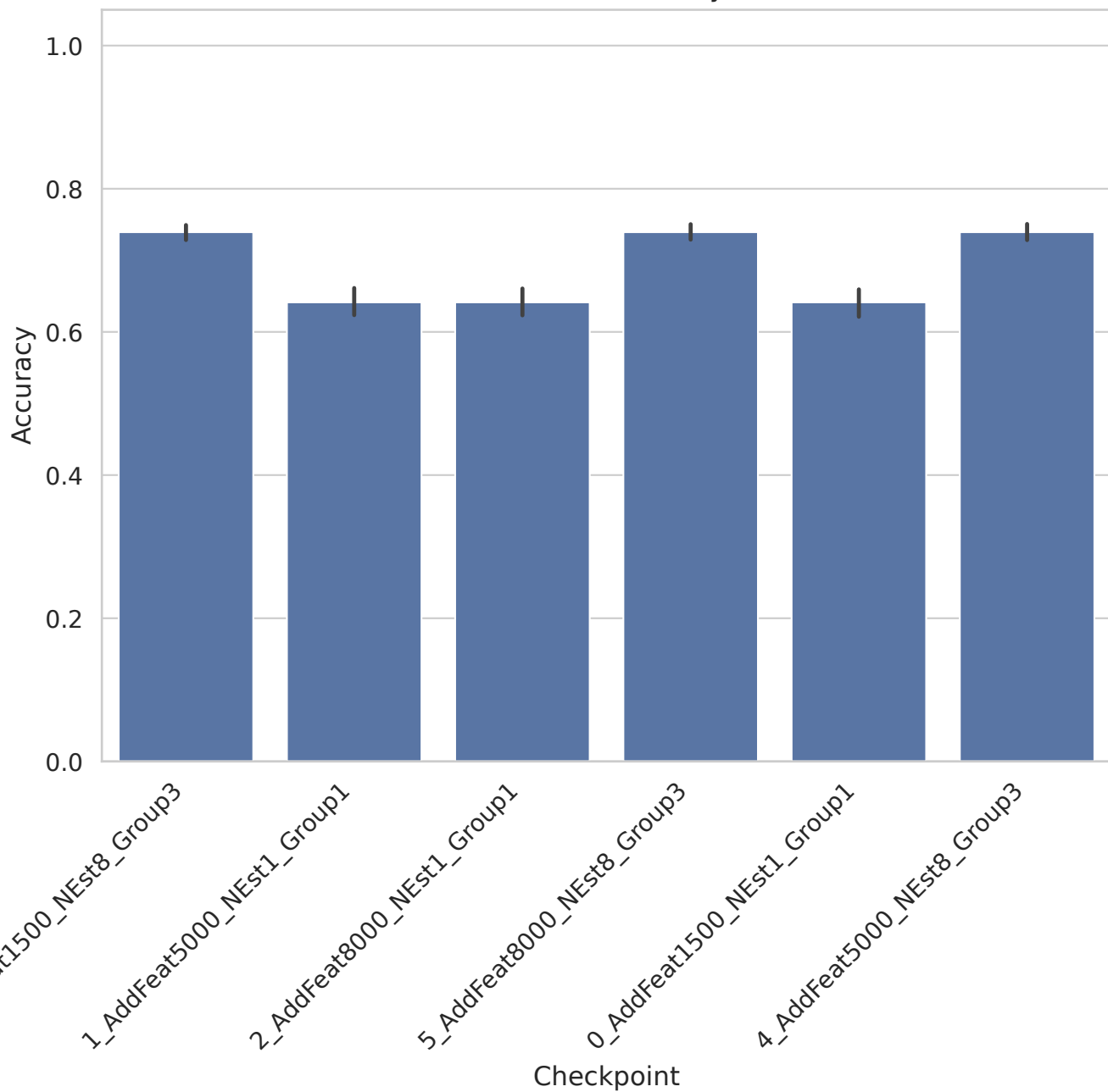
PCMAC - Accuracy
