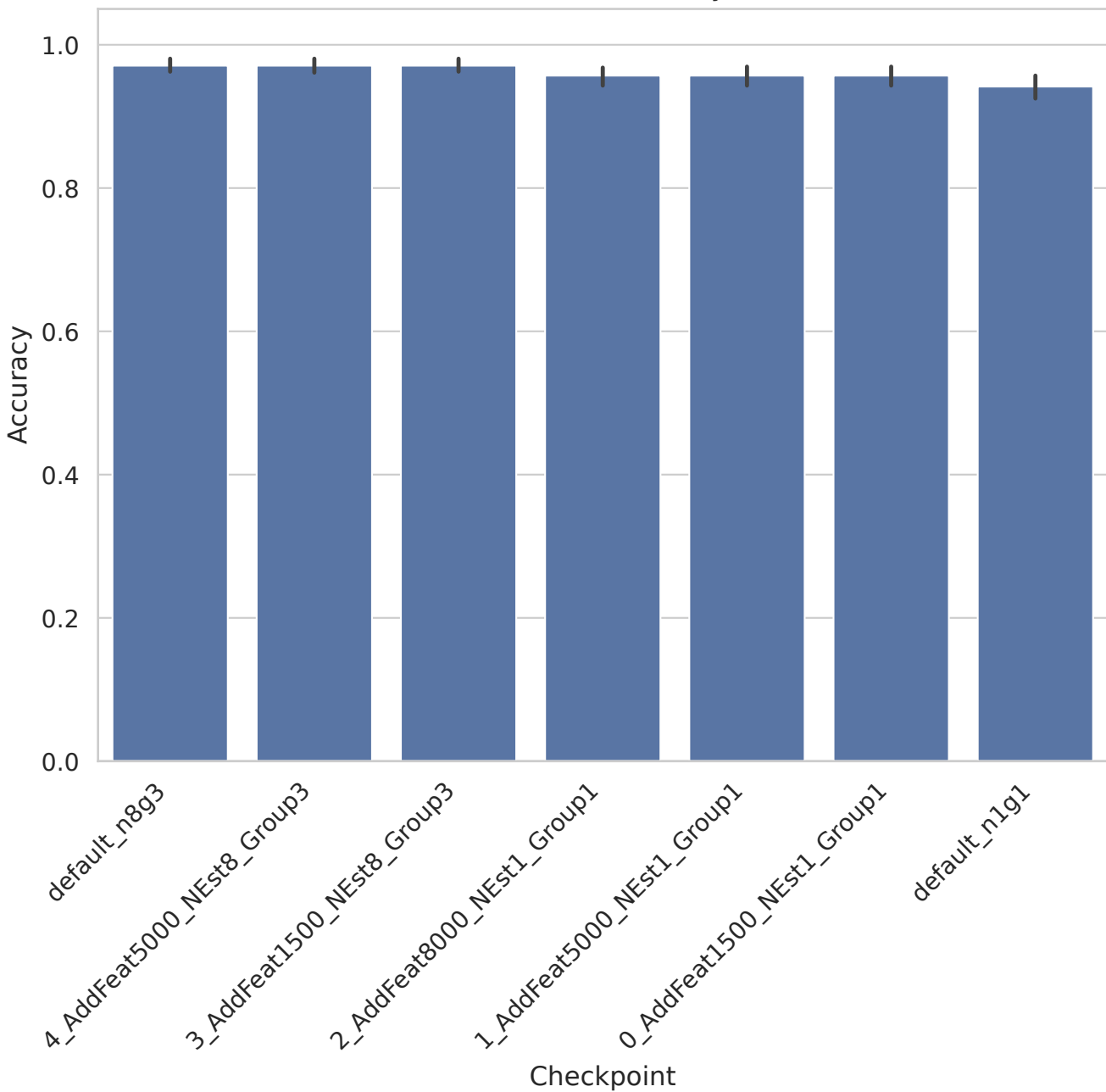
ALLAML - Accuracy
