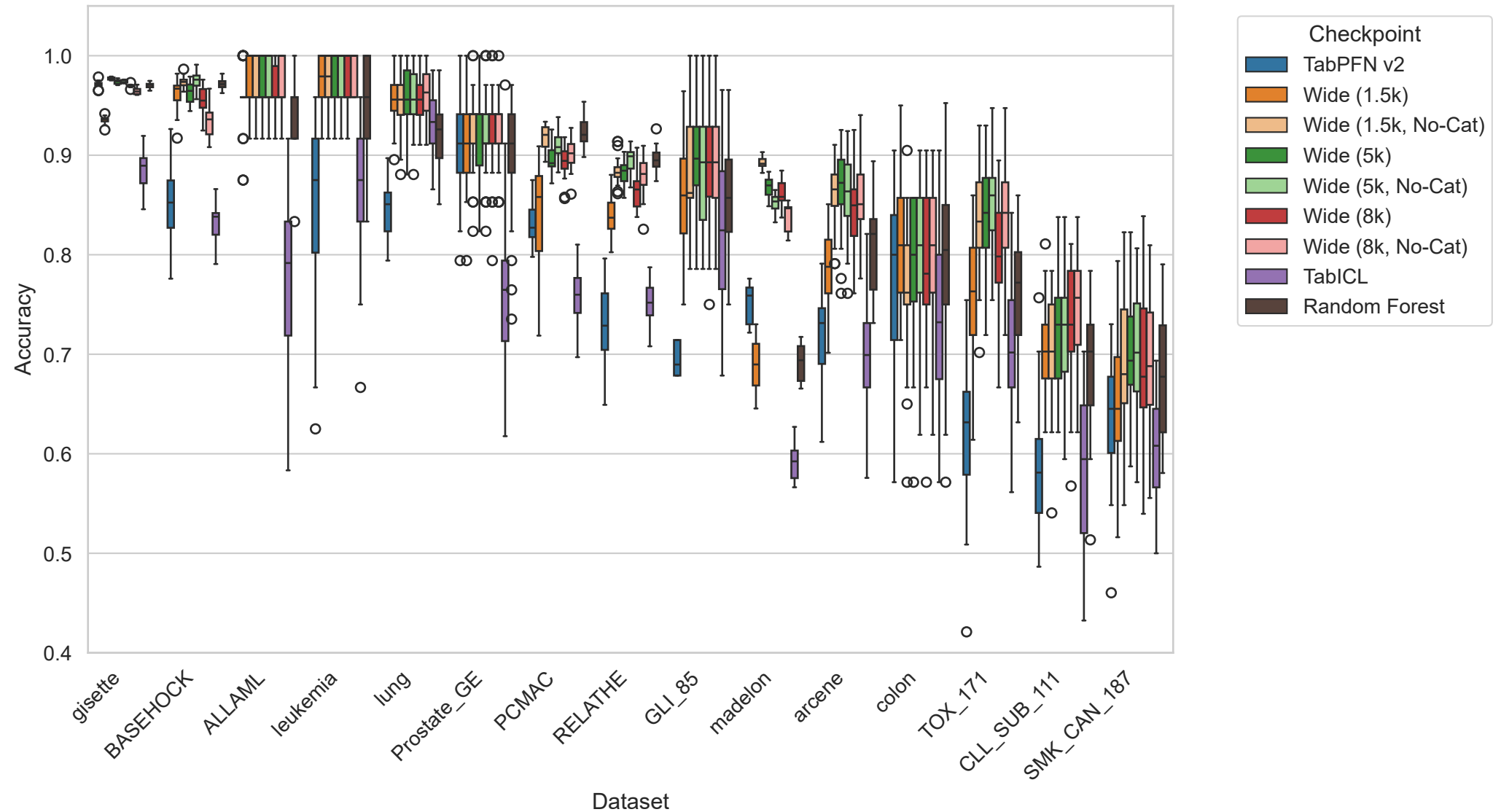
hdlss - accuracy
