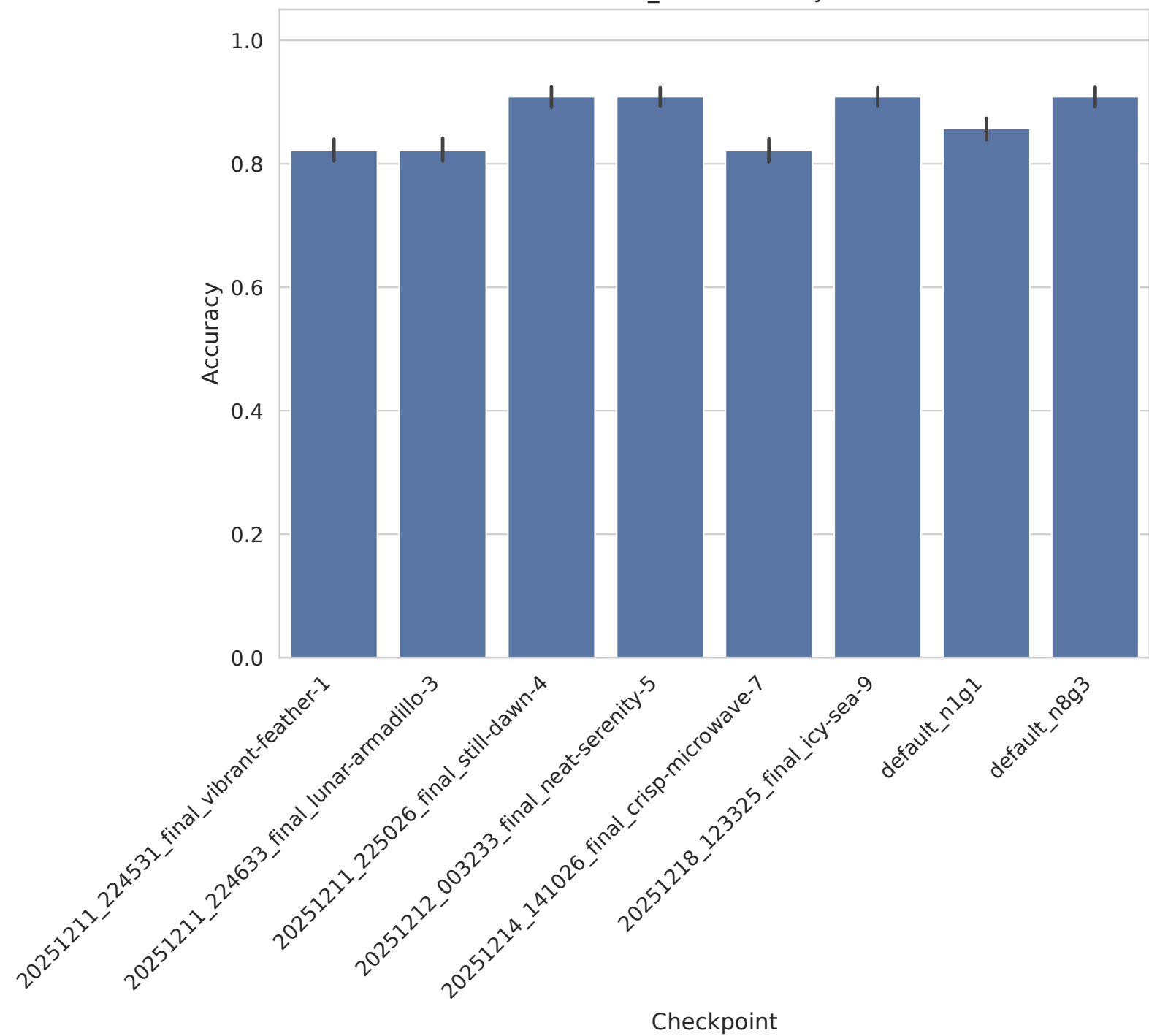
TOX_171 - Accuracy
