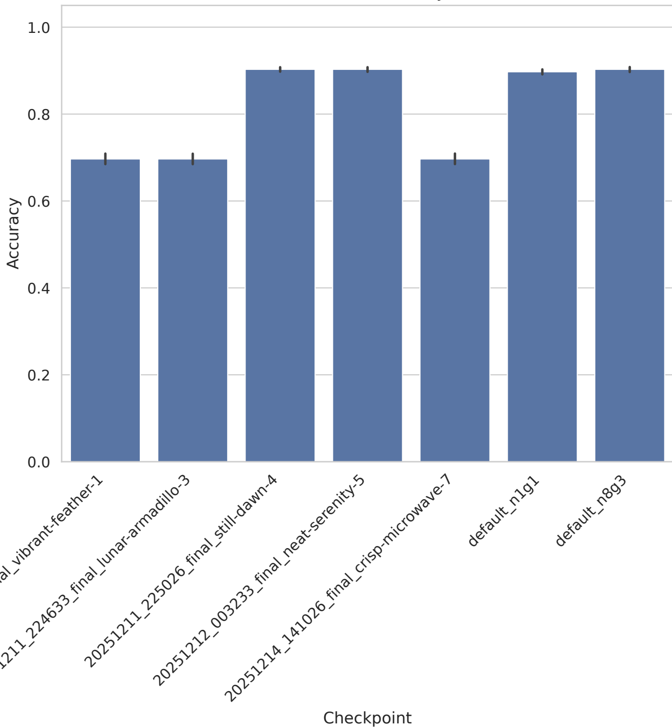
madelon - Accuracy
