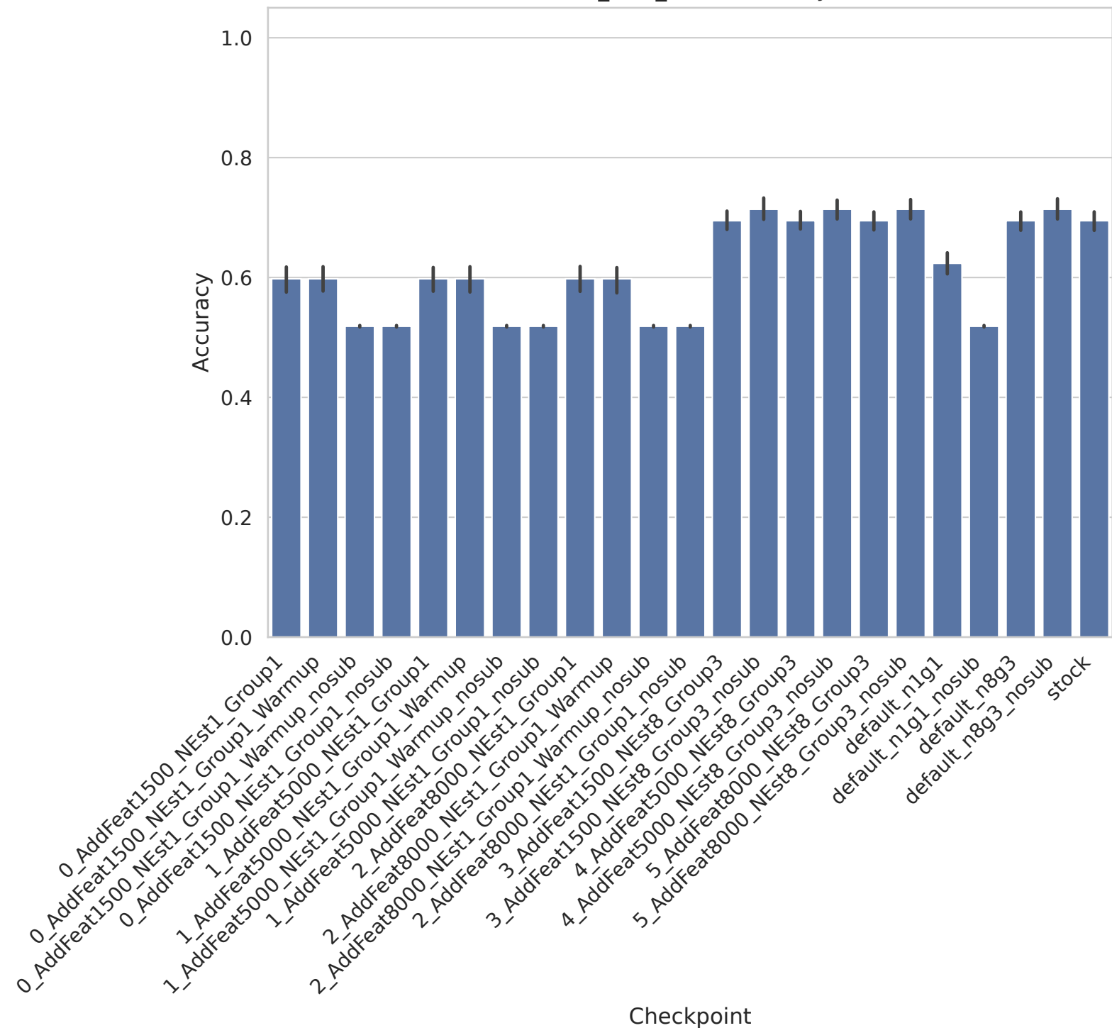
SMK_CAN_187 - Accuracy
