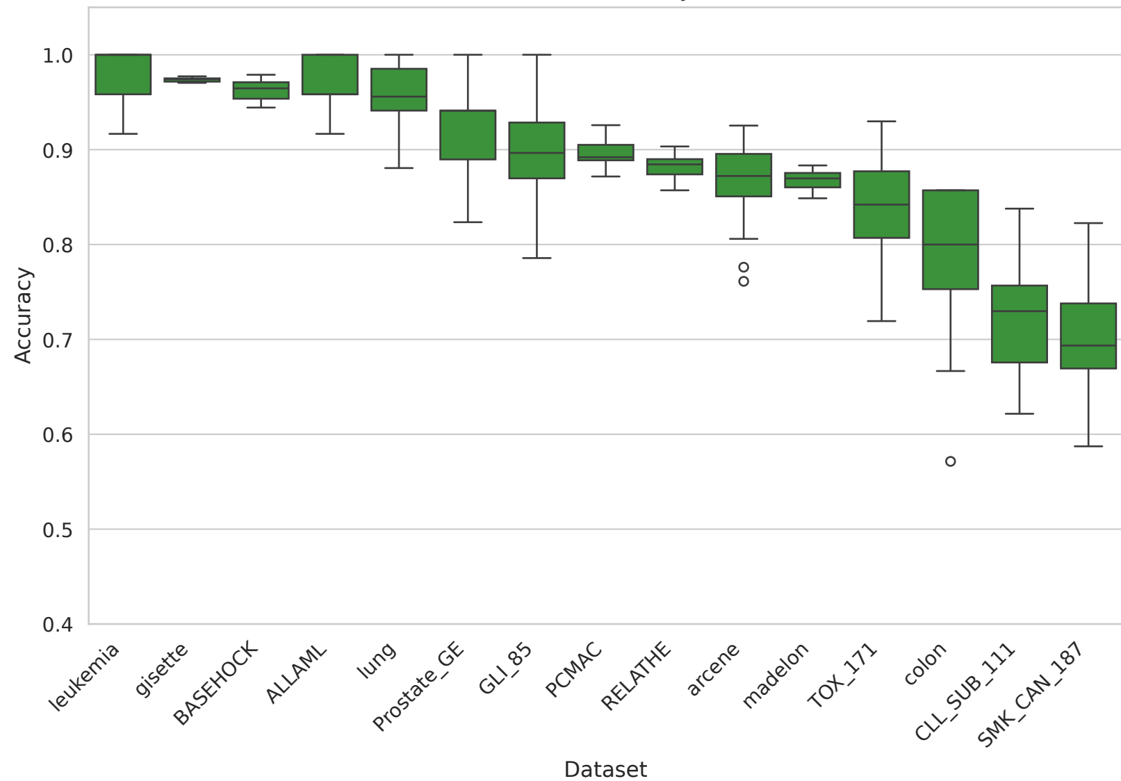
hdlss - accuracy
