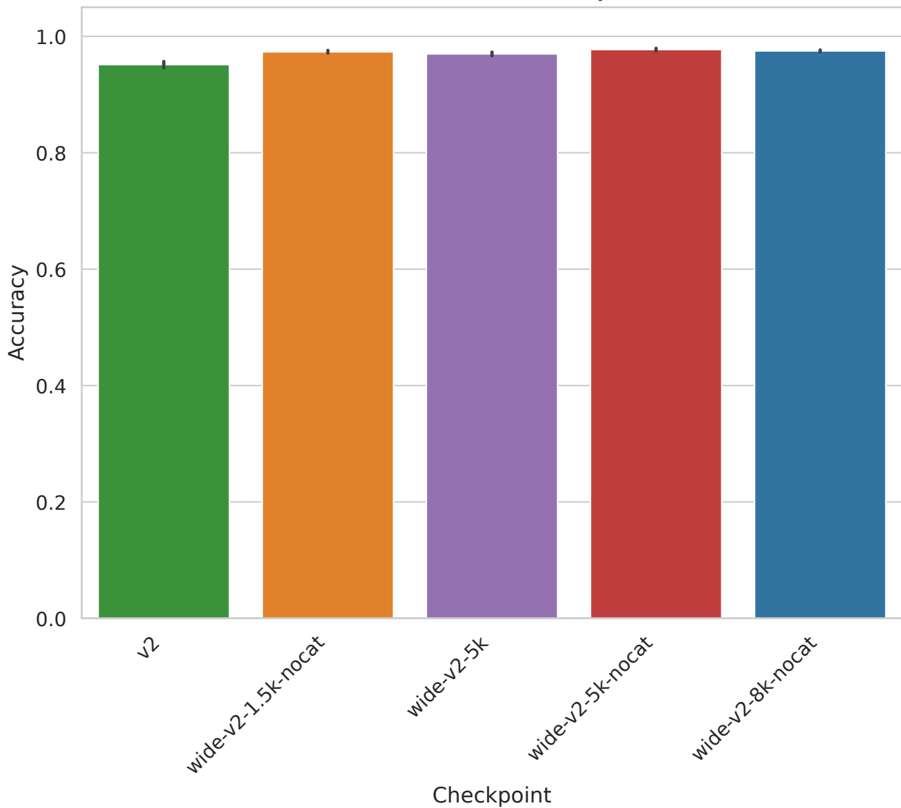
BASEHOCK - Accuracy
