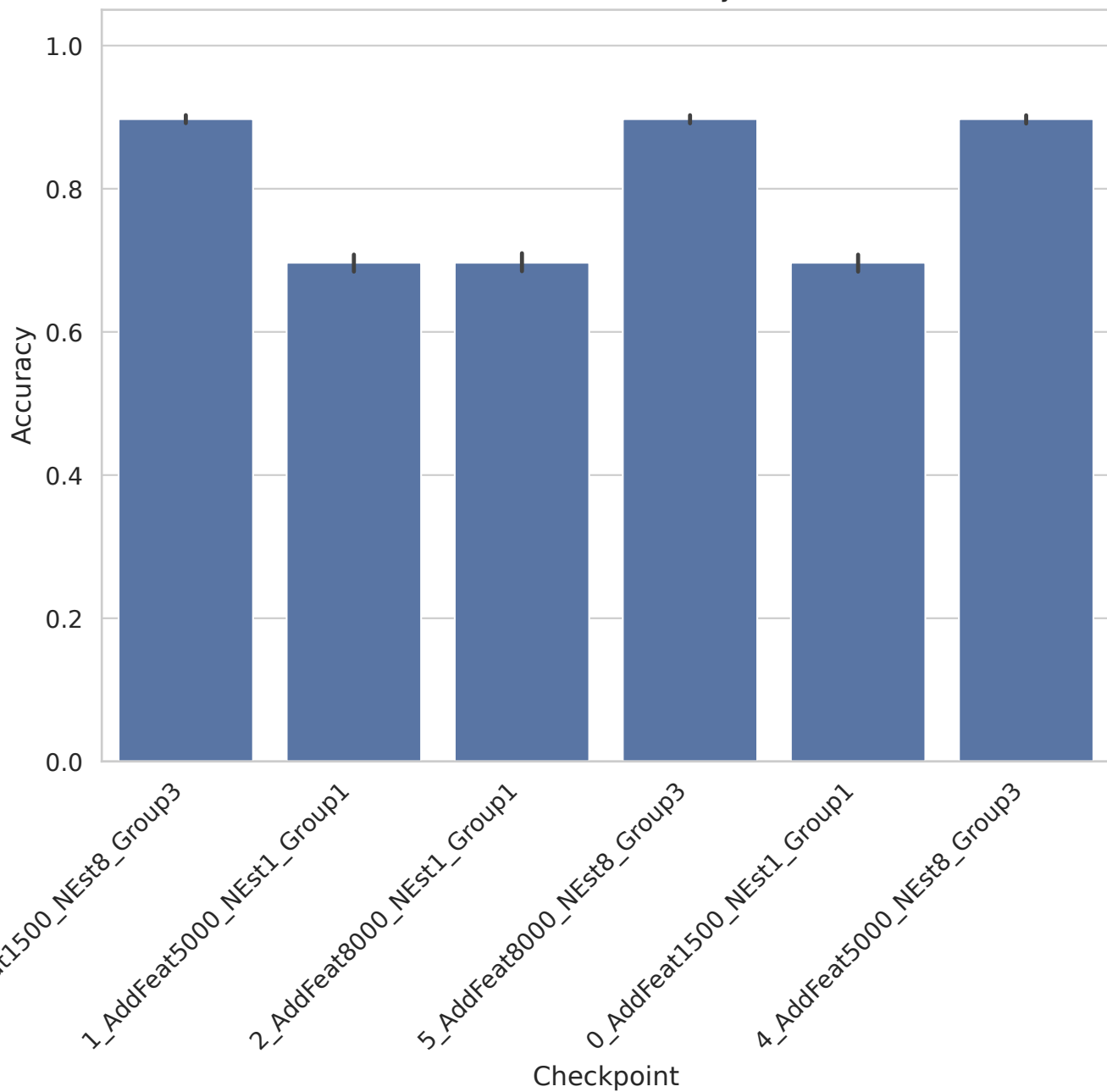
madelon - Accuracy
