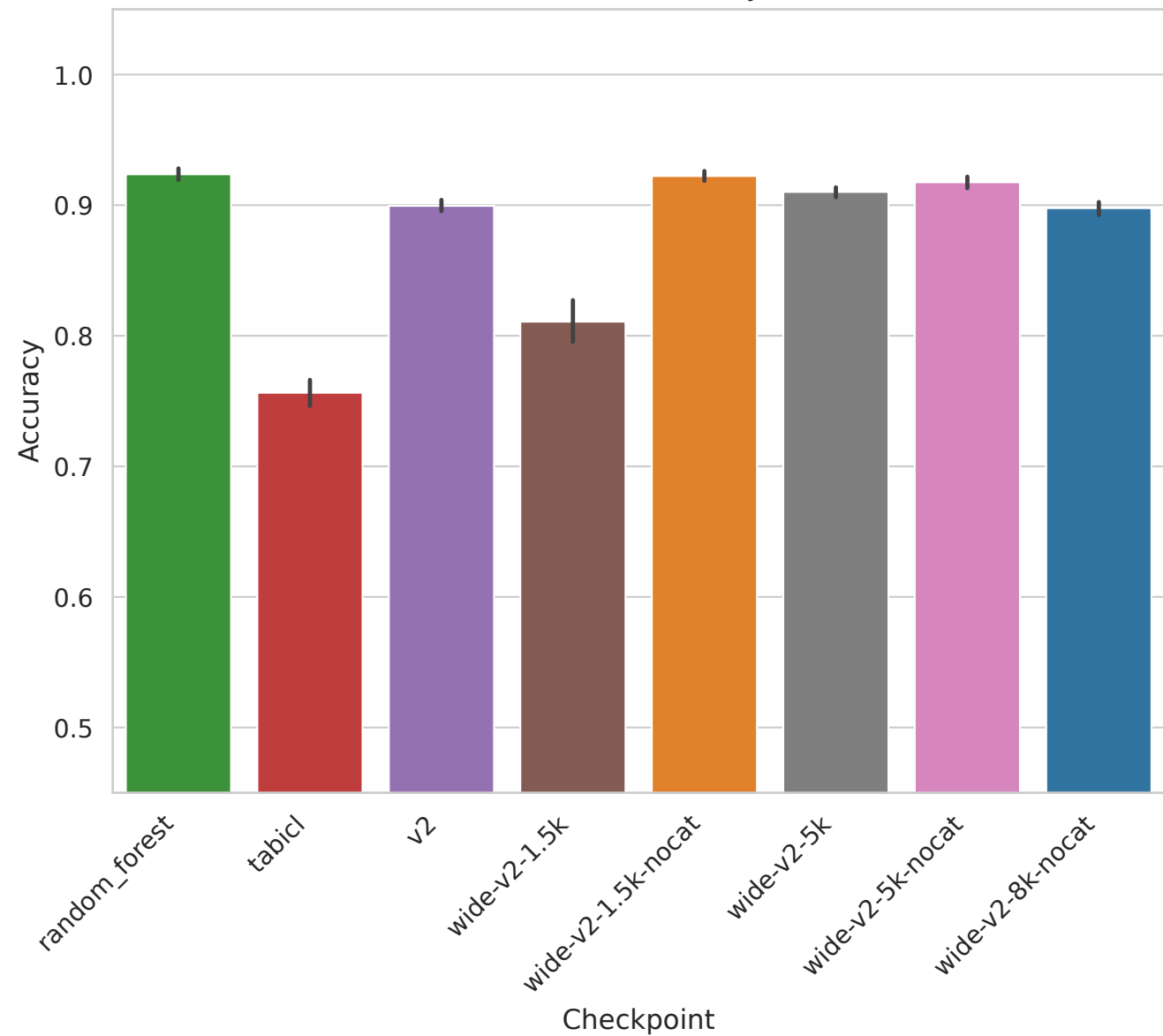
PCMAC - Accuracy
