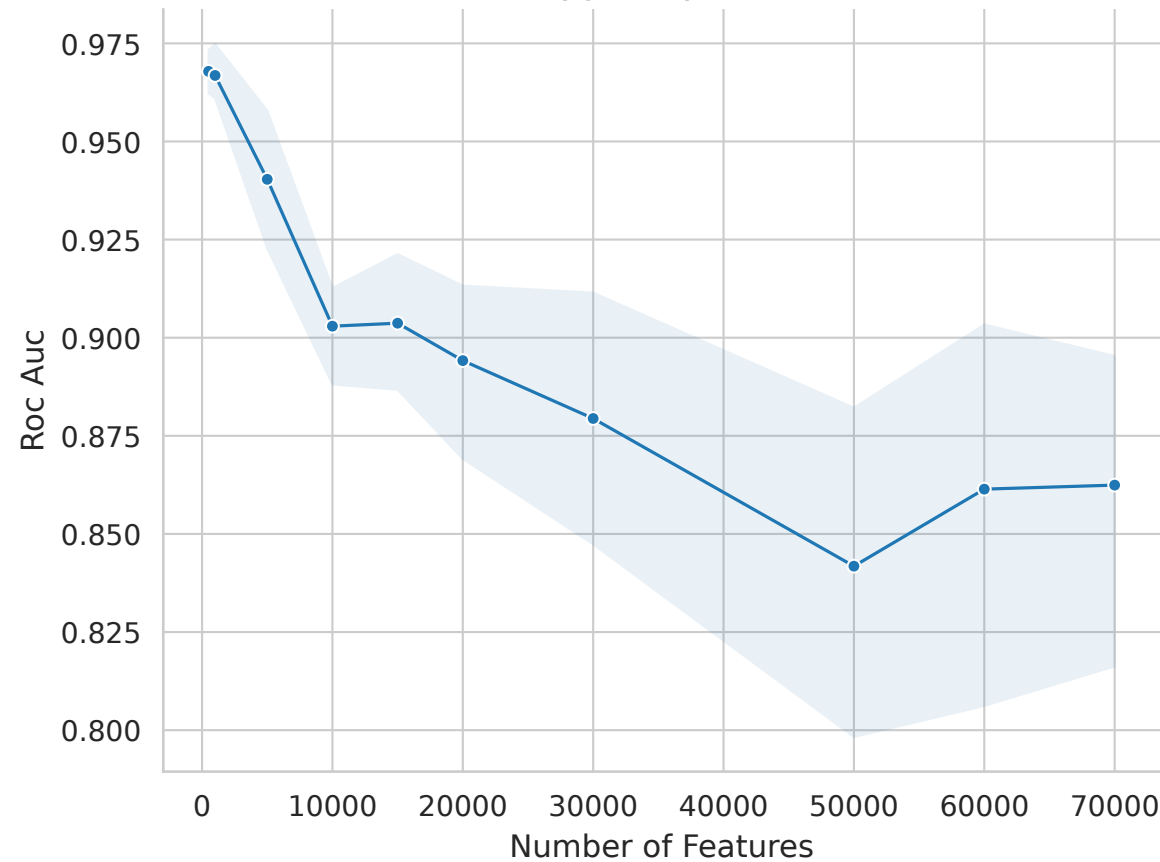
Polygenicity: 0.001
