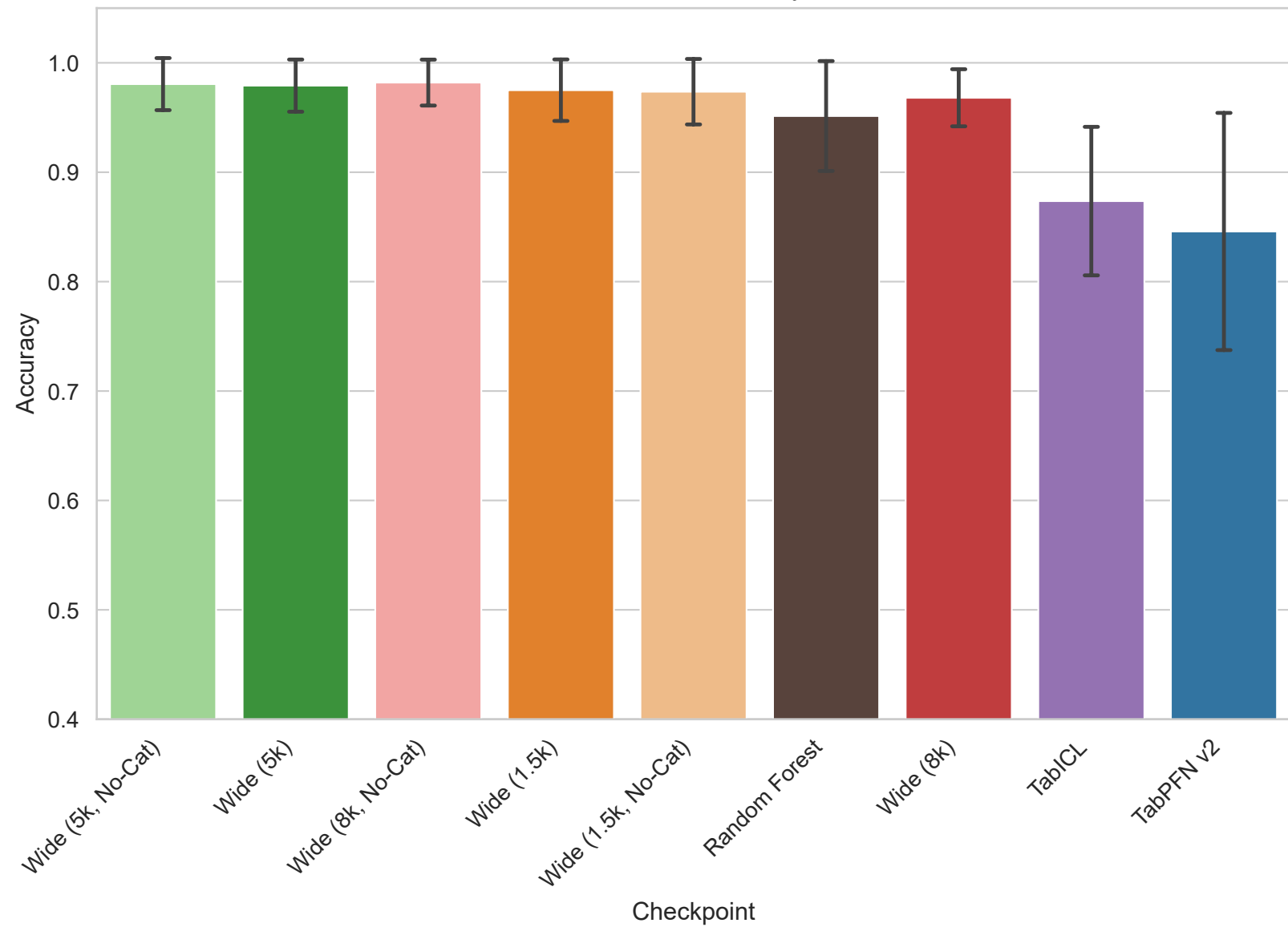
leukemia - Accuracy
