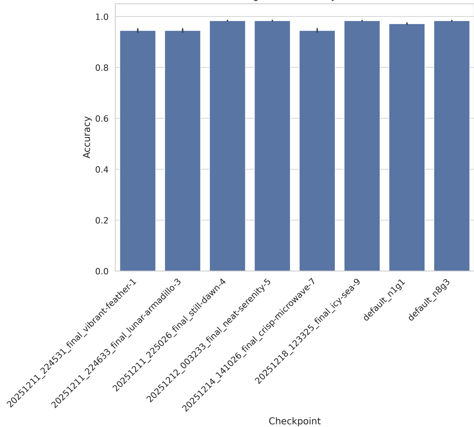
gisette - Accuracy
