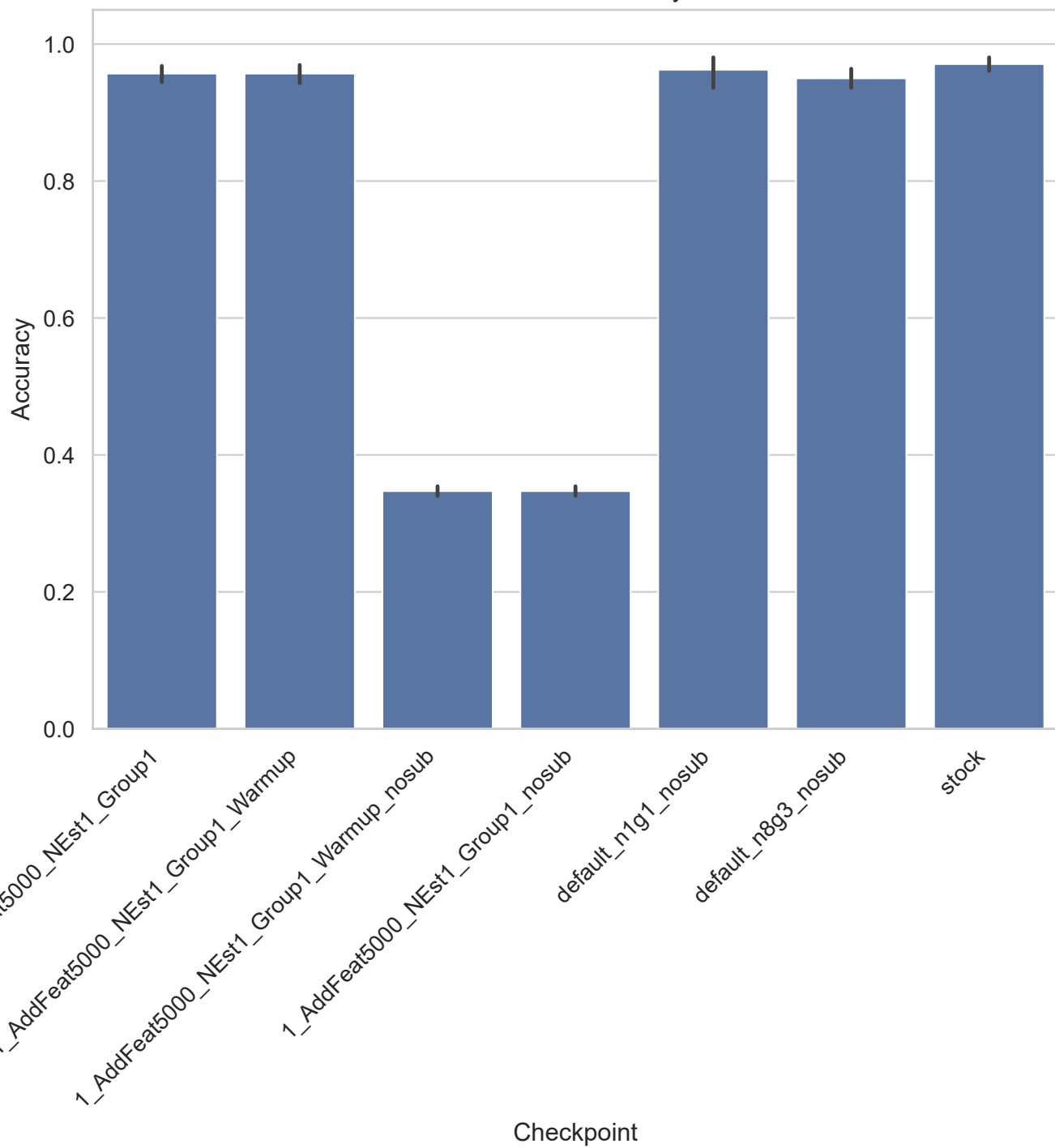
ALLAML - Accuracy
