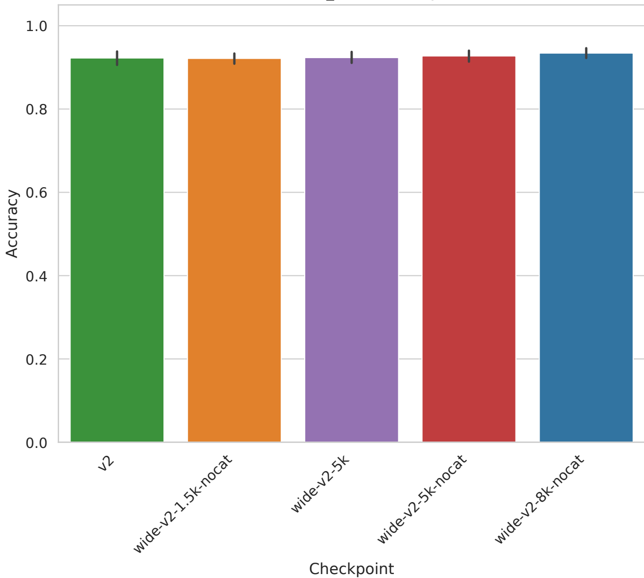
Prostate_GE - Accuracy
