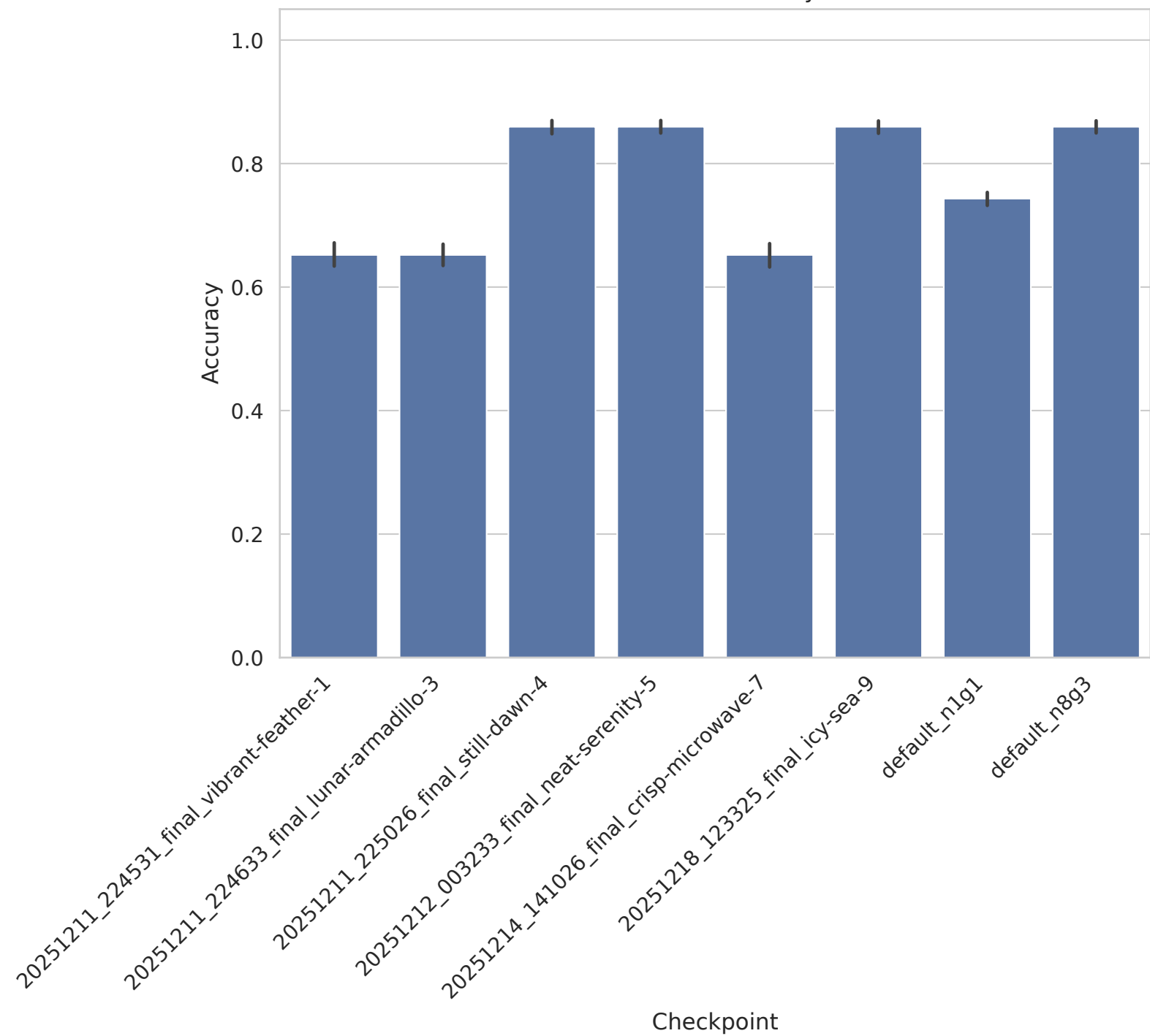
PCMAC - Accuracy
