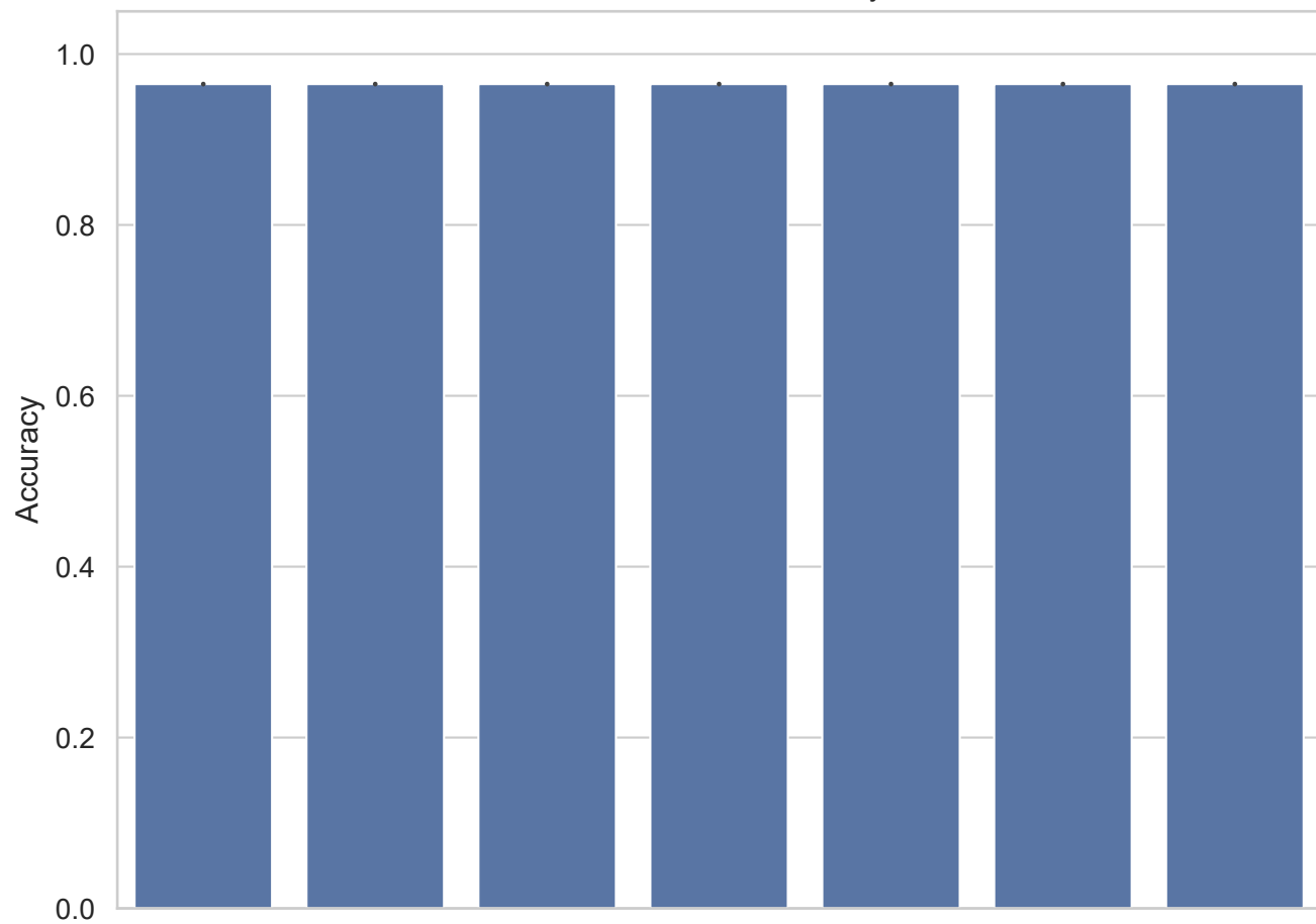
Task 363677 - Accuracy
