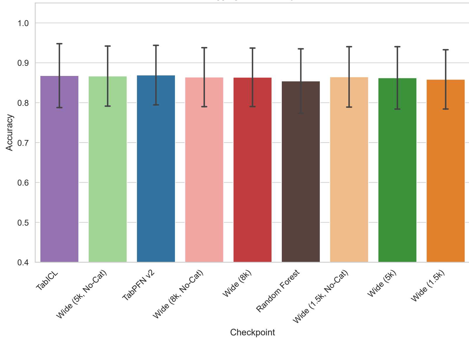
Aggregated Accuracy
