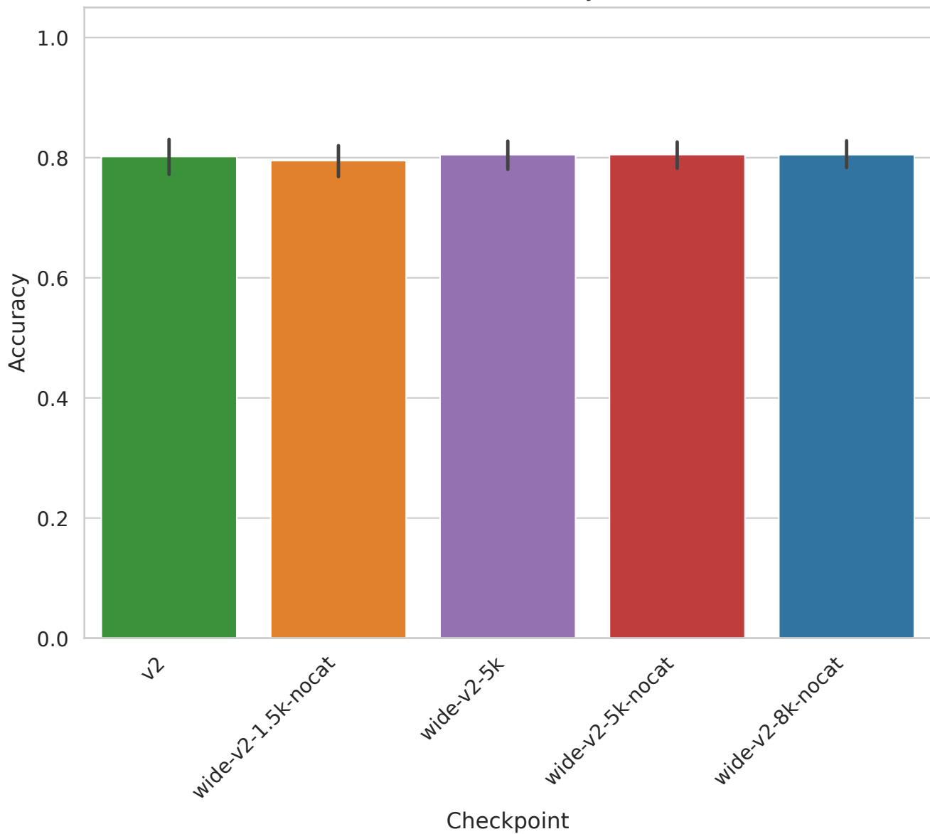
colon - Accuracy
