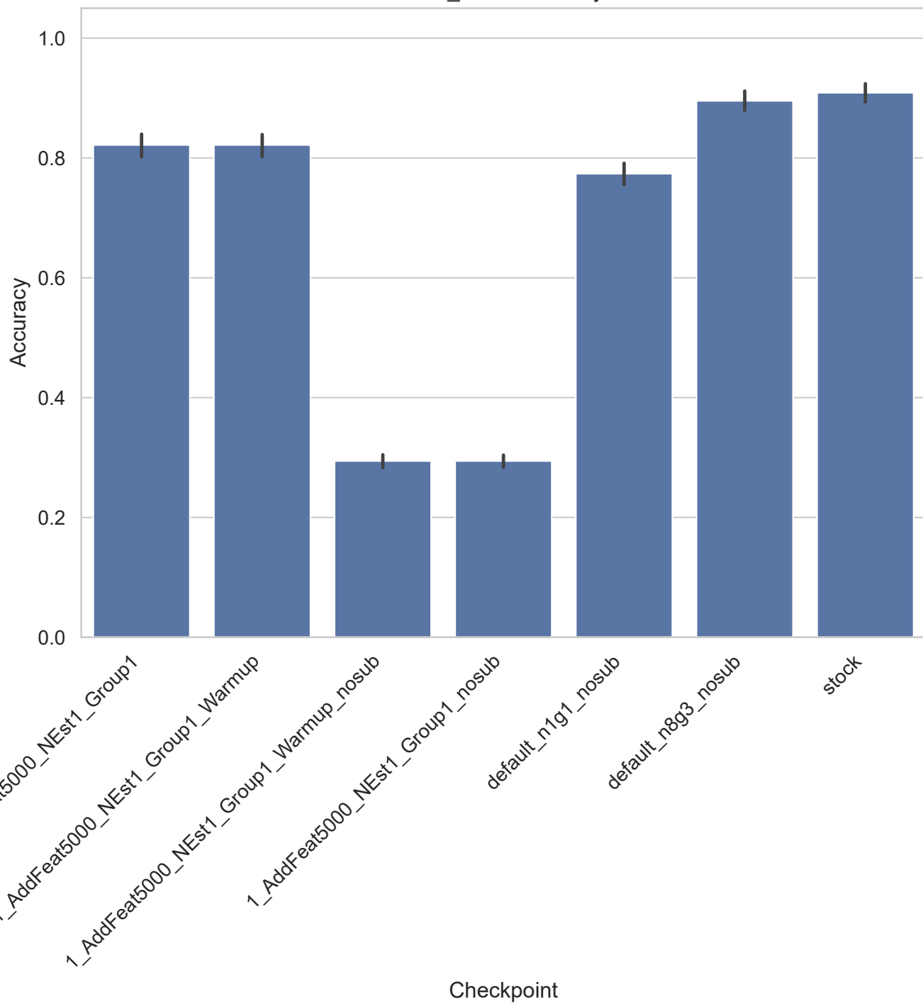
TOX_171 - Accuracy
