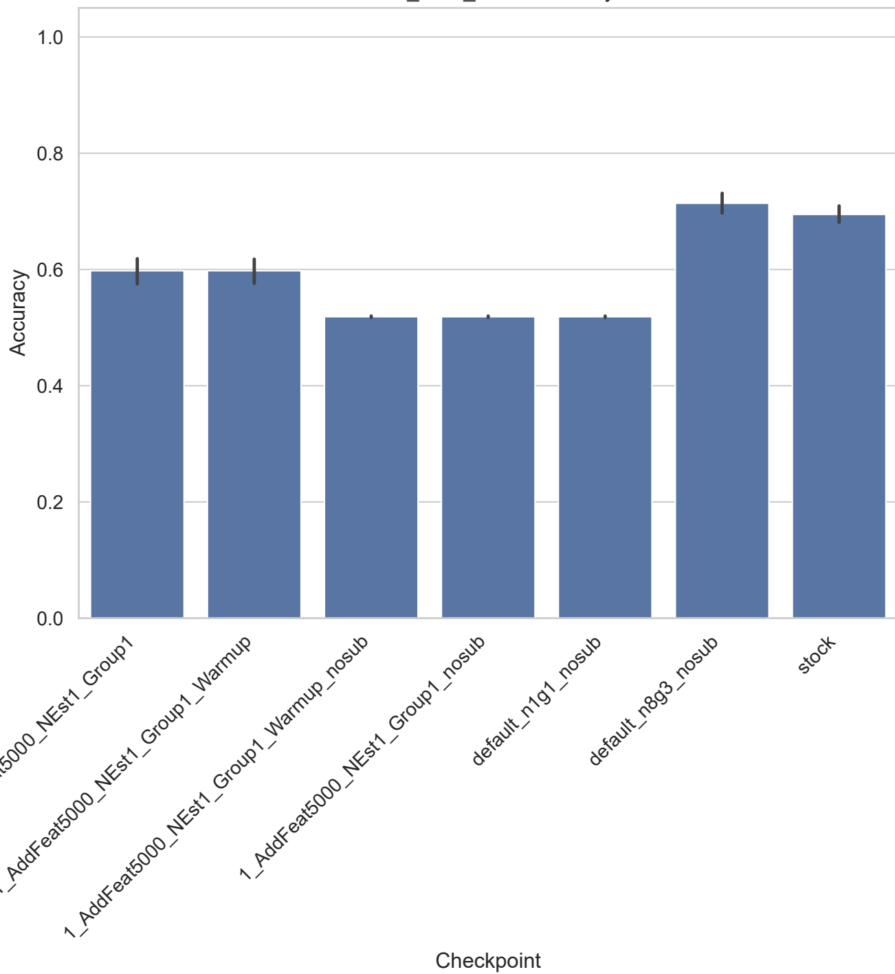
SMK_CAN_187 - Accuracy
