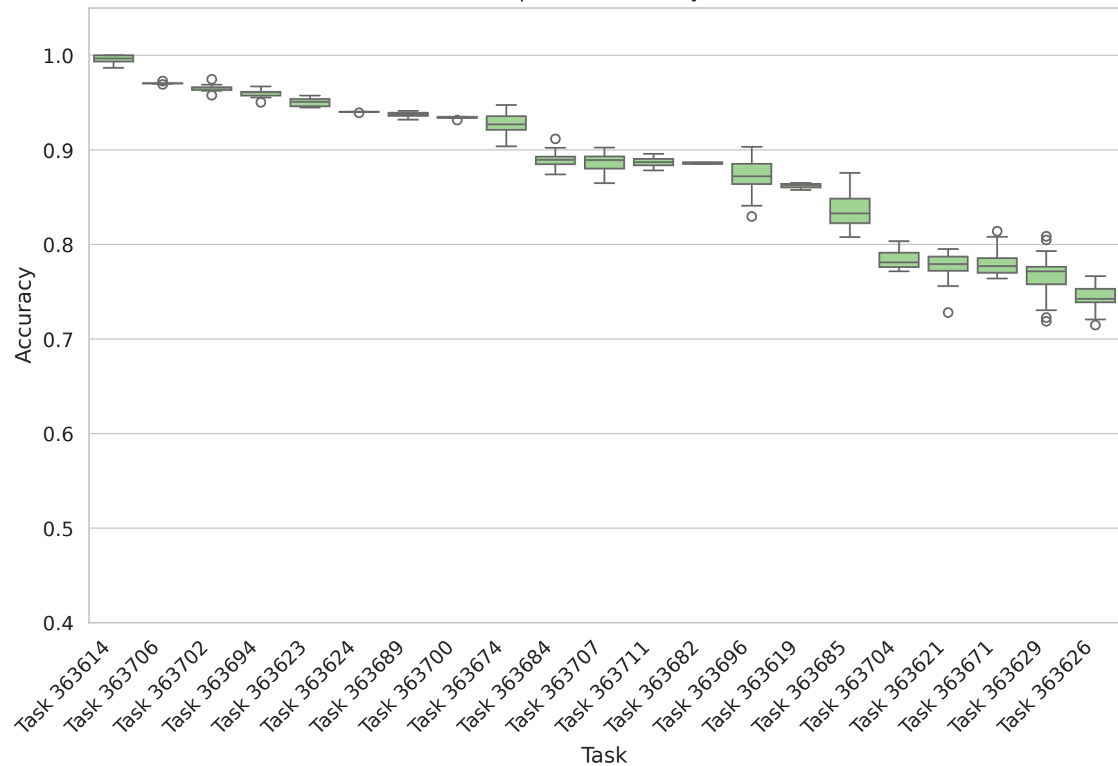
openml - accuracy
