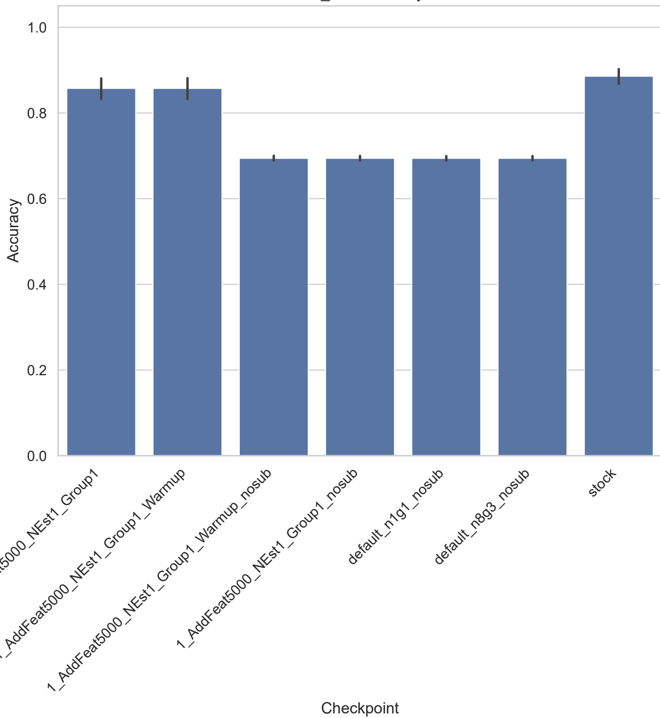
GLI_85 - Accuracy
