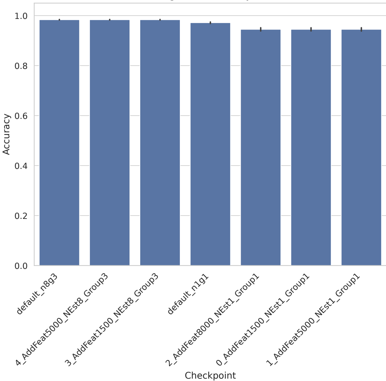
gisette - Accuracy
