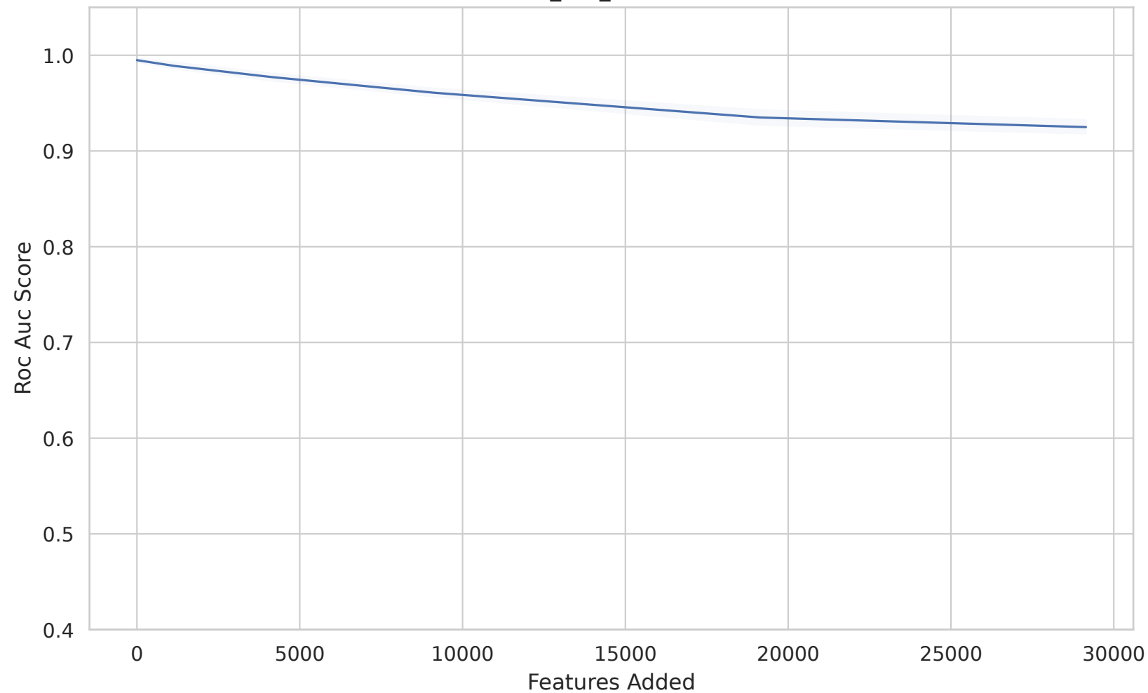
Dataset 1468 - roc_auc_score vs Features Added
