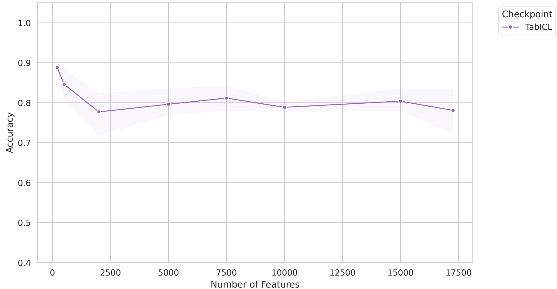
COAD - Accuracy vs Feature Count
