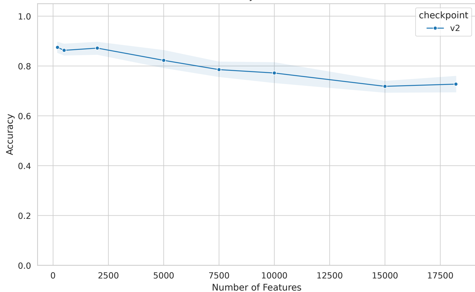
BRCA - Accuracy vs Feature Count
