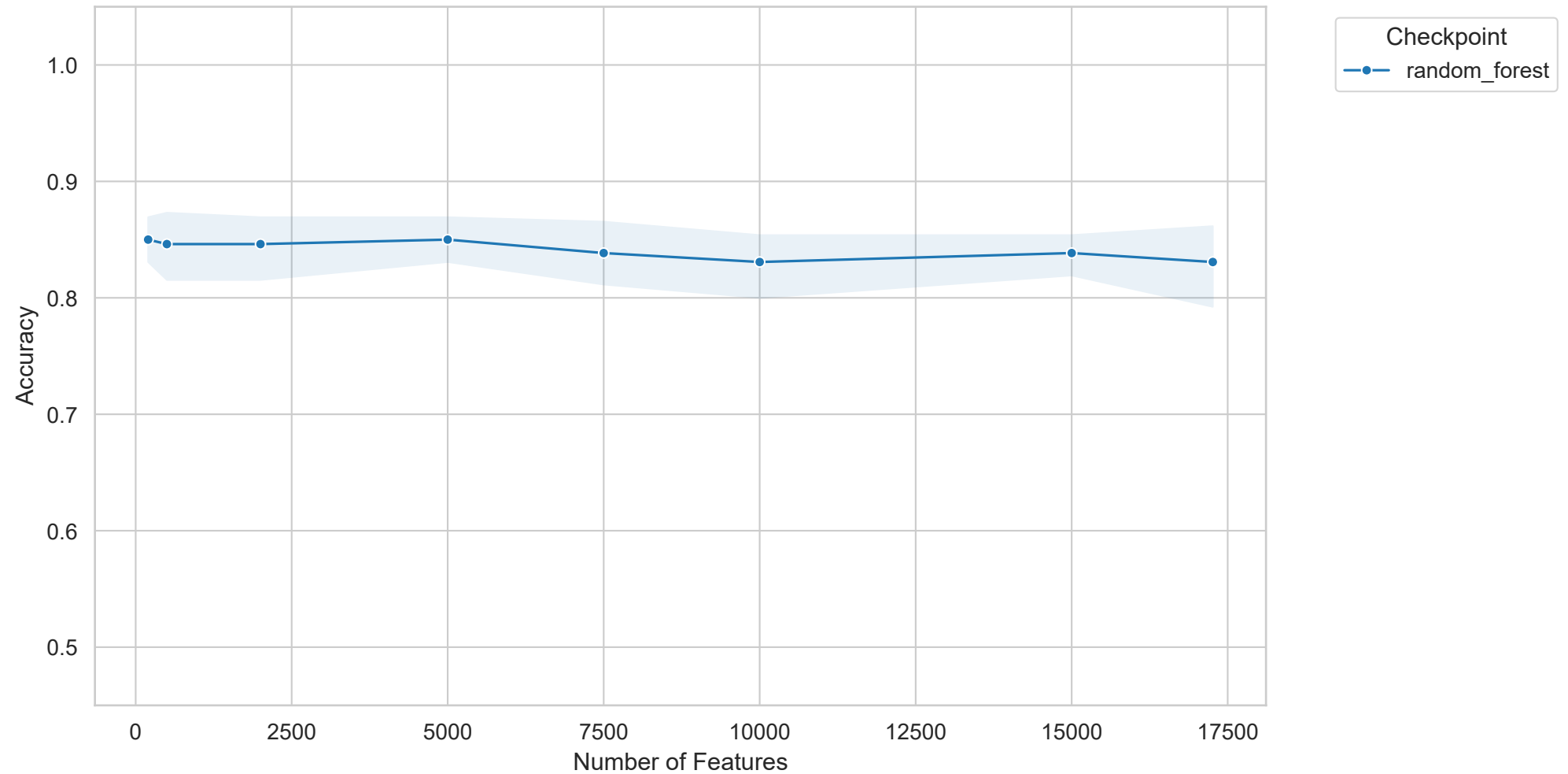
COAD - Accuracy vs Feature Count
