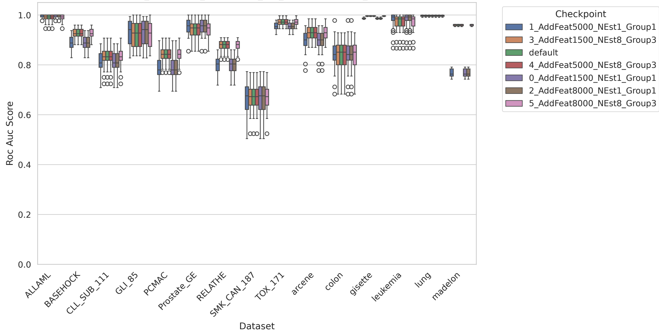
hdlss_benchmark_results - roc_auc_score per dataset_name
