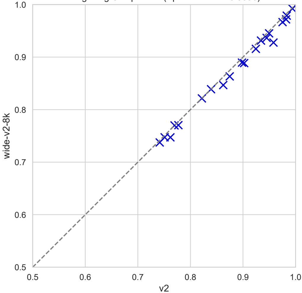
Forgetting Comparison (Spearman rho=0.9896)
