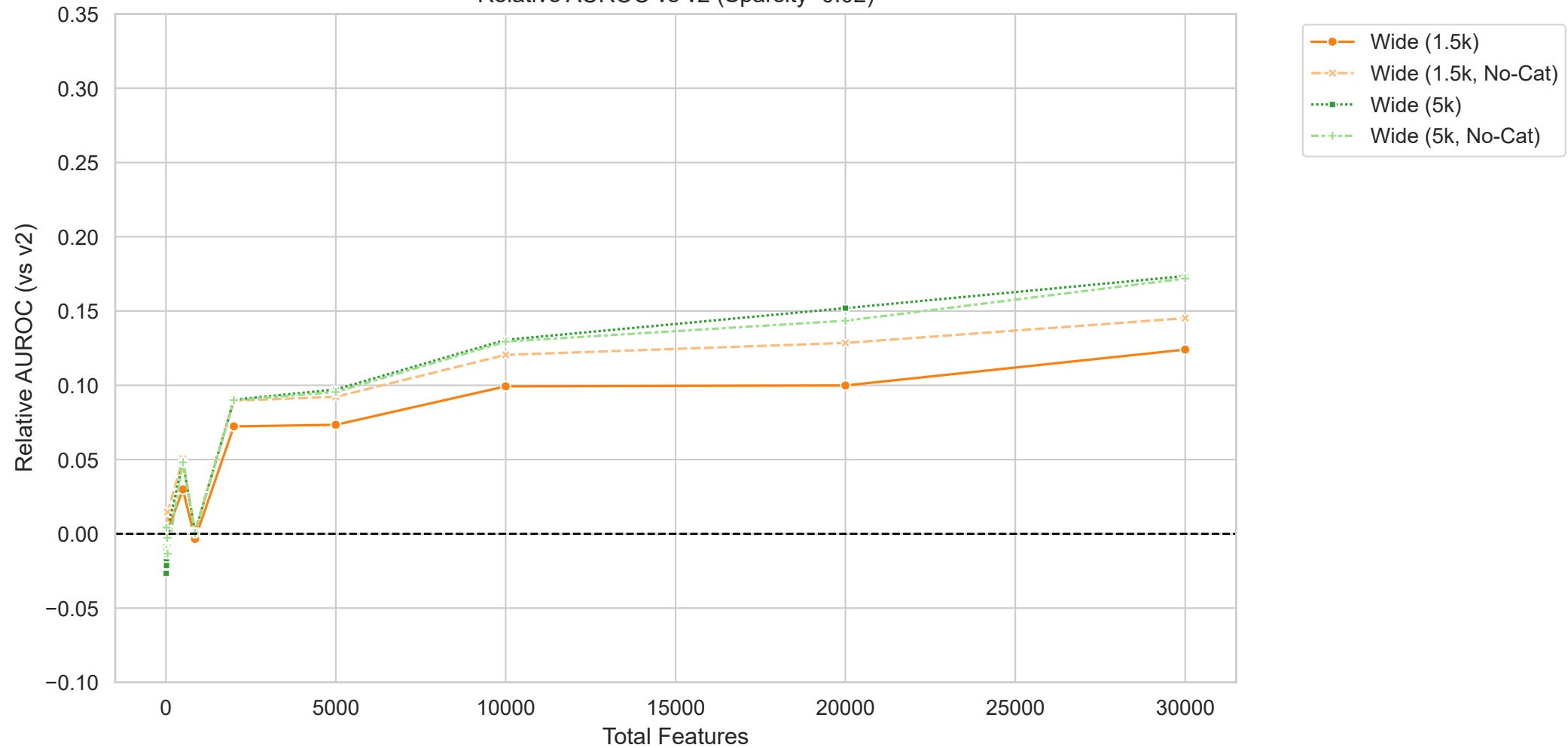
Relative AUROC vs v2 (Sparsity=0.02)
