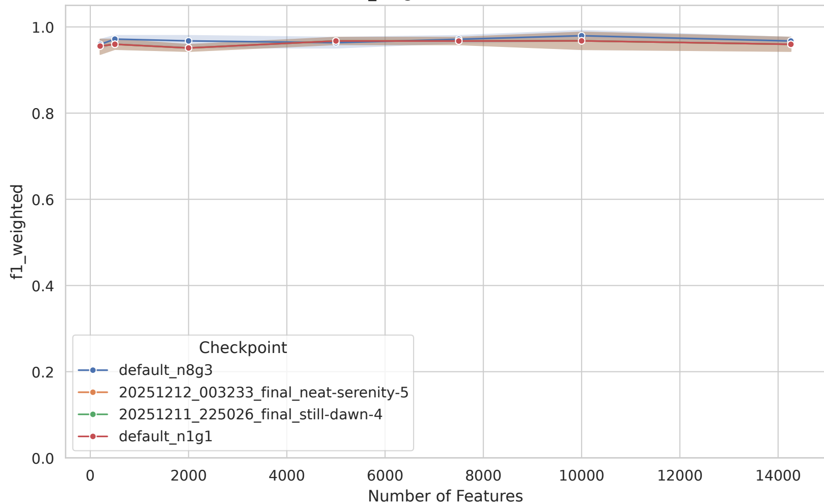
LGG - f1_weighted vs Feature Count
