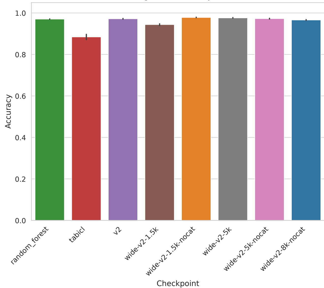
gisette - Accuracy
