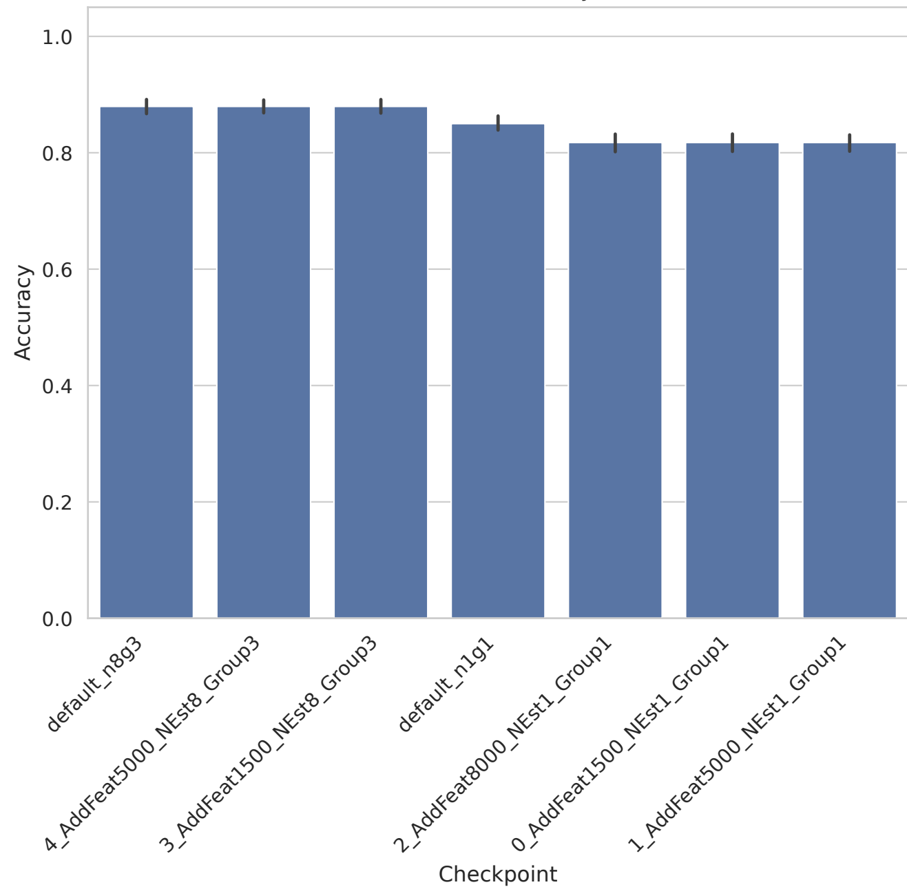
arcene - Accuracy
