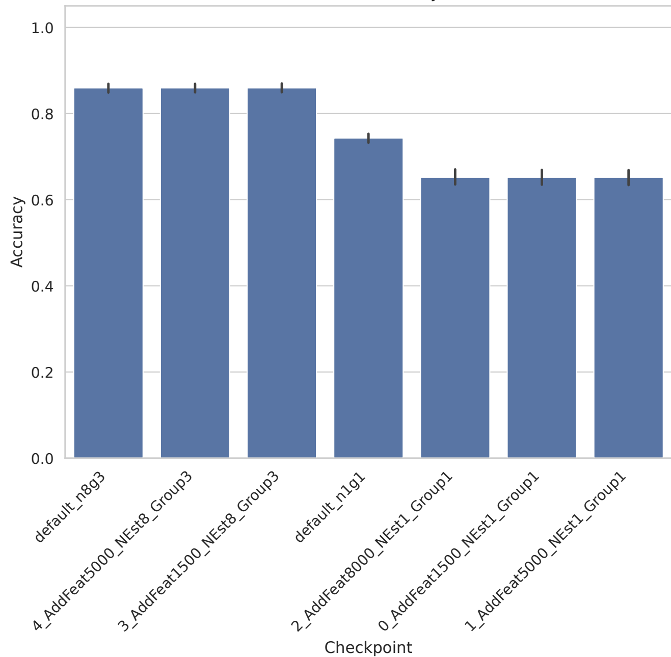
PCMAC - Accuracy
