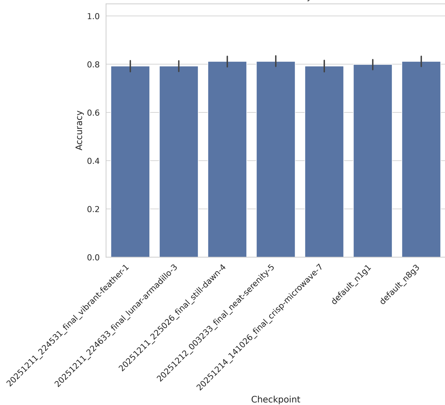
colon - Accuracy
