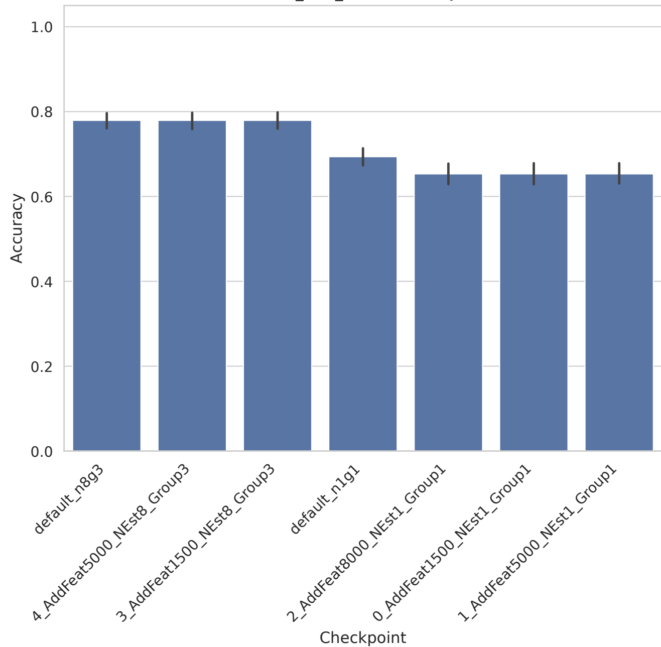
CLL_SUB_111 - Accuracy
