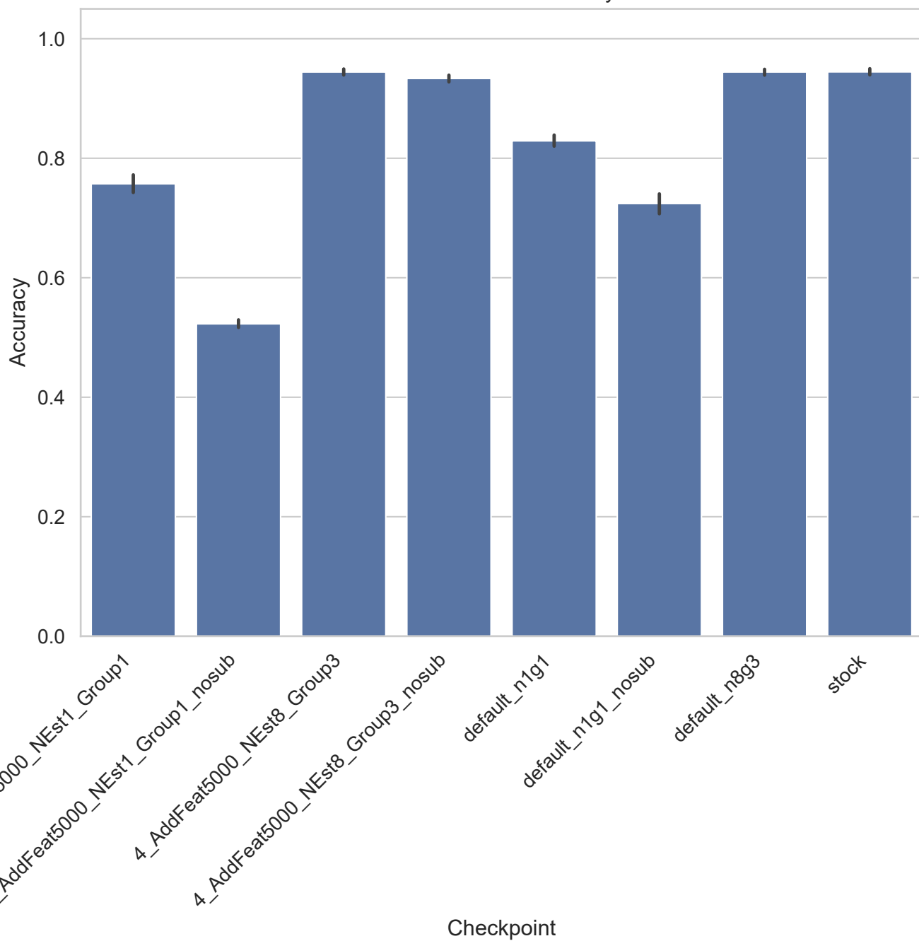
BASEHOCK - Accuracy
