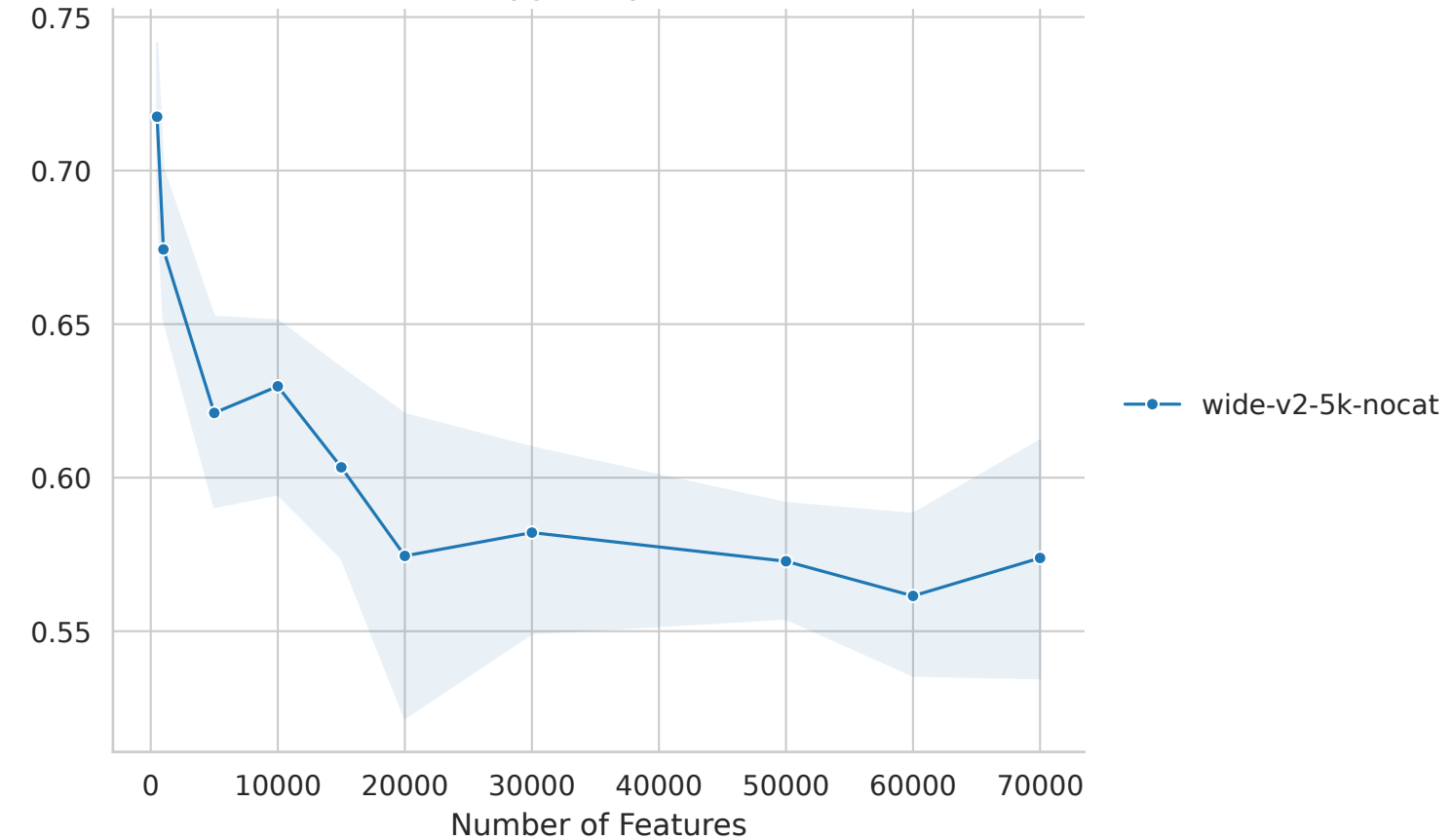
Polygenicity: 0.05
