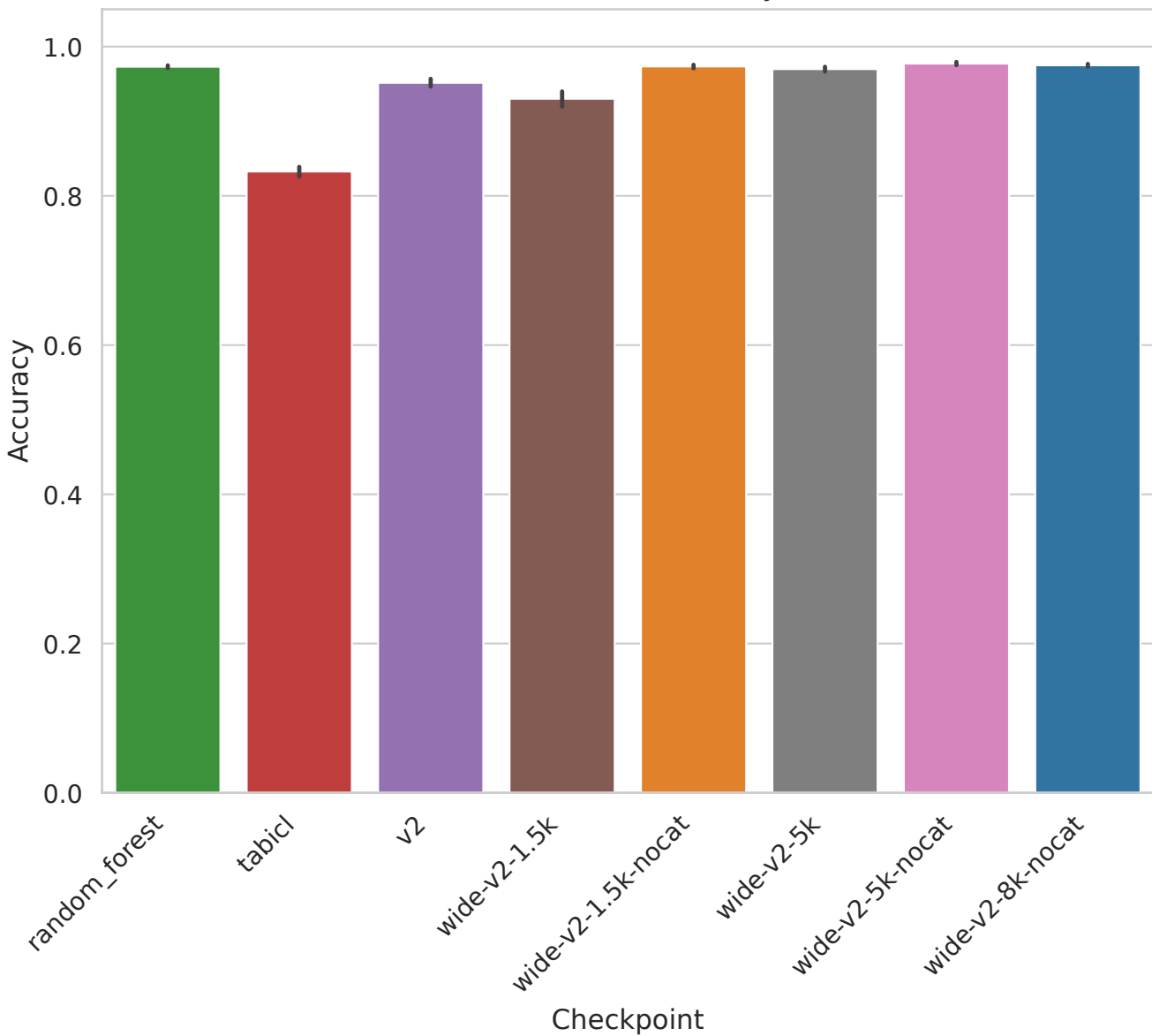
BASEHOCK - Accuracy
