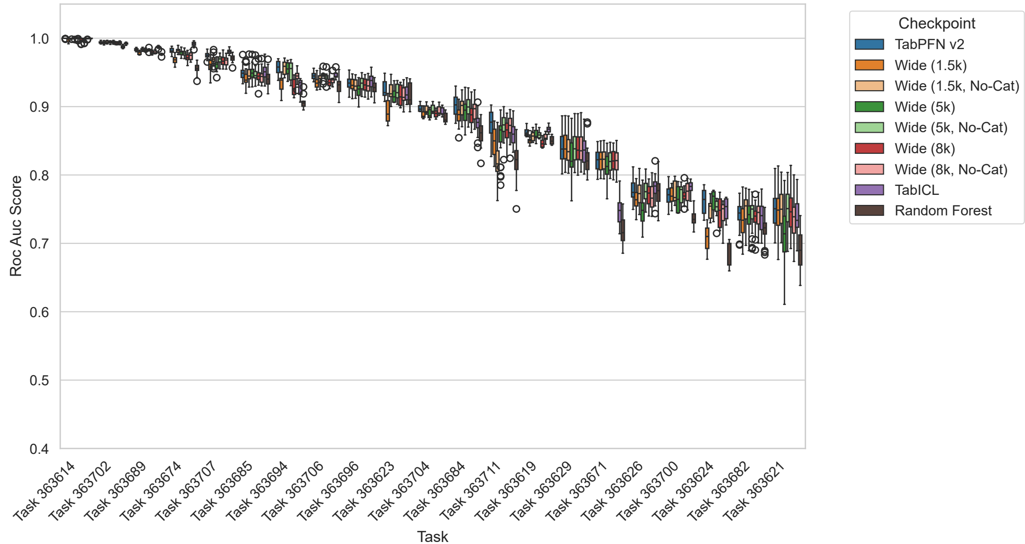
openml - roc_auc_score
