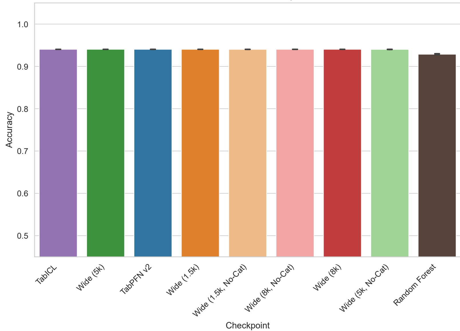
Task 363624 - Accuracy
