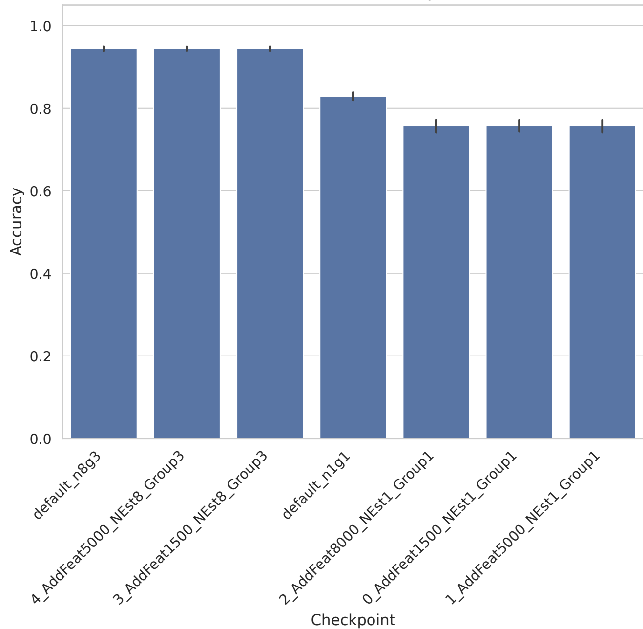
BASEHOCK - Accuracy
