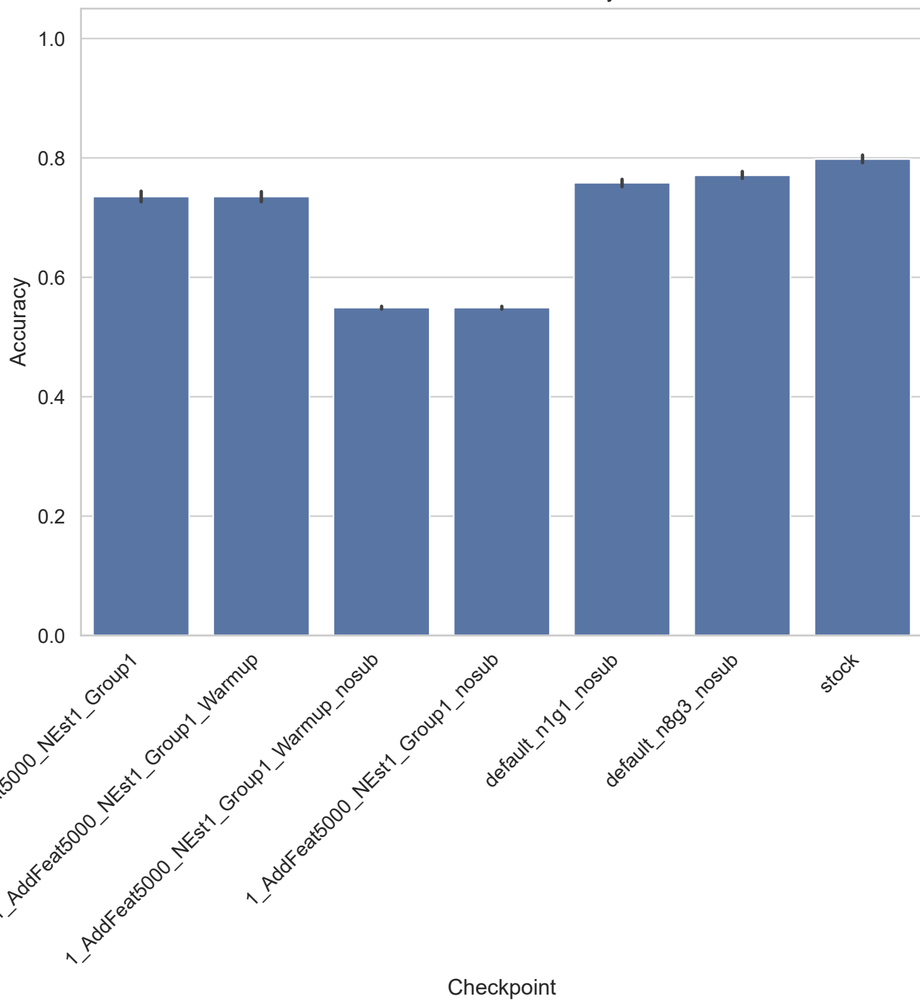
Task 363620 - Accuracy
