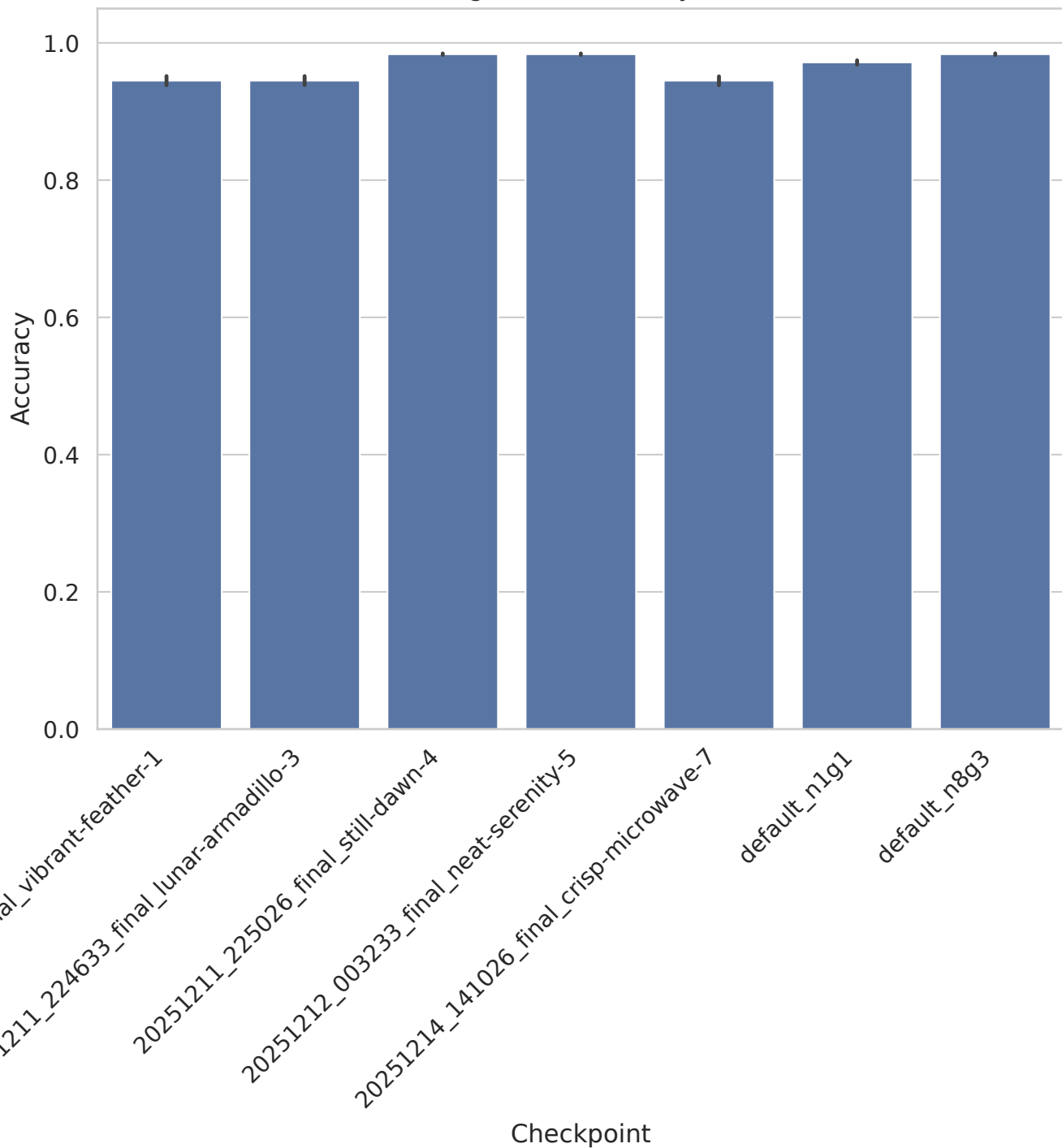
gisette - Accuracy
