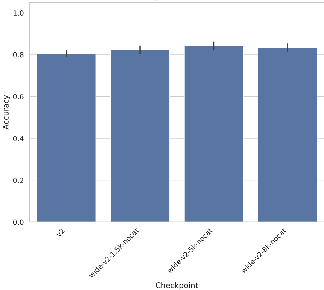
TOX_171 - Accuracy
