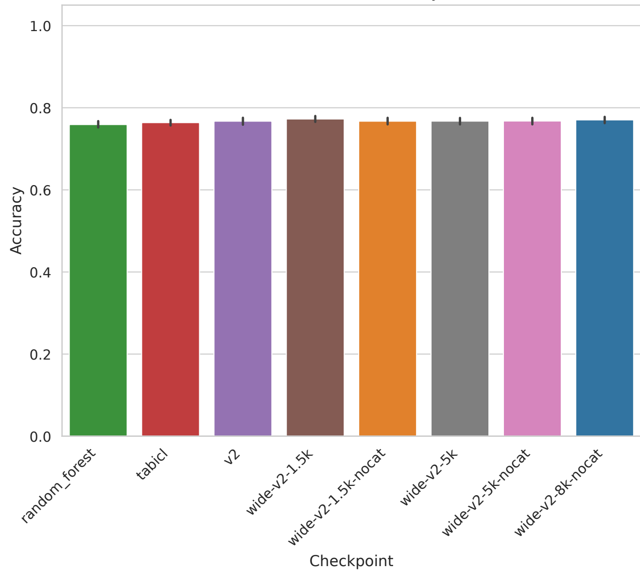
Task 363629 - Accuracy
