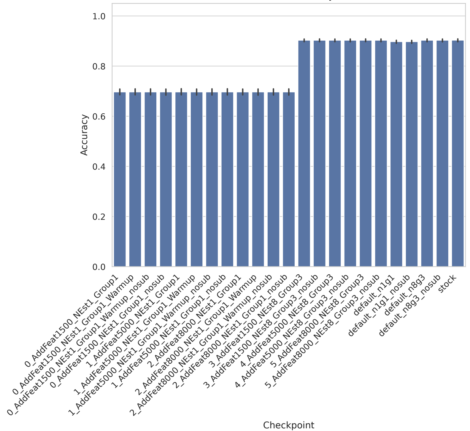
madelon - Accuracy
