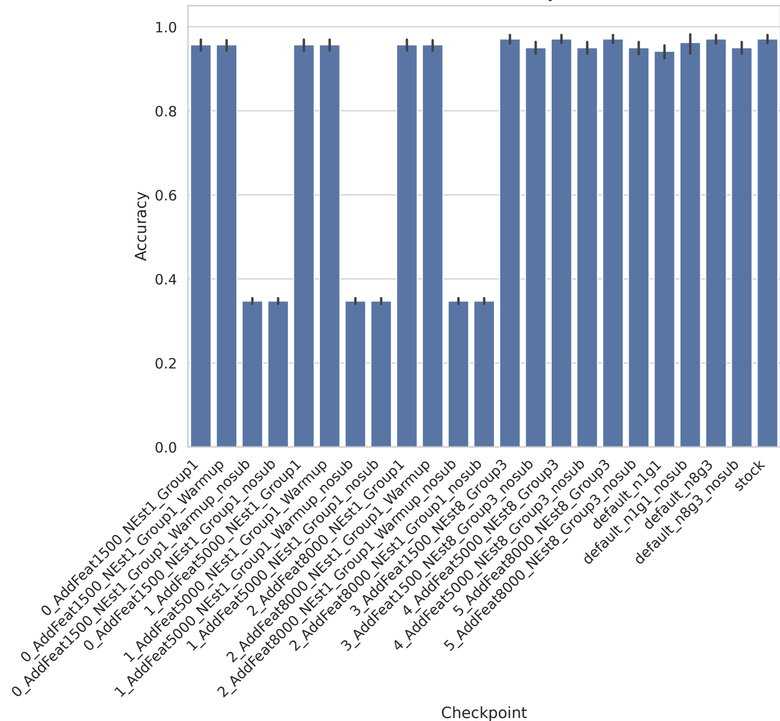
ALLAML - Accuracy
