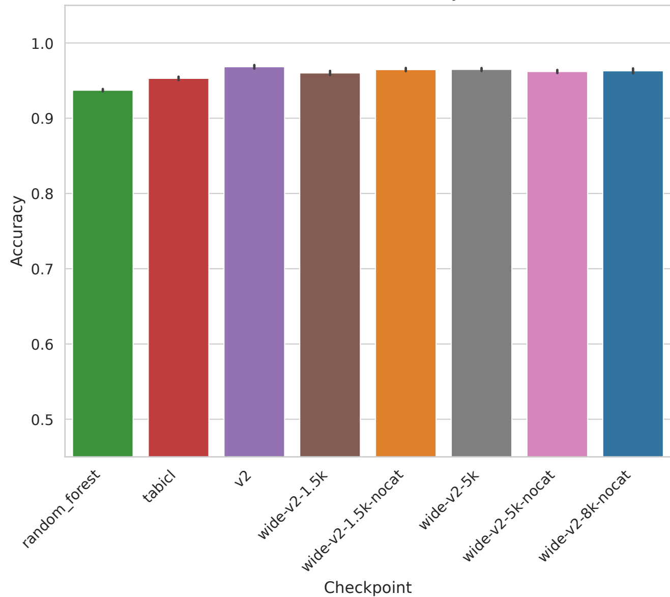
Task 363694 - Accuracy
