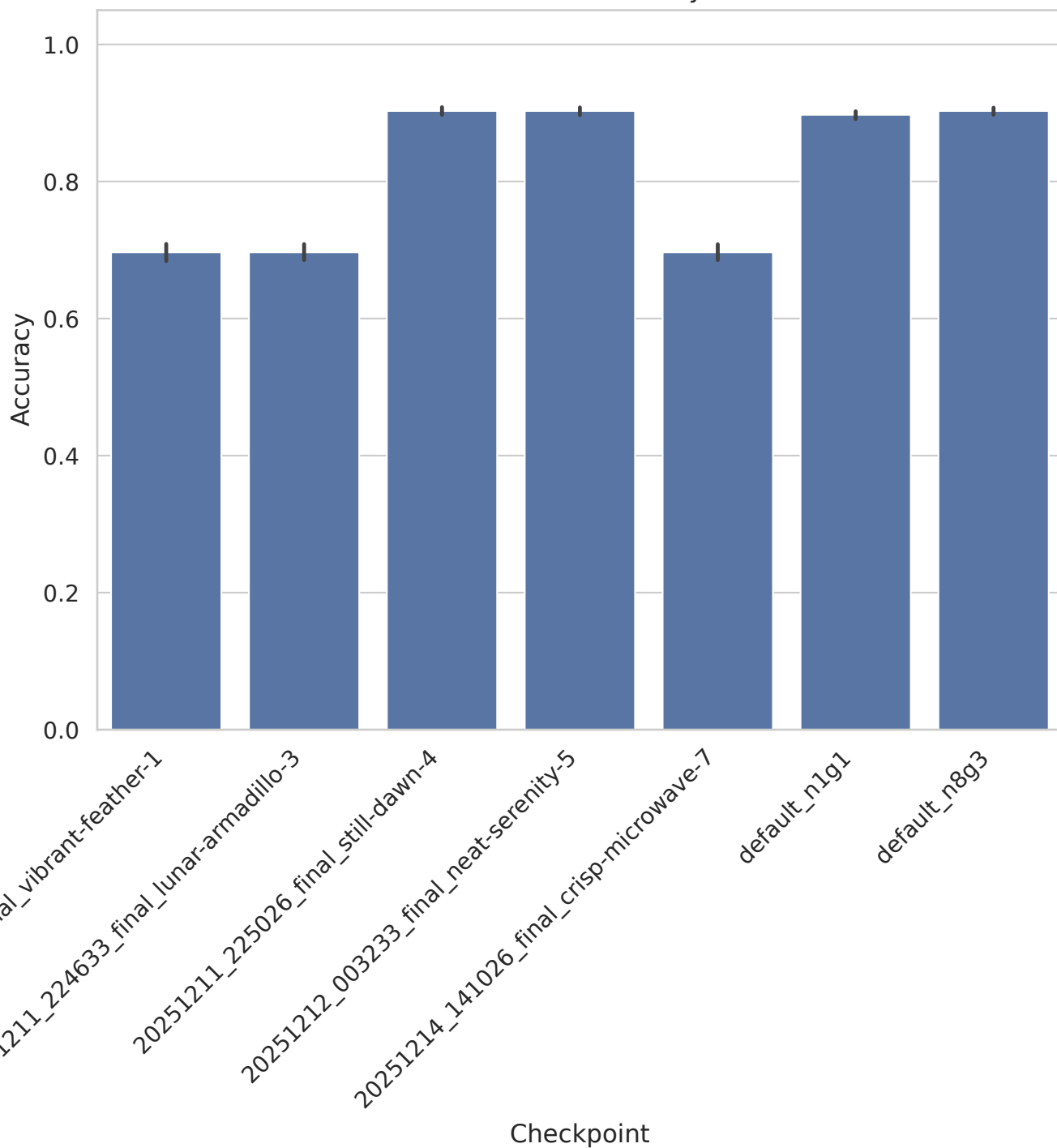
madelon - Accuracy
