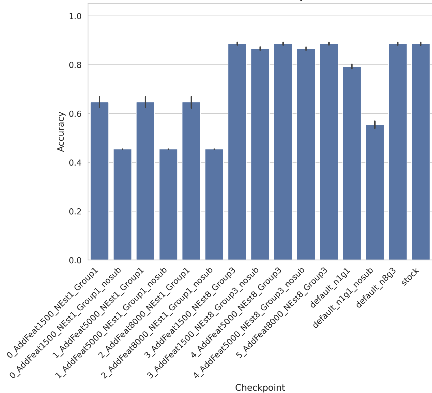
RELATHE - Accuracy
