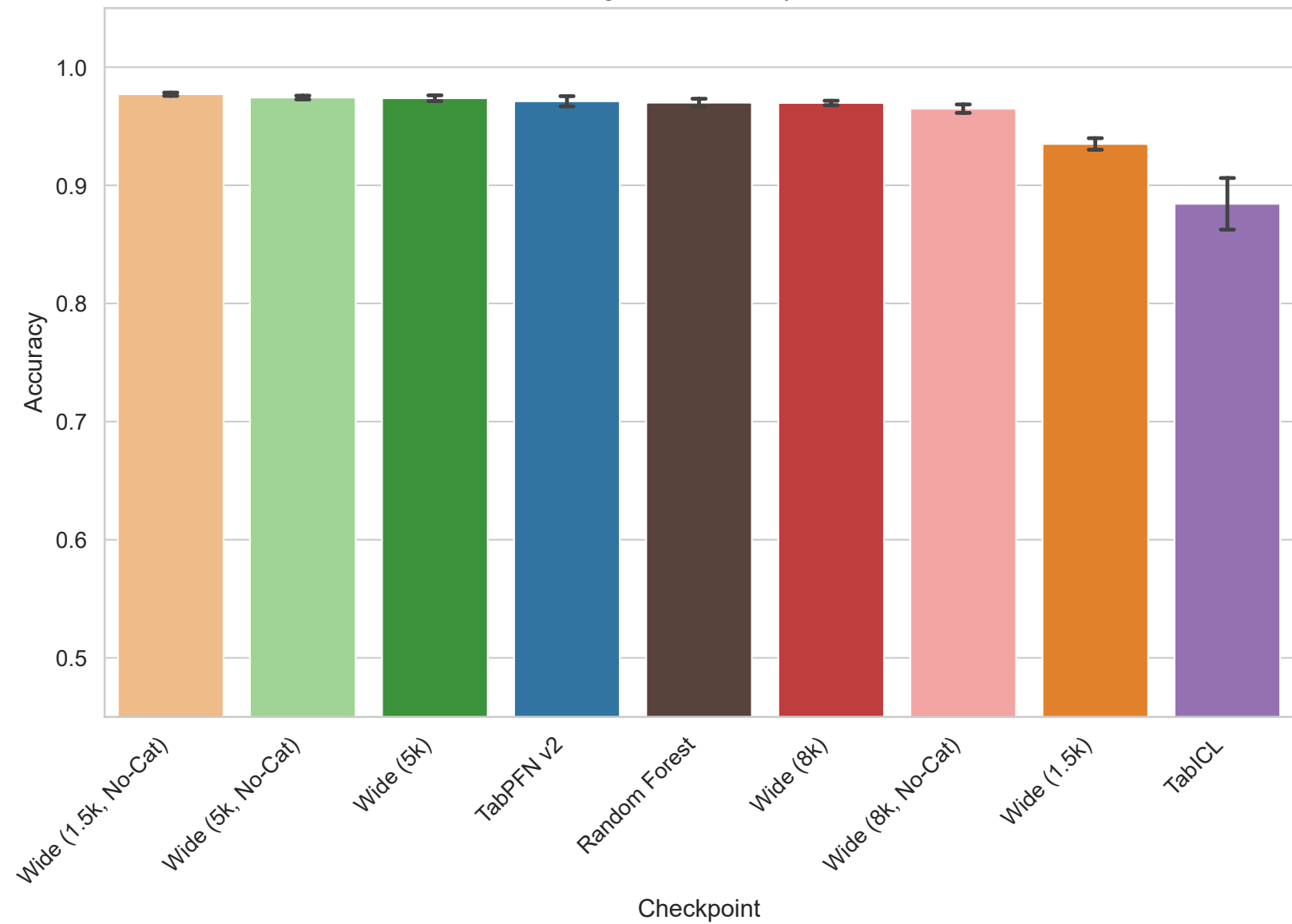
gisette - Accuracy
