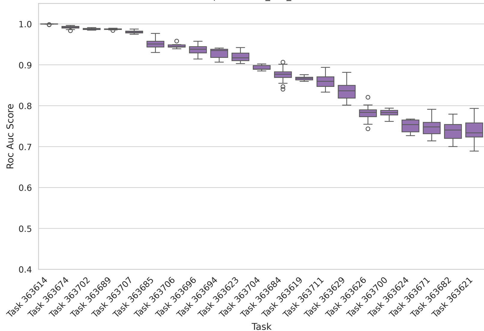
openml - roc_auc_score
