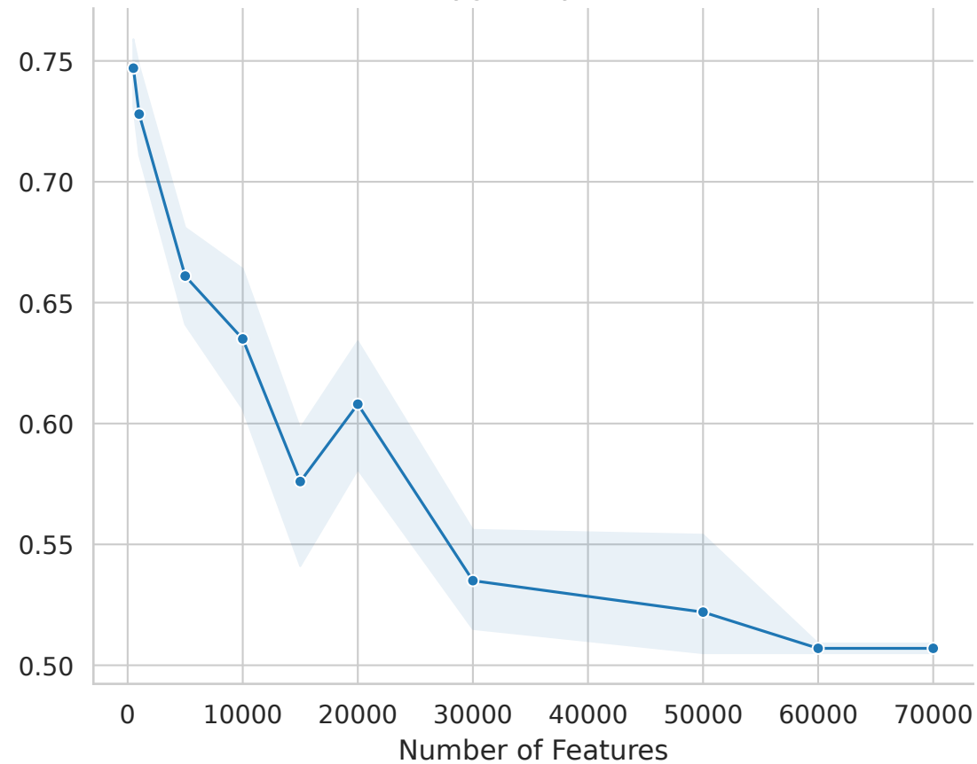
Polygenicity: 0.01
