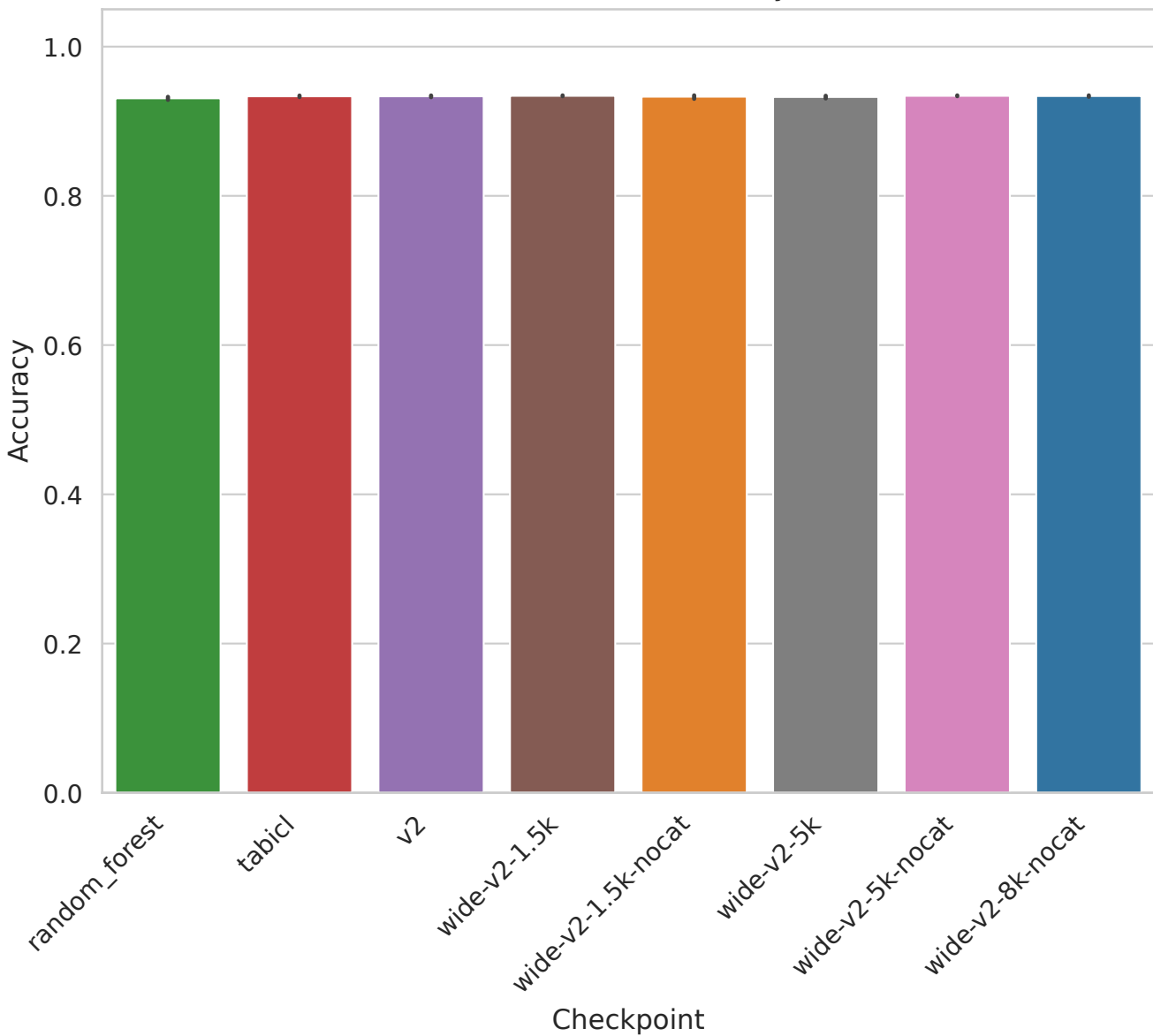
Task 363700 - Accuracy
