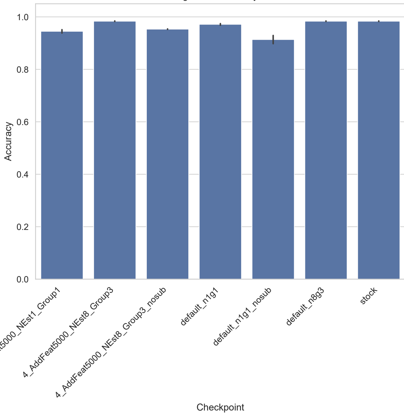
gisette - Accuracy
