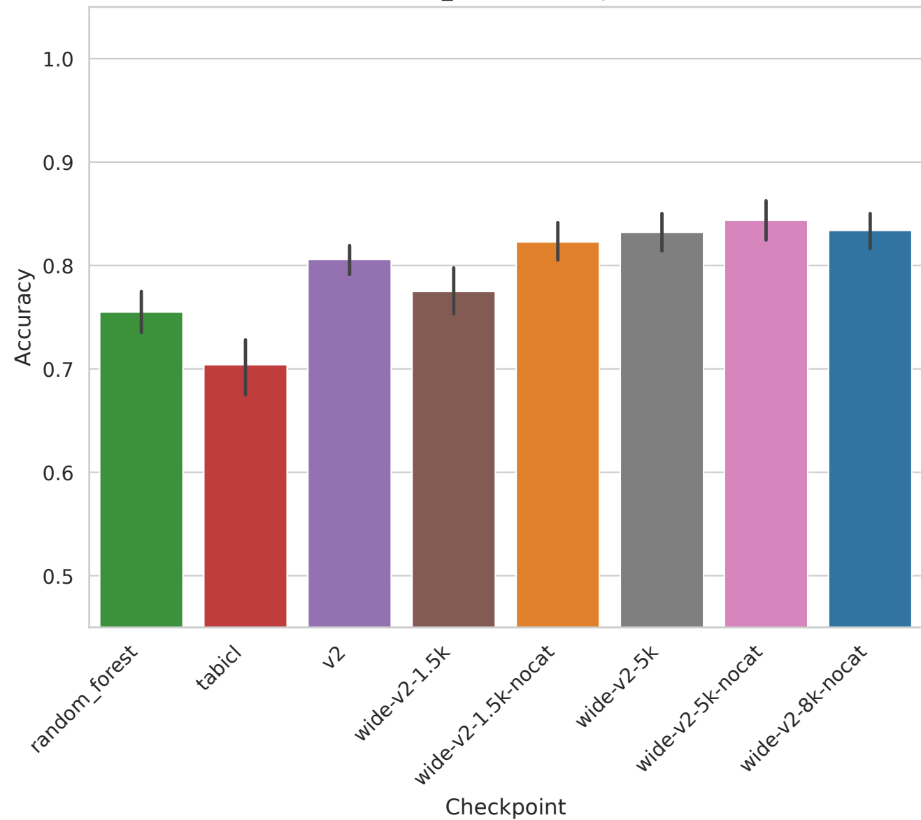
TOX_171 - Accuracy
