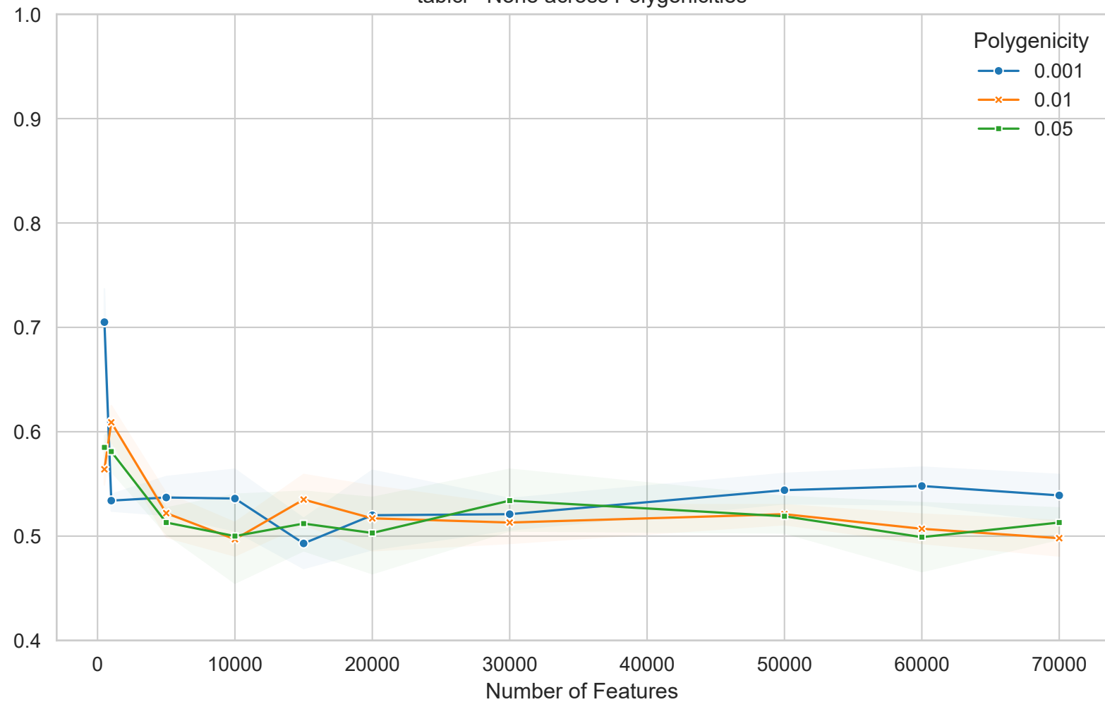
tab1c1 - None across Polygenicitities
