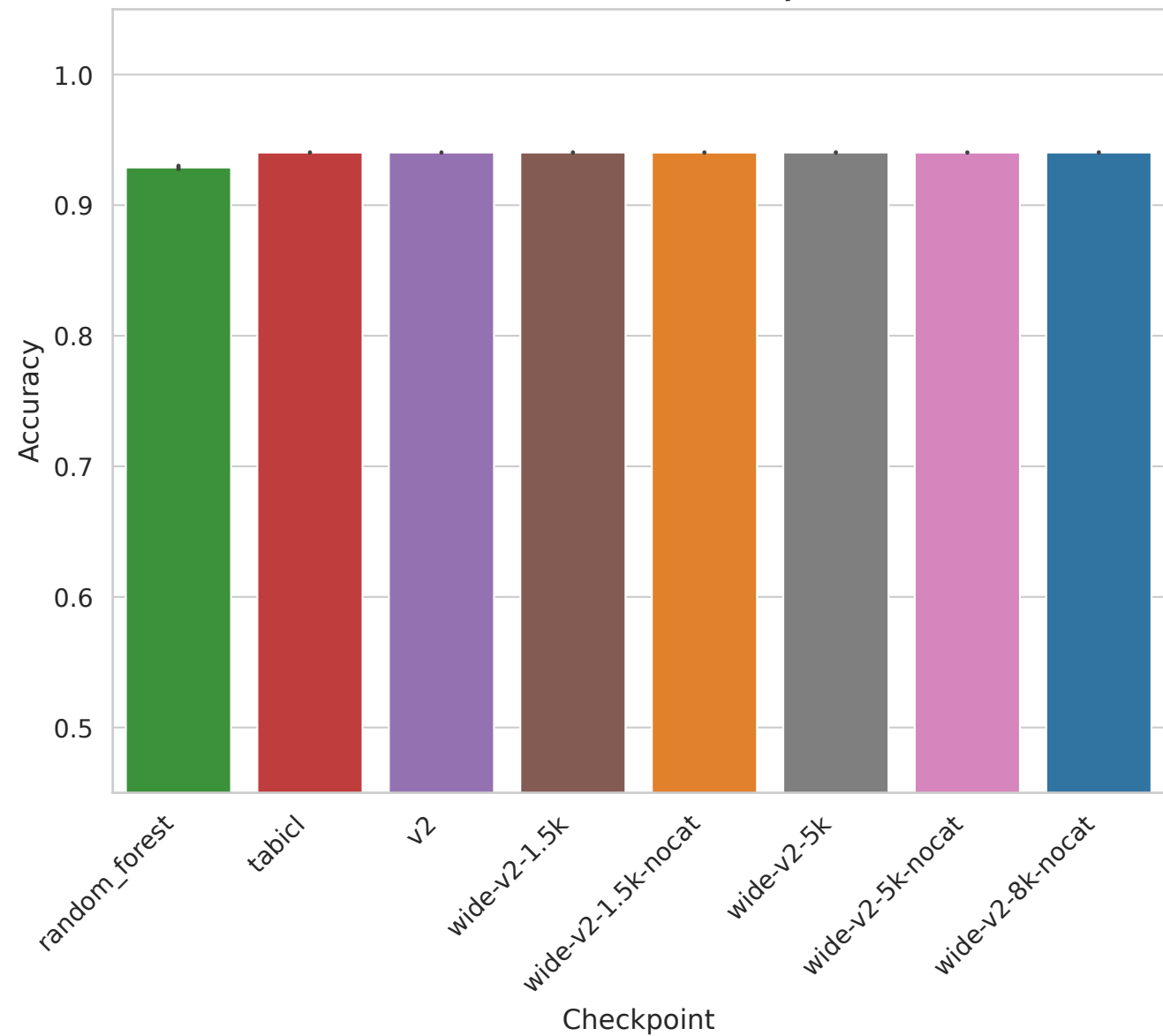
Task 363624 - Accuracy
