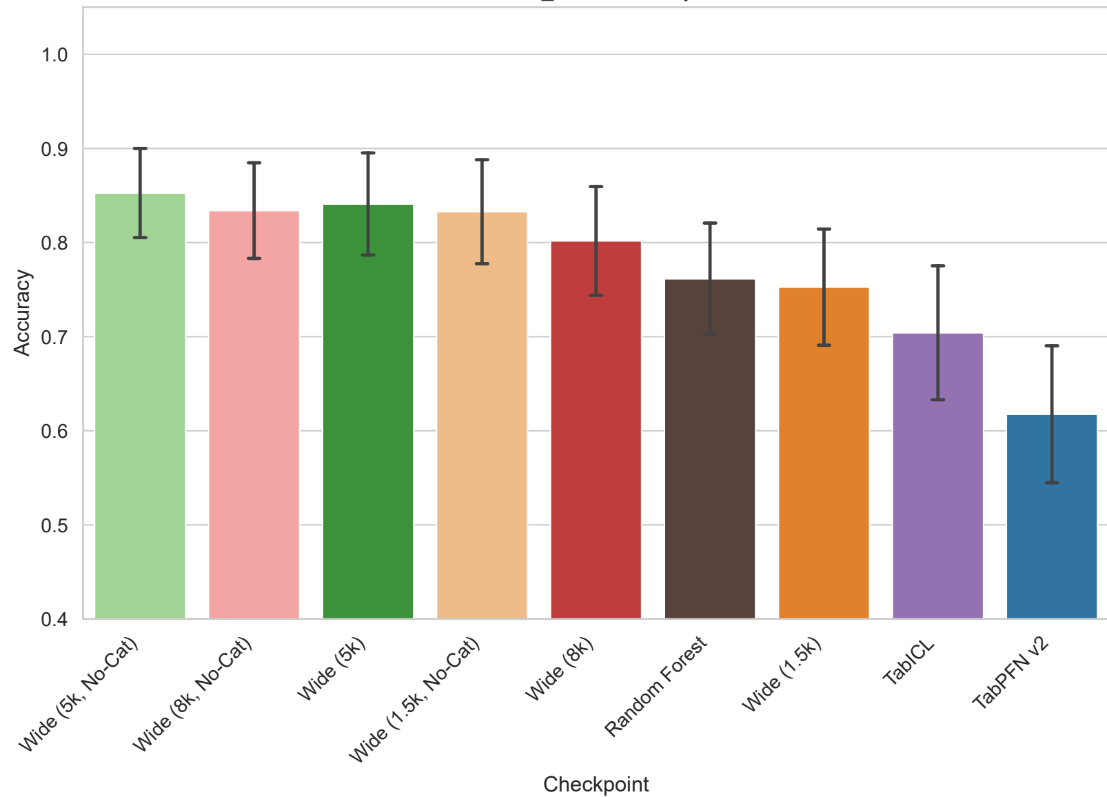
TOX_171 - Accuracy
