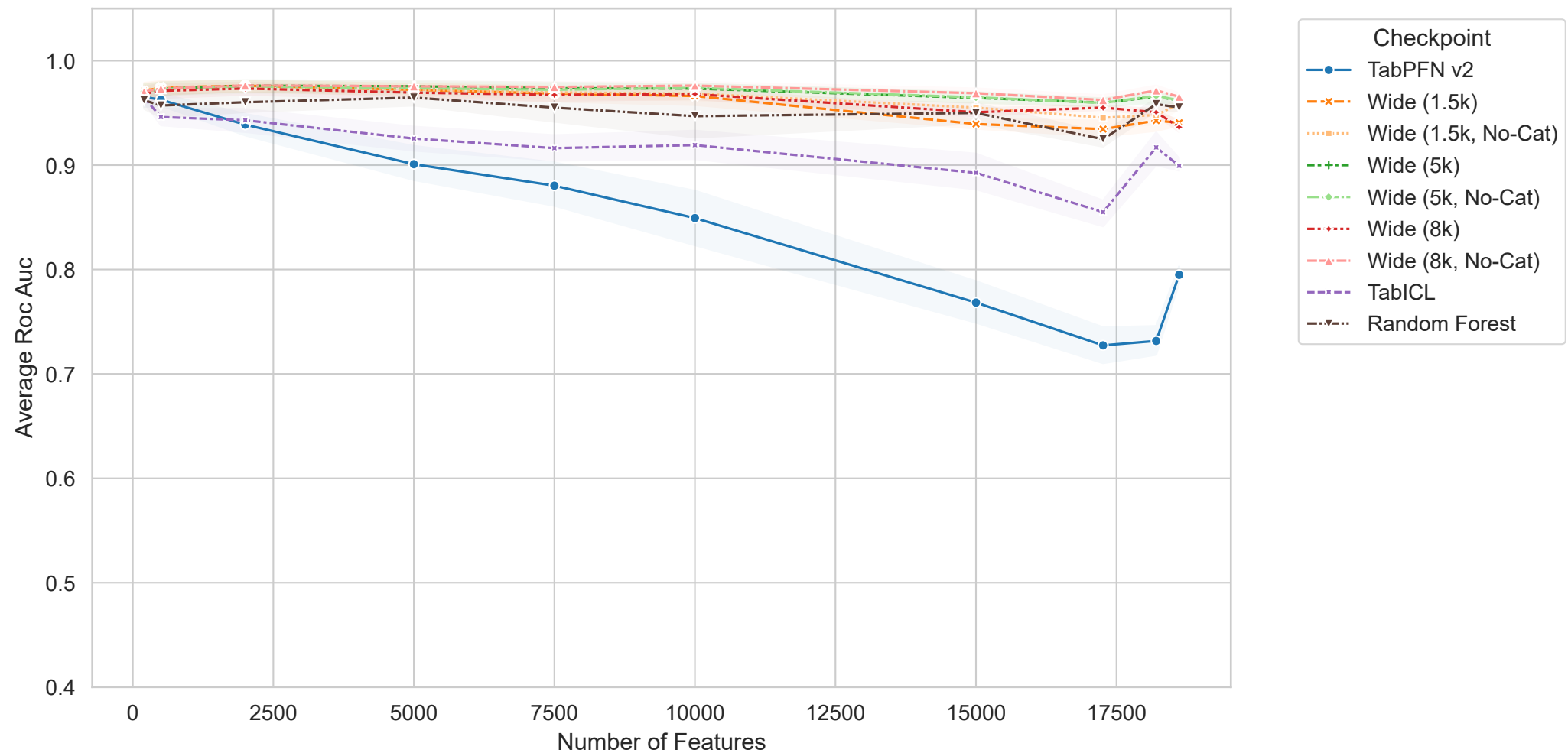
Multiomics Overview - Roc Auc vs Features
