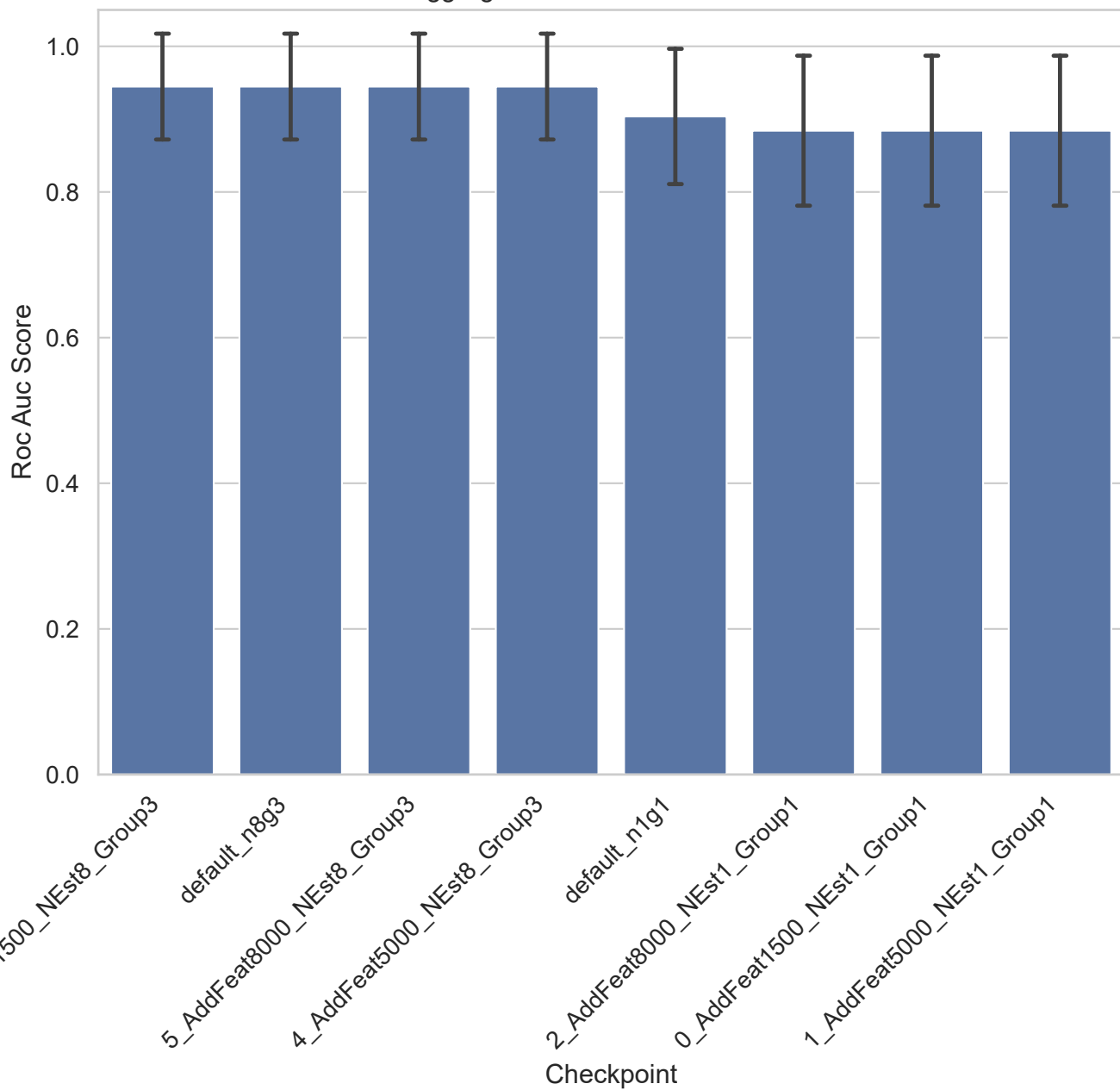
Aggregated Roc Auc Score - hdls
