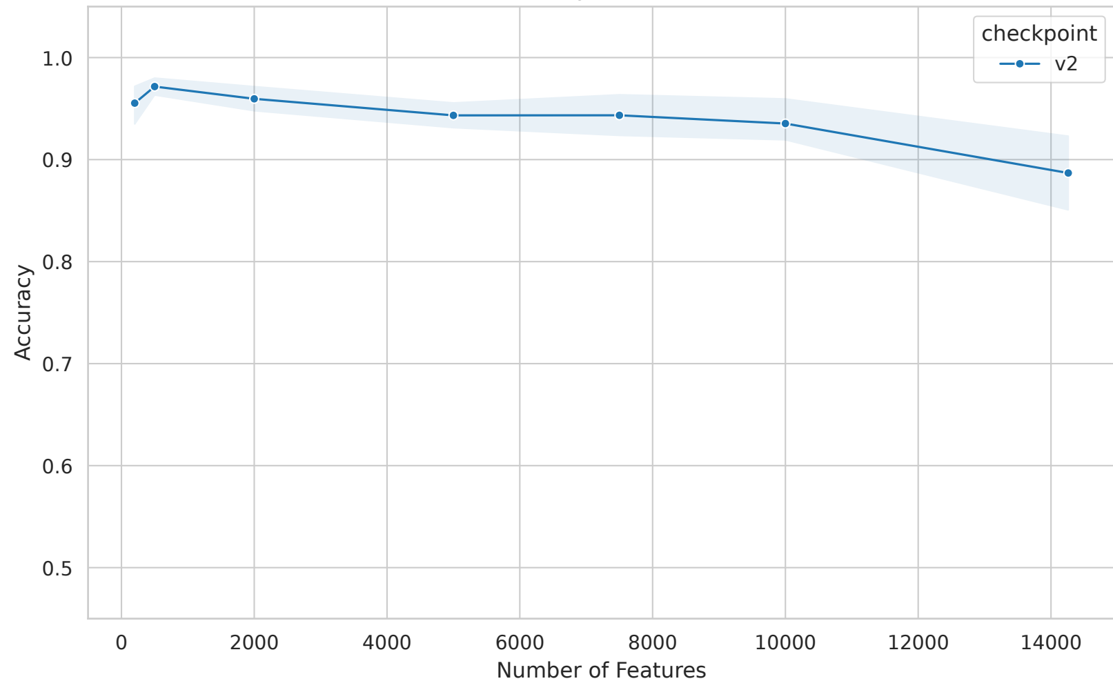
LGG - Accuracy vs Feature Count
