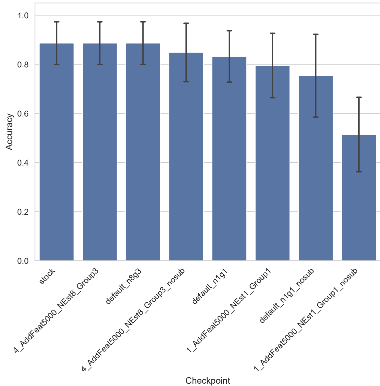
Aggregated Accuracy - hdlss
