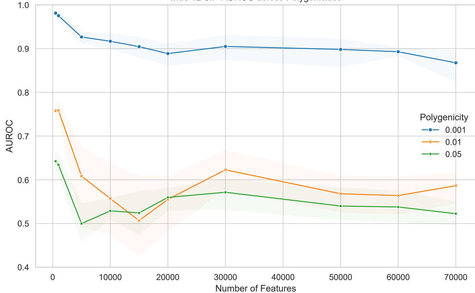
wide-v2-8k - AUROC across Polygenicities
