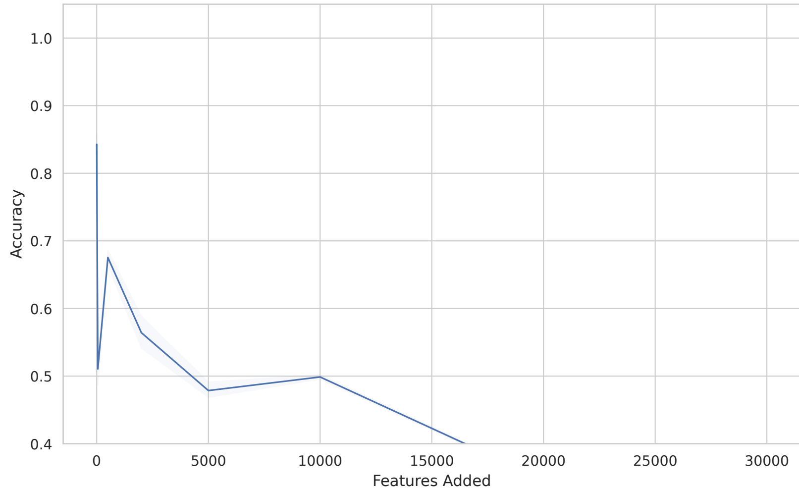
Dataset 40982 - accuracy vs Features Added
