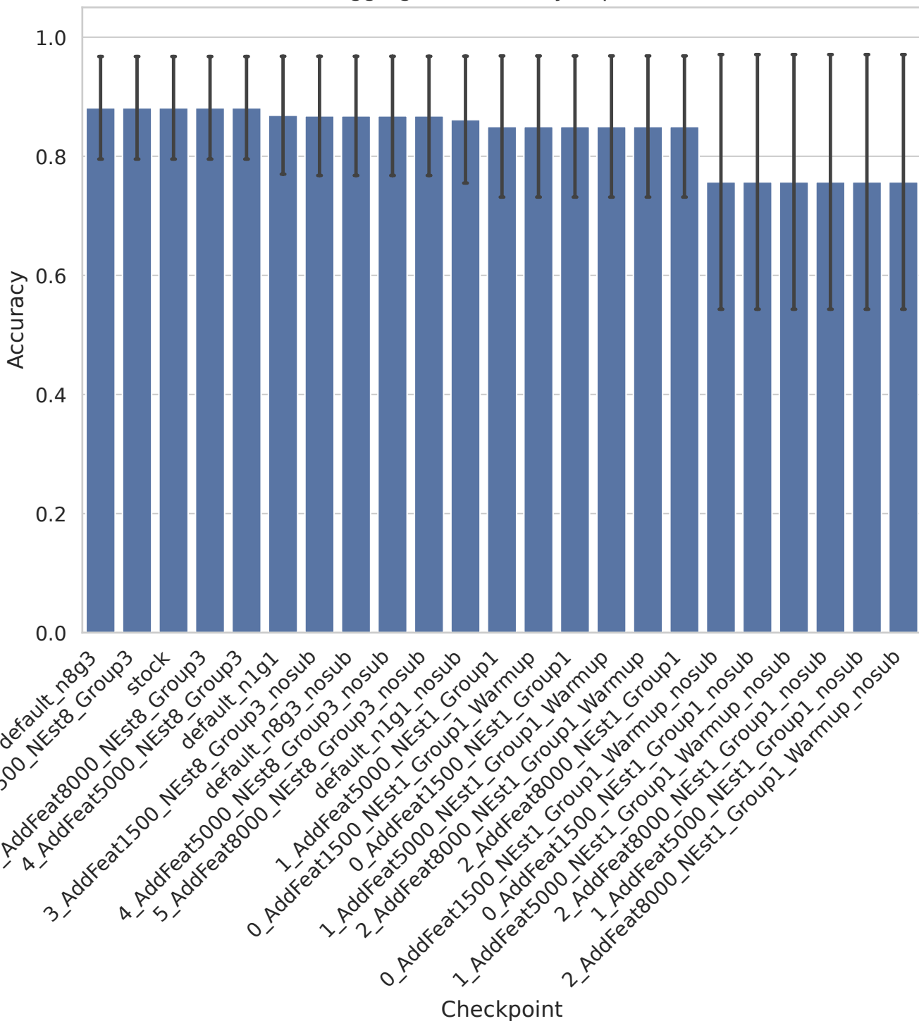
Aggregated Accuracy - openml
