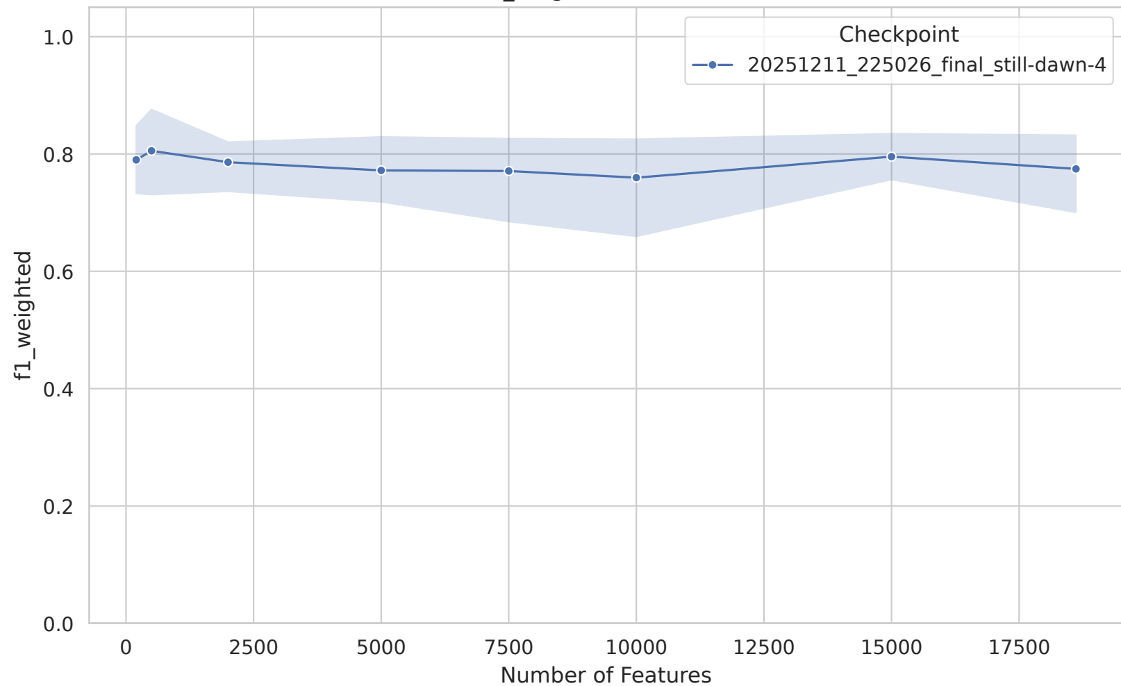
GBM - f1_weighted vs Feature Count
