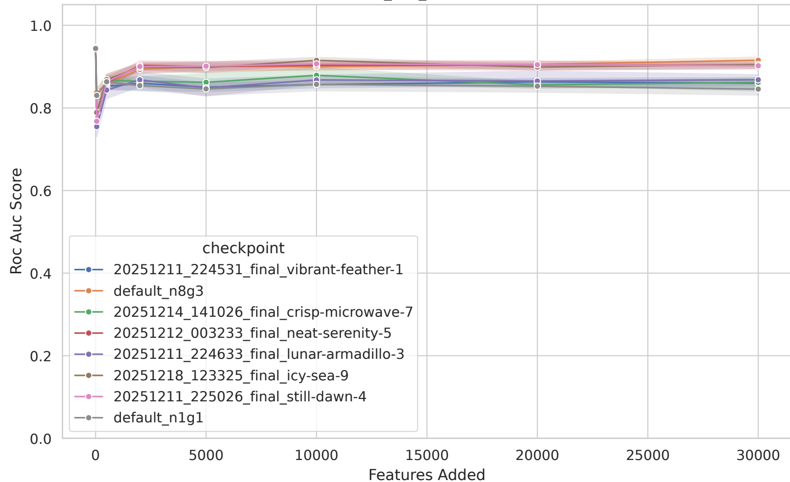
Dataset 1494 - roc_auc_score vs Features Added
