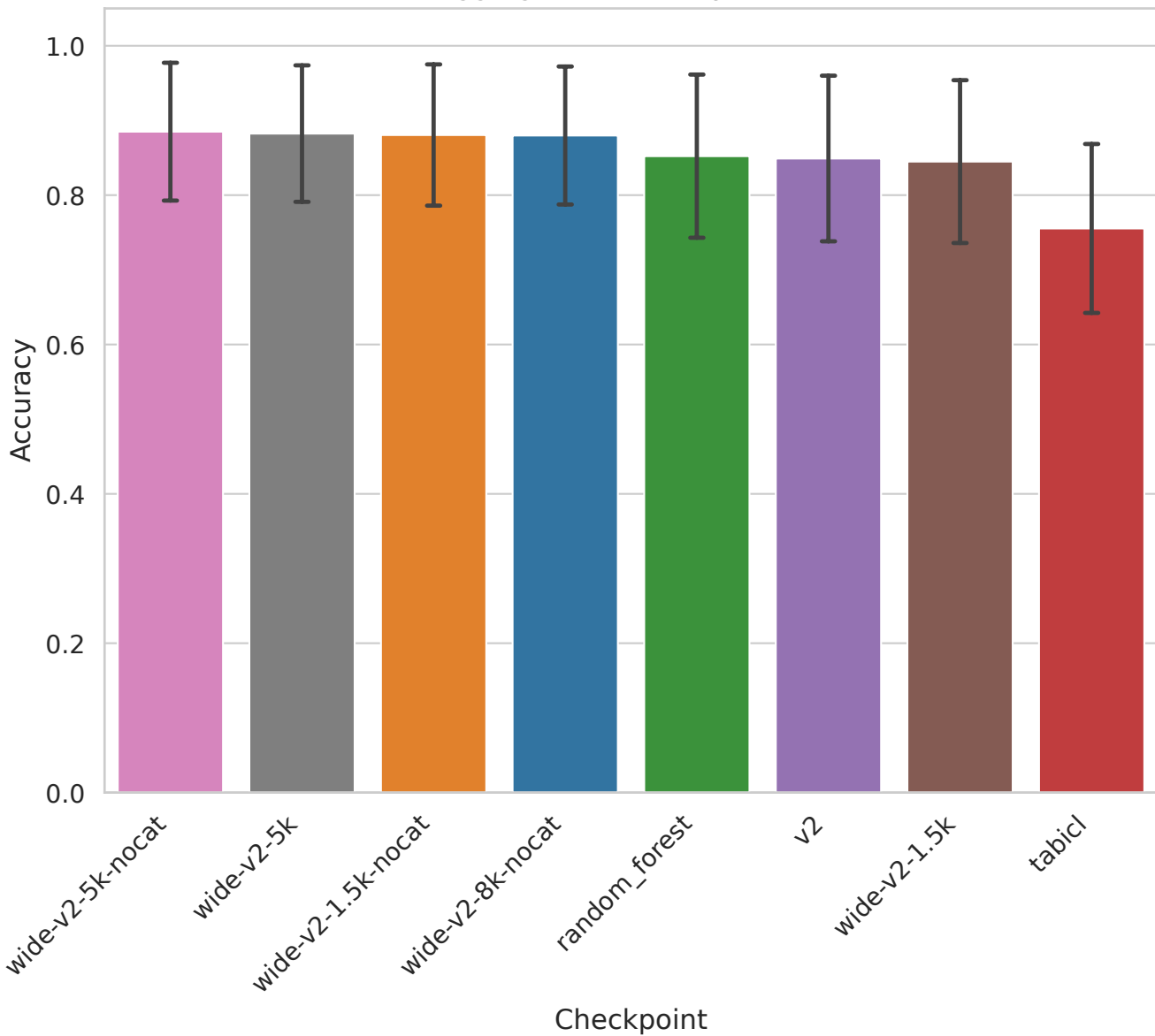
Aggregated Accuracy - hdlss
