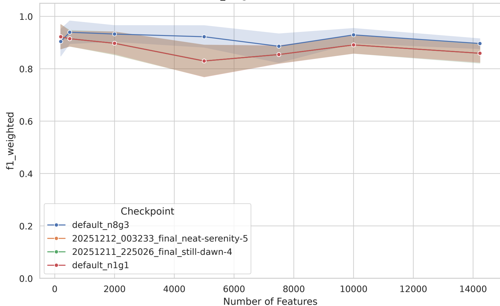
OV - f1_weighted vs Feature Count
