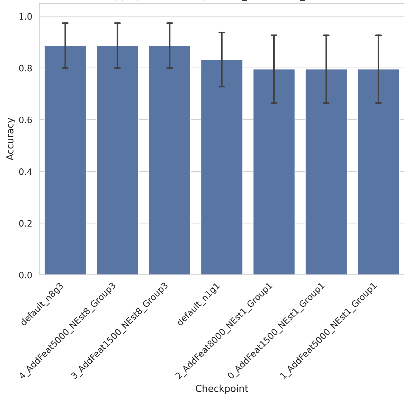
Aggregated Accuracy - hdlss_benchmark_results
