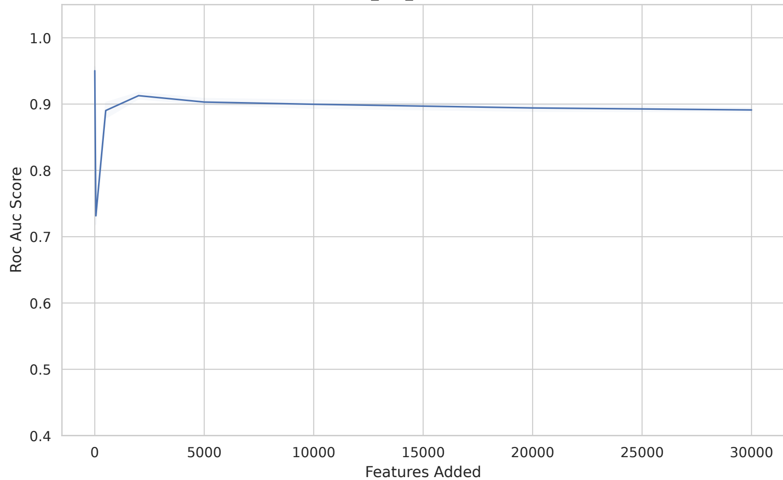
Dataset 54 - roc_auc_score vs Features Added
