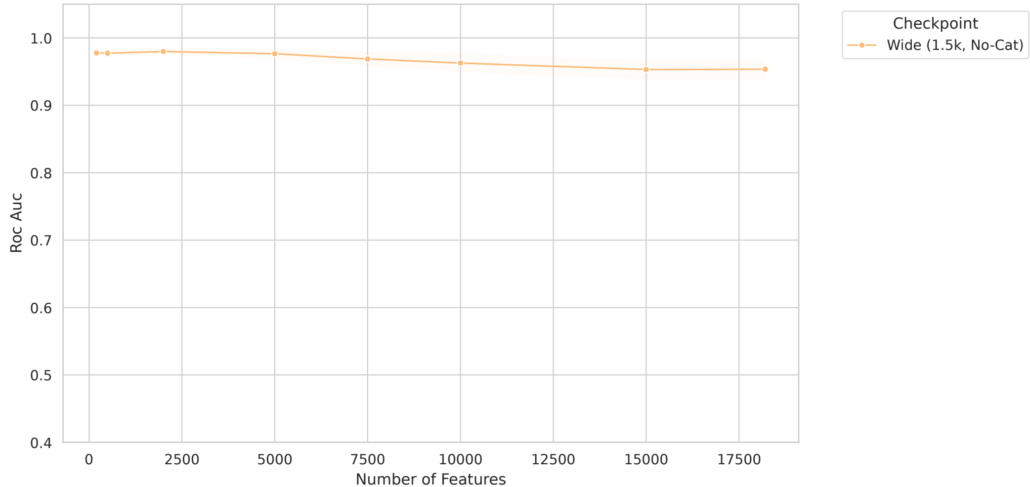
BRCA - Roc Auc vs Feature Count
