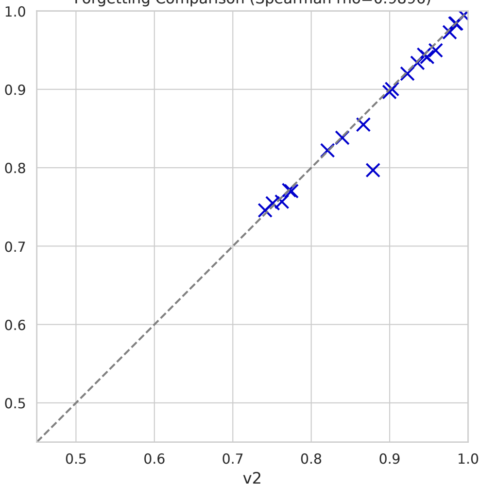
Forgetting Comparison (Spearman rho=0.9896)
