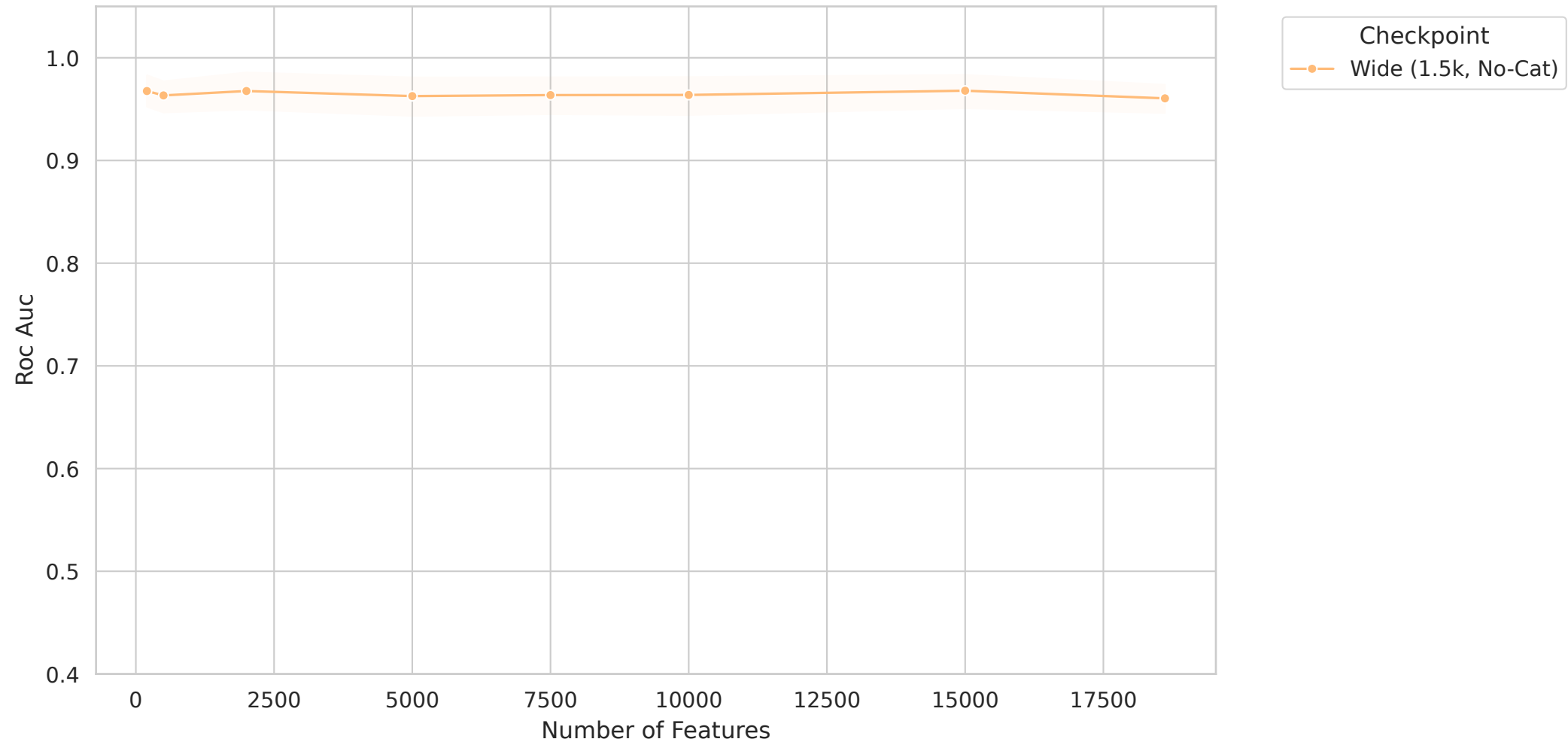
GBM - Roc Auc vs Feature Count
