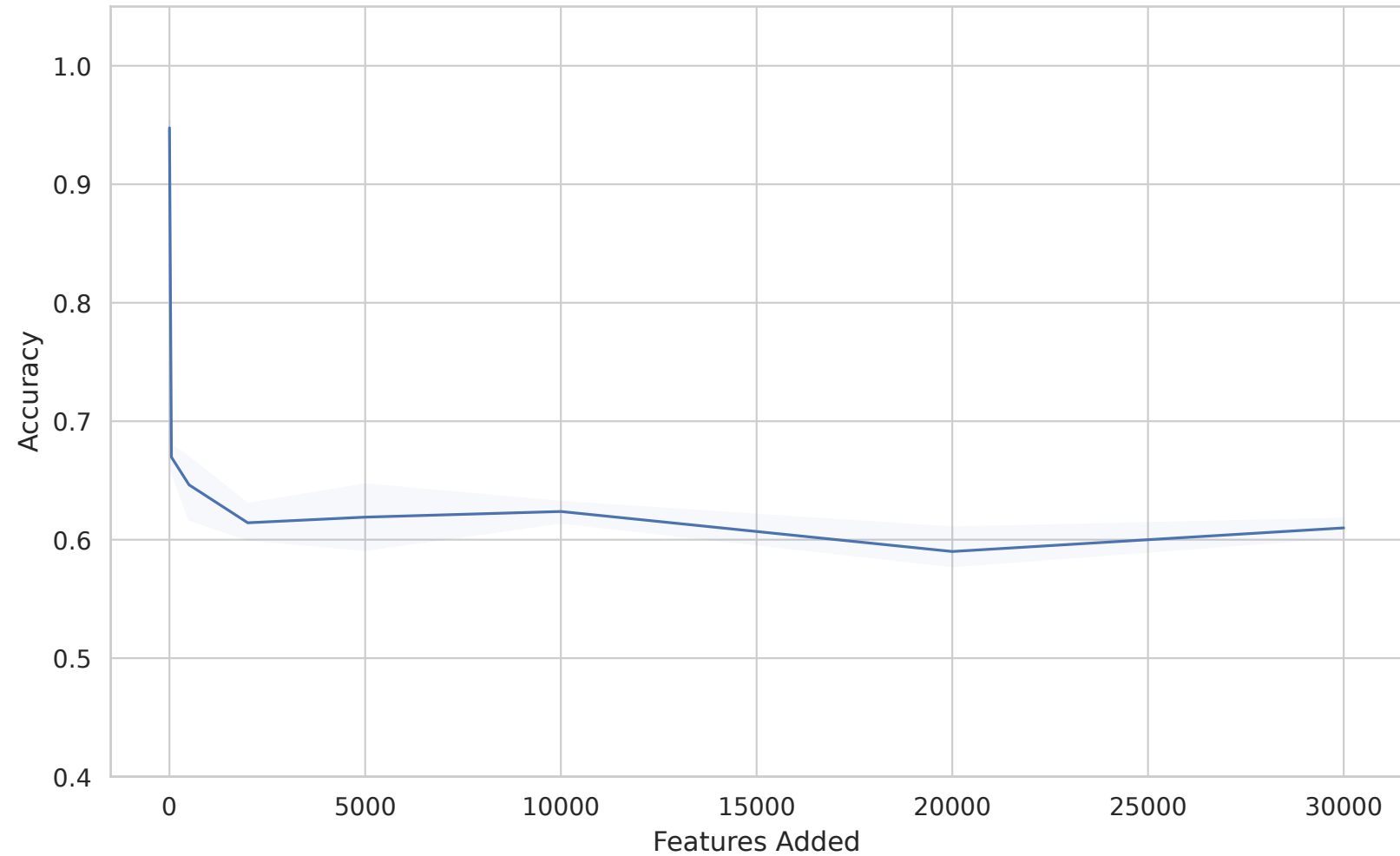
Dataset 40984 - accuracy vs Features Added
