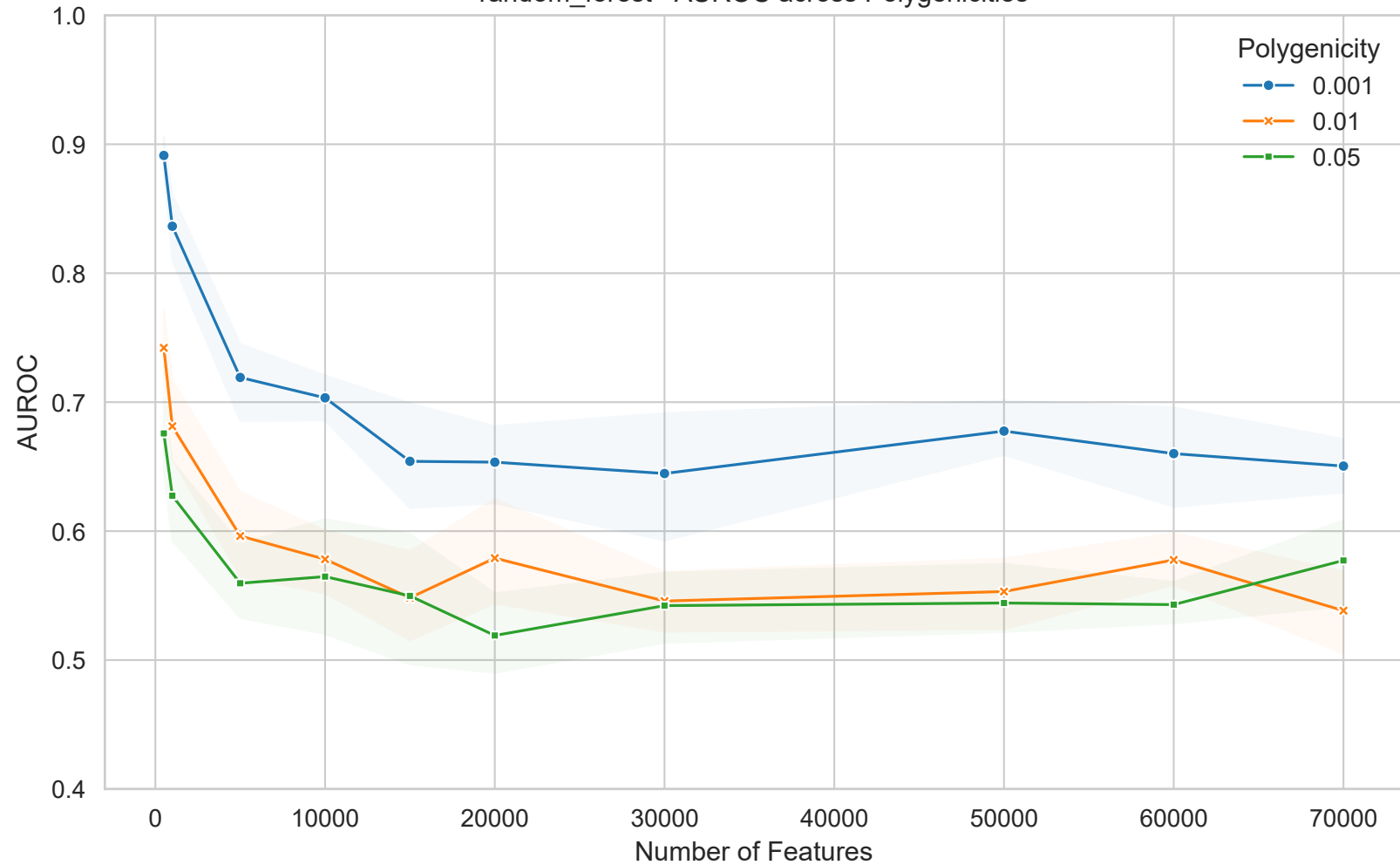
random_forest - AUROC across Polygenicities
