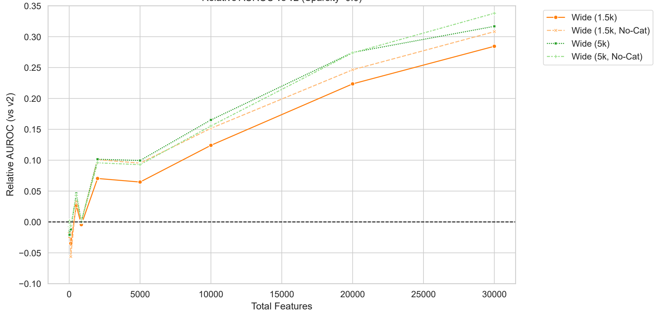
Relative AUROC vs v2 (Sparsity=0.0)
