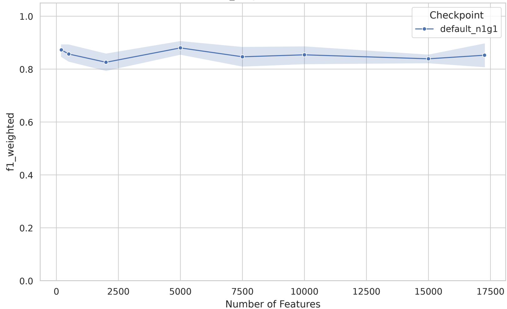
COAD - f1_weighted vs Feature Count
