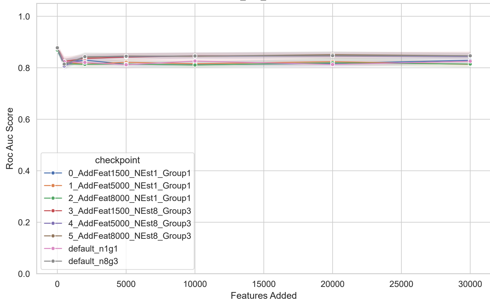
Dataset 40536 - roc_auc_score vs Features Added
