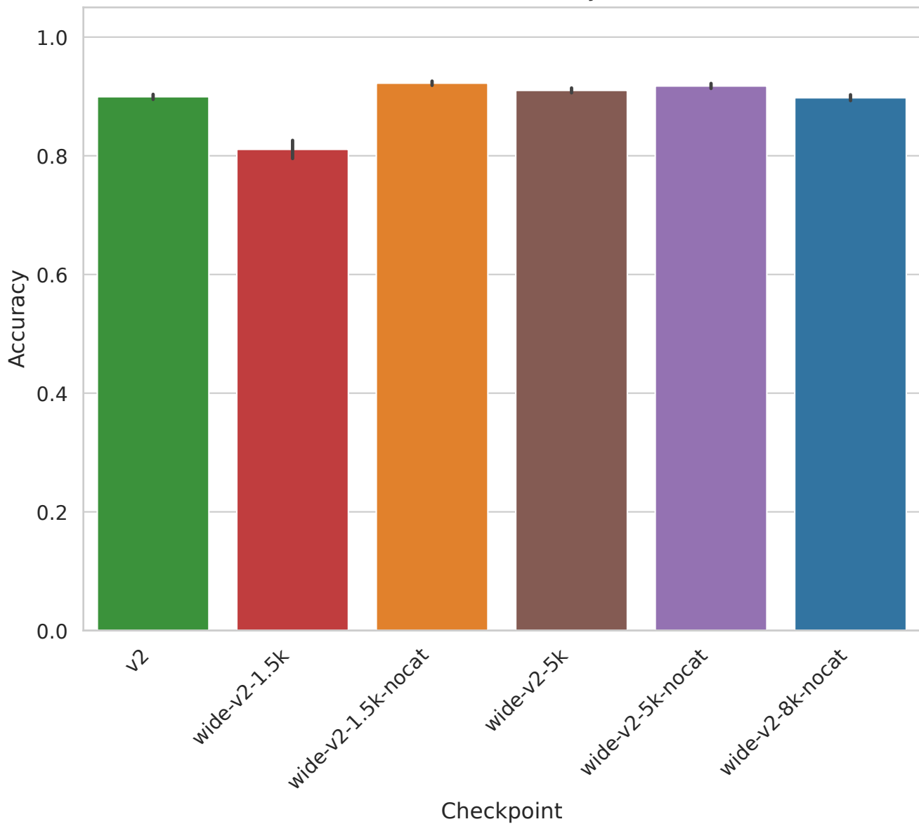
PCMAC - Accuracy
