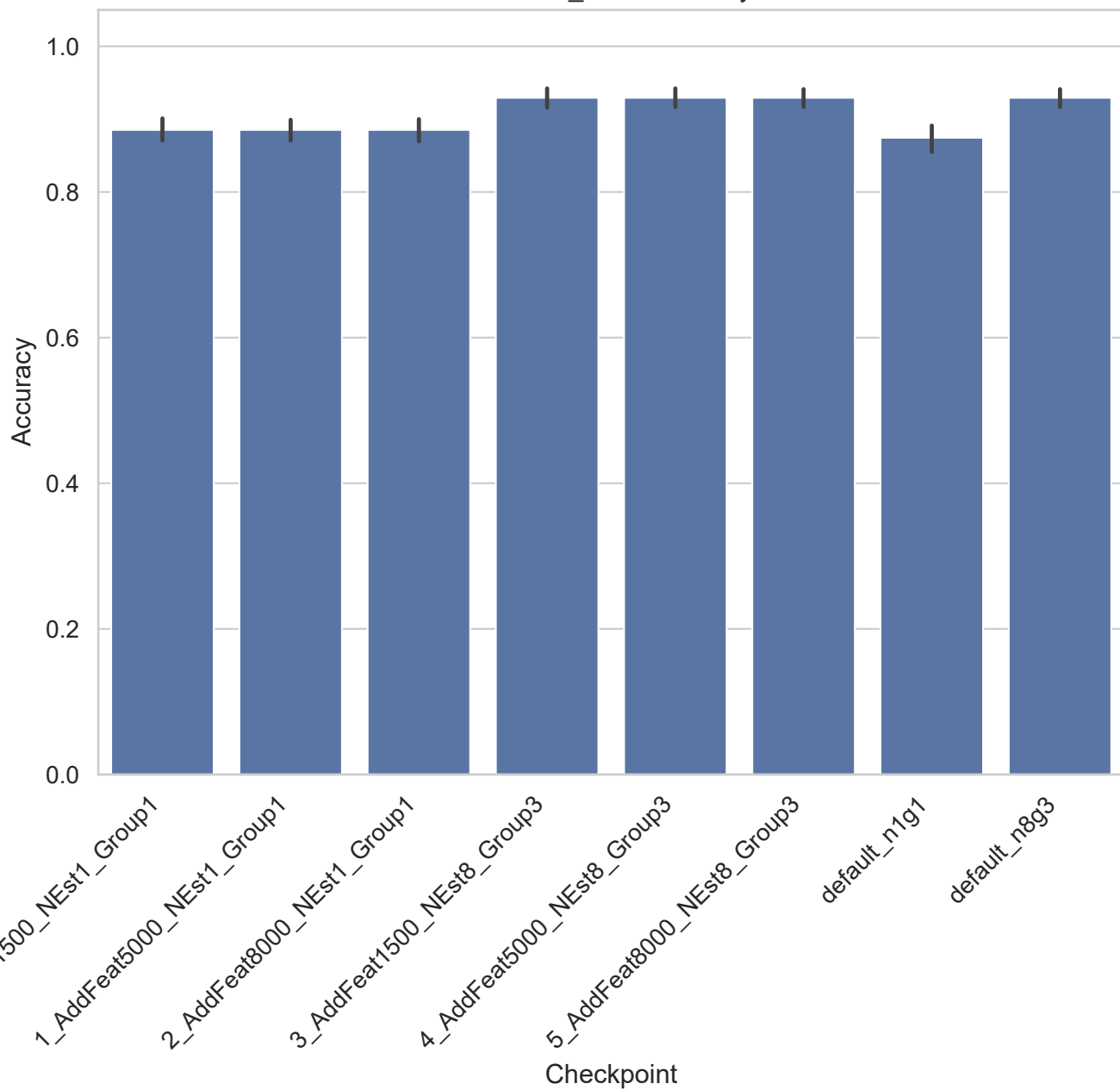
Prostate_GE - Accuracy
