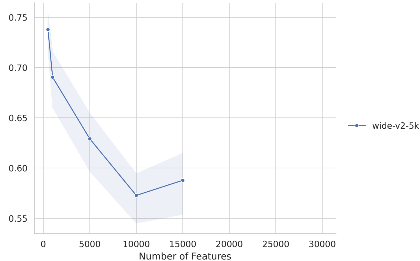
Polygenicity: 0.05
