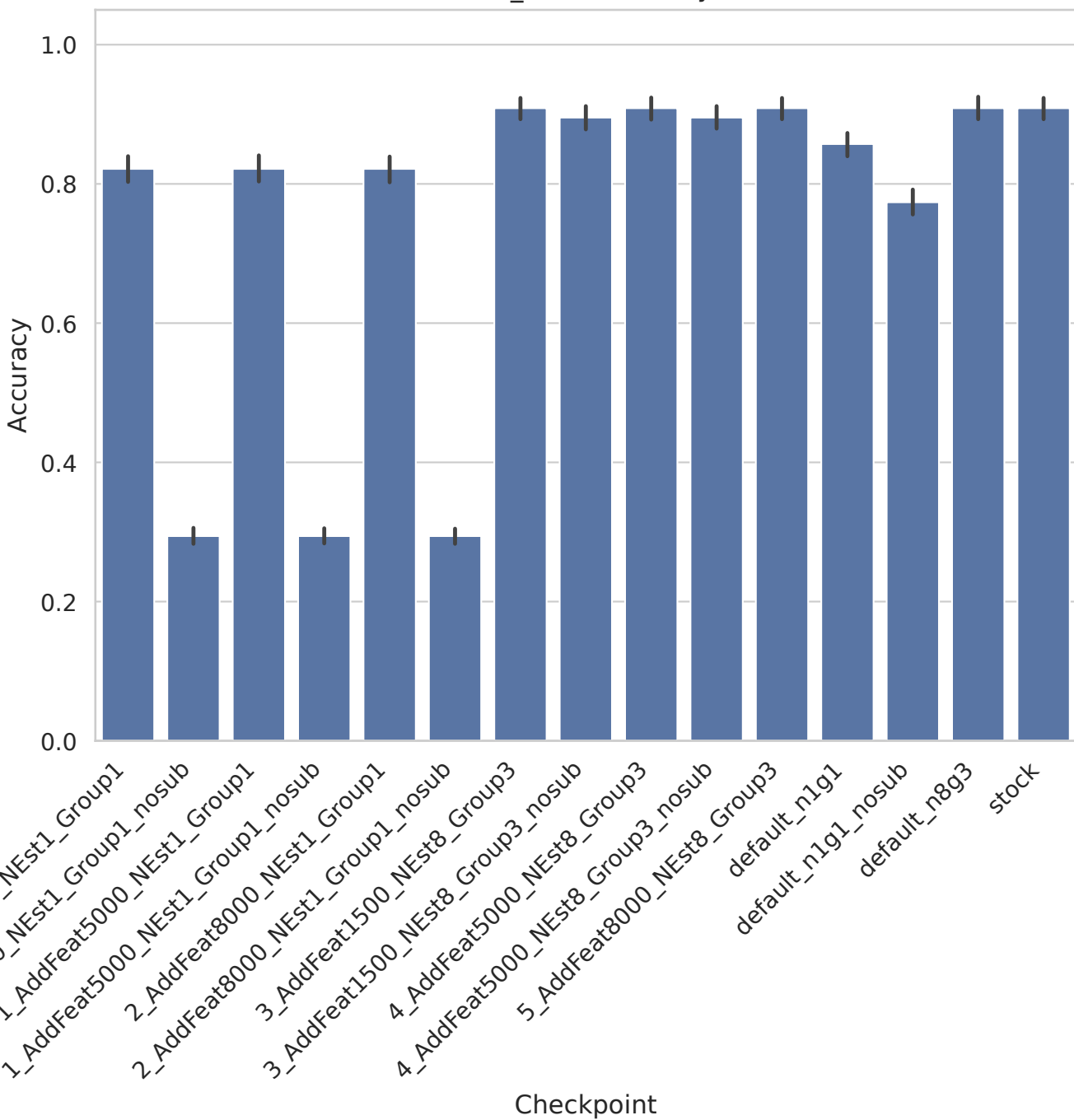
TOX_171 - Accuracy
