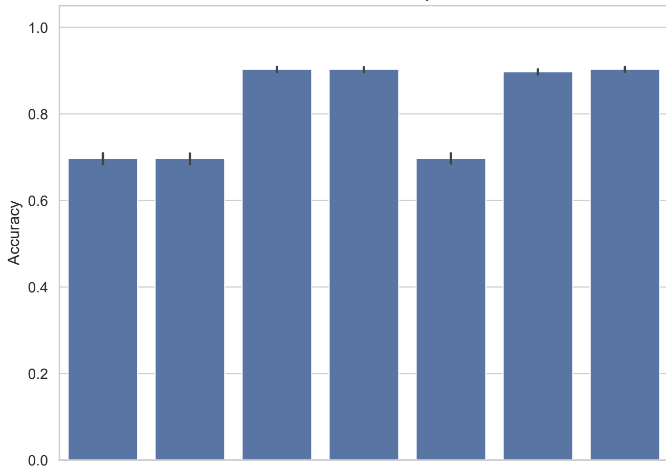
madelon - Accuracy
