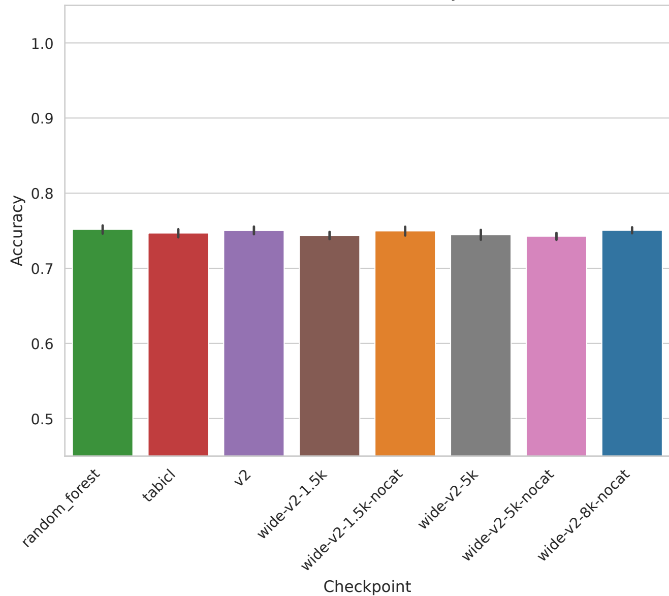
Task 363626 - Accuracy
