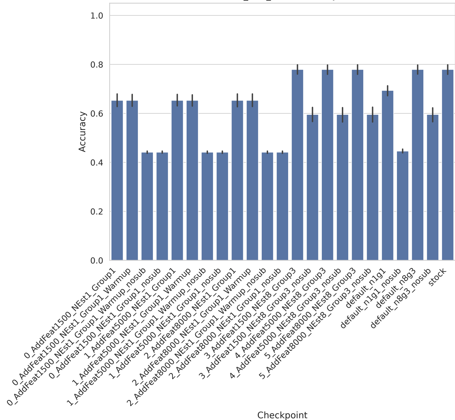
CLL_SUB_111 - Accuracy
