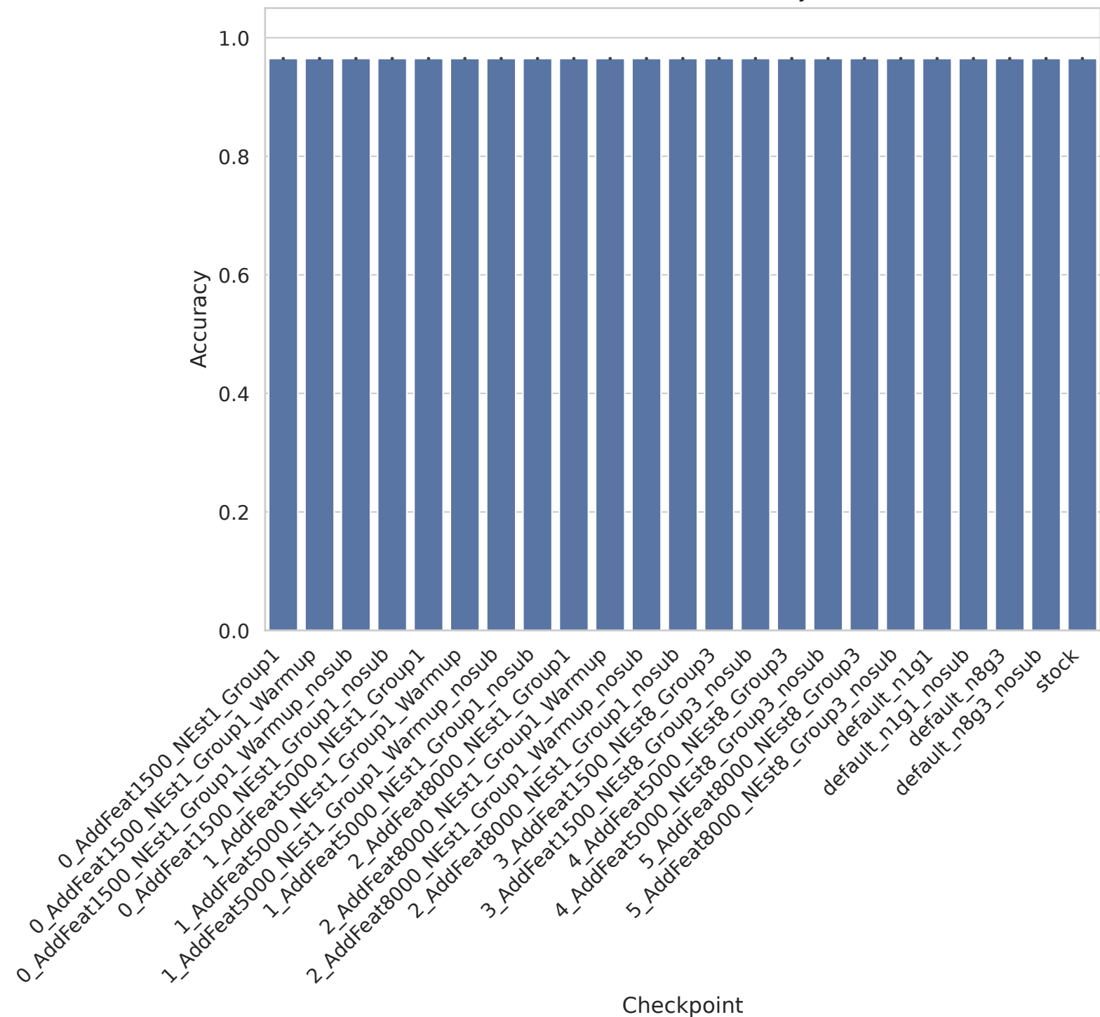
Task 363677 - Accuracy
