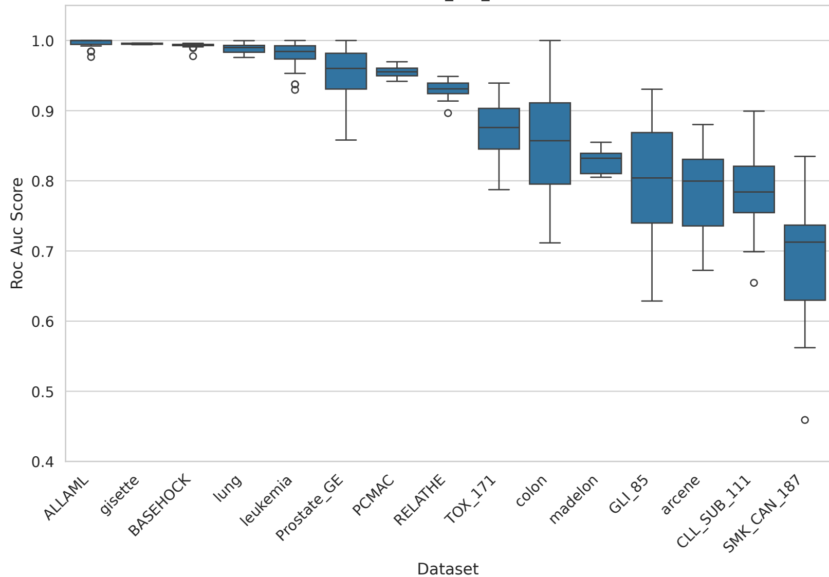
hdlss - roc_auc_score
