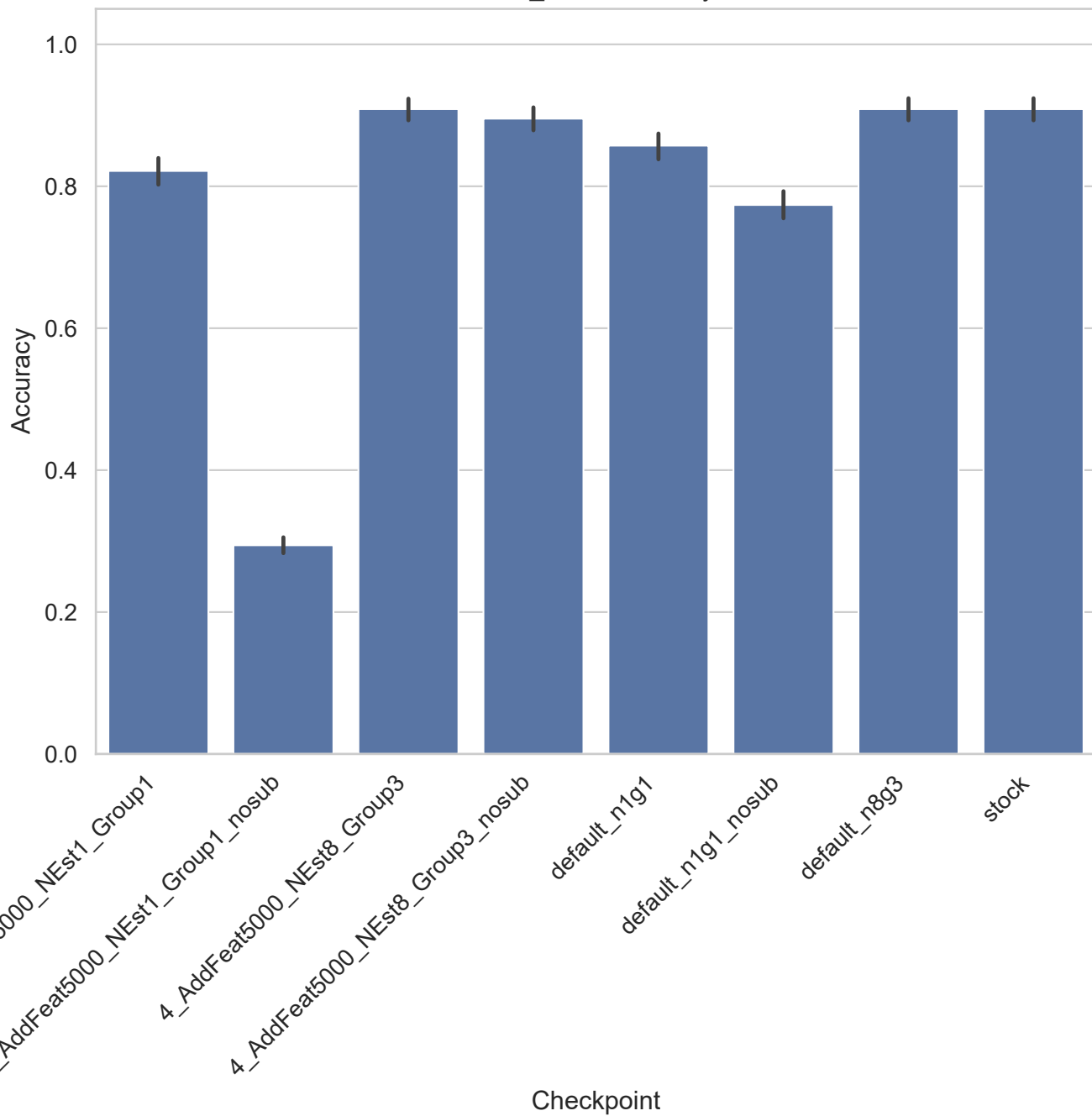
TOX_171 - Accuracy
