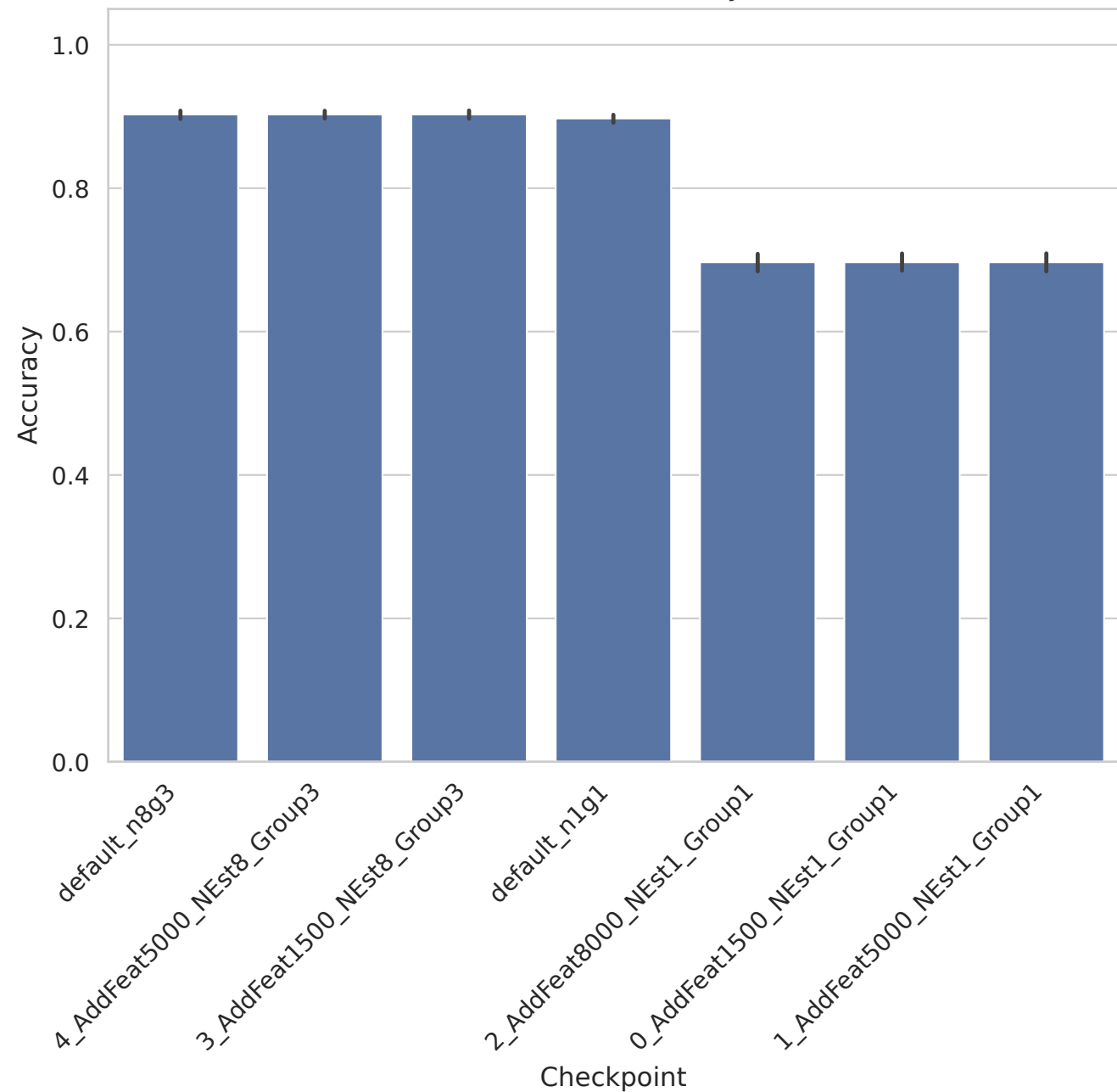
madelon - Accuracy
