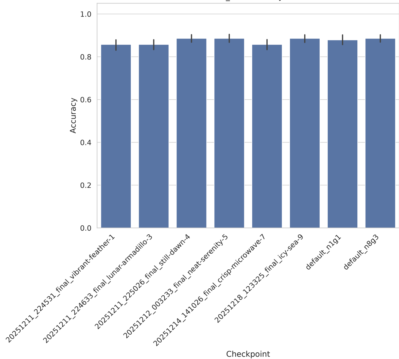
GLI_85 - Accuracy
