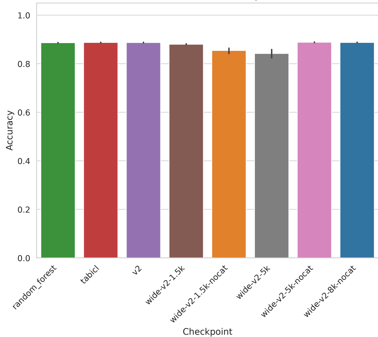
Task 363711 - Accuracy
