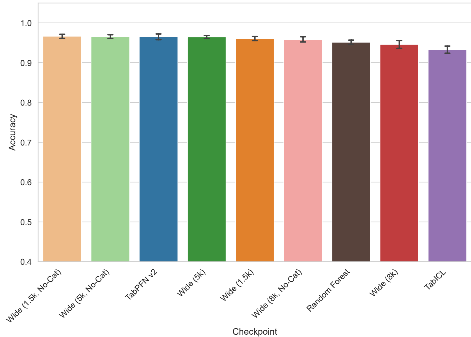
Task 363702 - Accuracy
