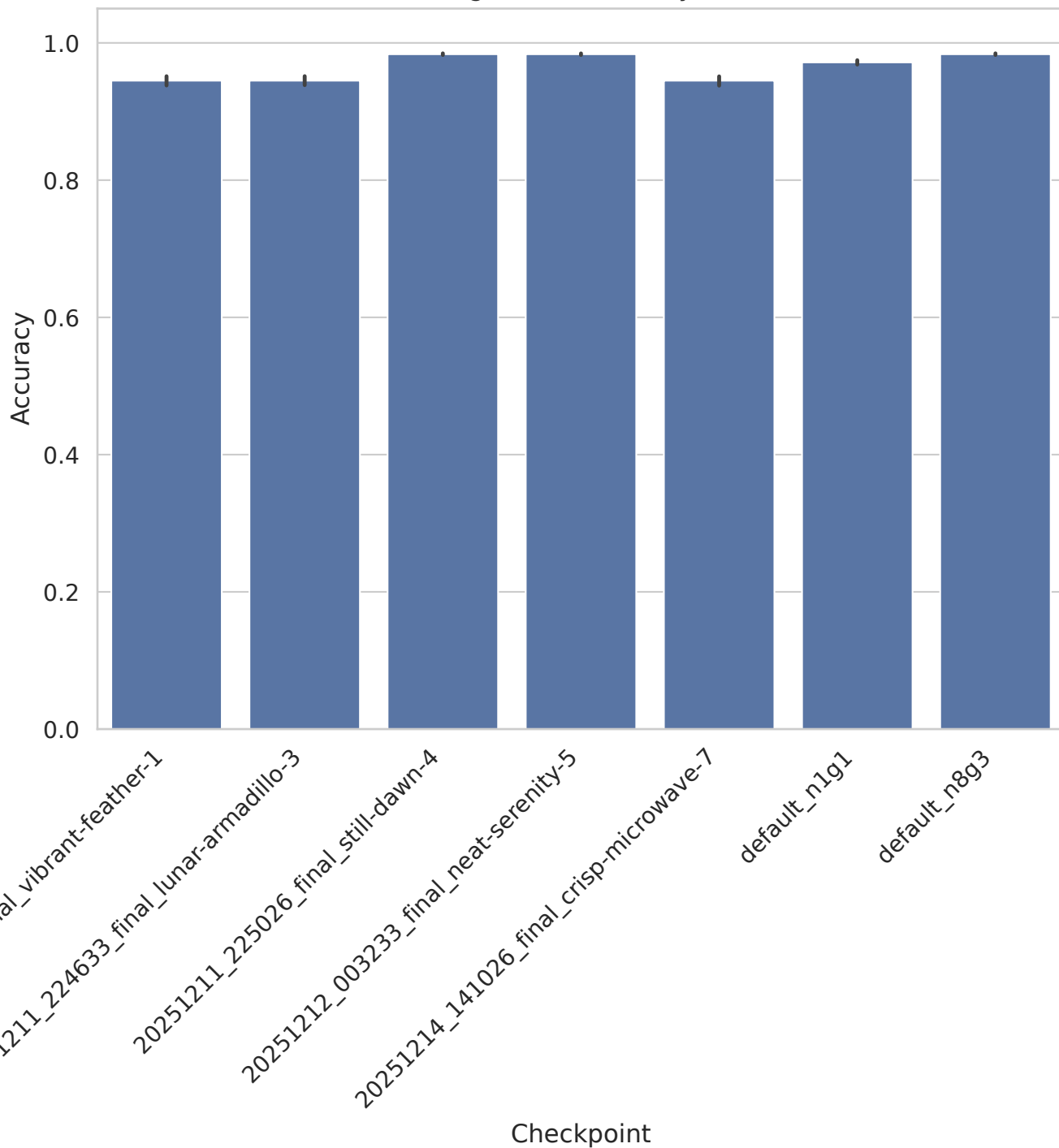
gisette - Accuracy
