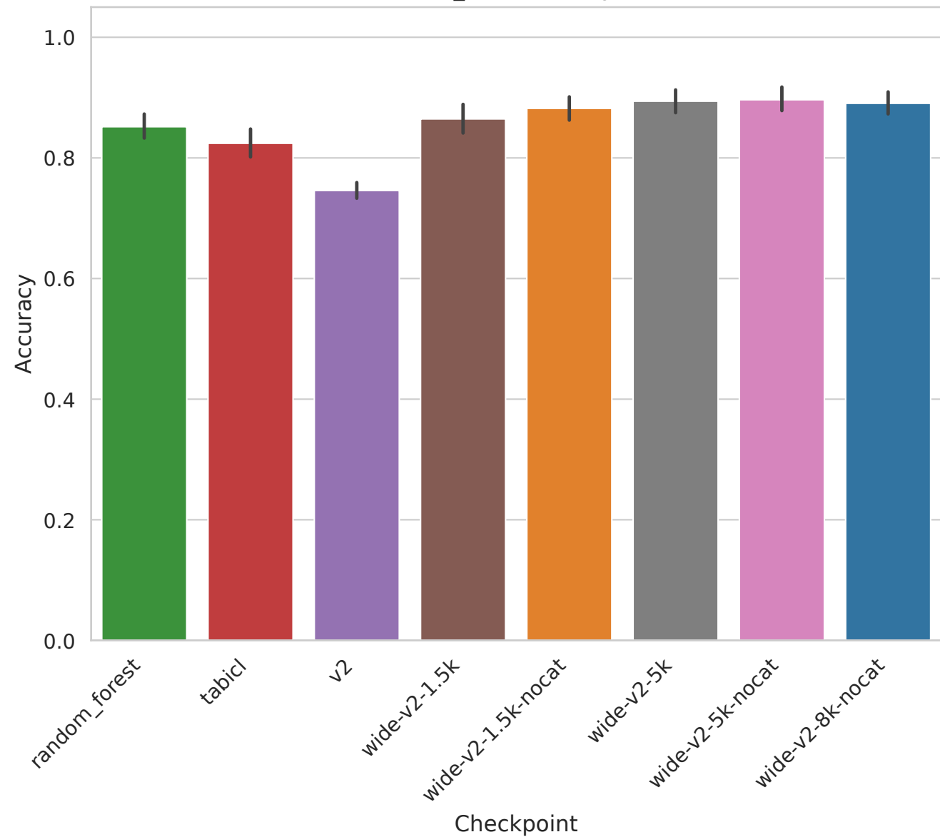
GLI_85 - Accuracy
