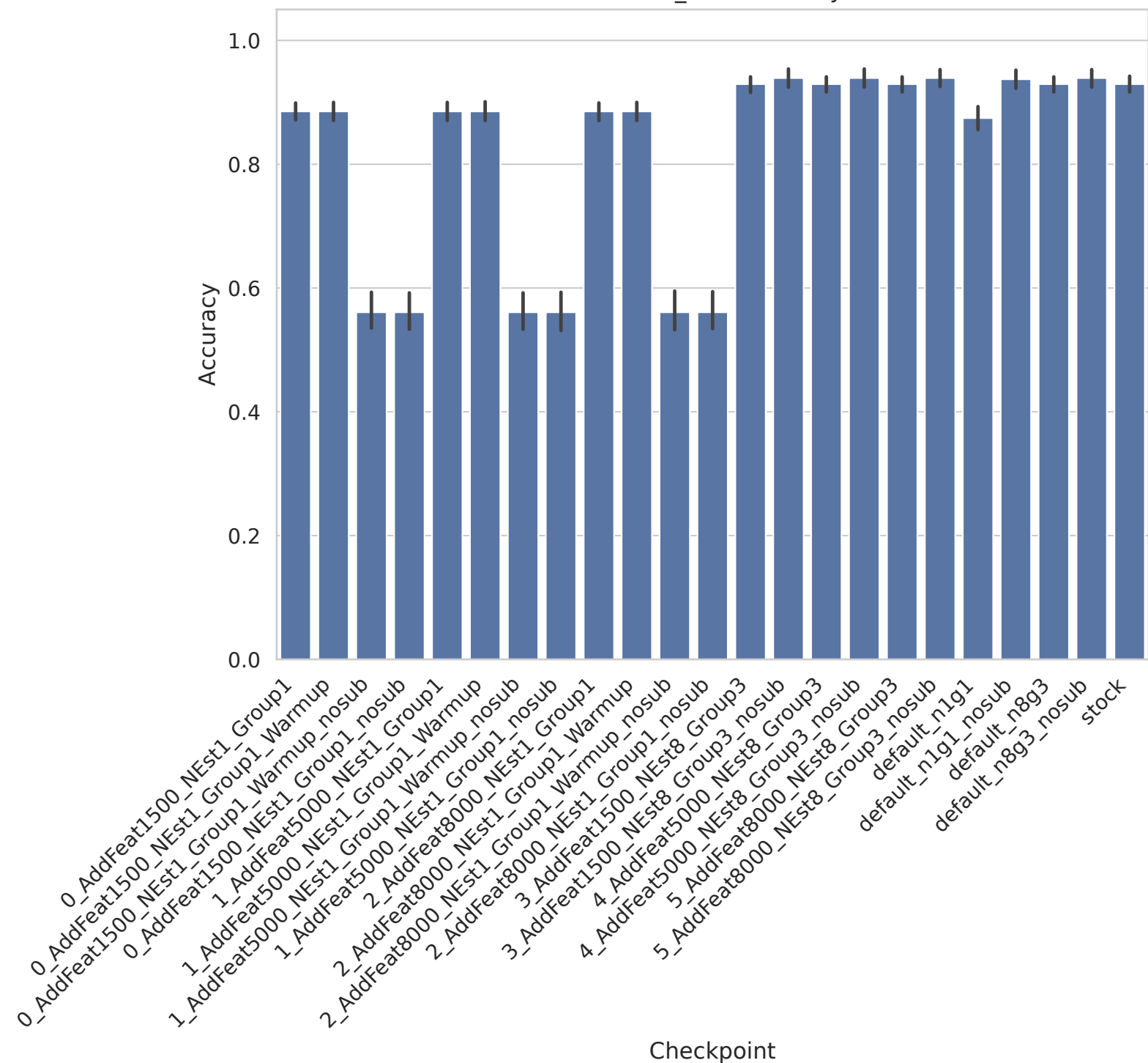
Prostate_GE - Accuracy
