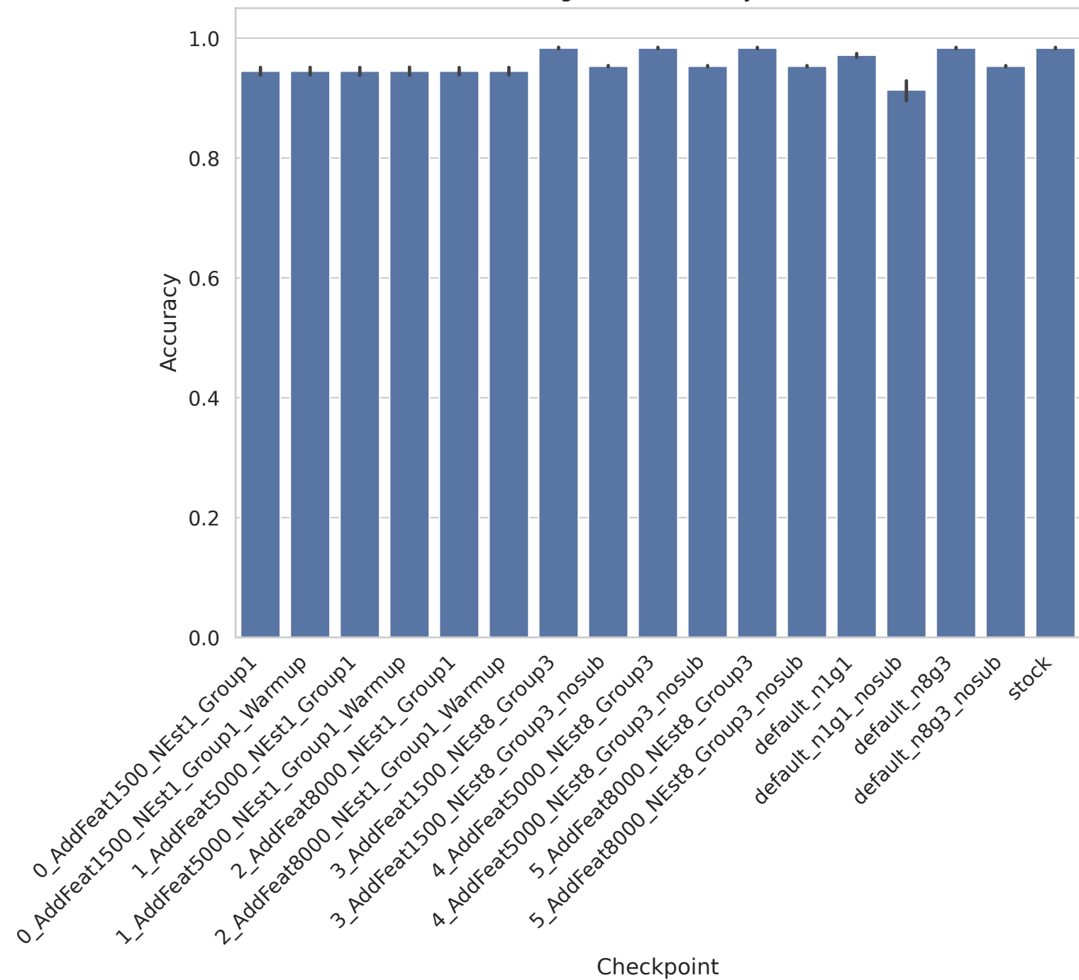
gisette - Accuracy
