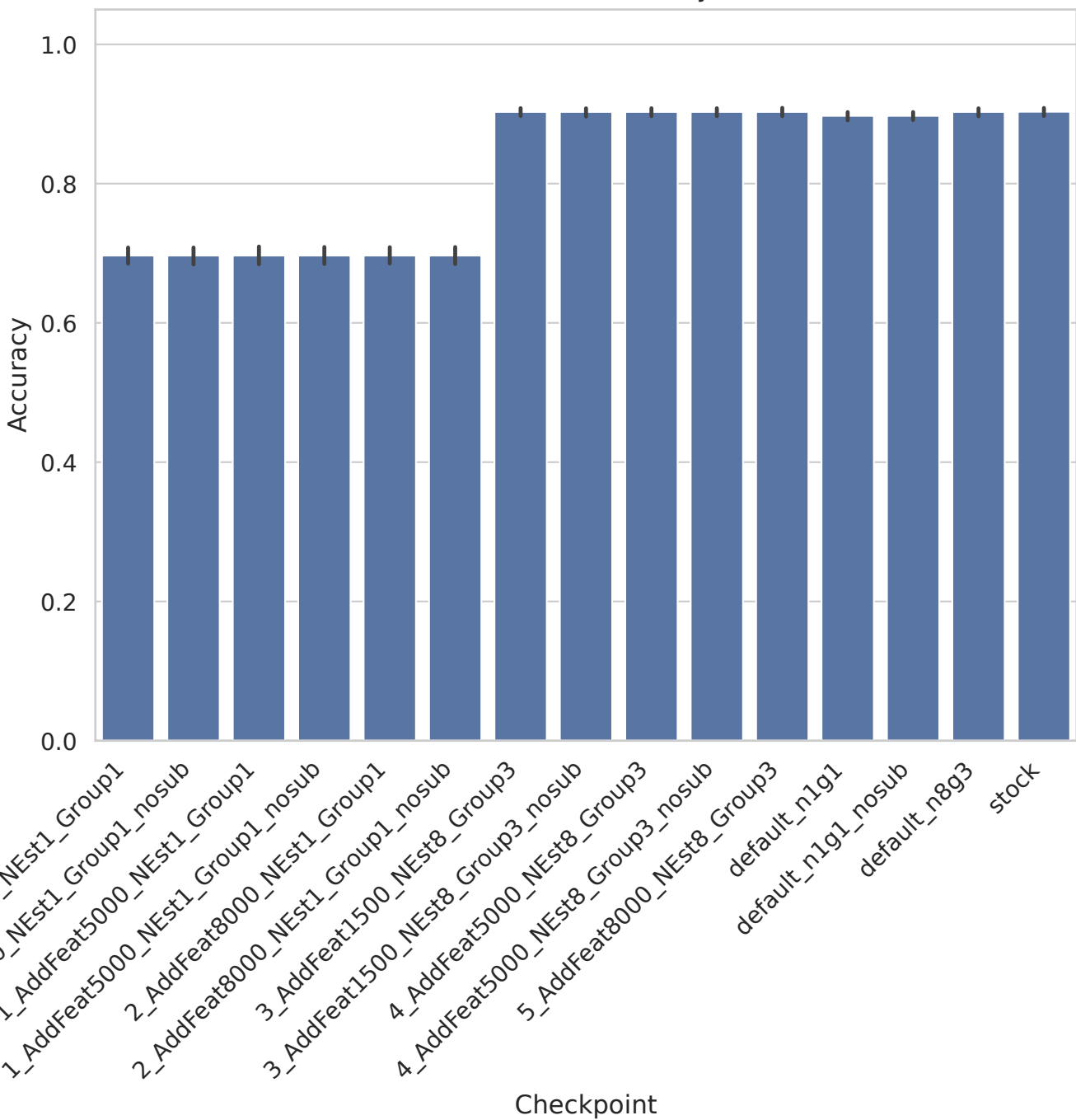
madelon - Accuracy
