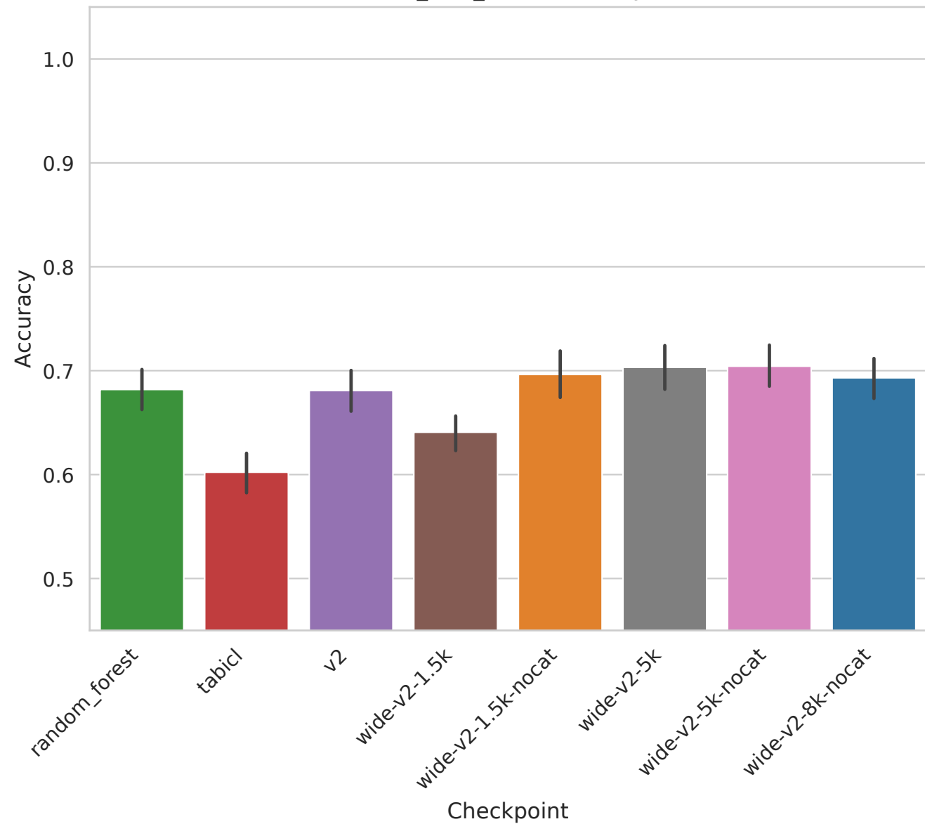
SMK_CAN_187 - Accuracy
