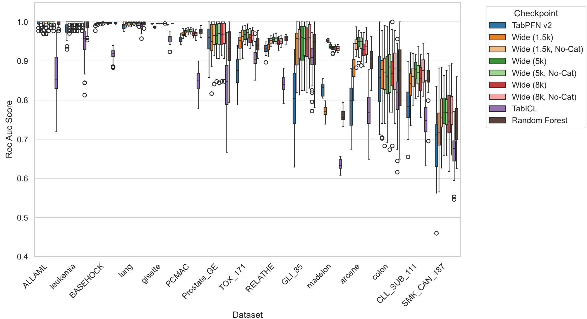
hdlss - roc_auc_score
