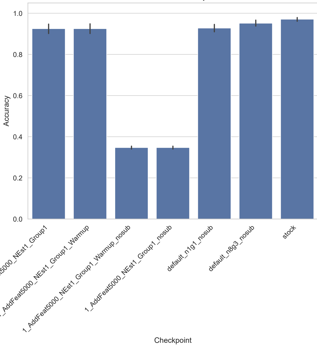
leukemia - Accuracy
