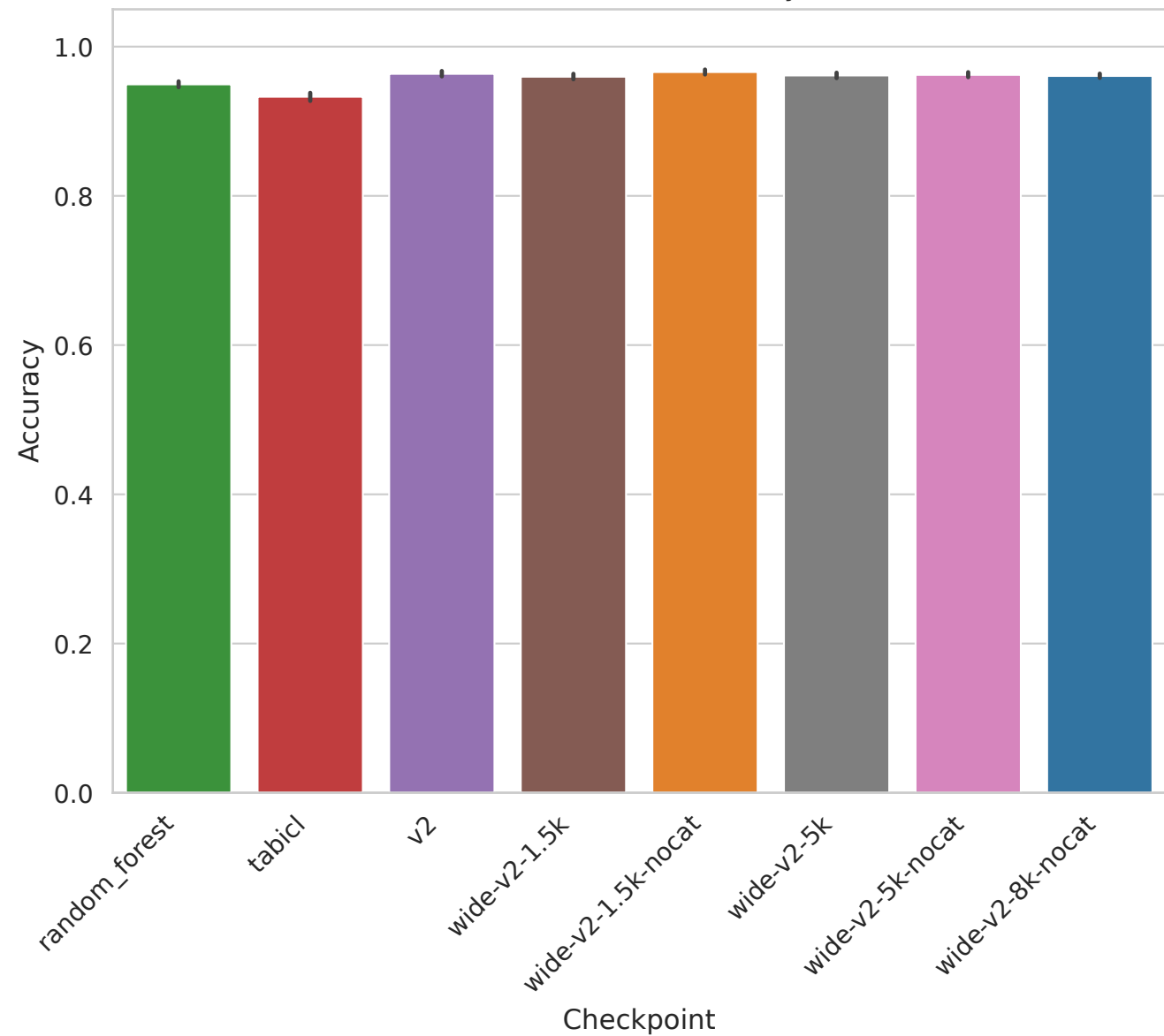
Task 363702 - Accuracy
