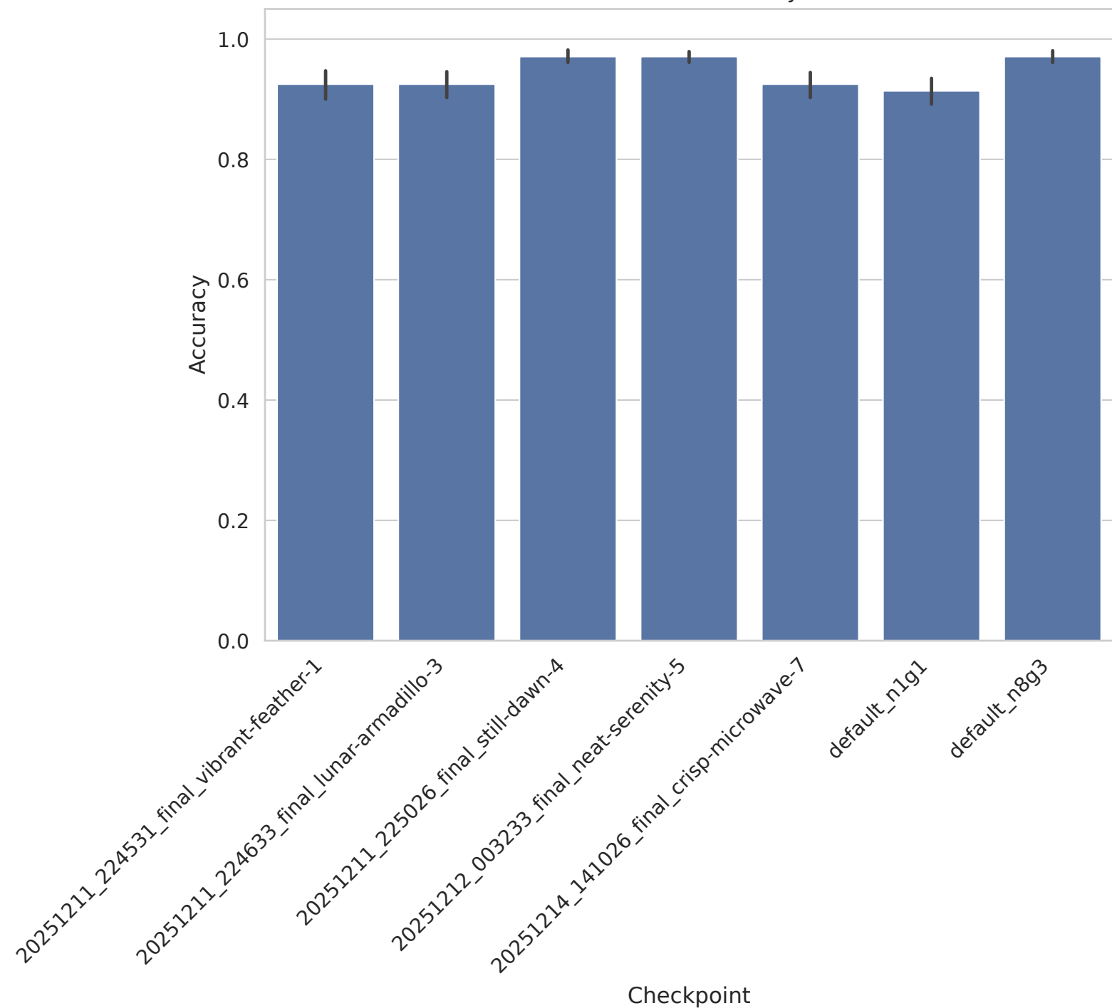
leukemia - Accuracy
