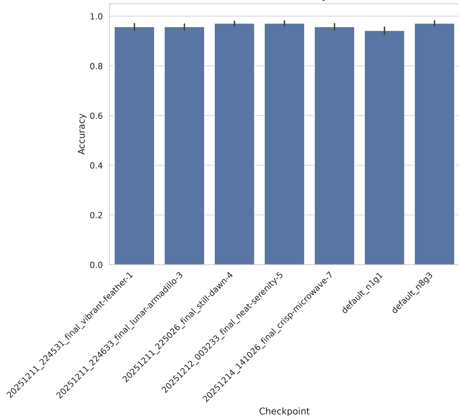
ALLAML - Accuracy
