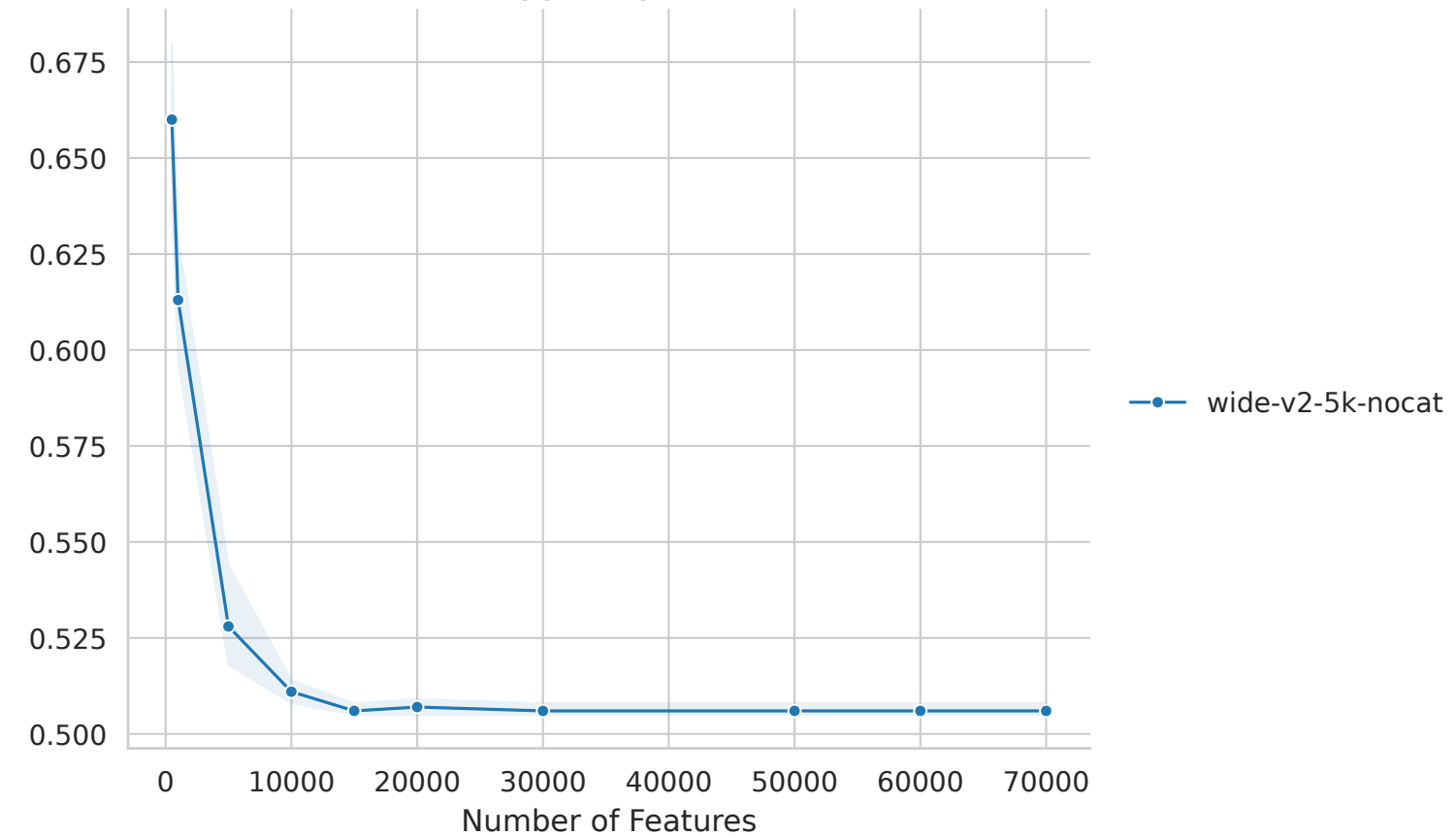
Polygenicity: 0.05
