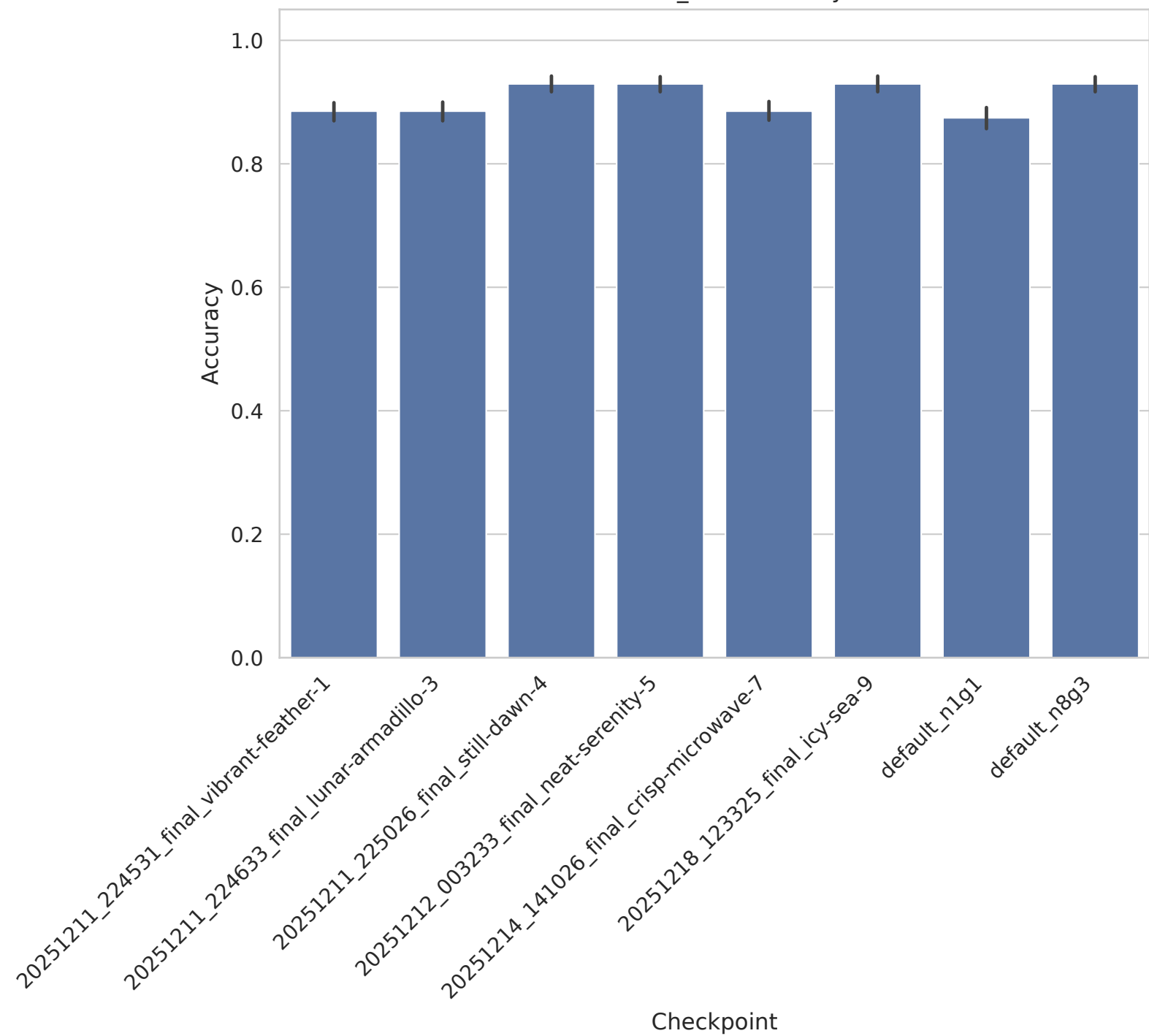
Prostate_GE - Accuracy
