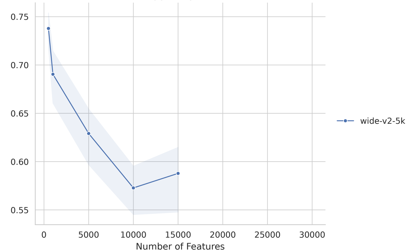
Polygenicity: 0.05
