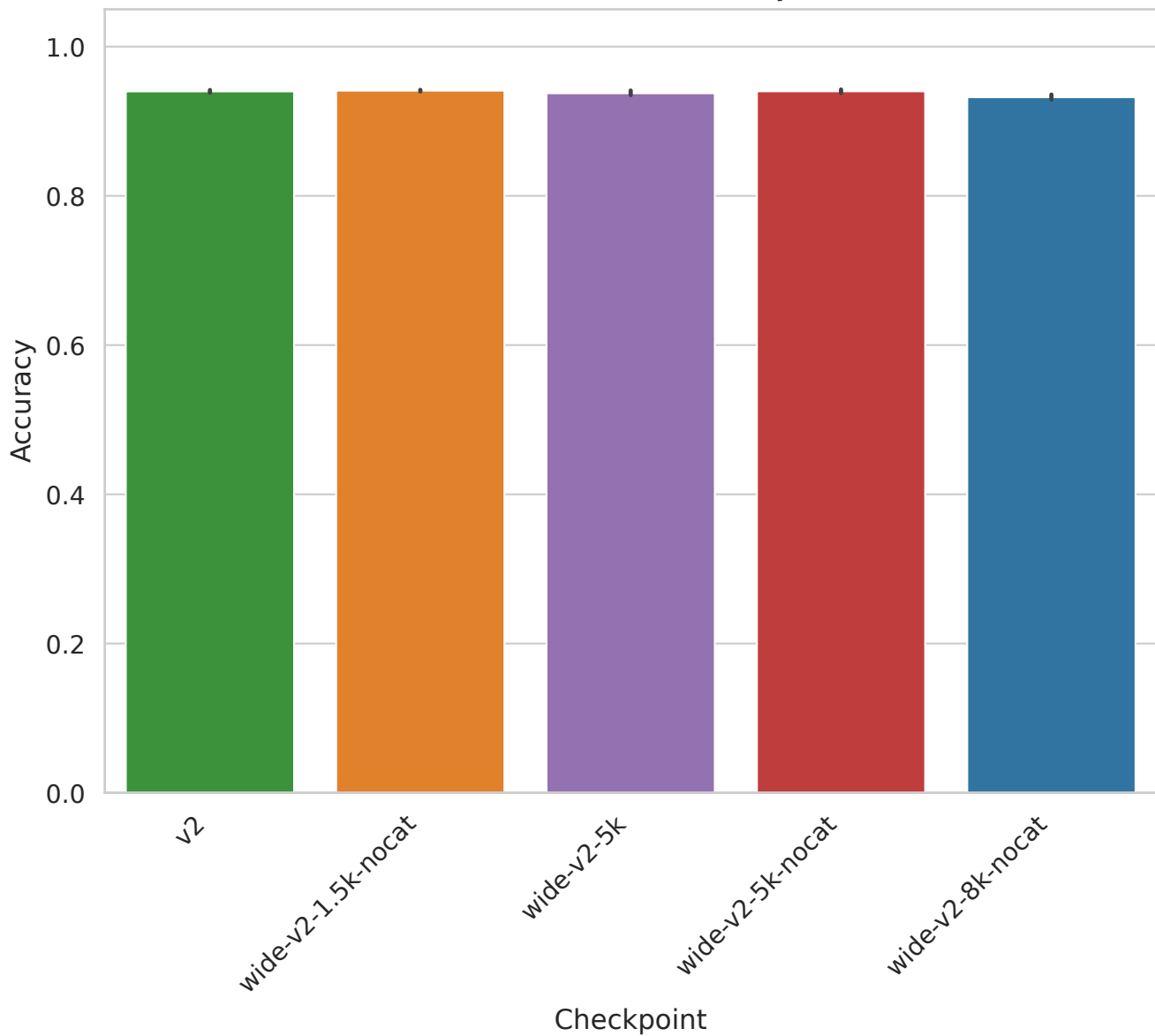
Task 363689 - Accuracy
