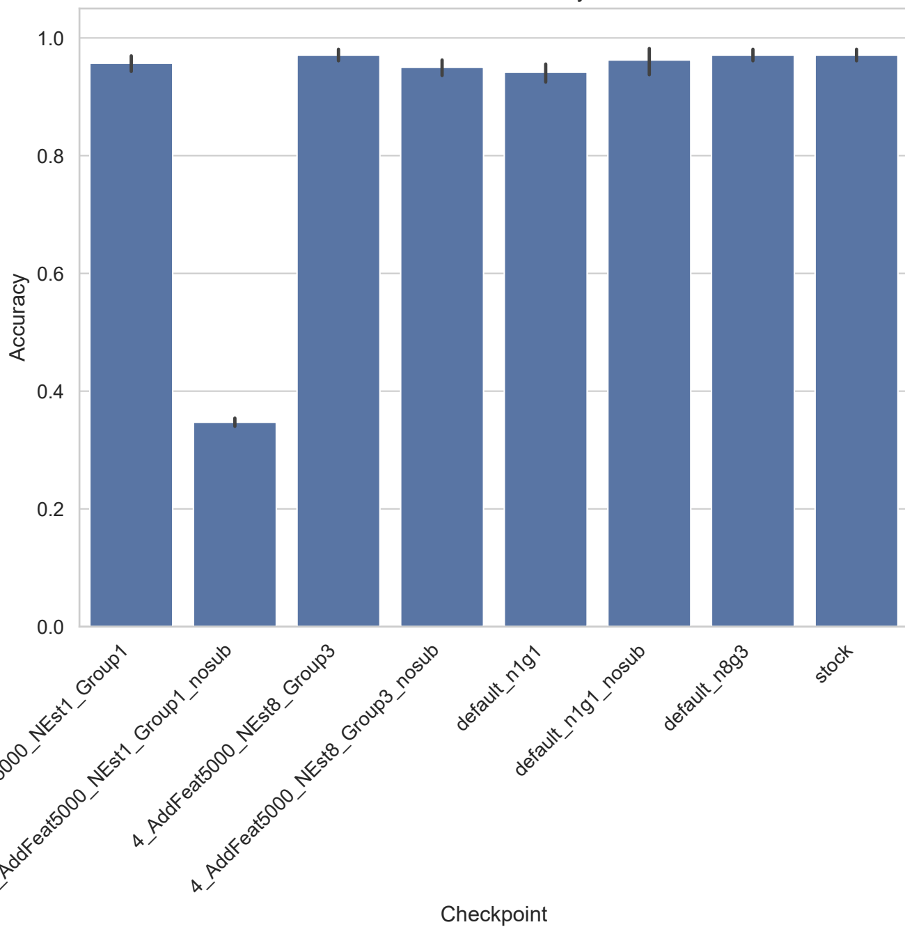
ALLAML - Accuracy
