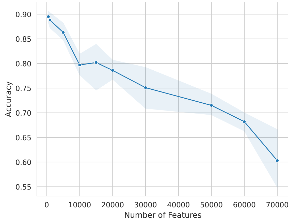
Polygenicity: 0.001
