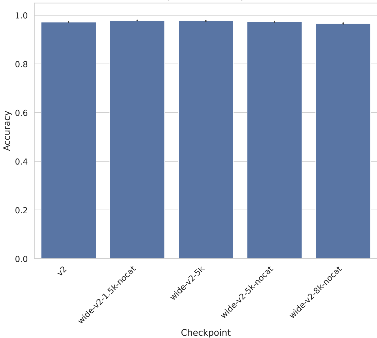
gisette - Accuracy
