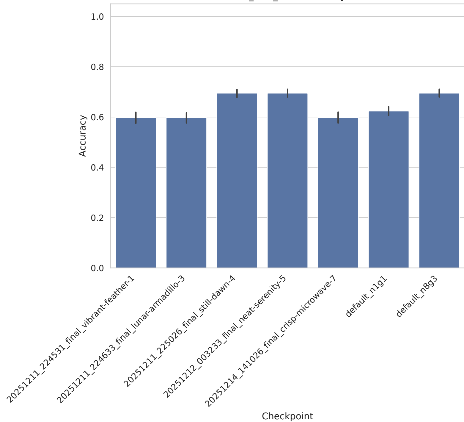
SMK_CAN_187 - Accuracy
