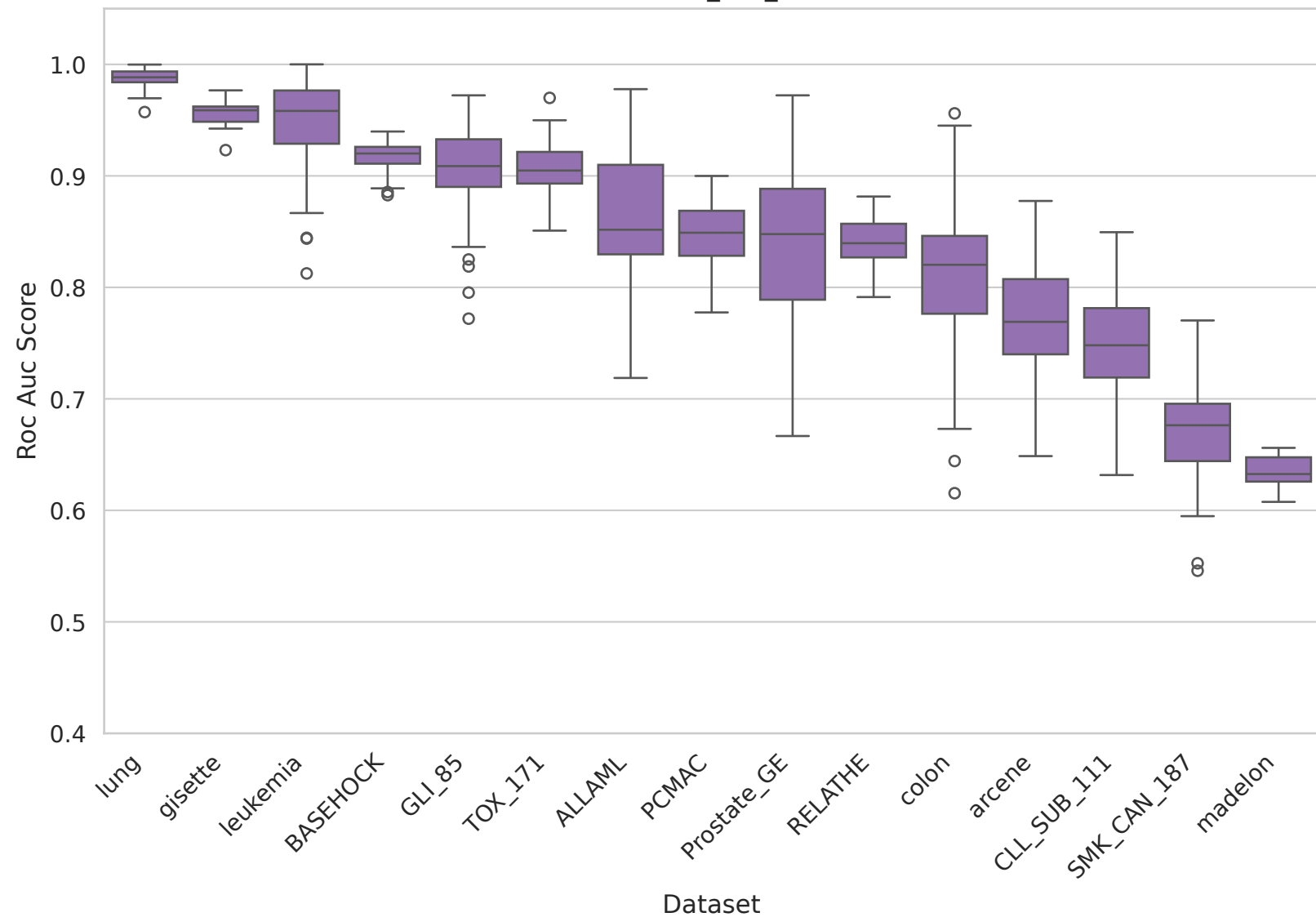
hdls - roc_auc_score
