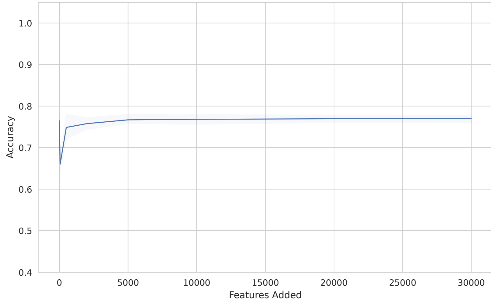
Dataset 46921 - accuracy vs Features Added
