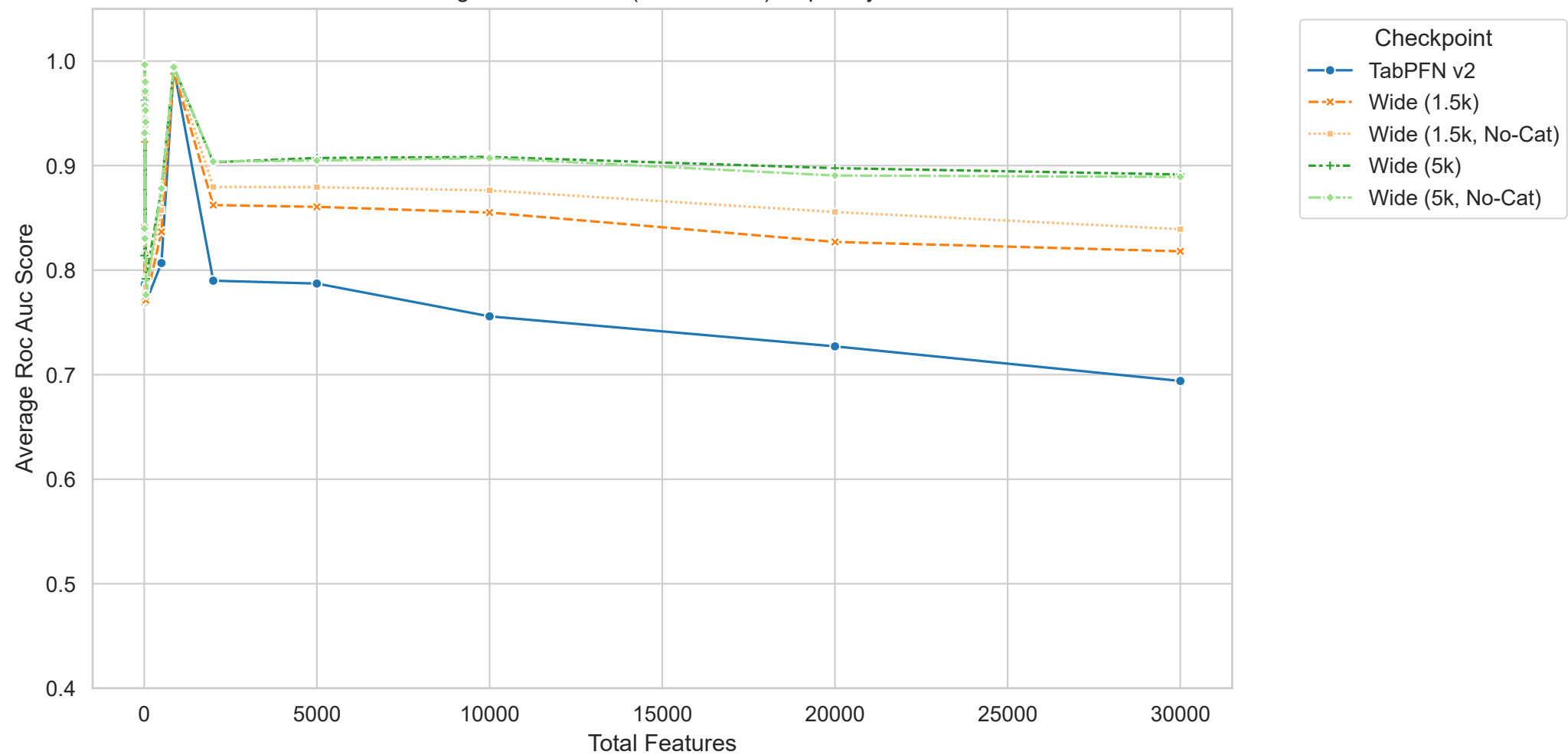
Average Performance (All Datasets) - Sparsity 0.02
