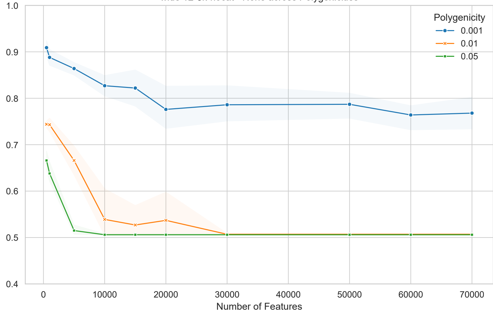
wide-v2-8k-nocat - None across Polygenicities
