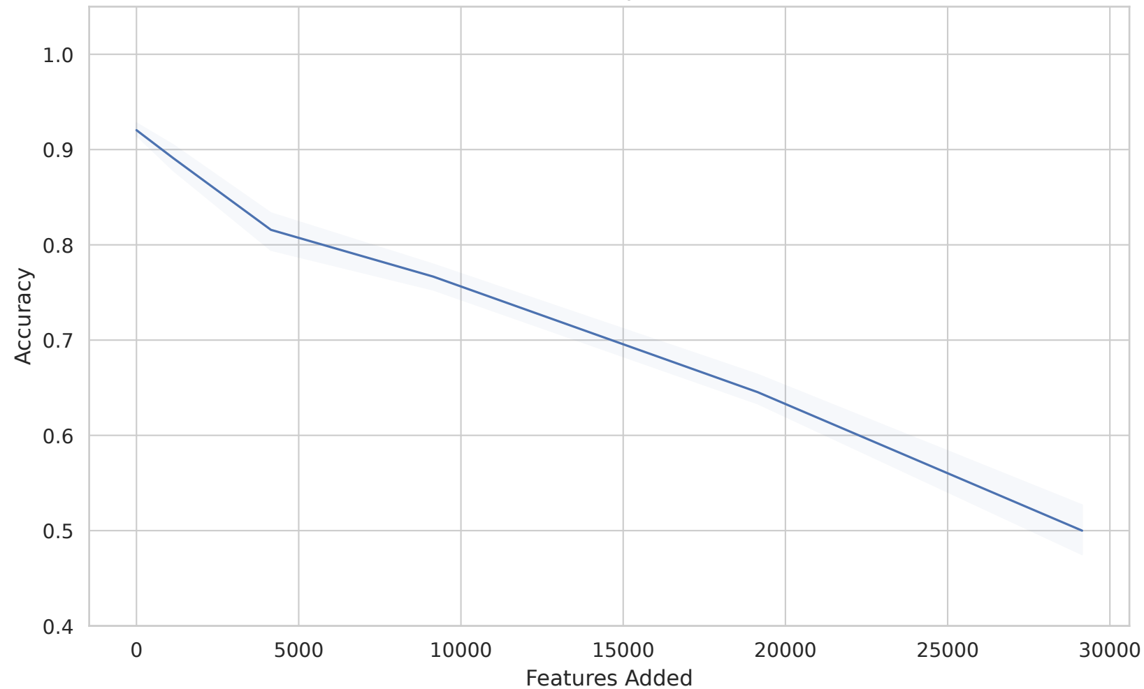
Dataset 1468 - accuracy vs Features Added
