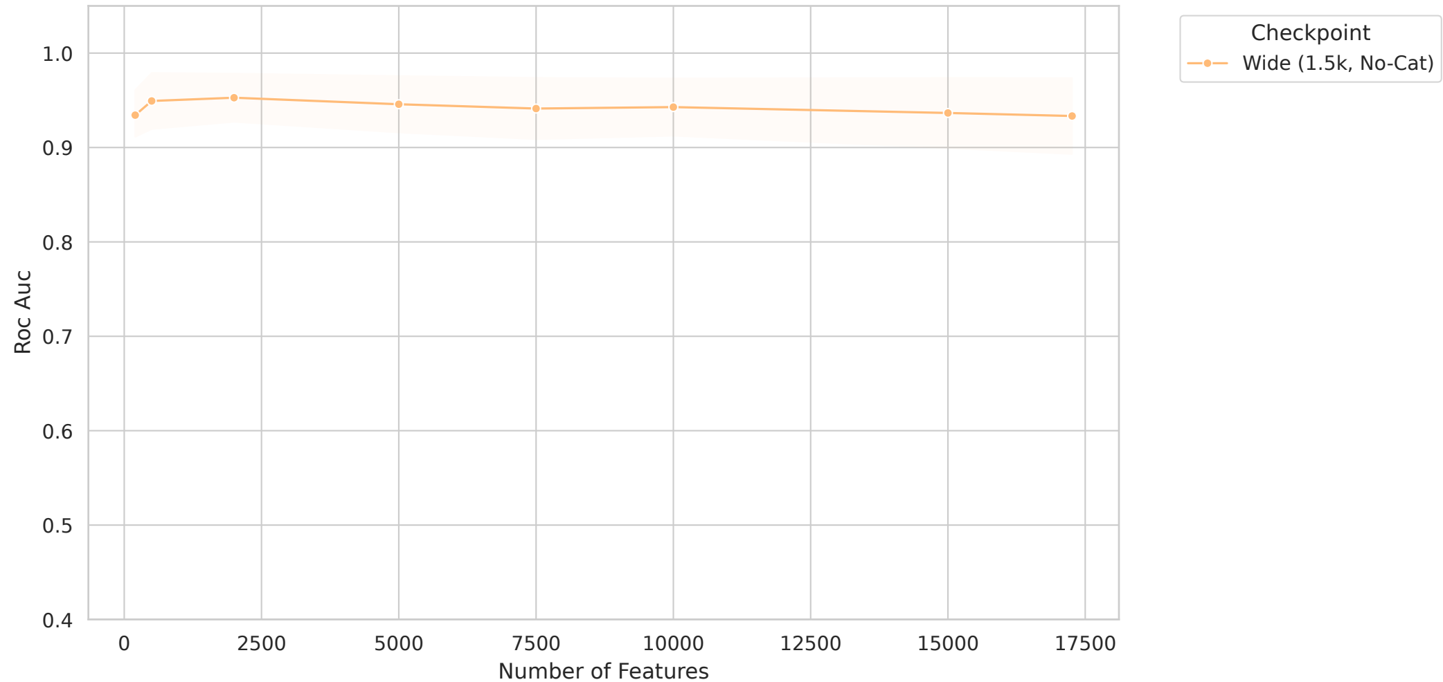
COAD - Roc Auc vs Feature Count
