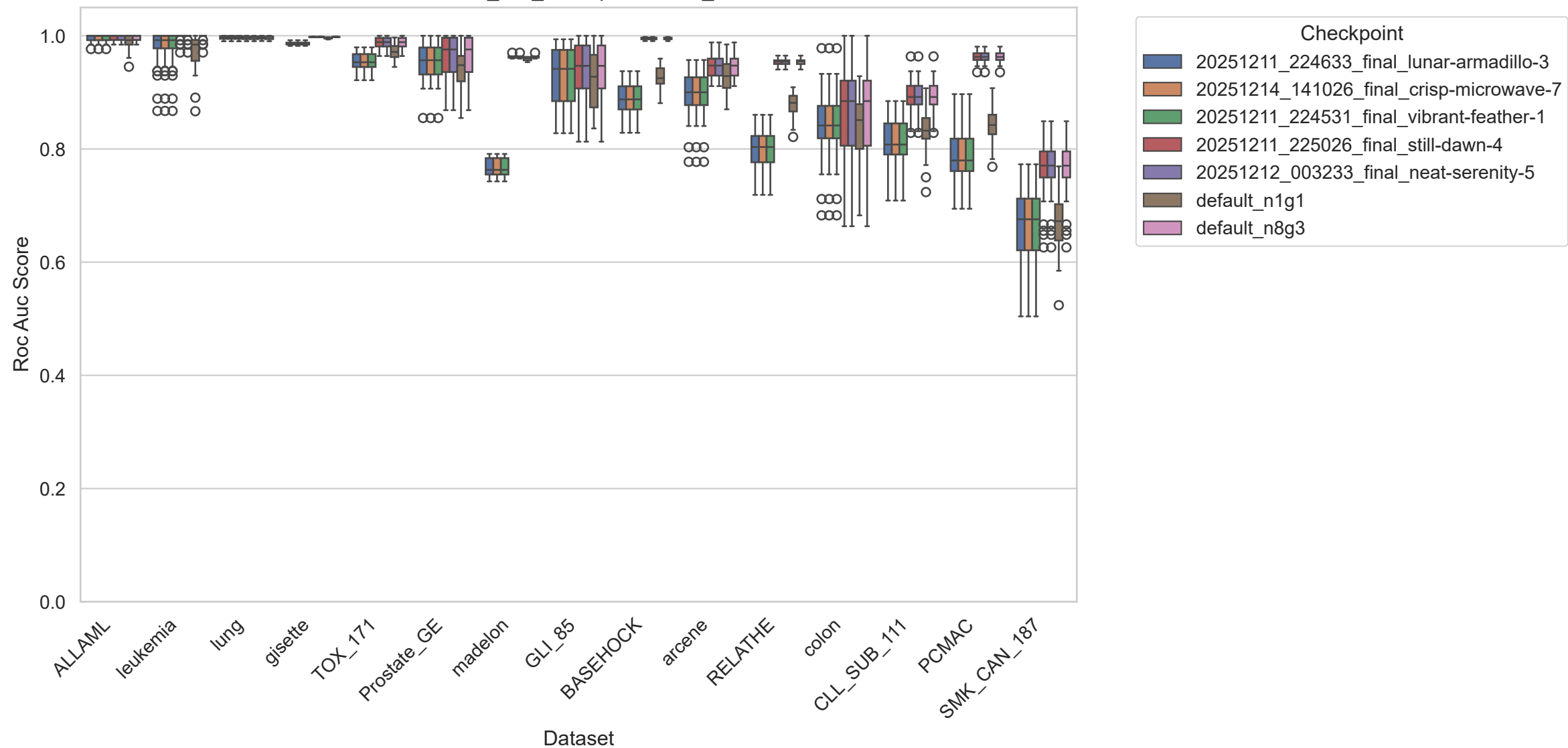
hdlss - roc_auc_score per dataset_name
