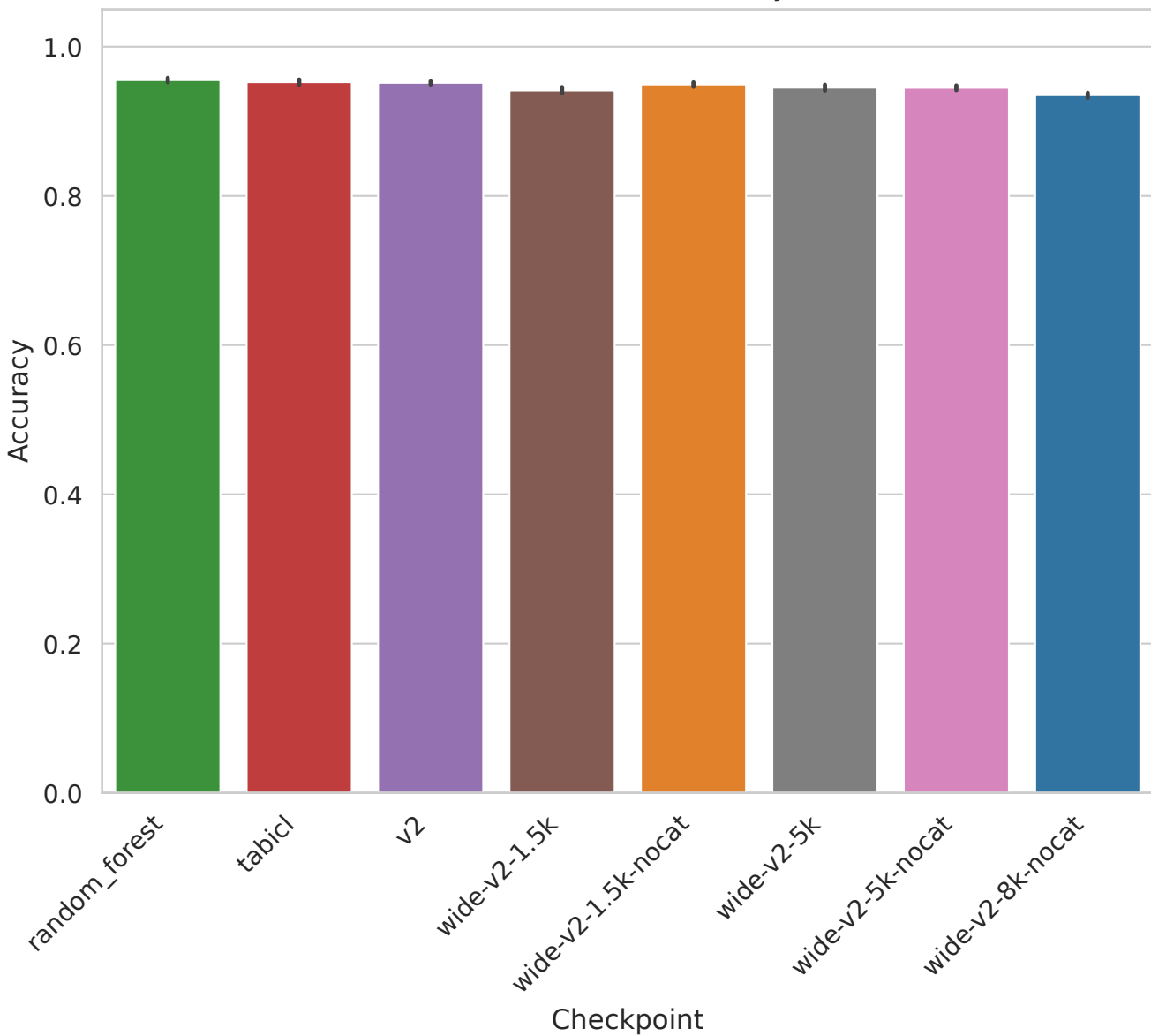
Task 363623 - Accuracy
