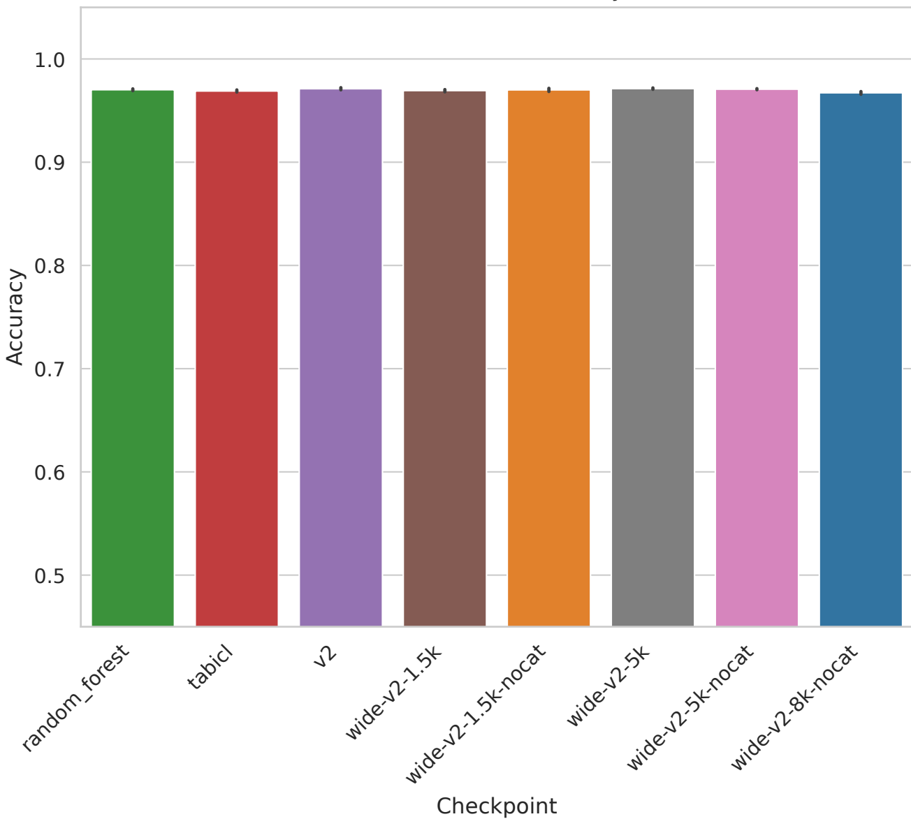
Task 363706 - Accuracy
