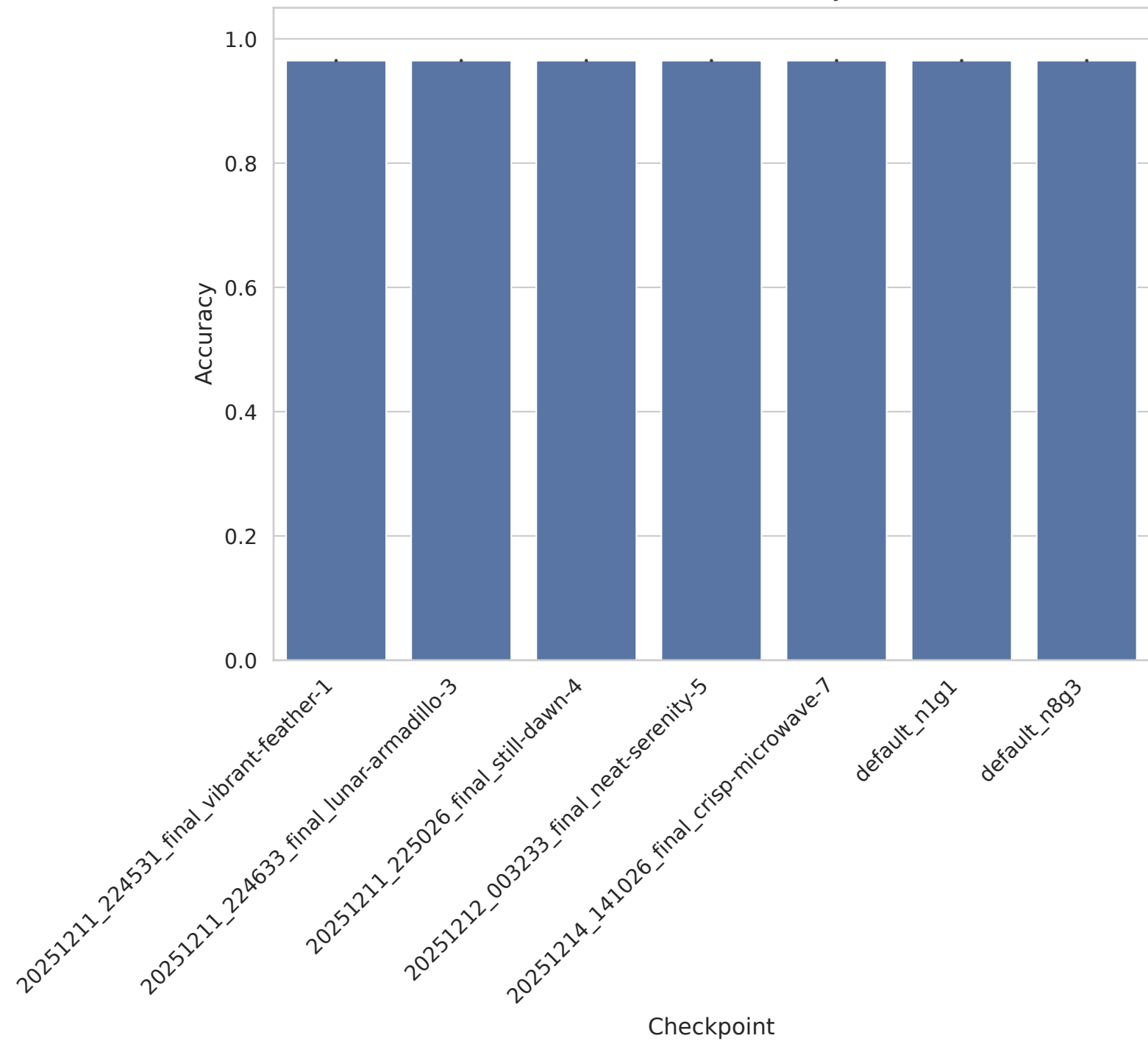
Task 363677 - Accuracy
