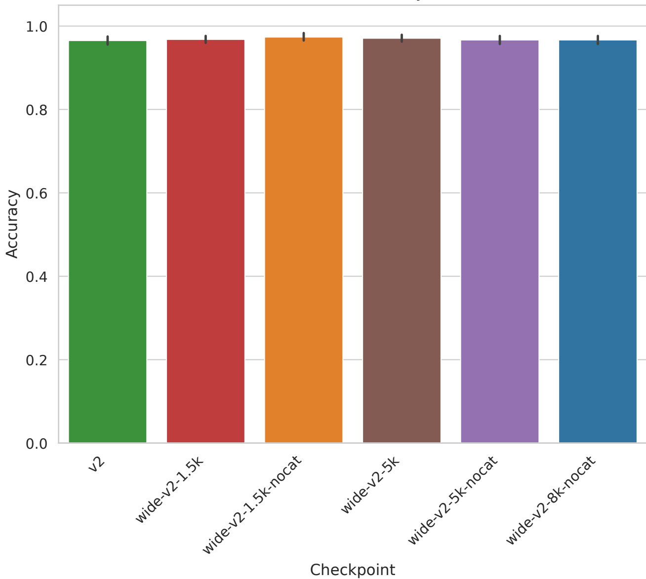
ALLAML - Accuracy
