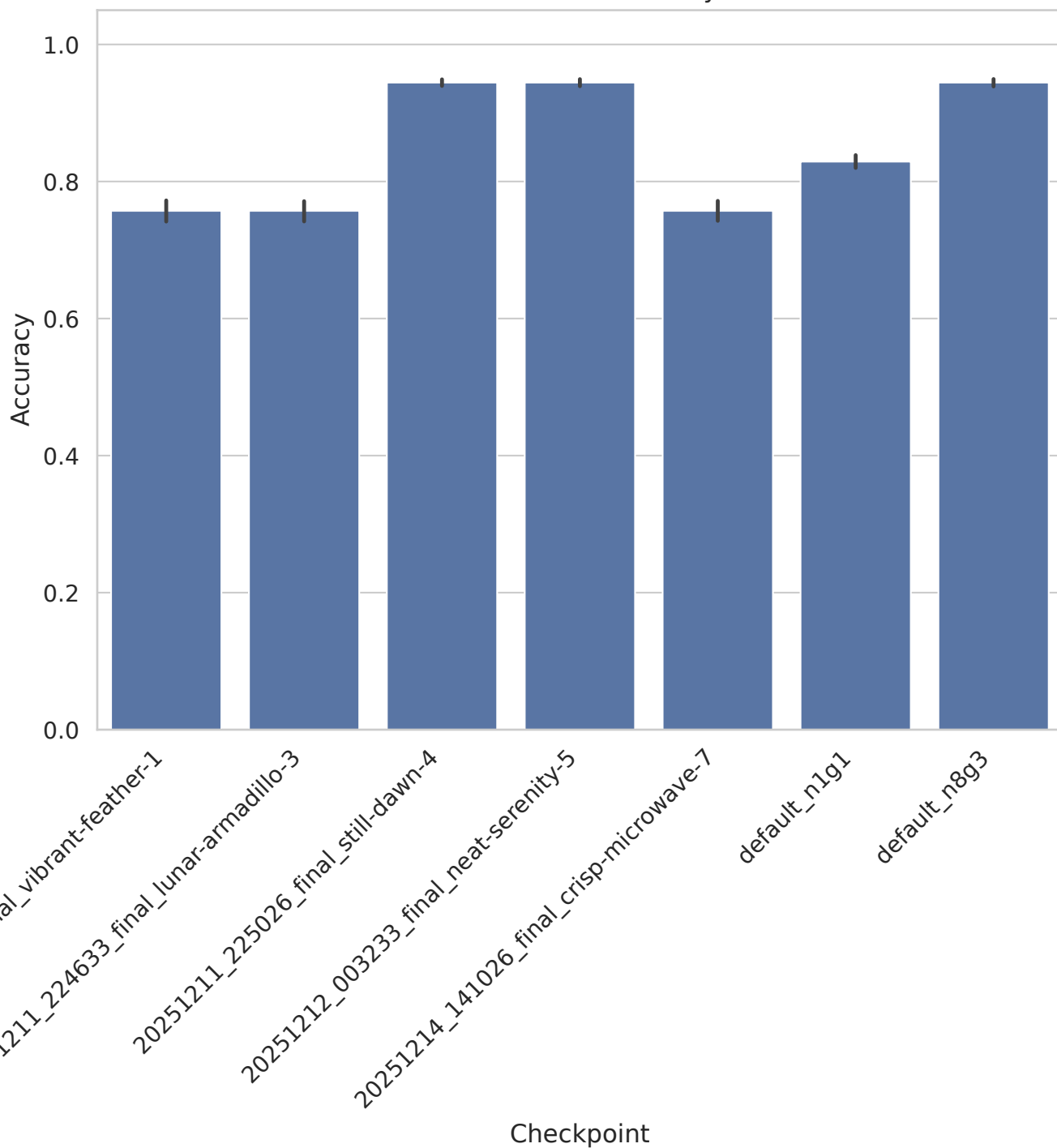
BASEHOCK - Accuracy
