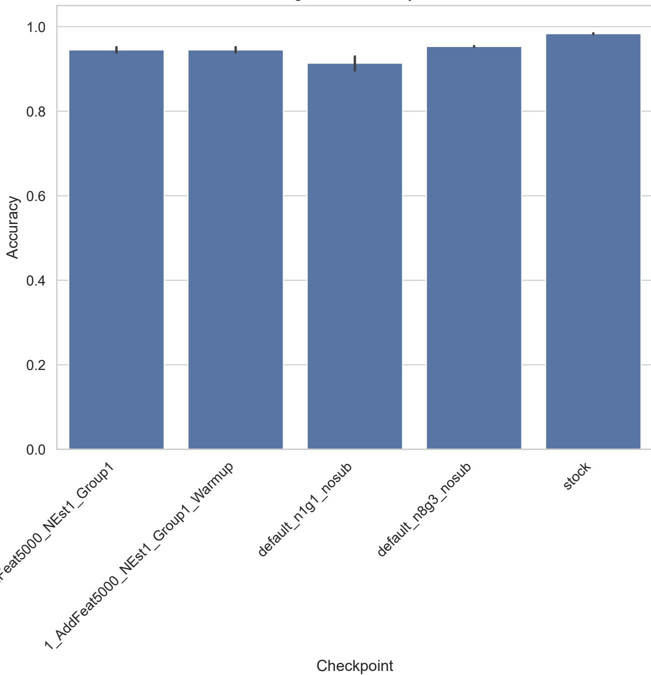
gisette - Accuracy
