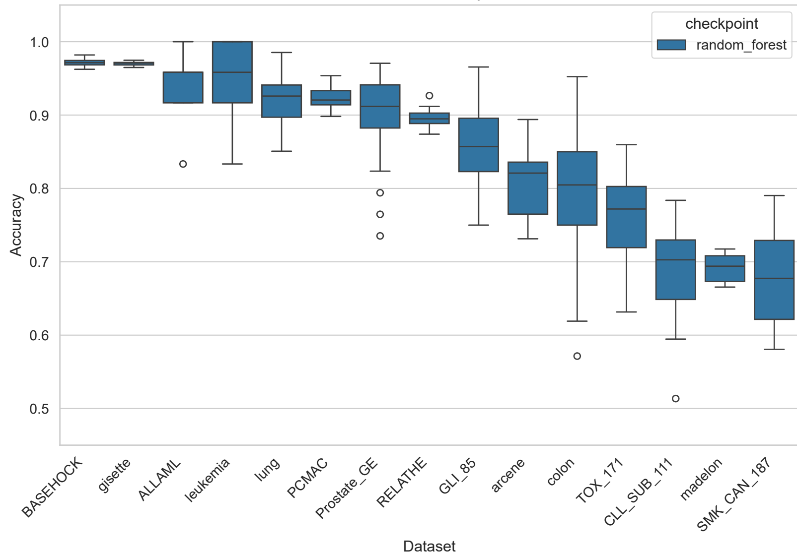
hdls - accuracy
