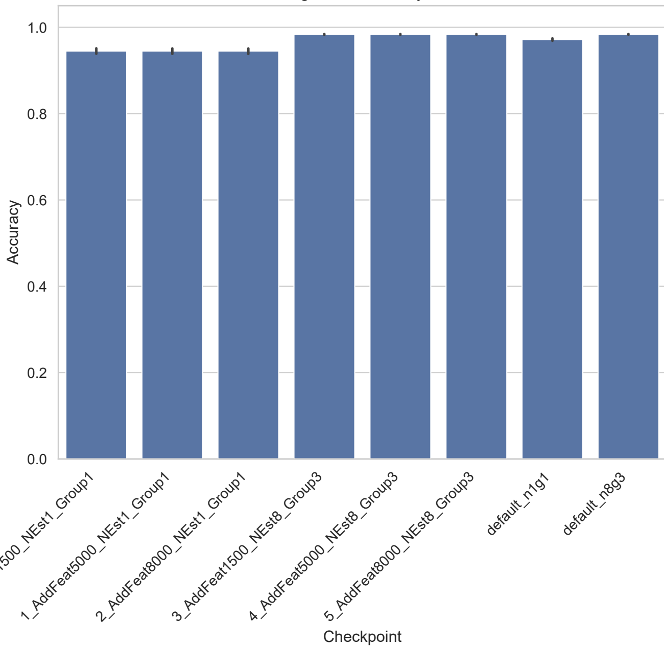
gisette - Accuracy
