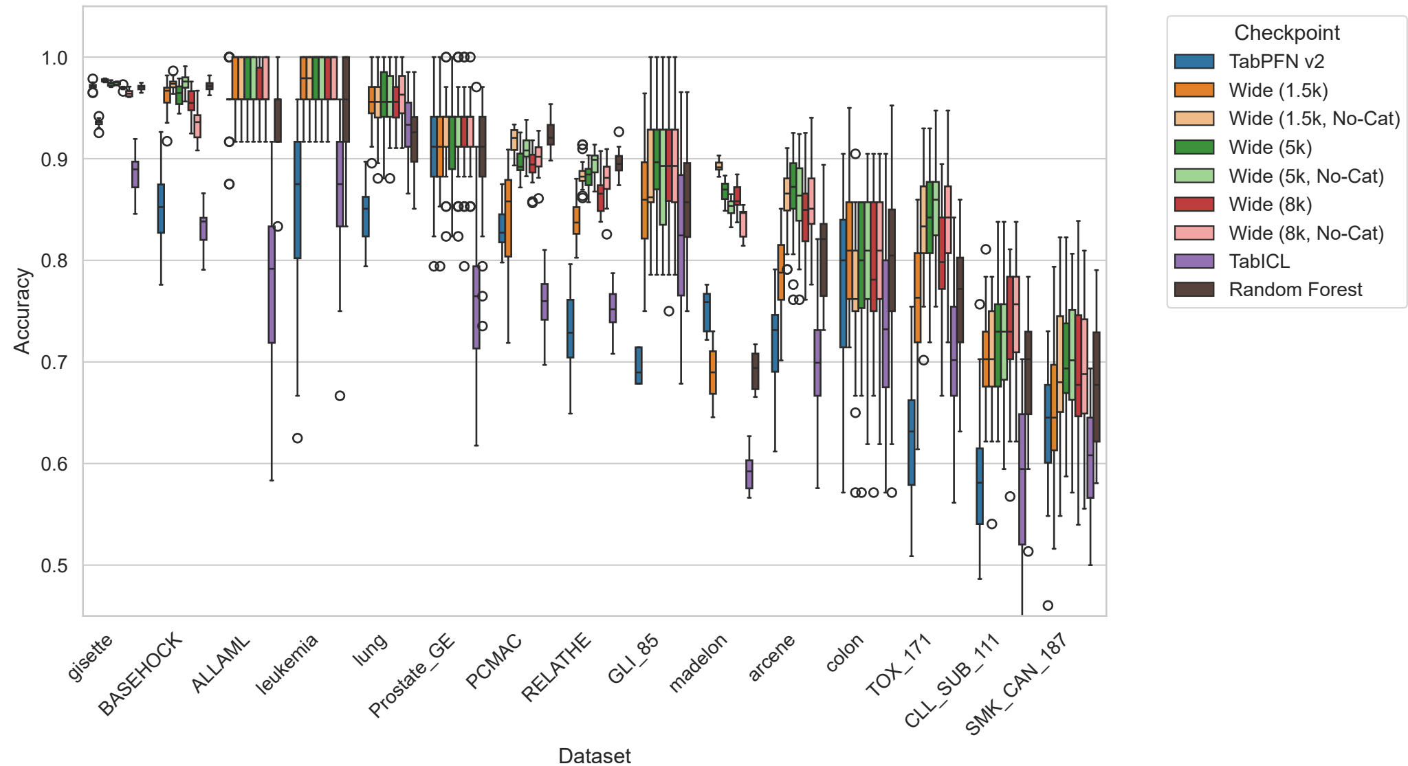
hdls - accuracy
