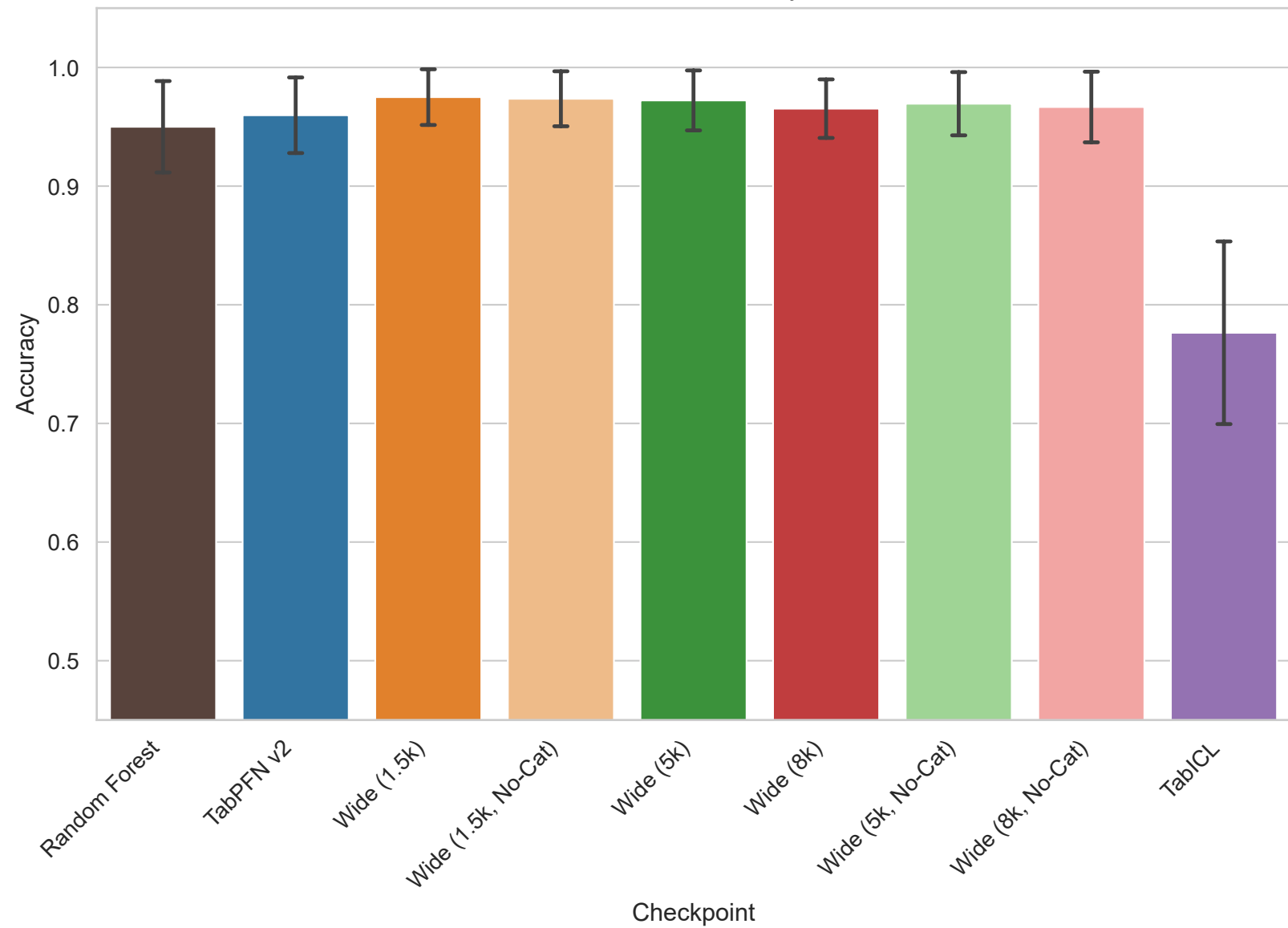
ALLAML - Accuracy
