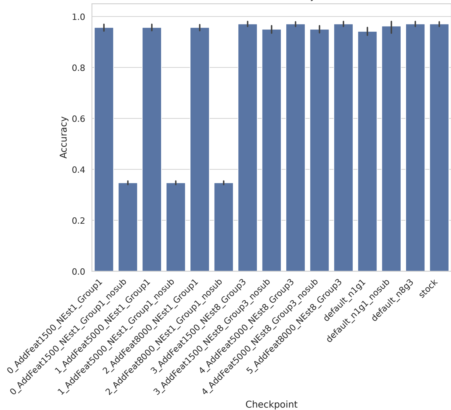
ALLAML - Accuracy
