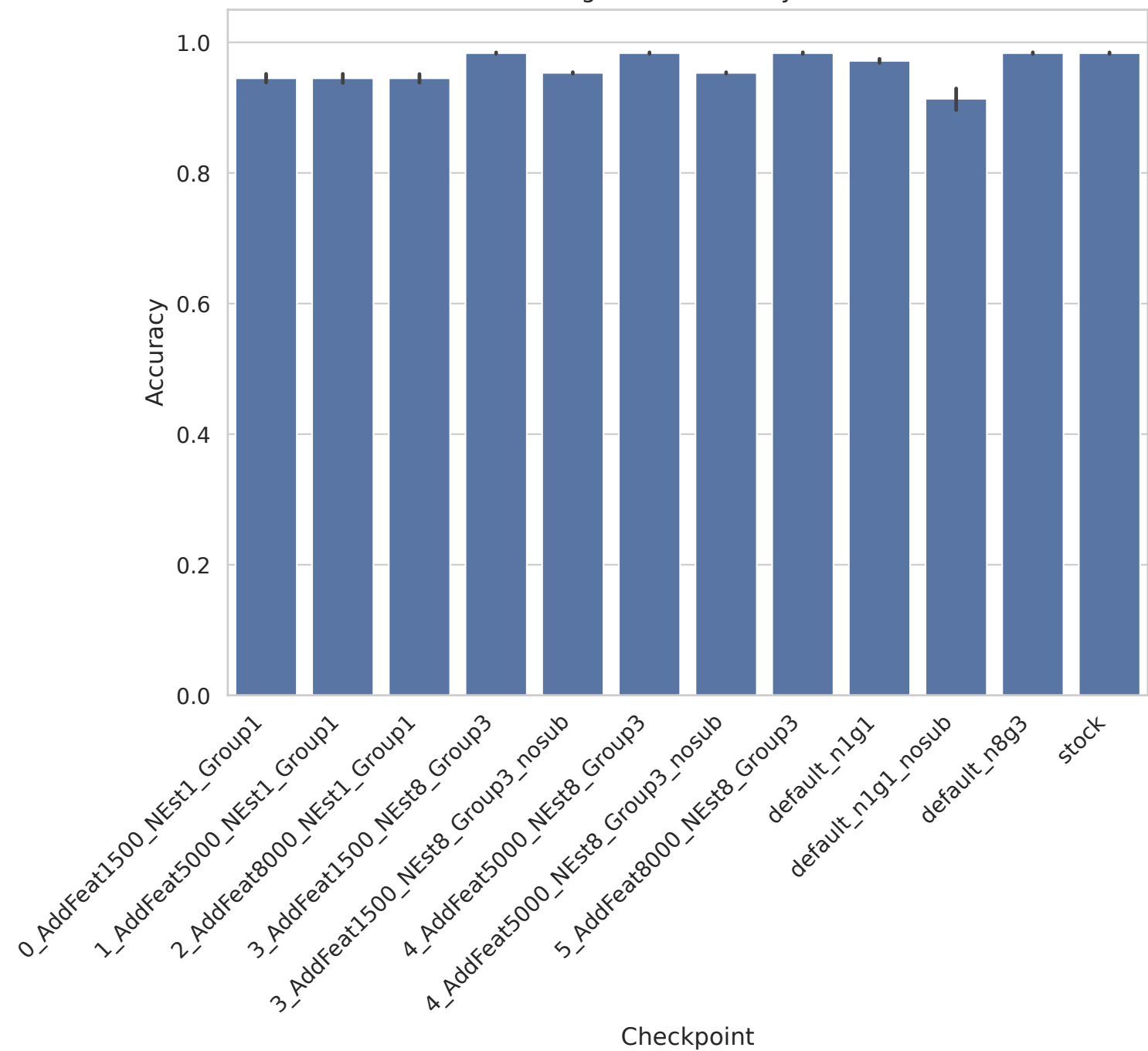
gisette - Accuracy
