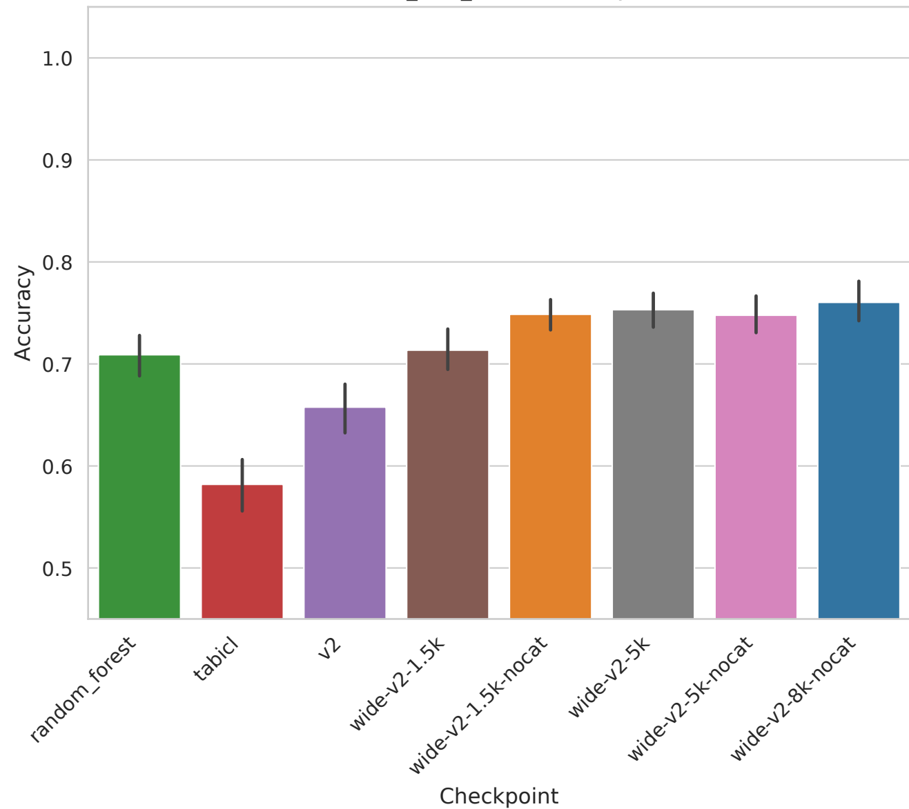
CLL_SUB_111 - Accuracy
