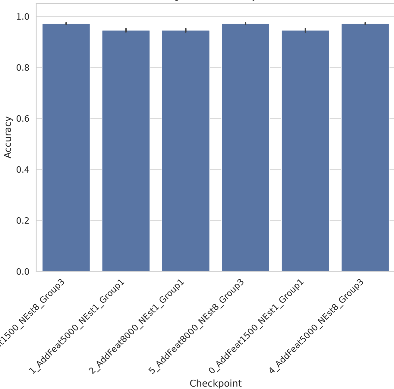
gisette - Accuracy
