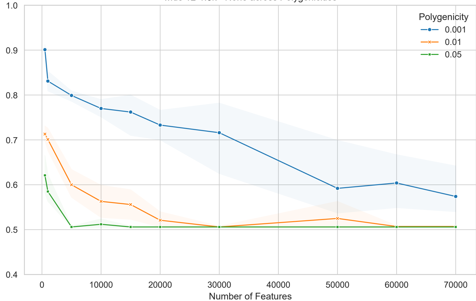
wide-v2-1.5k - None across Polygenicities
