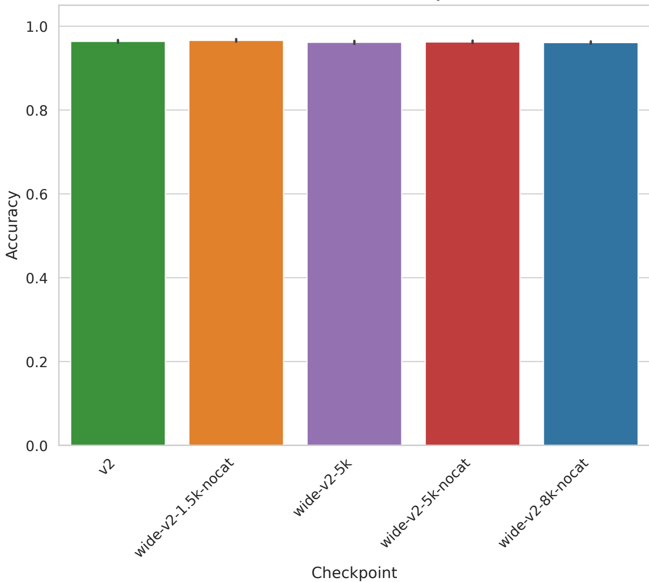
Task 363702 - Accuracy
