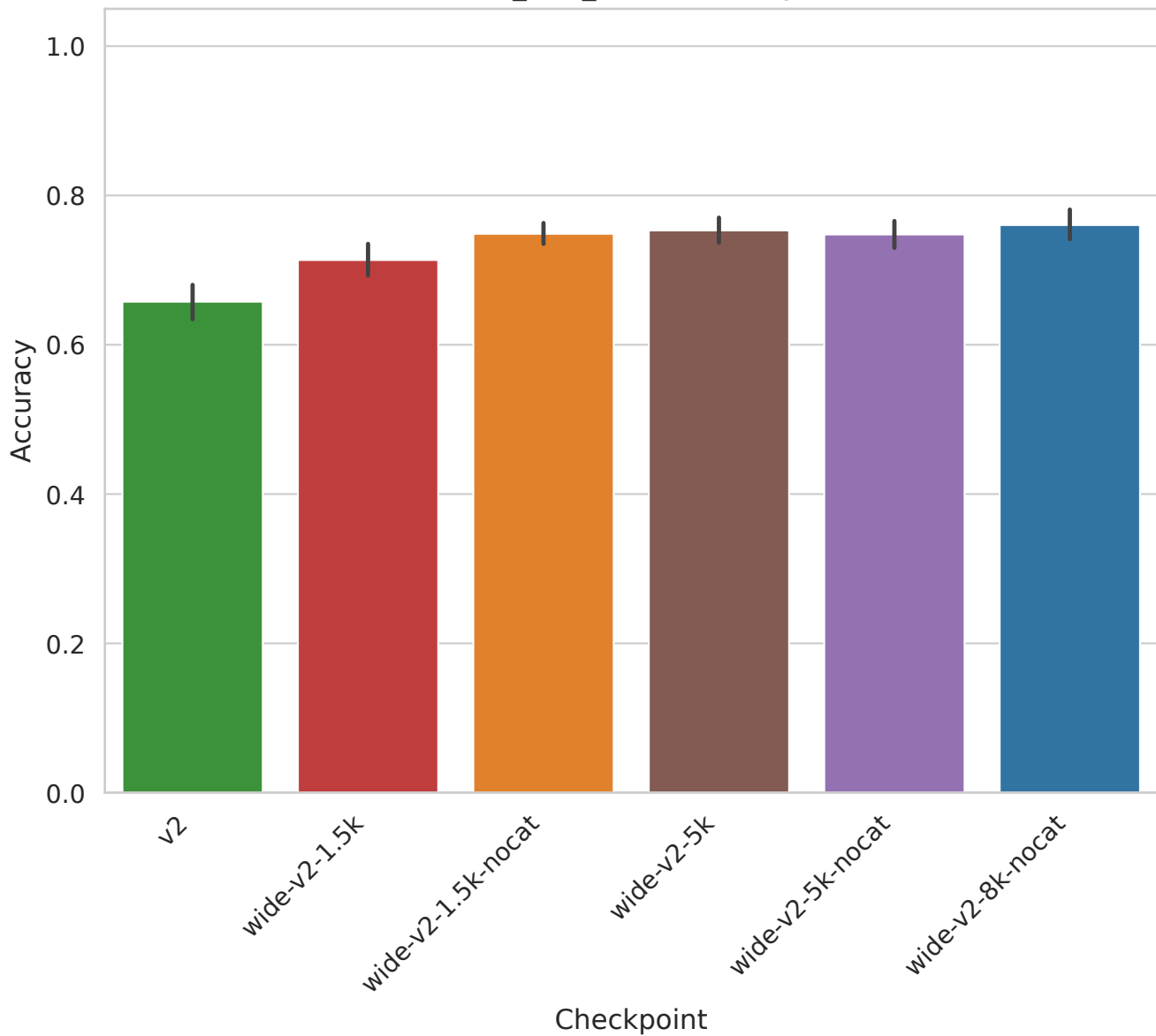
CLL_SUB_111 - Accuracy
