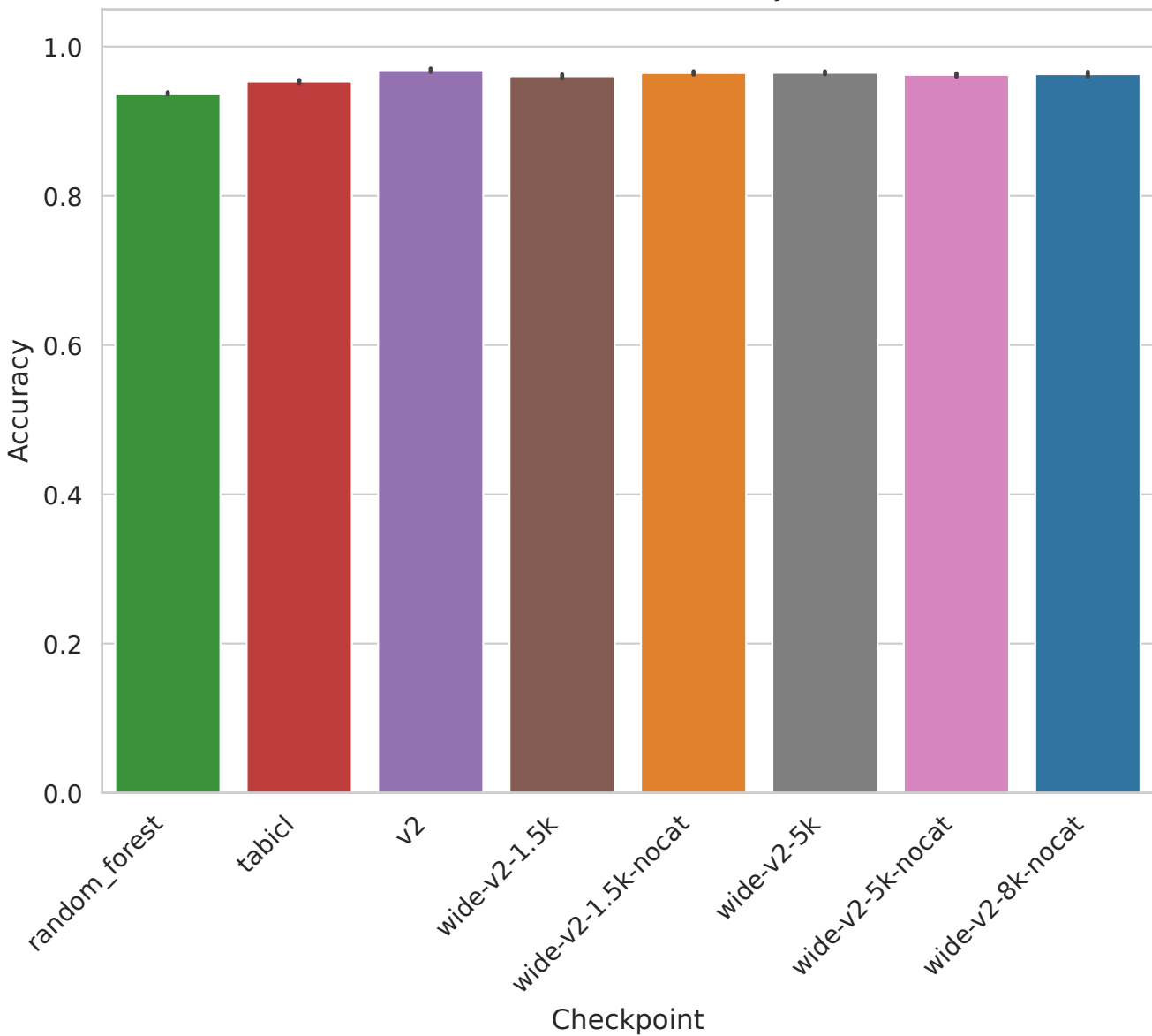
Task 363694 - Accuracy
