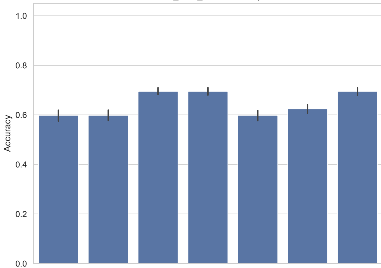
SMK_CAN_187 - Accuracy
