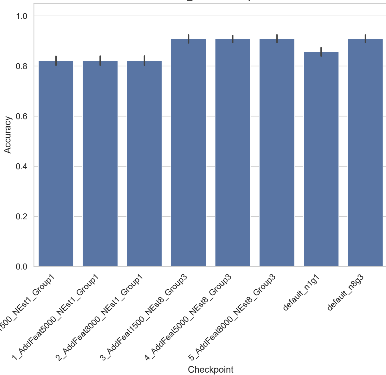
TOX_171 - Accuracy
