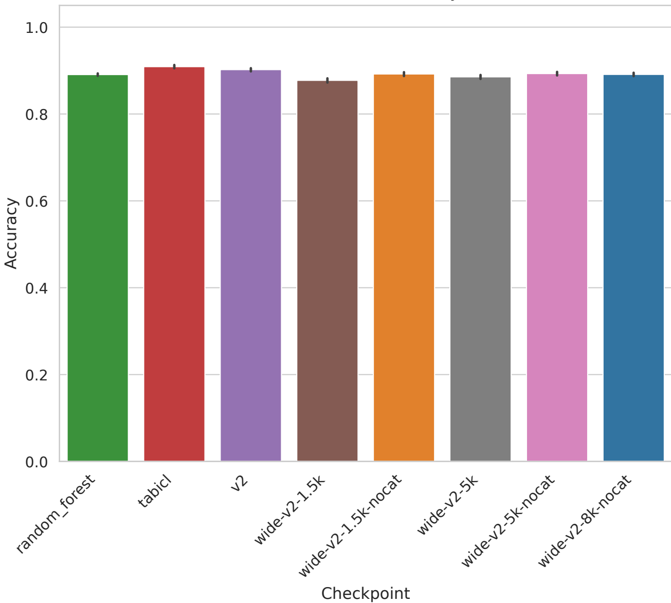
Task 363707 - Accuracy
