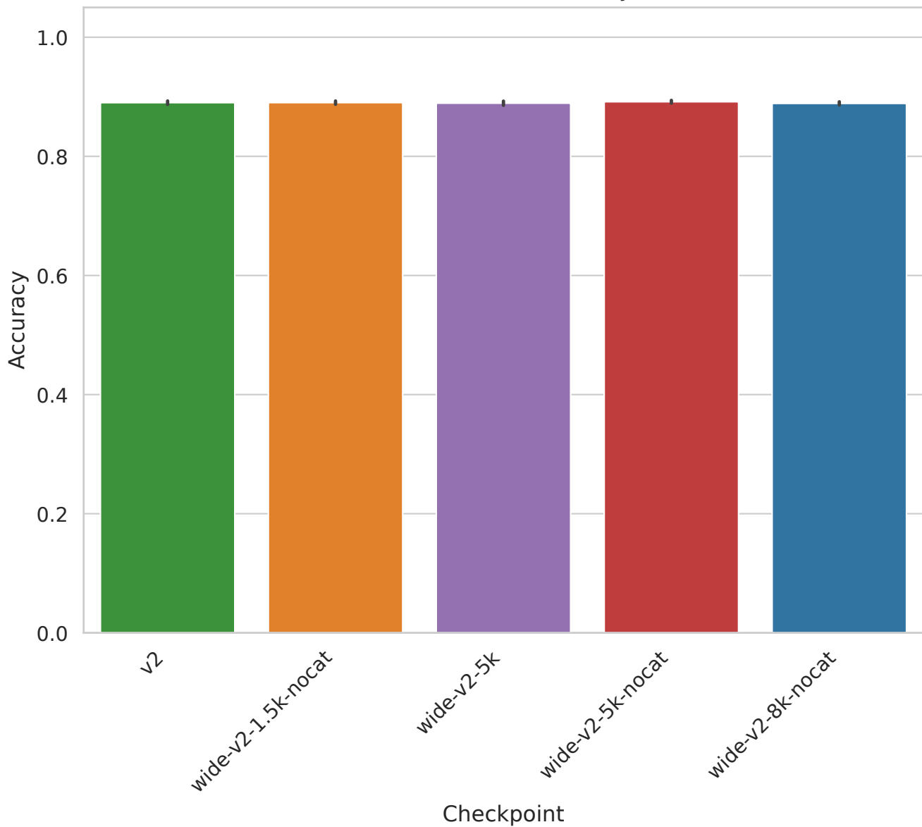
Task 363684 - Accuracy
