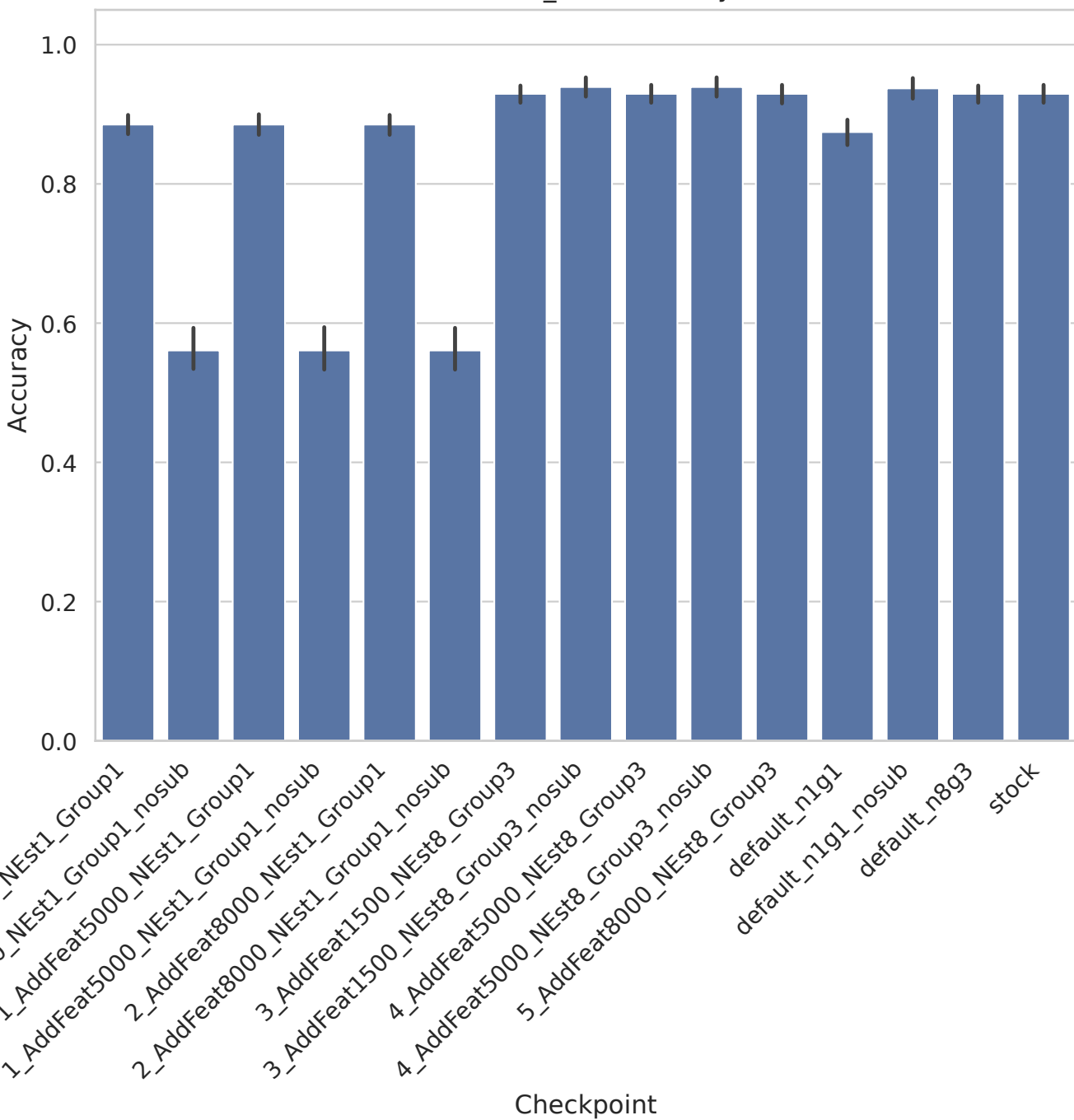
Prostate_GE - Accuracy
