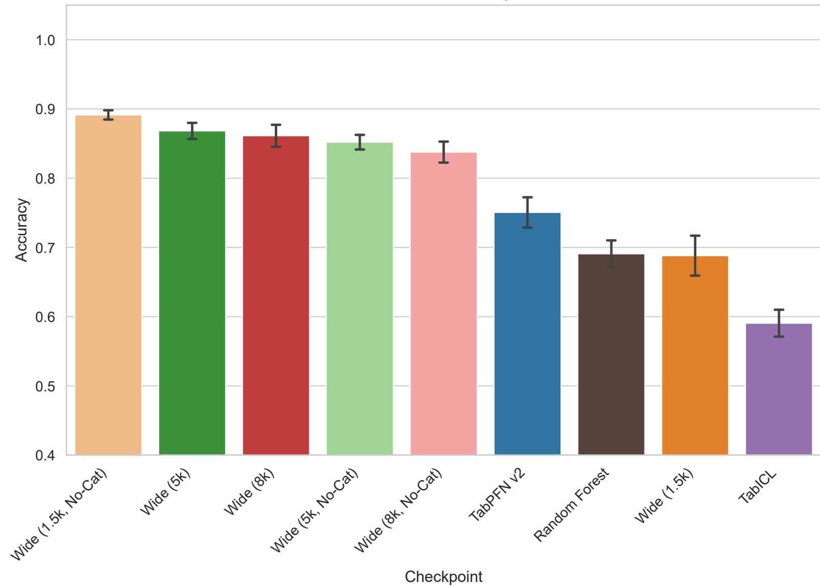
madelon - Accuracy
