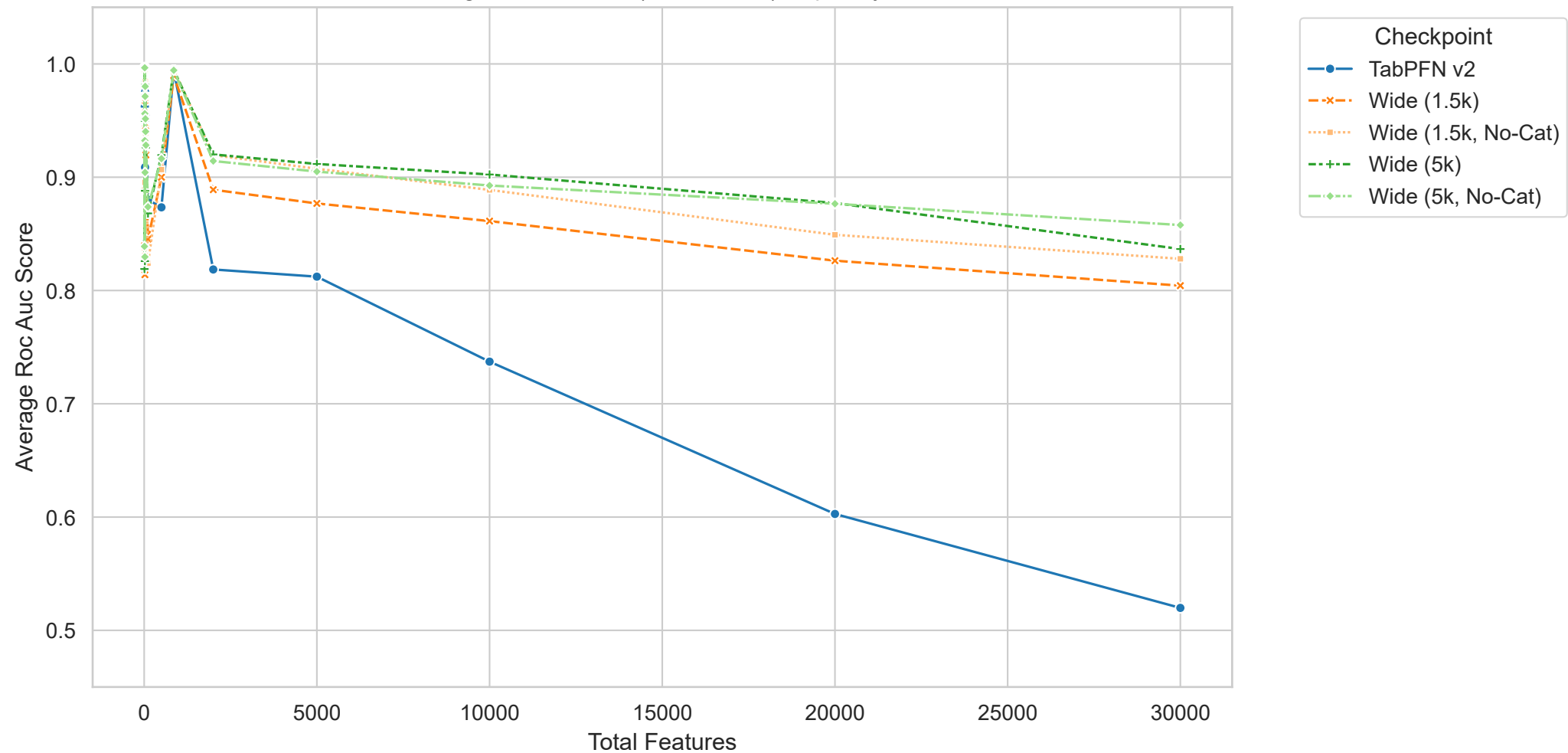
Average Performance (All Datasets) - Sparsity 0.0
