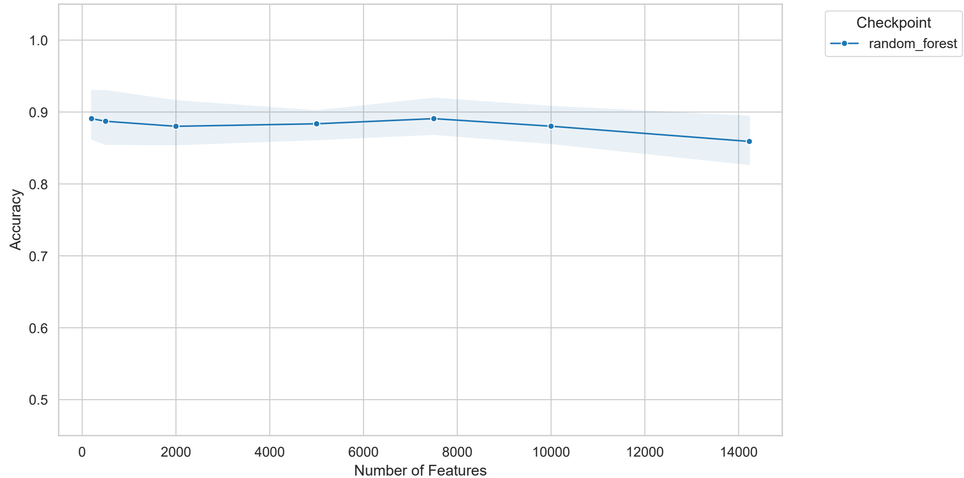
OV - Accuracy vs Feature Count
