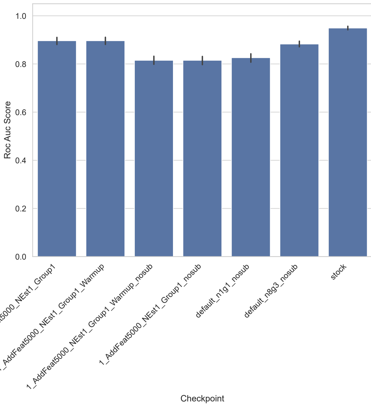
arcene - Roc Auc Score
