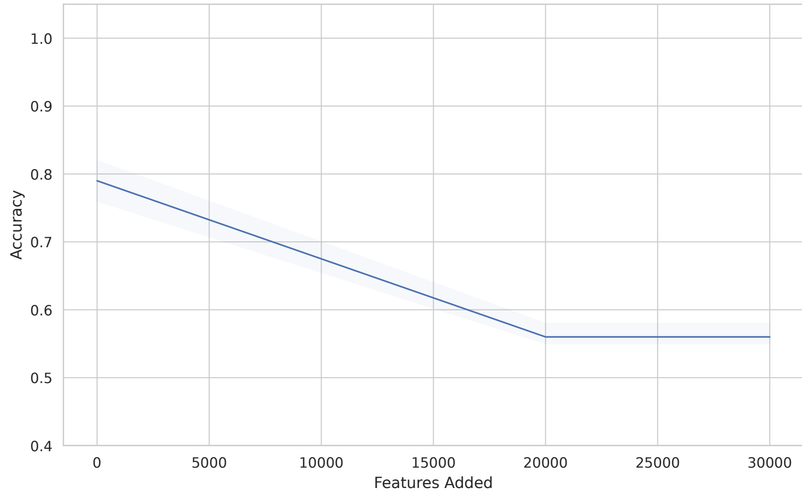
Dataset 41157 - accuracy vs Features Added
