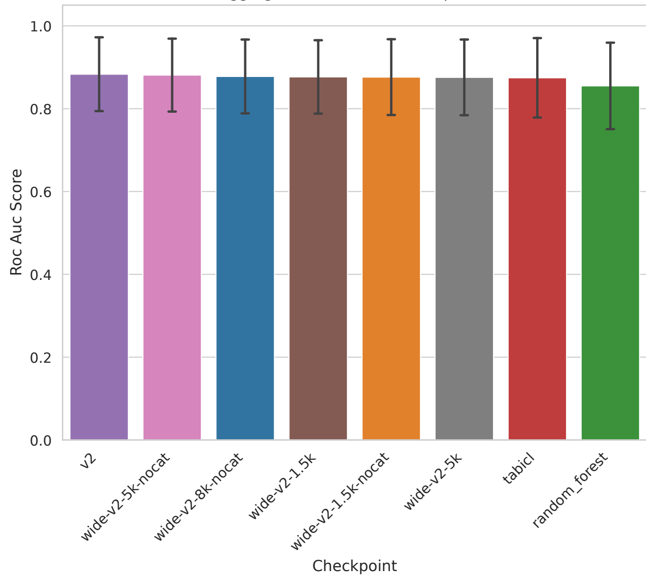
Aggregated Roc Auc Score - openml
