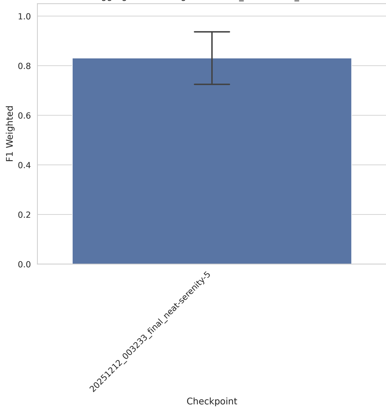
Aggregated F1 Weighted - hdls_benchmark_results
