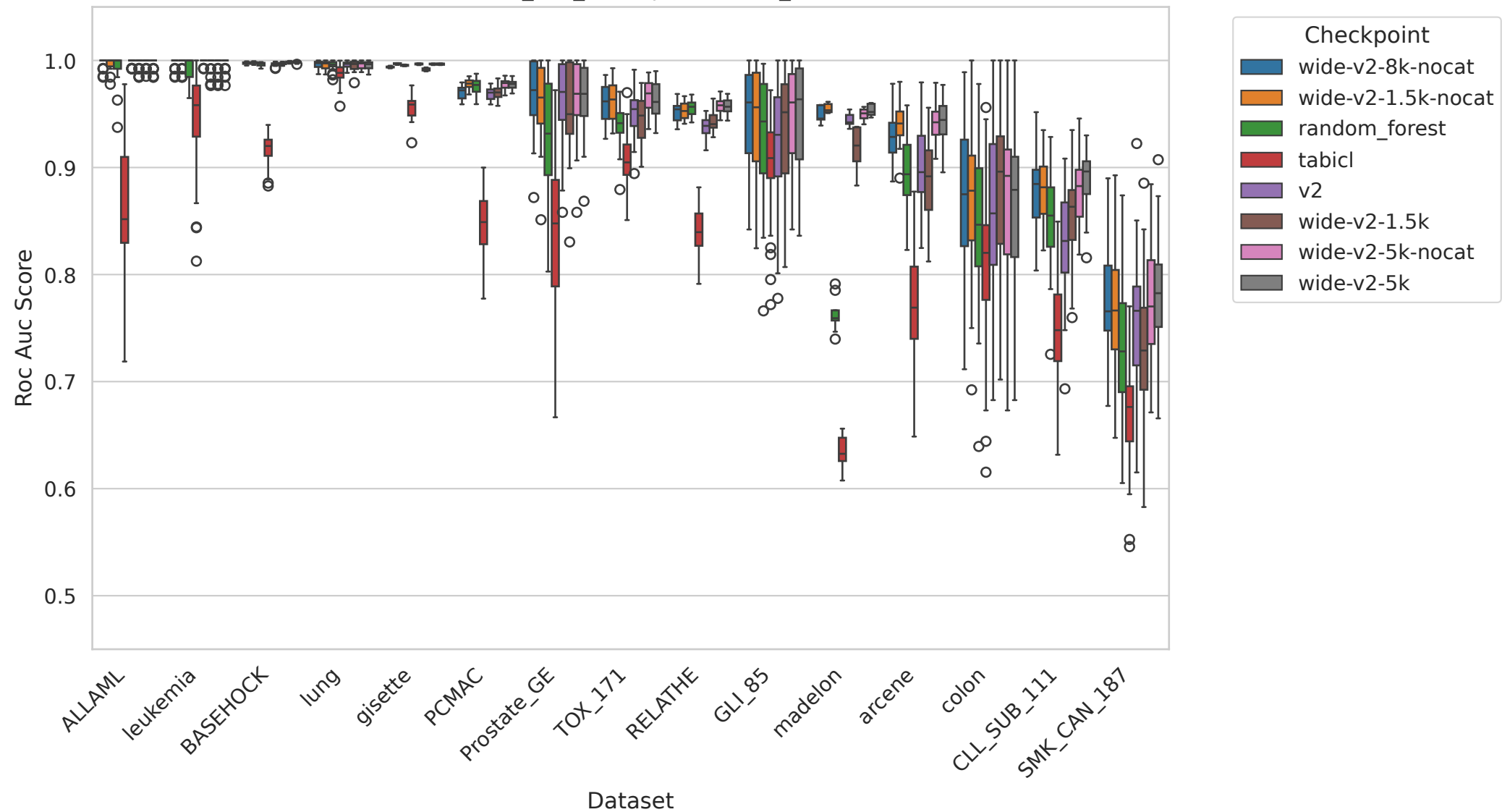
hdlss - roc_auc_score per dataset_name
