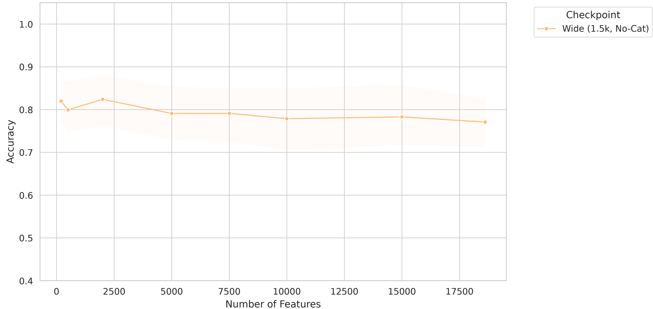
GBM - Accuracy vs Feature Count
