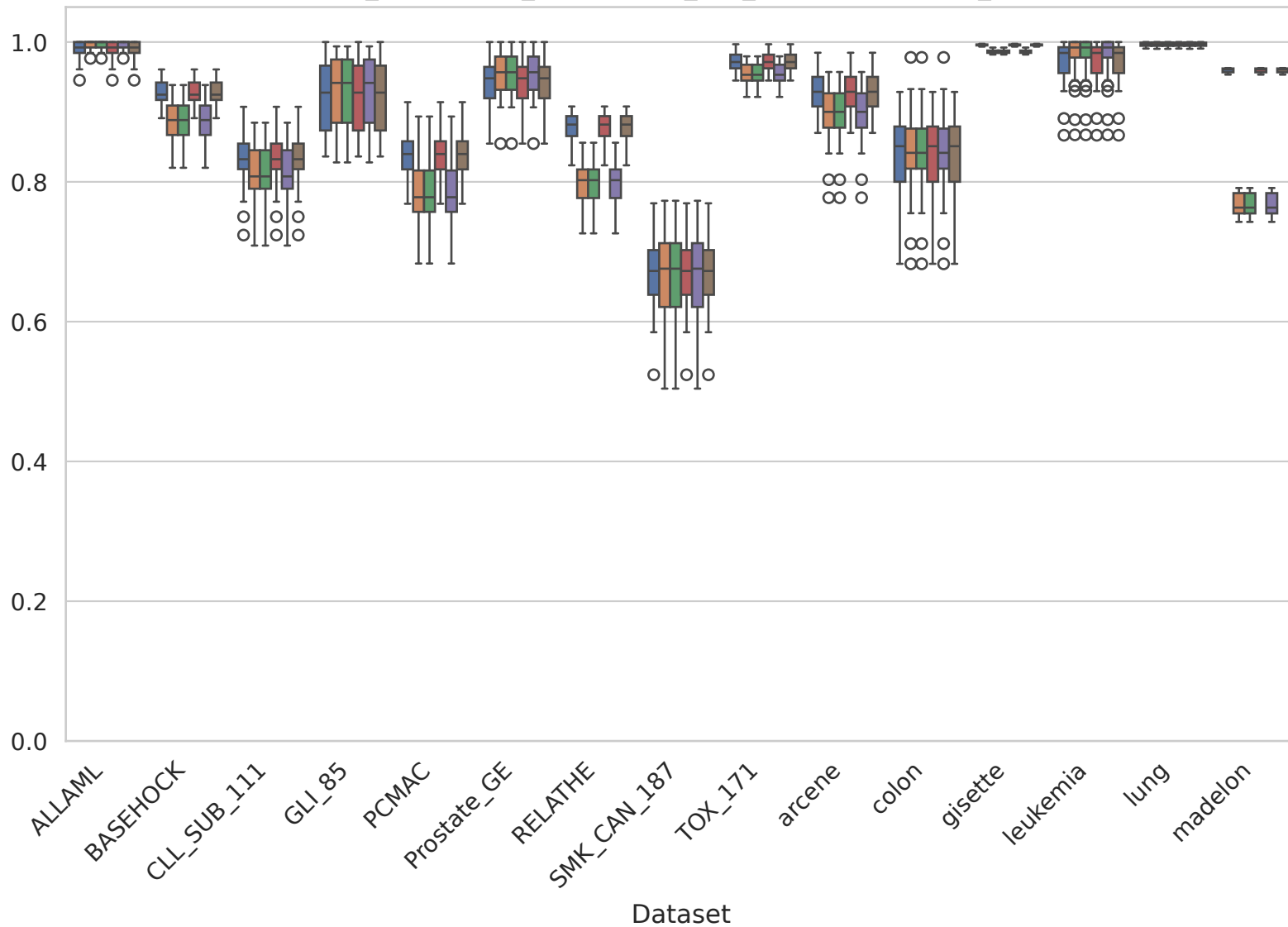
hdlss_benchmark_results - roc_auc_score per dataset_name
