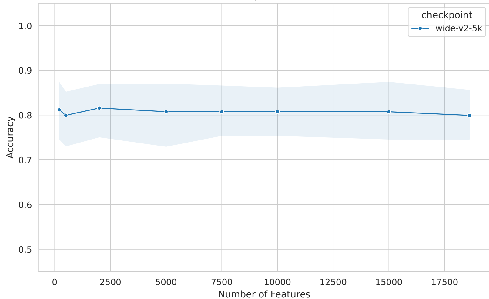
GBM - Accuracy vs Feature Count
