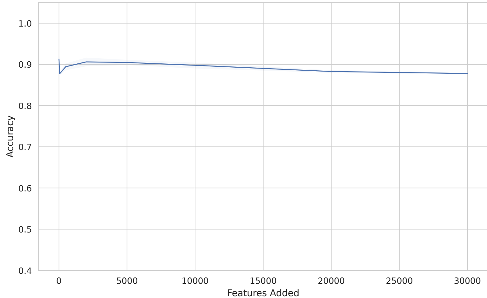
Dataset 1049 - accuracy vs Features Added
