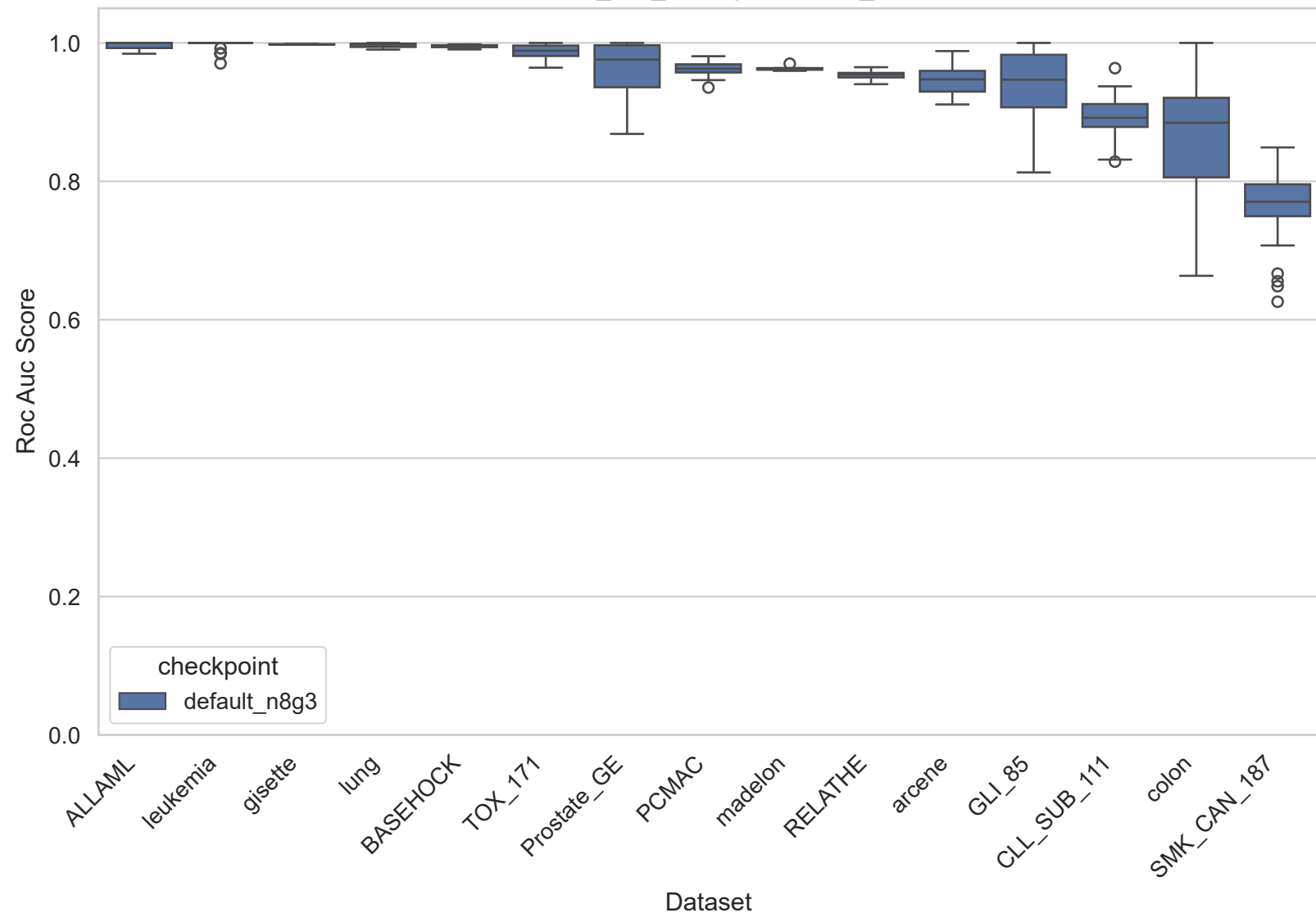
hdlss - roc_auc_score per dataset_name
