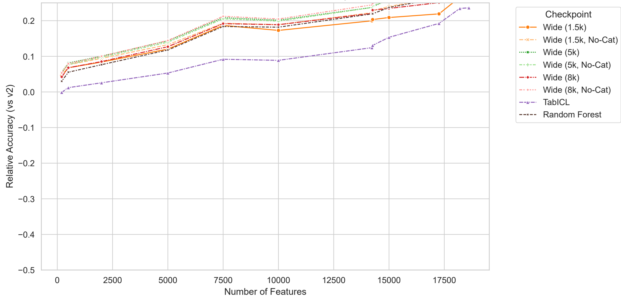
Multiomics Overview - Relative Accuracy
