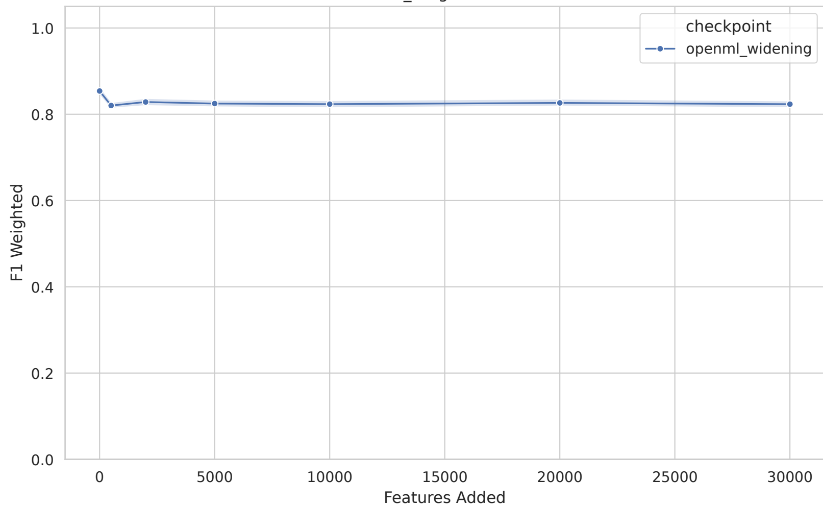
Dataset 40536 - f1_weighted vs Features Added
