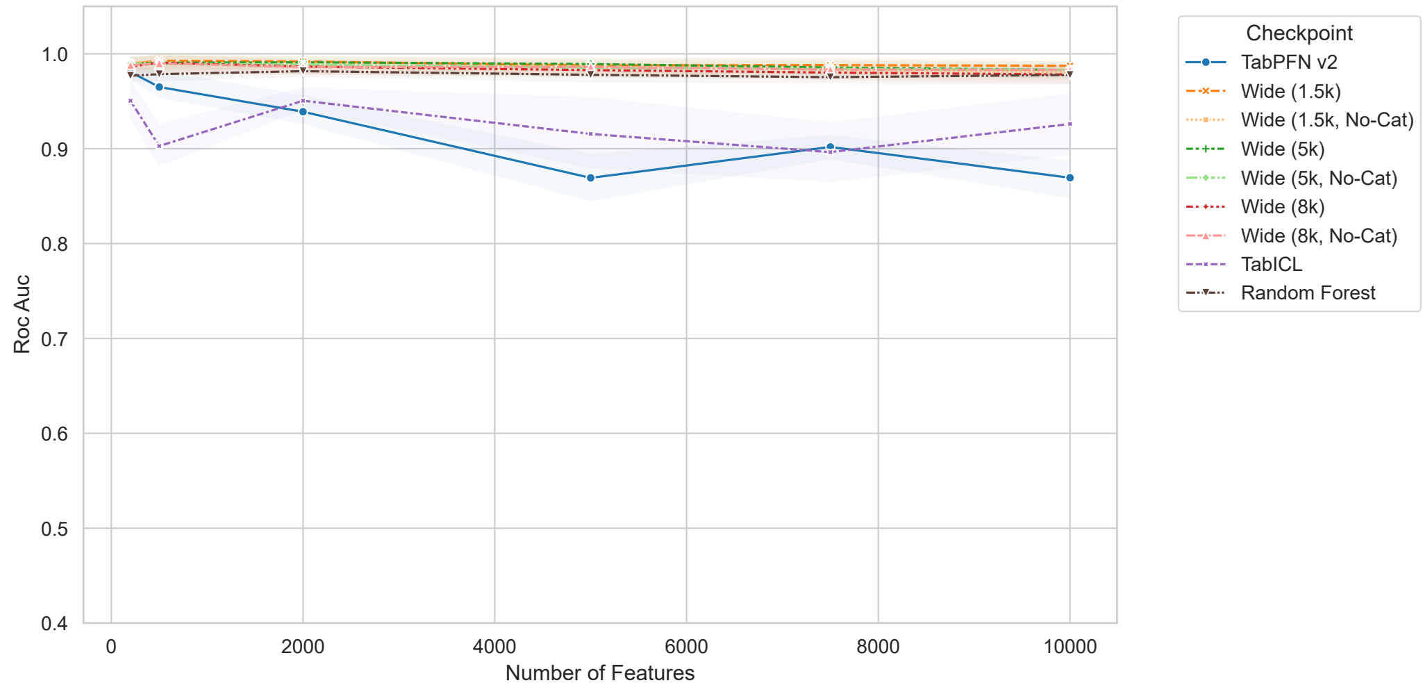
OV - Roc Auc vs Feature Count
