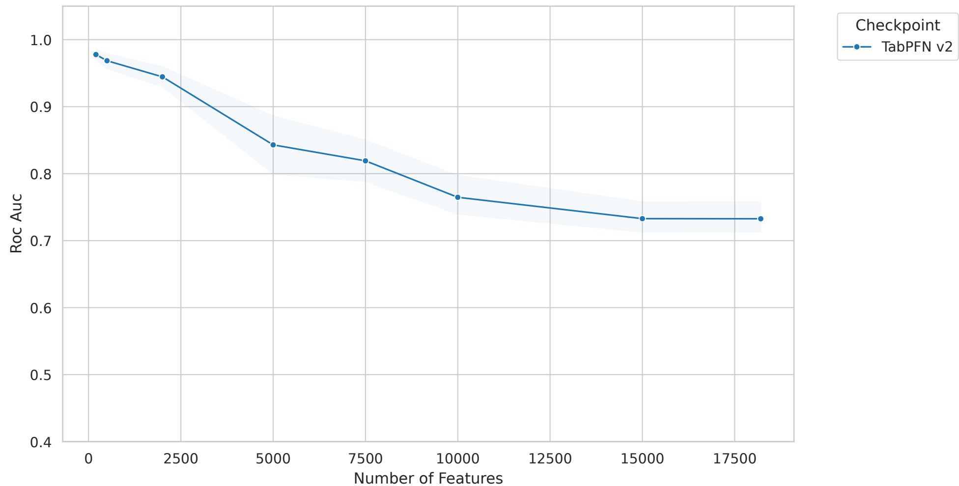
BRCA - Roc Auc vs Feature Count
