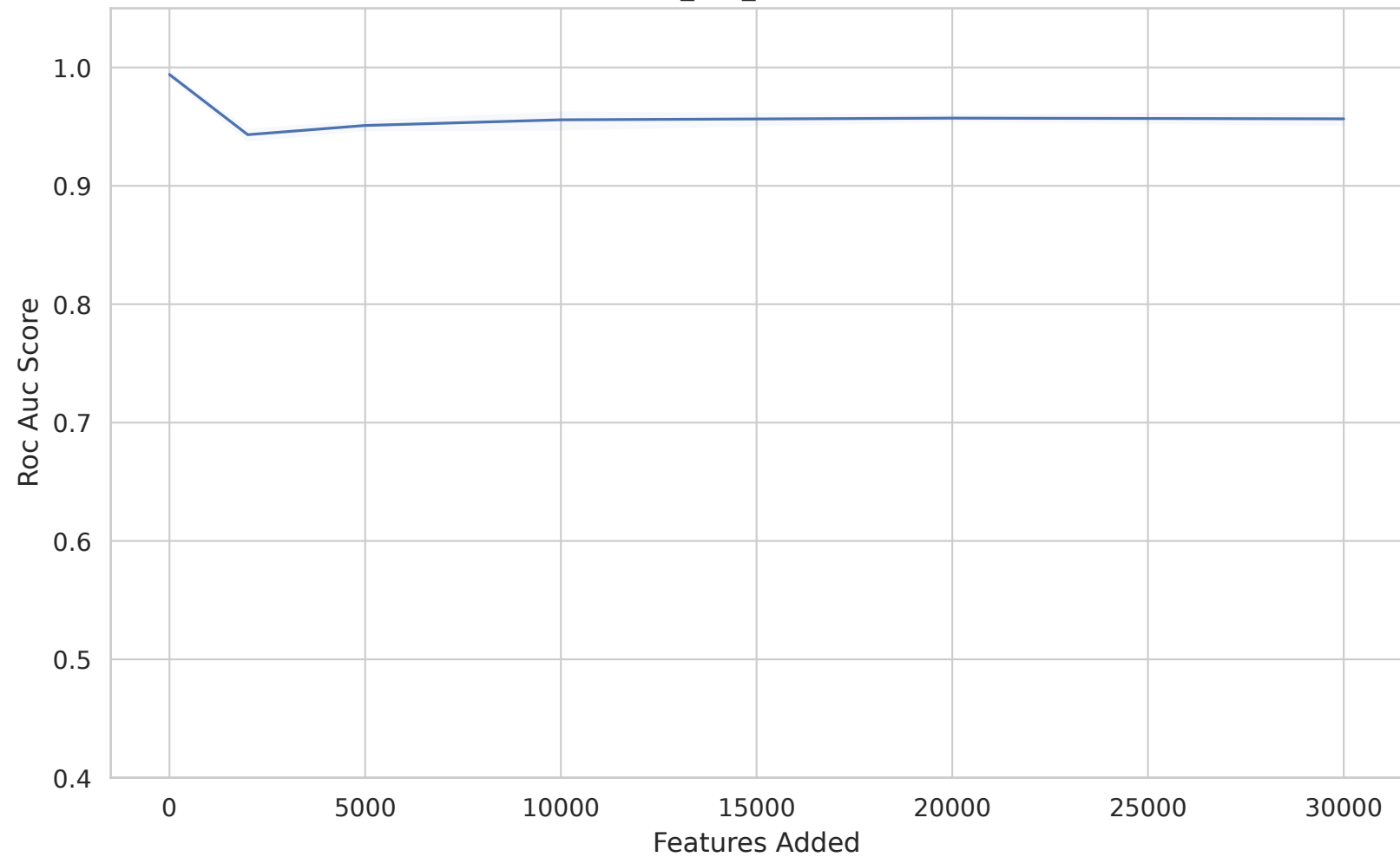
Dataset 1468 - roc_auc_score vs Features Added
