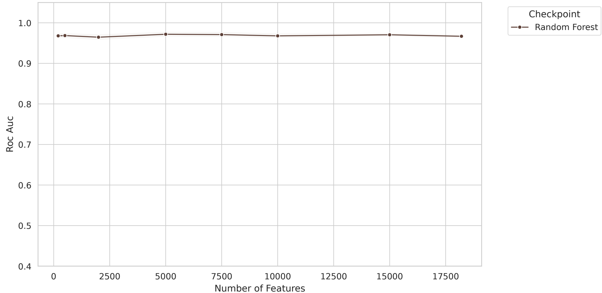
BRCA - Roc Auc vs Feature Count
