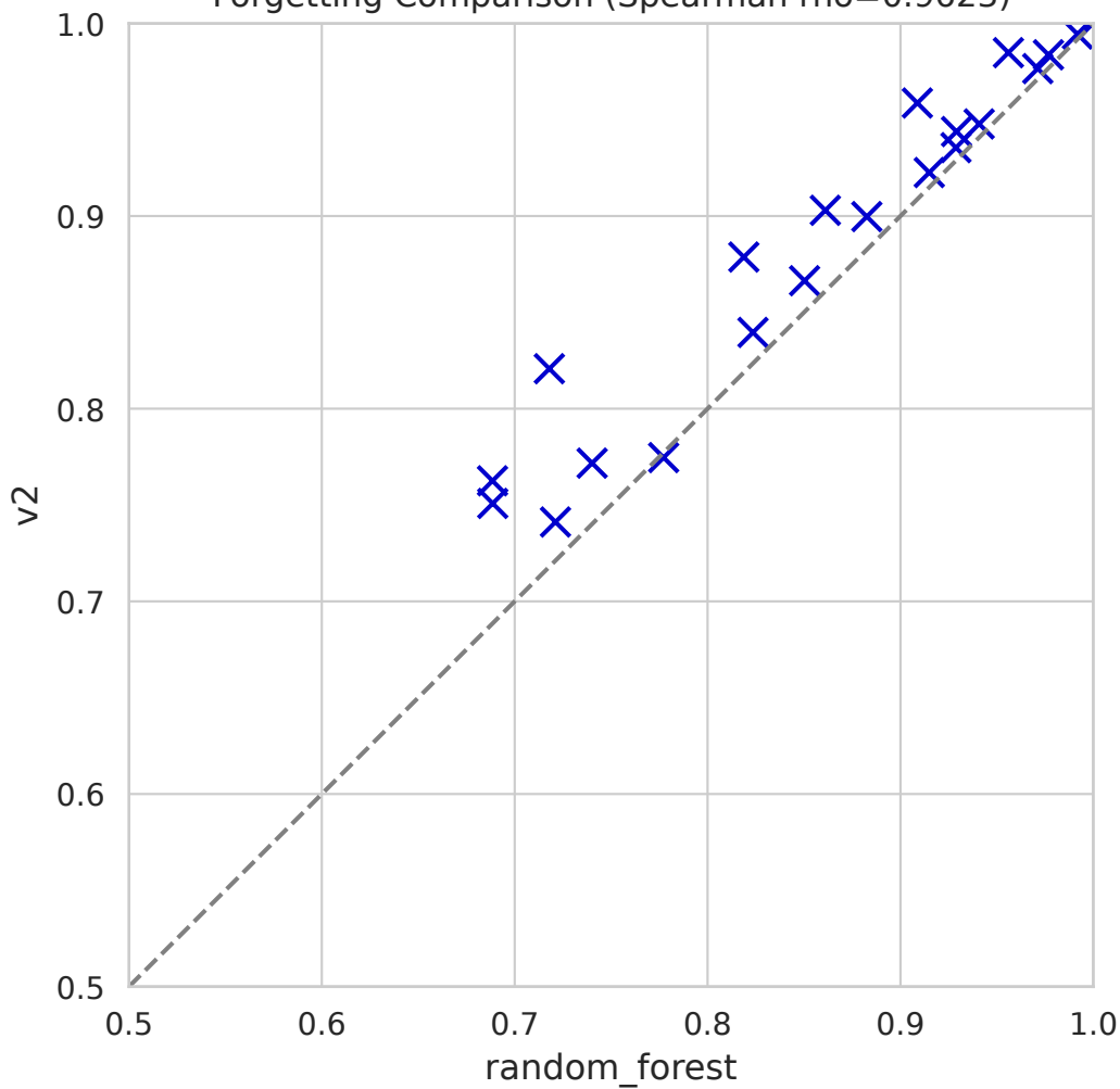
Forgetting Comparison (Spearman rho=0.9623)
