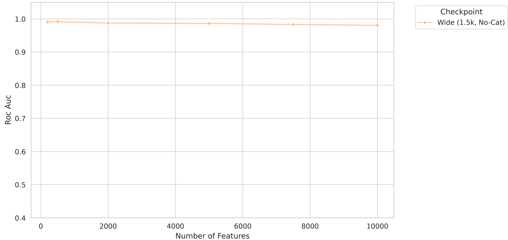
OV - Roc Auc vs Feature Count
