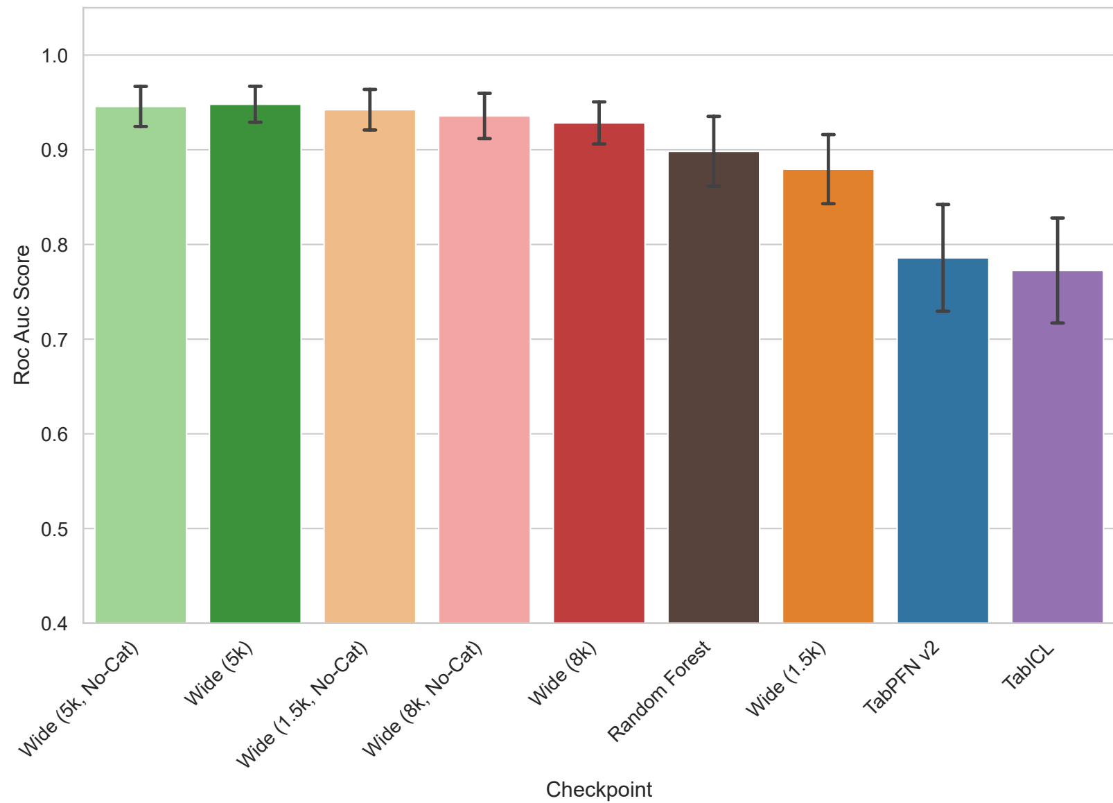
arcene - Roc Auc Score
