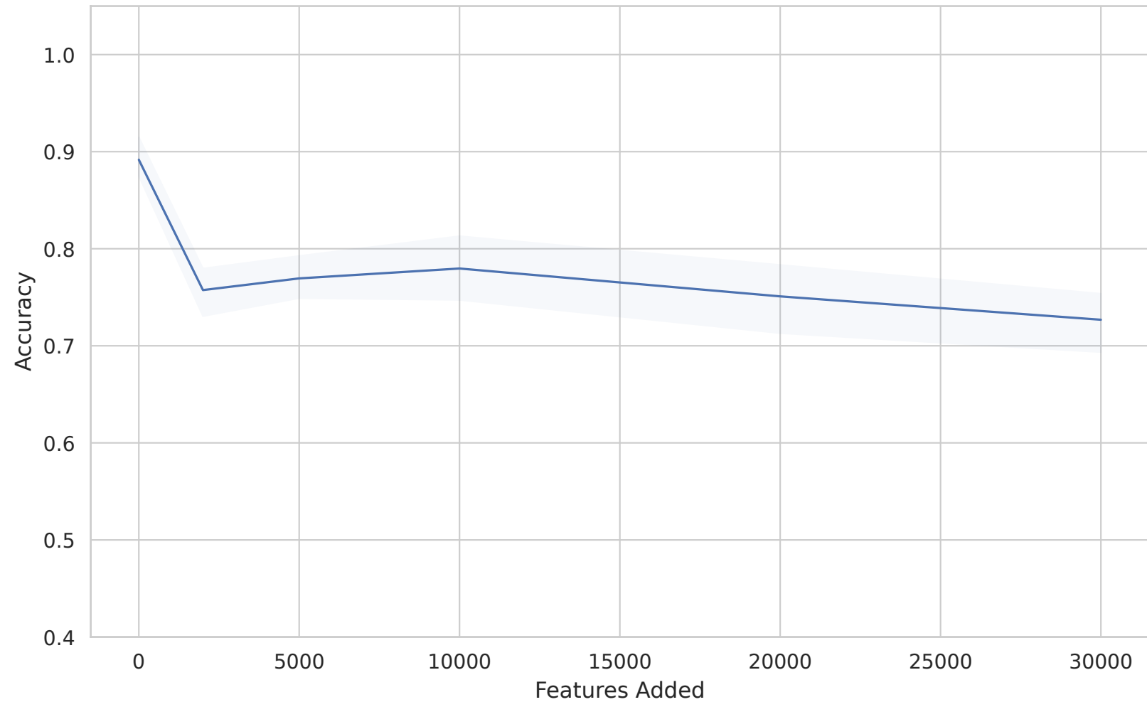
Dataset 1468 - accuracy vs Features Added
