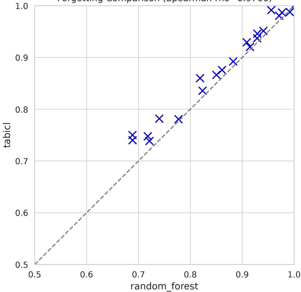
Forgetting Comparison (Spearman rho=0.9766)
