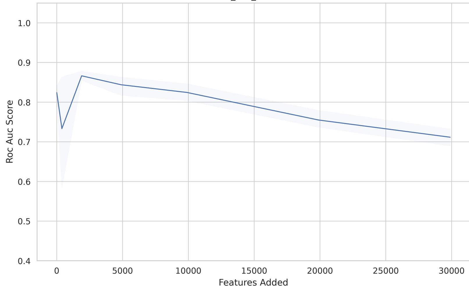
Dataset 46980 - roc_auc_score vs Features Added
