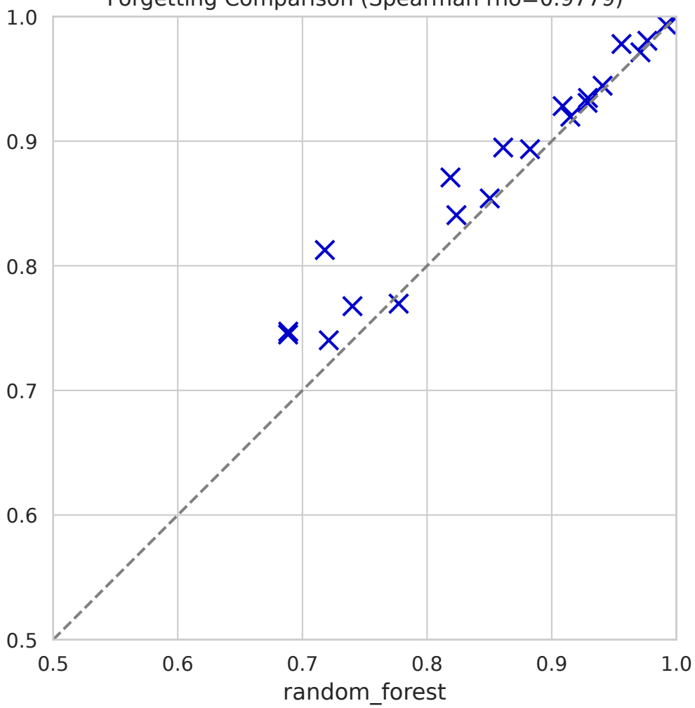
Forgetting Comparison (Spearman rho=0.9779)
