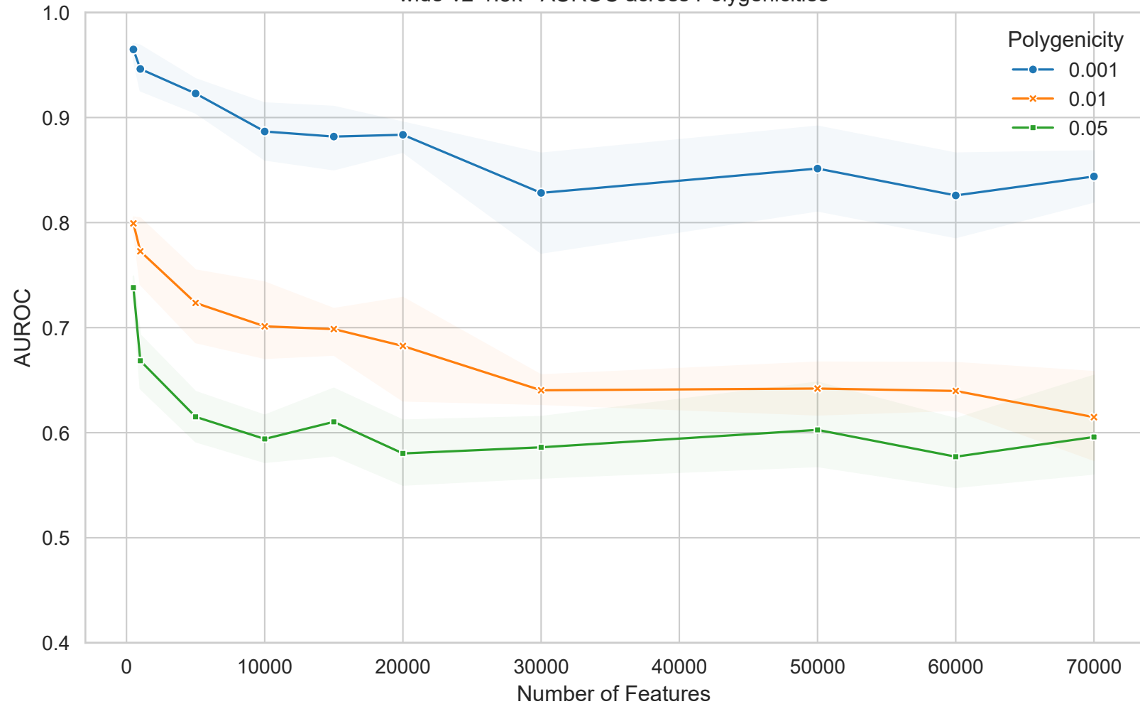
wide-v2-1.5k - AUROC across Polygenicities
