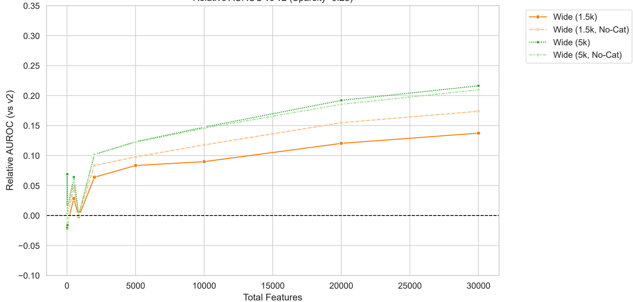
Relative AUROC vs v2 (Sparsity=0.25)
