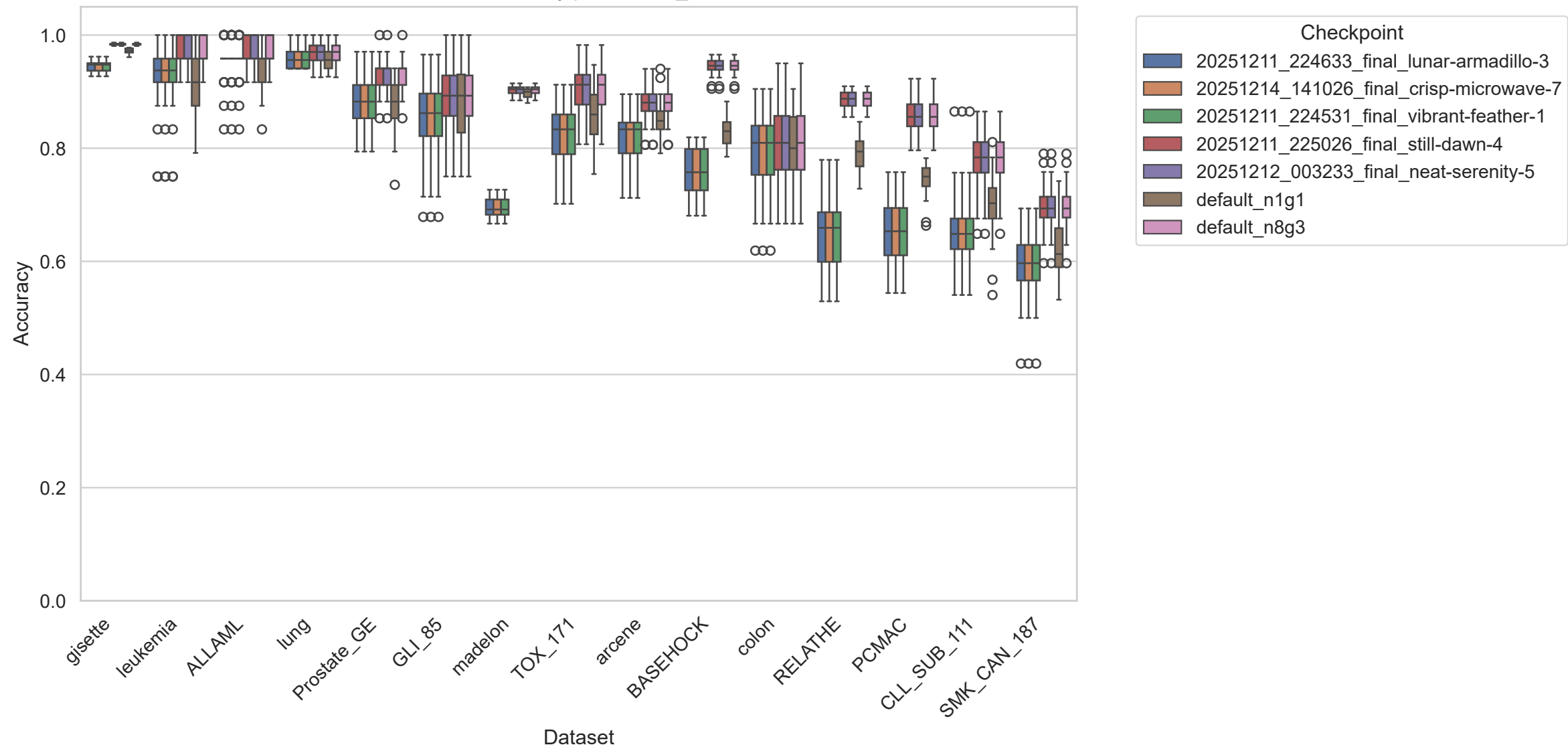
hdls - accuracy per dataset_name
