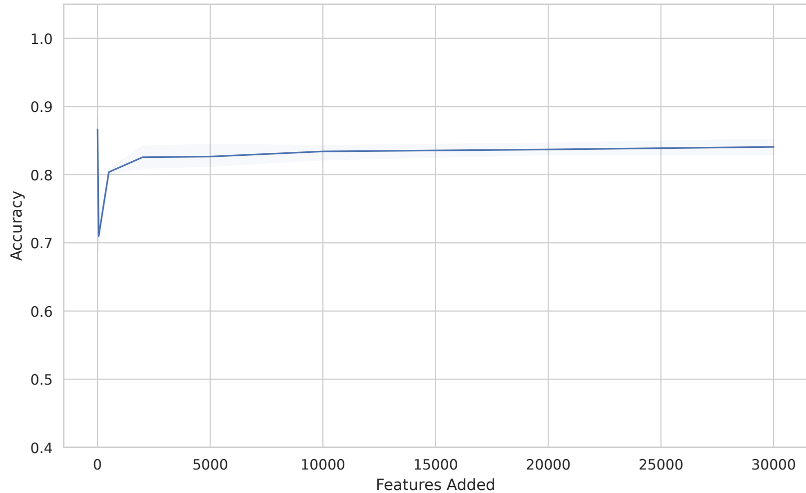
Dataset 1494 - accuracy vs Features Added
