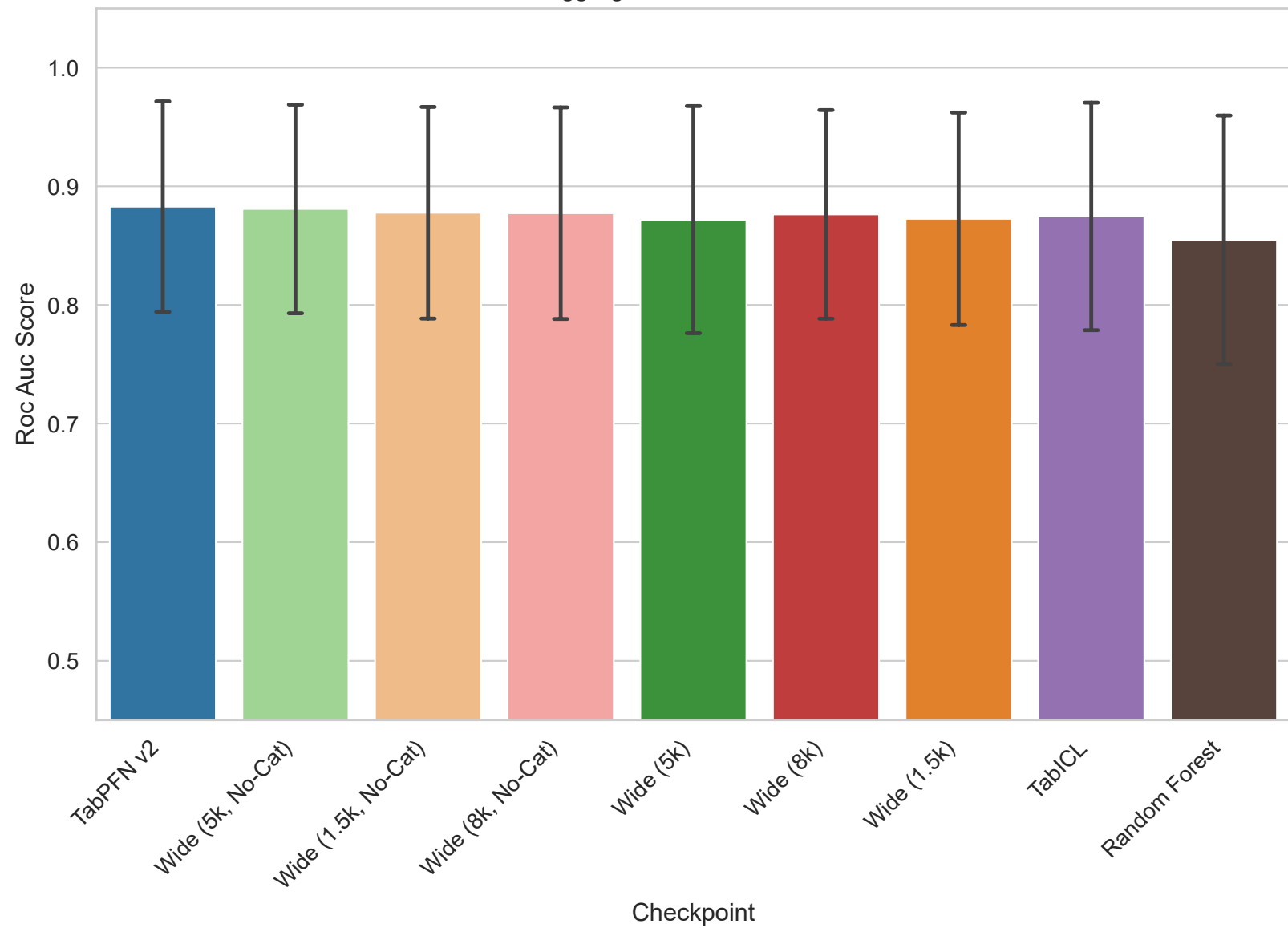
Aggregated Roc Auc Score
