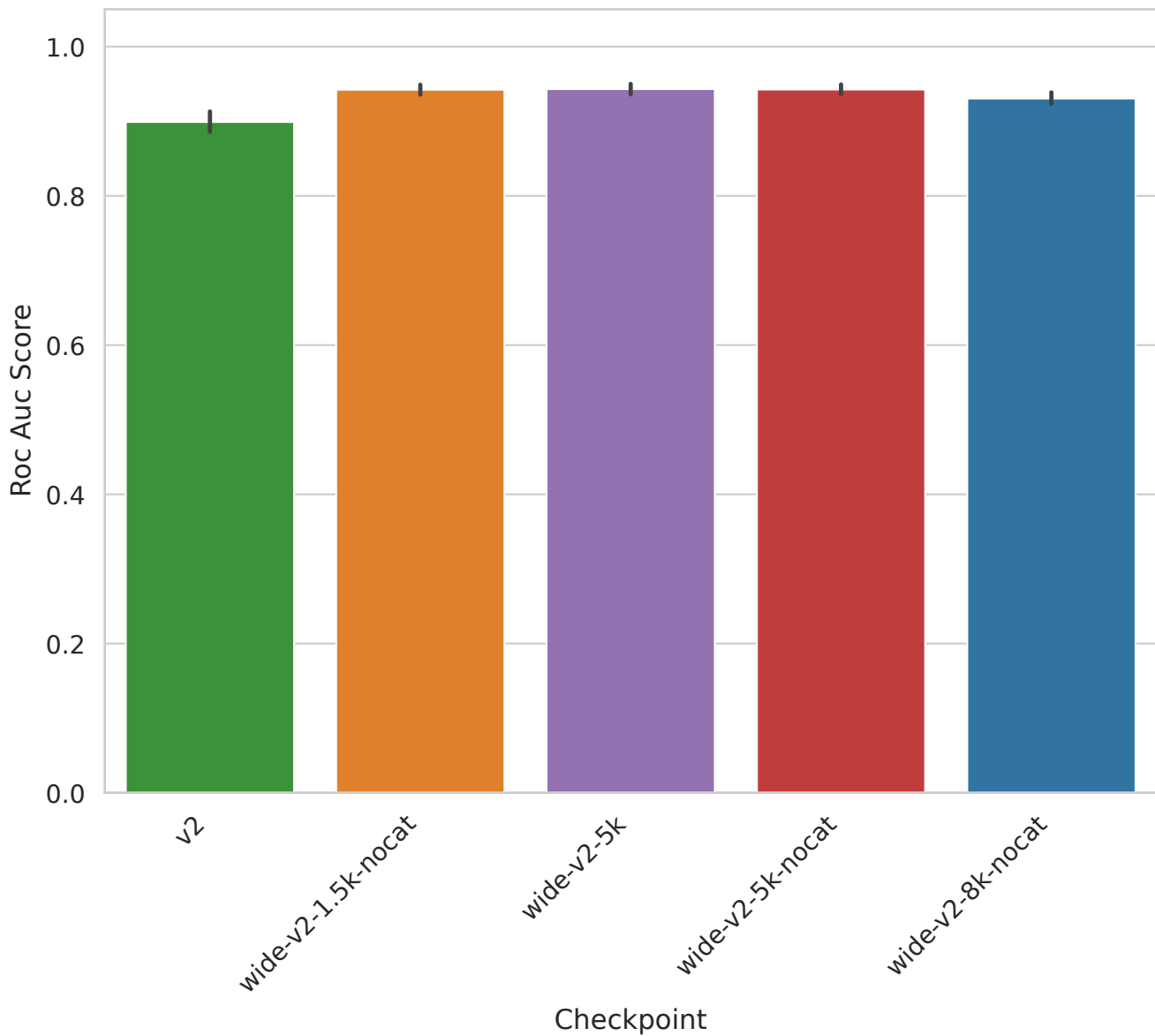
arcene - Roc Auc Score
