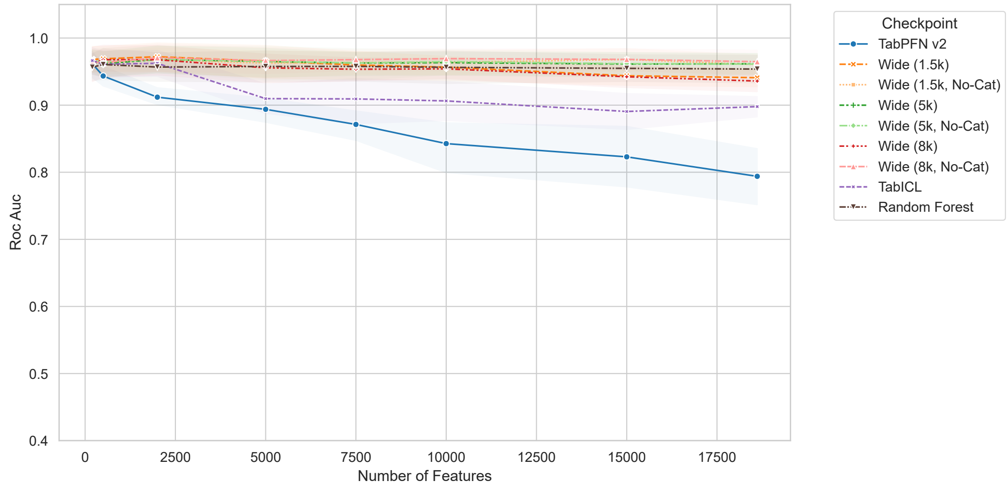
GBM - Roc Auc vs Feature Count
