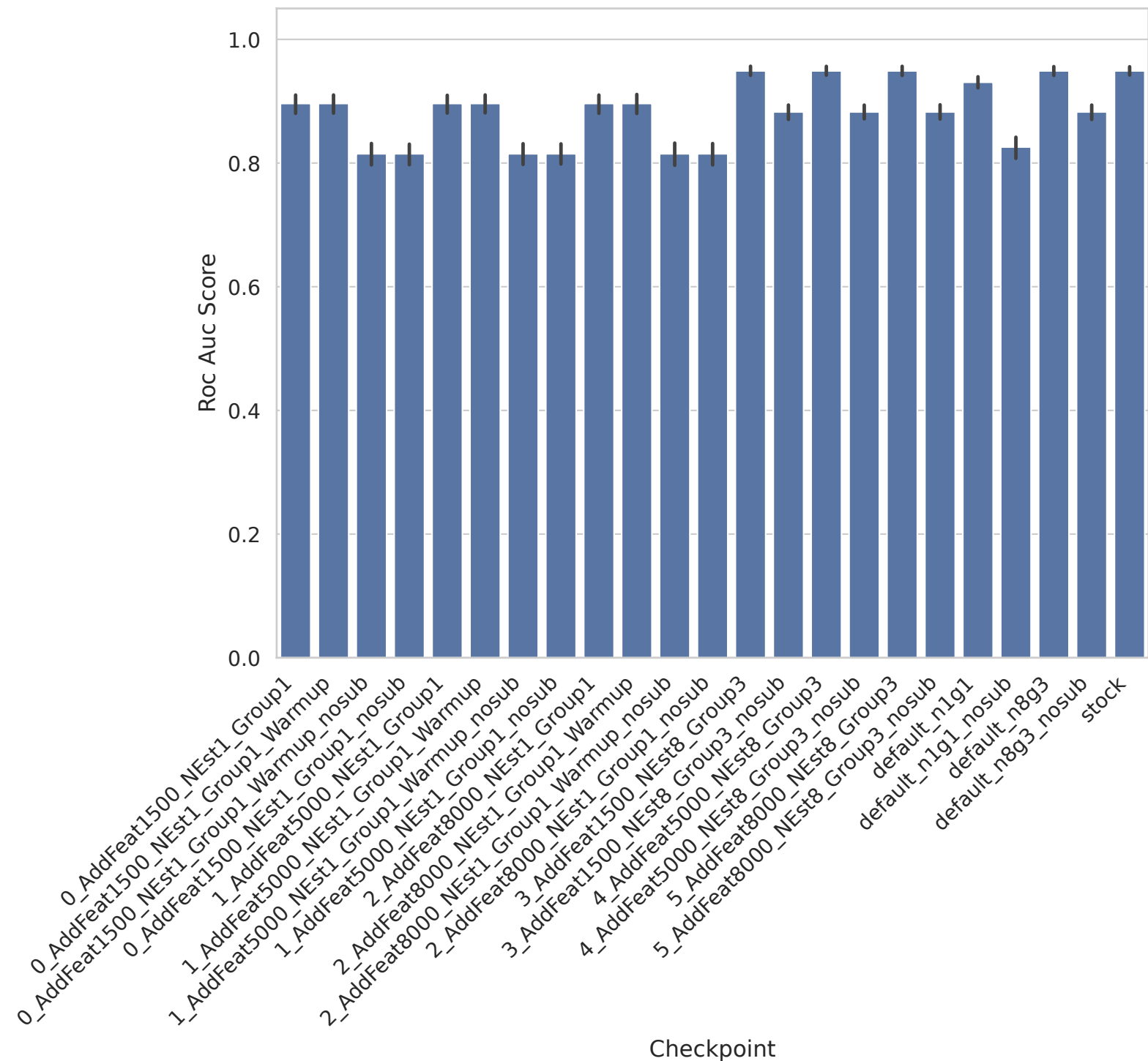
arcene - Roc Auc Score
