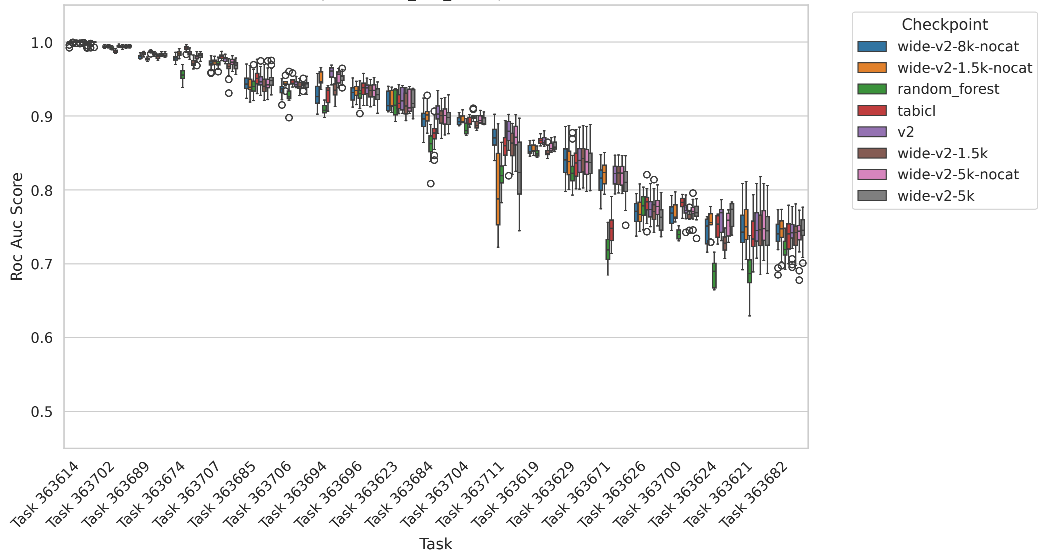
openml - roc_auc_score per Task
