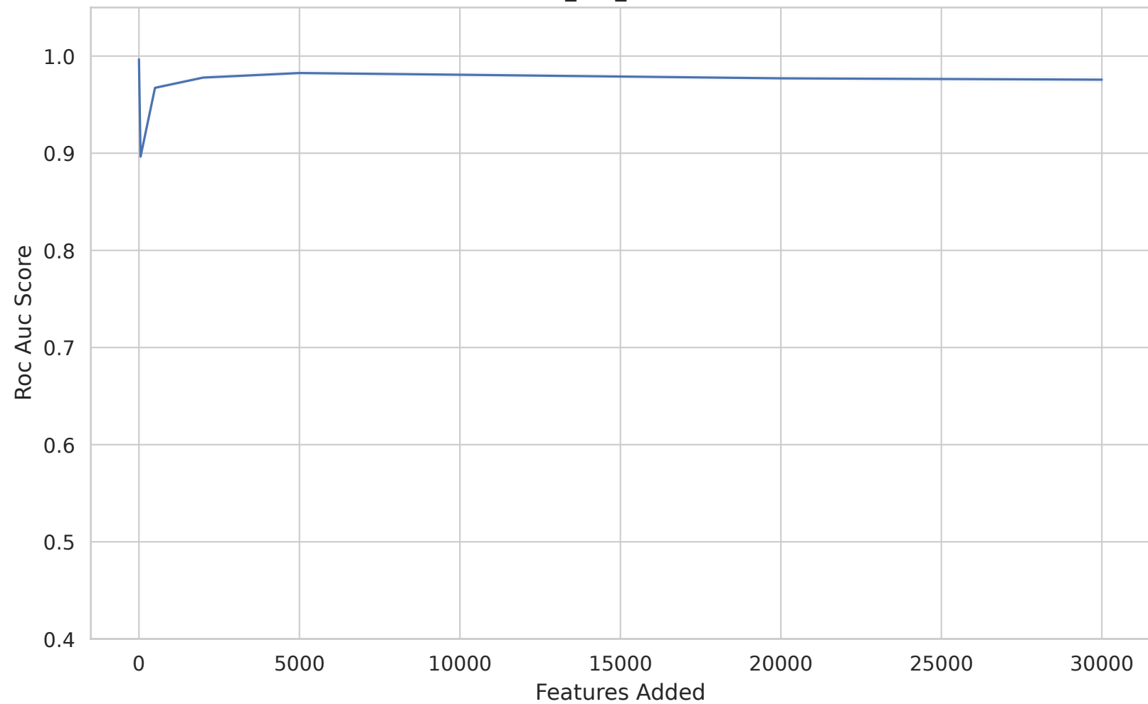
Dataset 40984 - roc_auc_score vs Features Added
