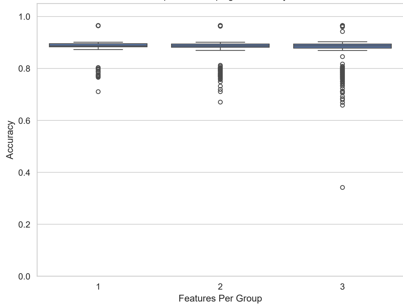
Impact of Grouping on Accuracy
