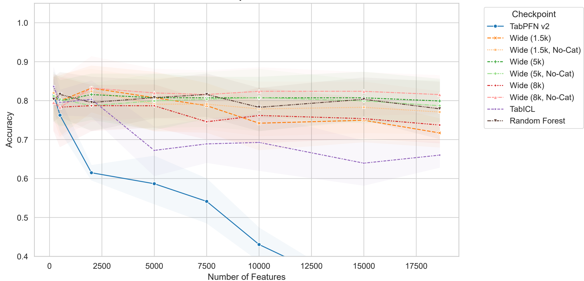
GBM - Accuracy vs Feature Count
