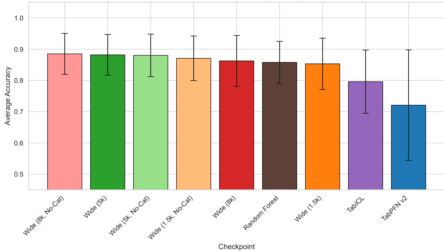
Multiomics Overview - Average Accuracy
