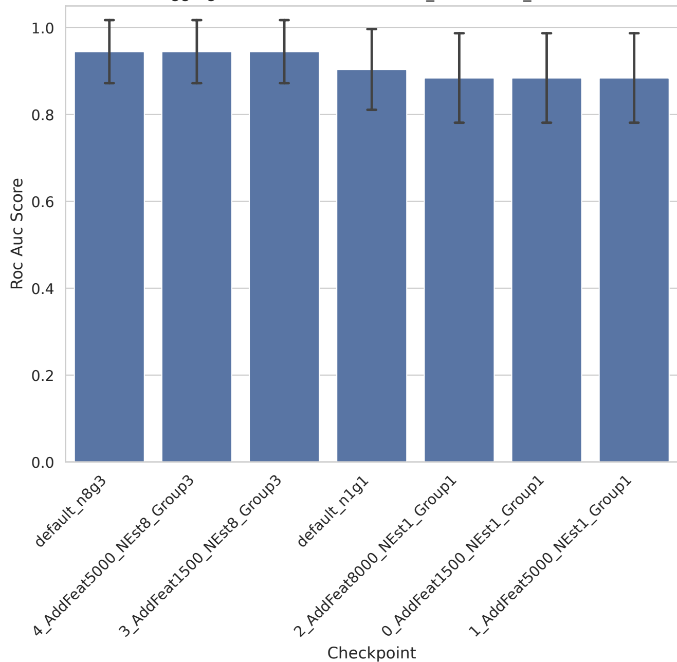
Aggregated Roc Auc Score - hdlss_benchmark_results
