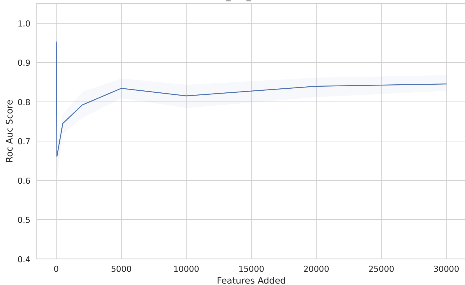
Dataset 1049 - roc_auc_score vs Features Added
