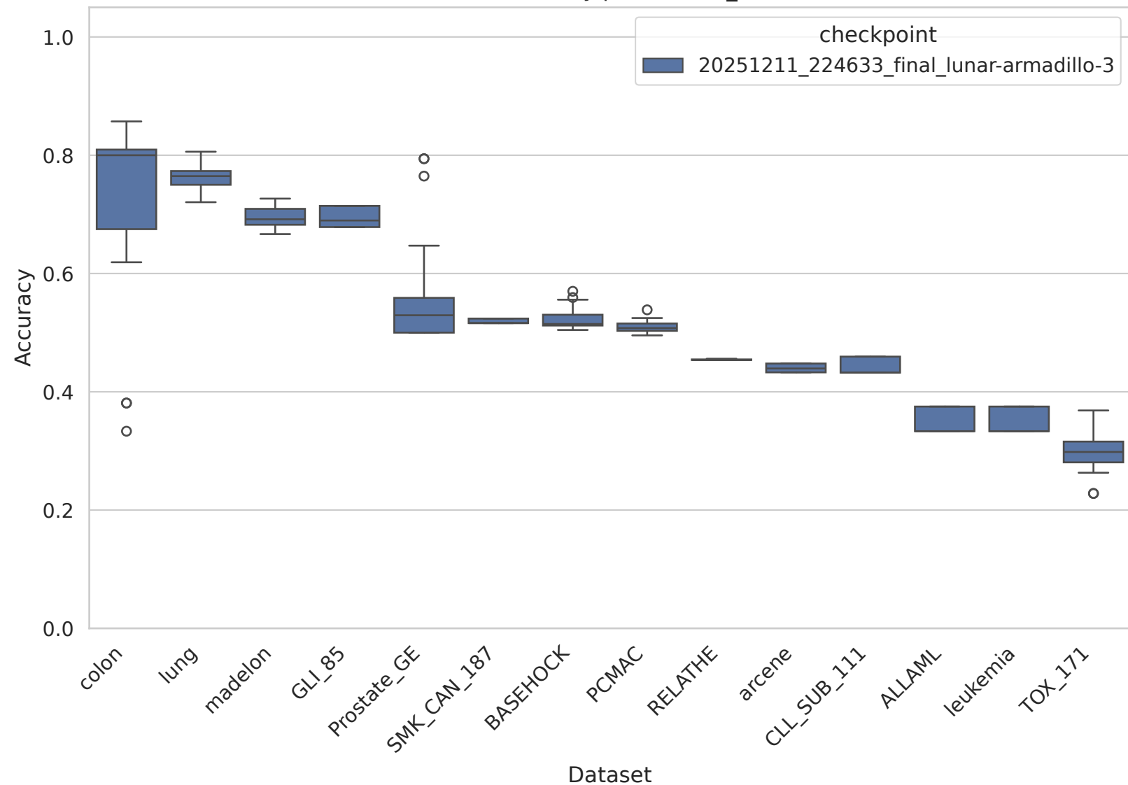
hdls - accuracy per dataset_name
