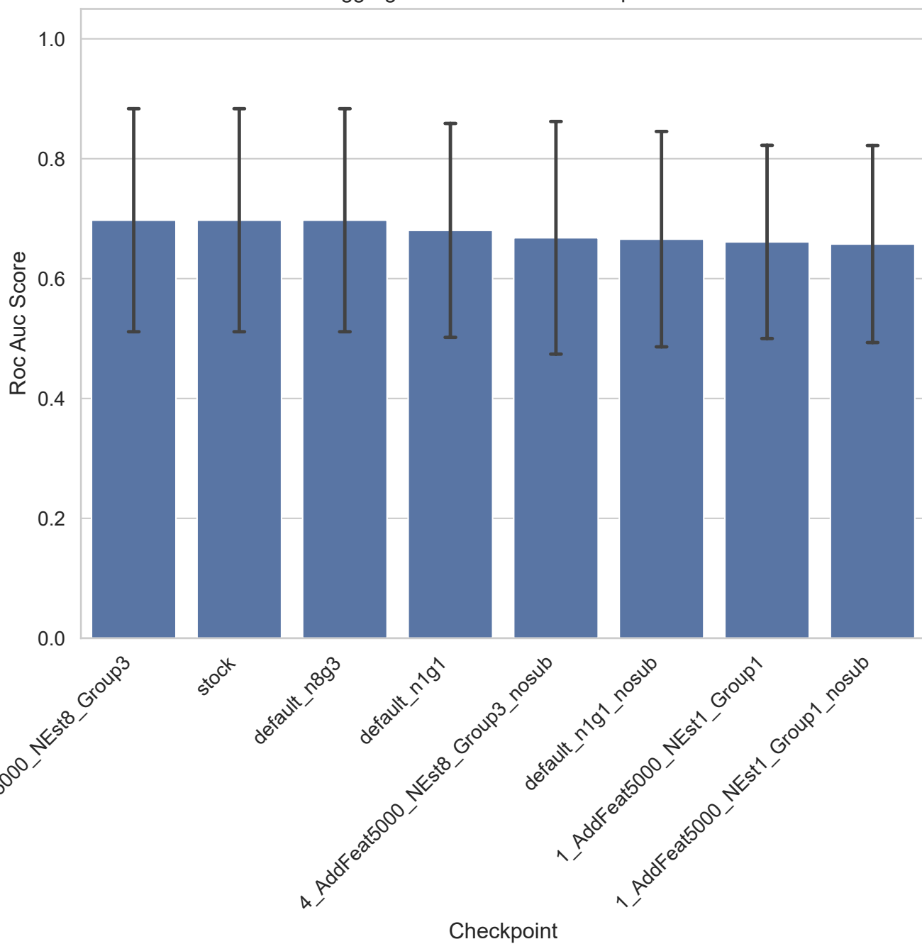
Aggregated Roc Auc Score - openml
