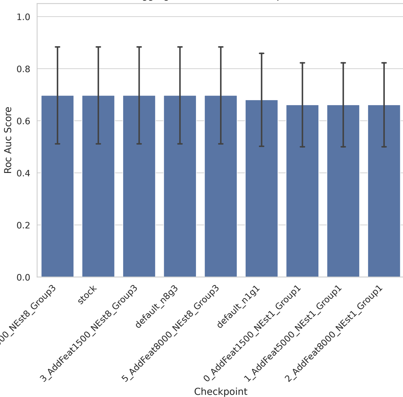
Aggregated Roc Auc Score - openml
