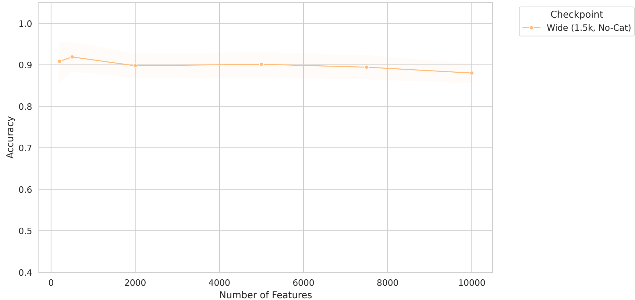
OV - Accuracy vs Feature Count
