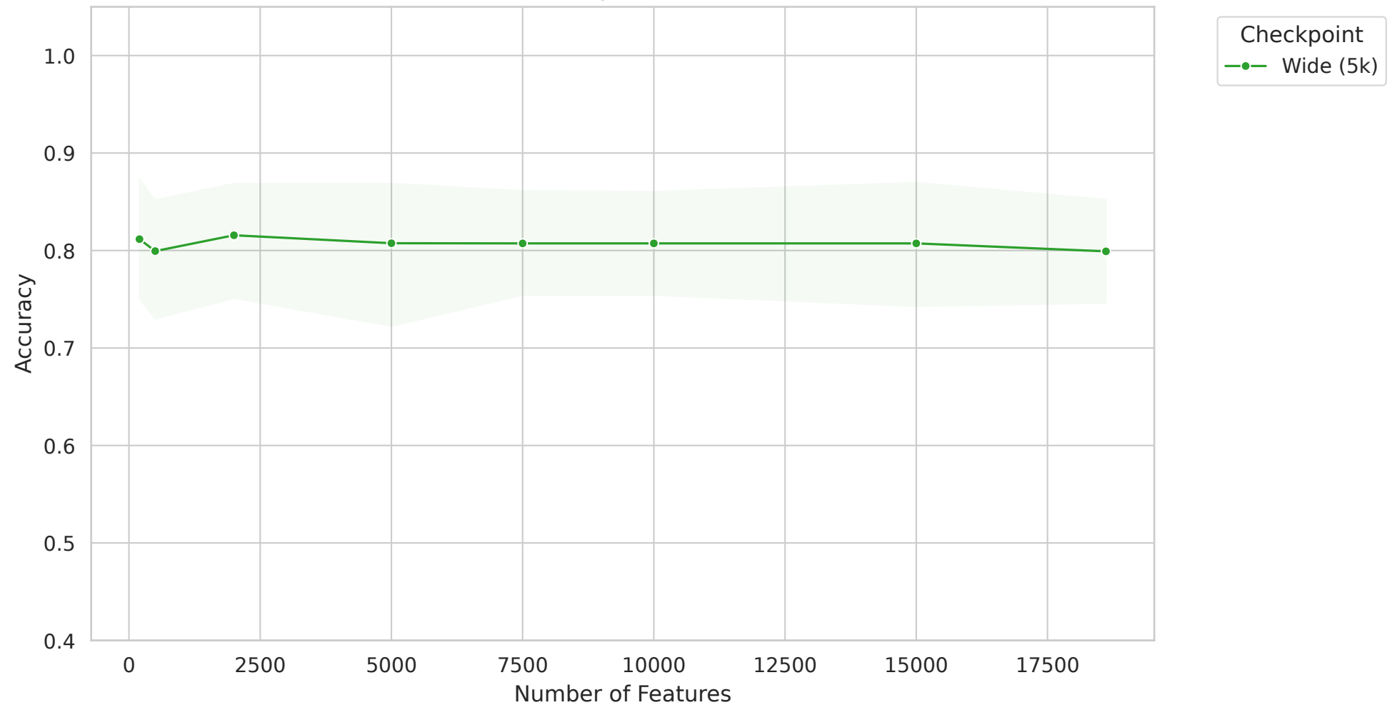
GBM - Accuracy vs Feature Count
