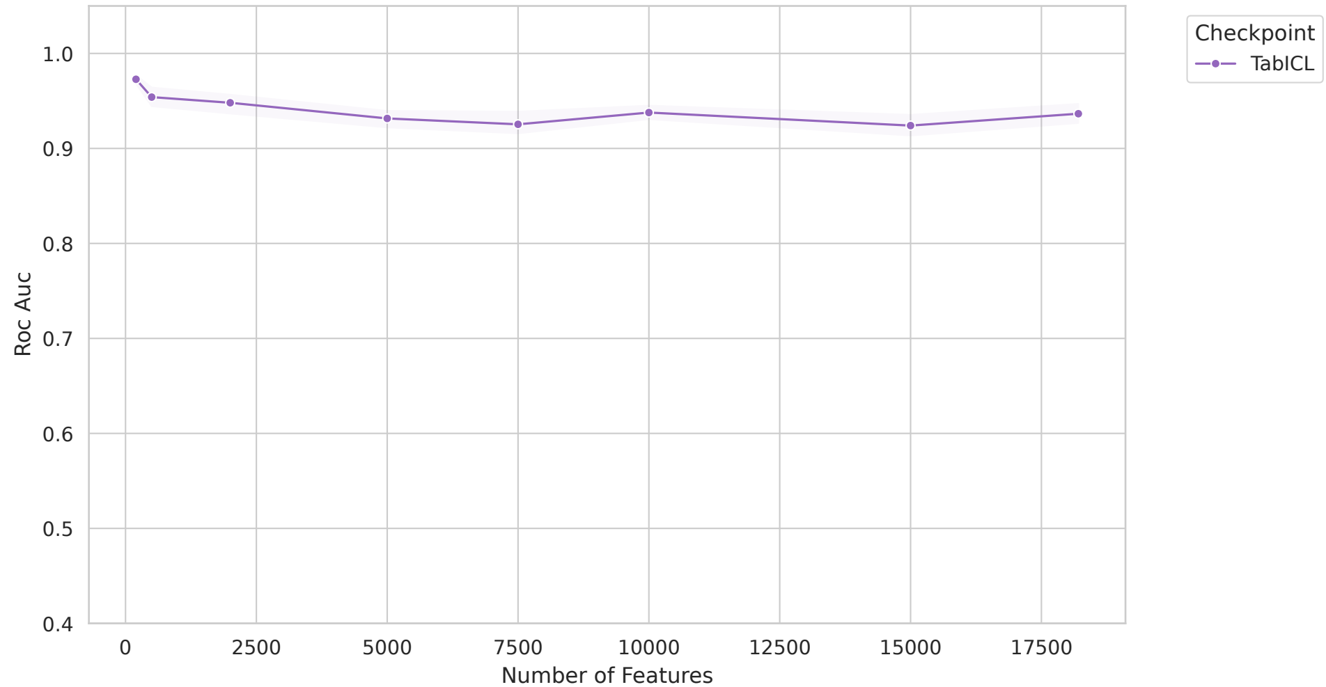
BRCA - Roc Auc vs Feature Count
