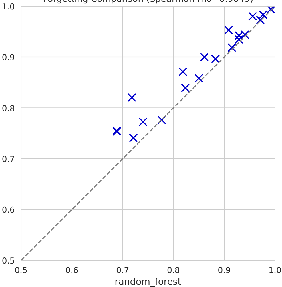
Forgetting Comparison (Spearman rho=0.9649)
