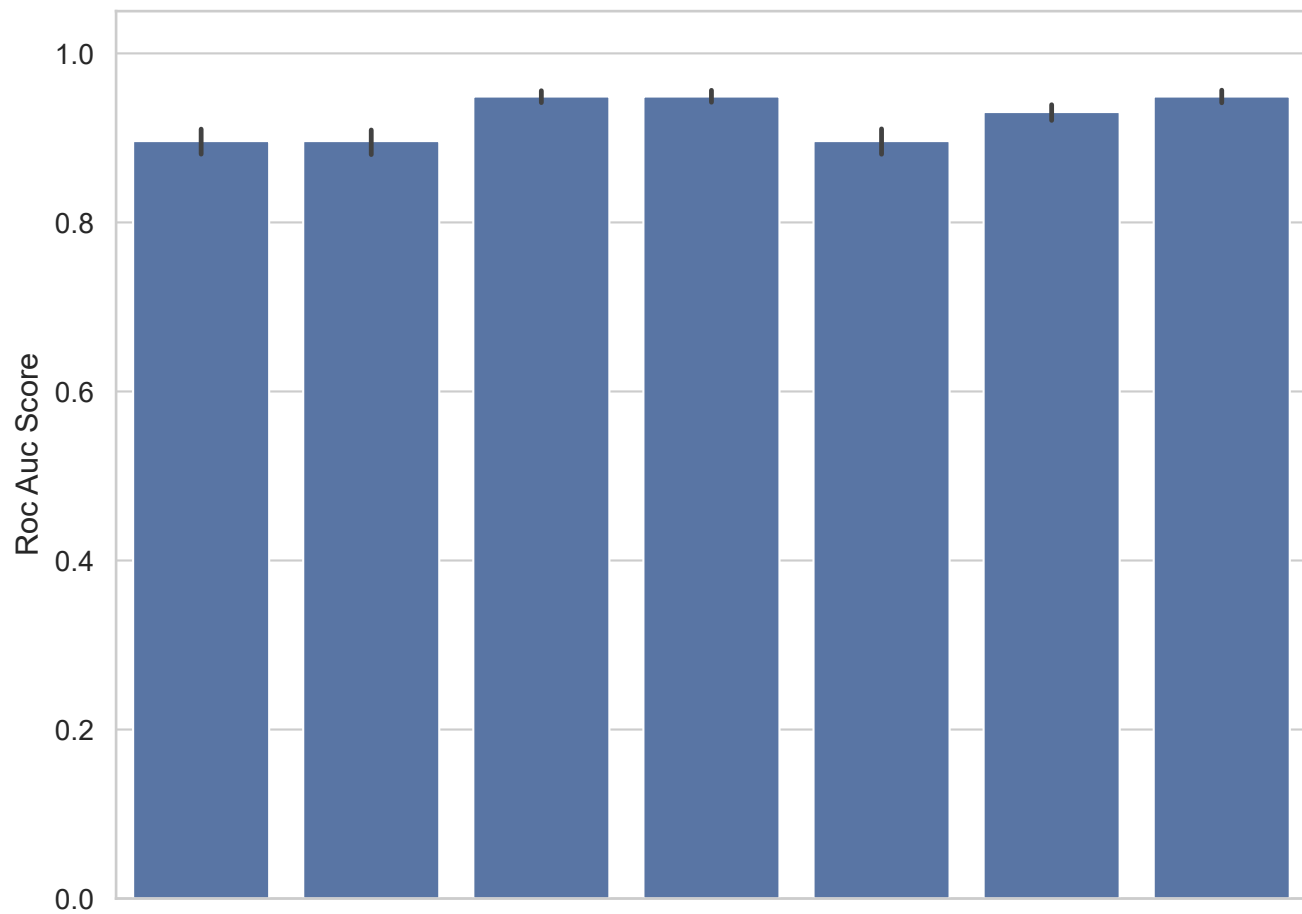
arcene - Roc Auc Score
