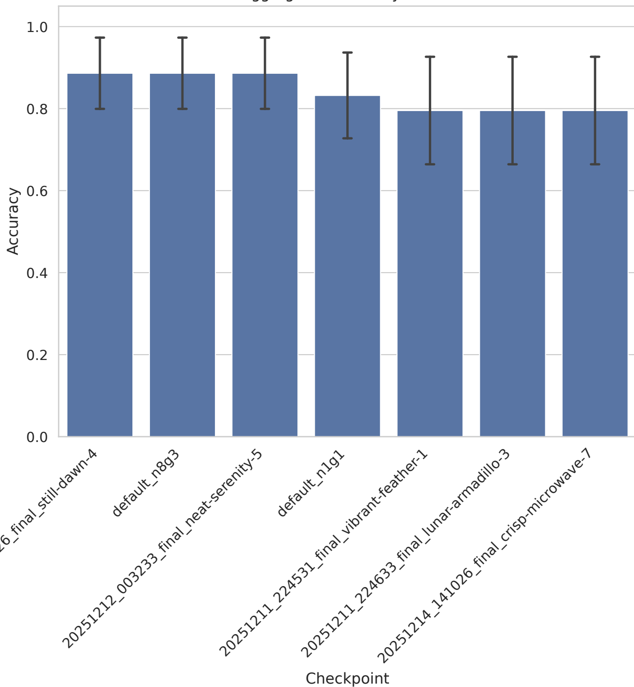
Aggregated Accuracy - hdlss
