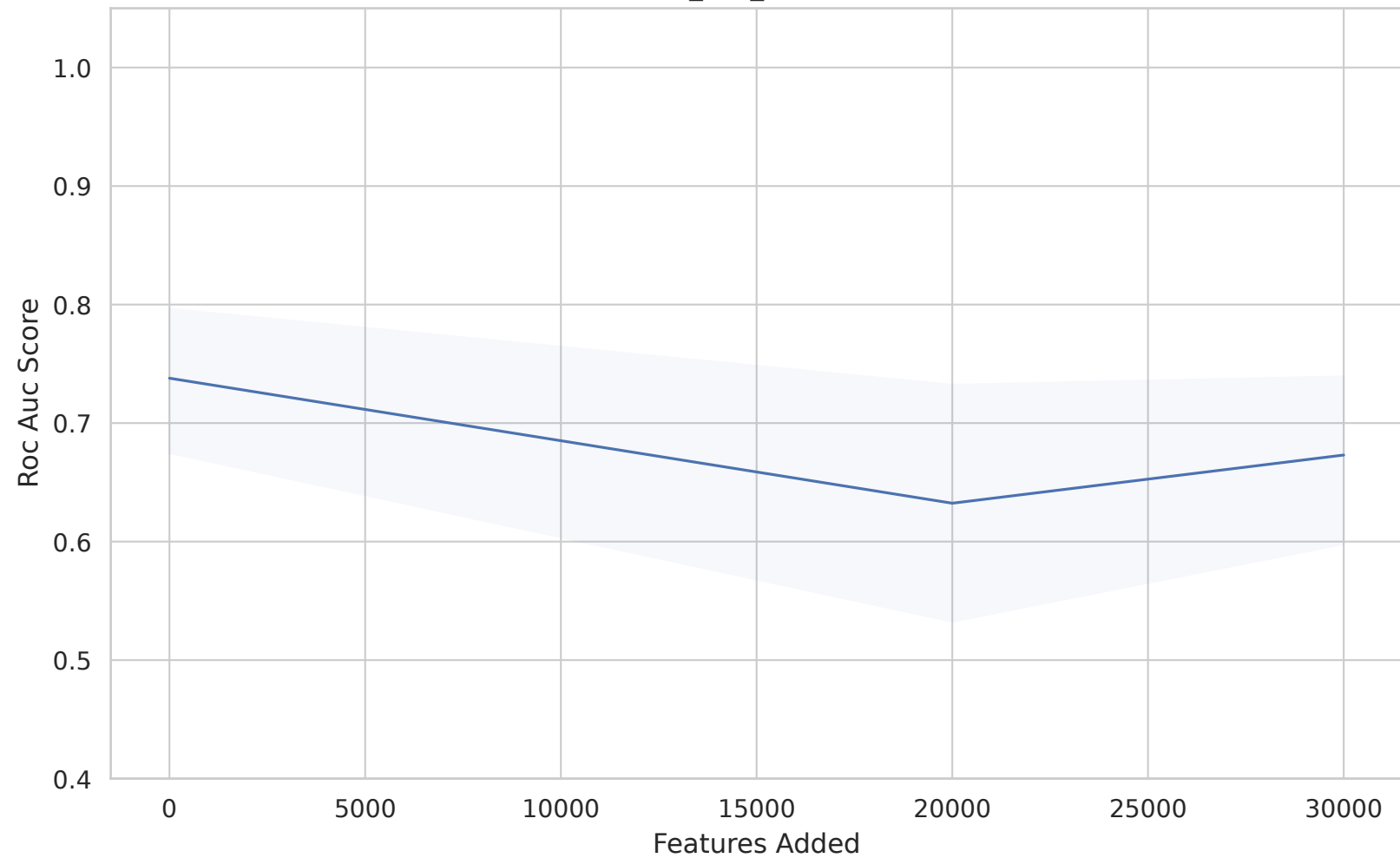
Dataset 41157 - roc_auc_score vs Features Added
