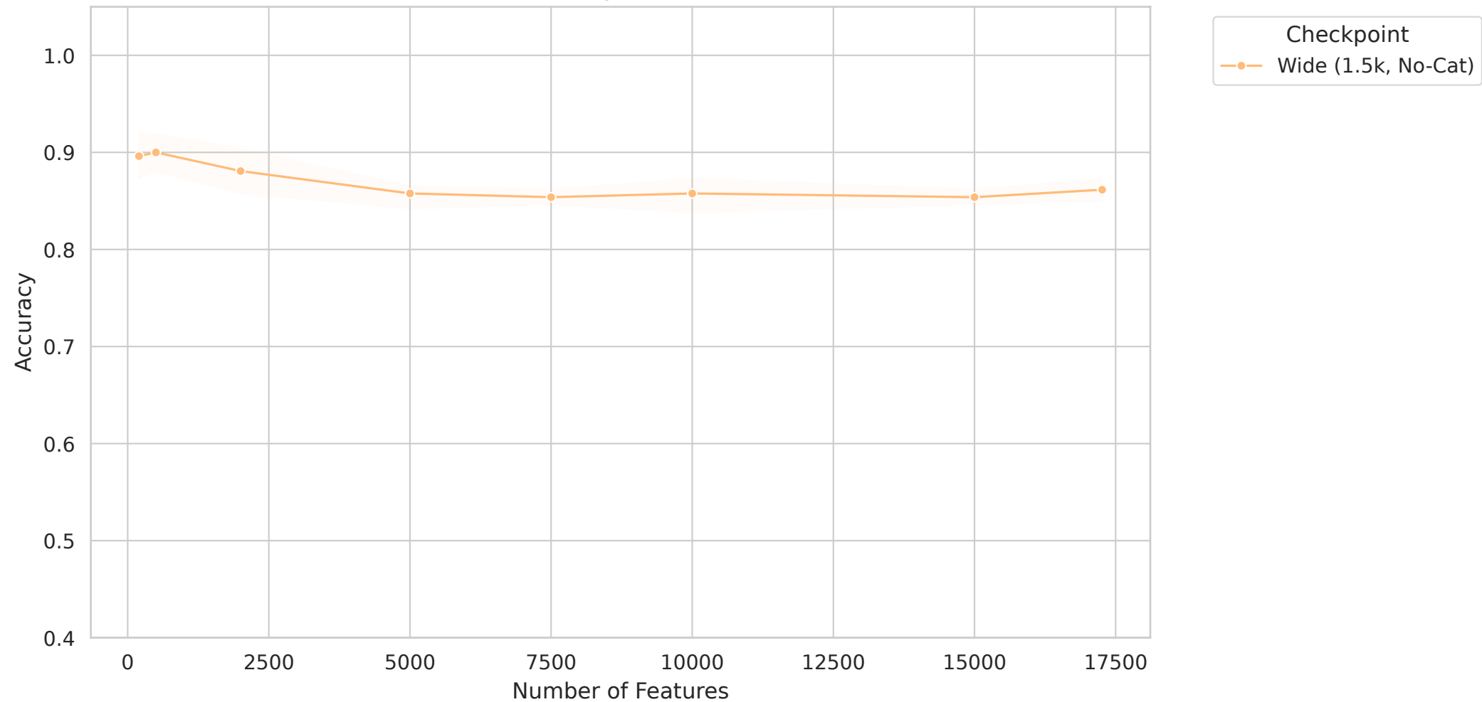
COAD - Accuracy vs Feature Count
