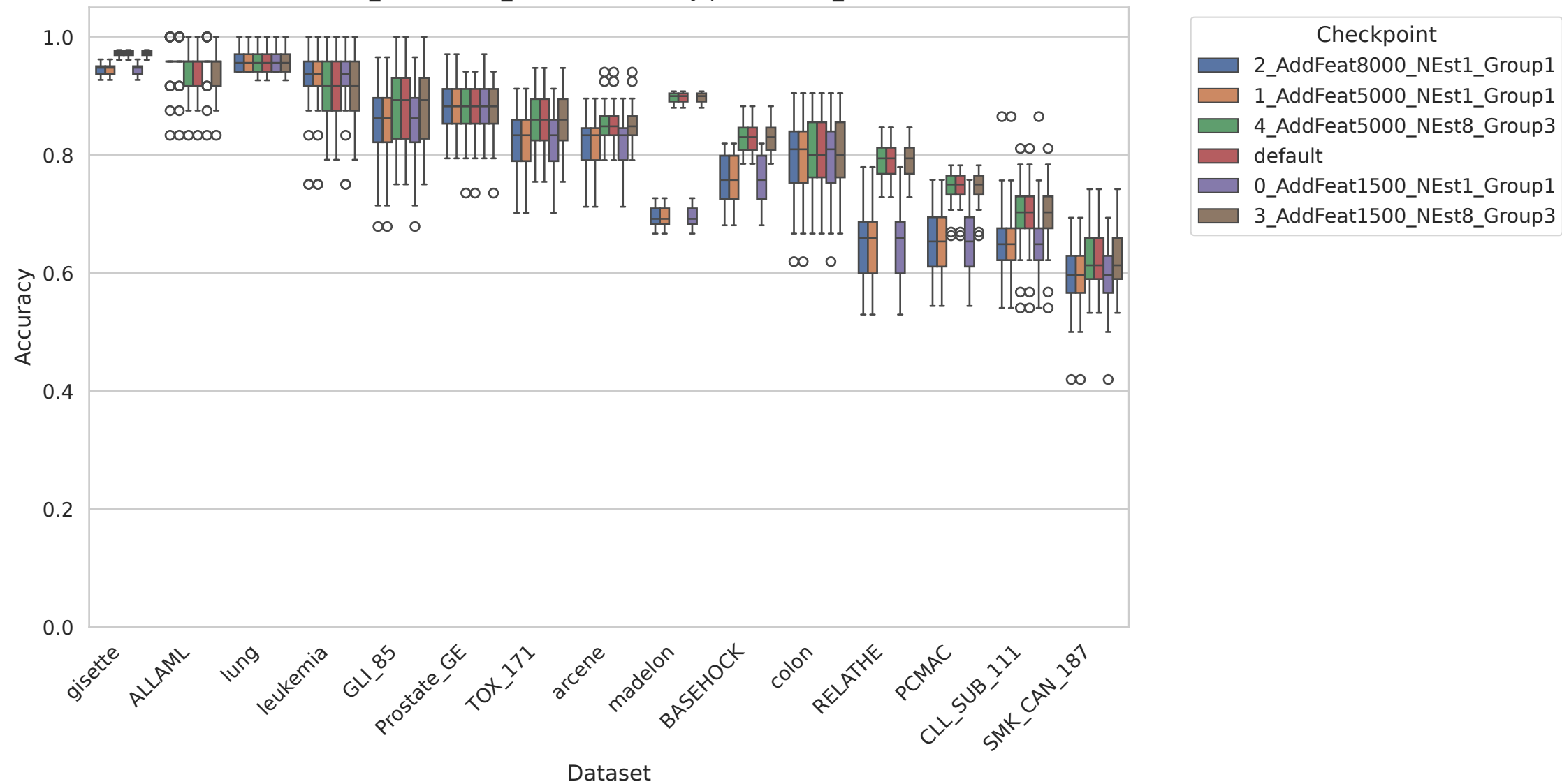
hdlss_benchmark_results - accuracy per dataset_name
