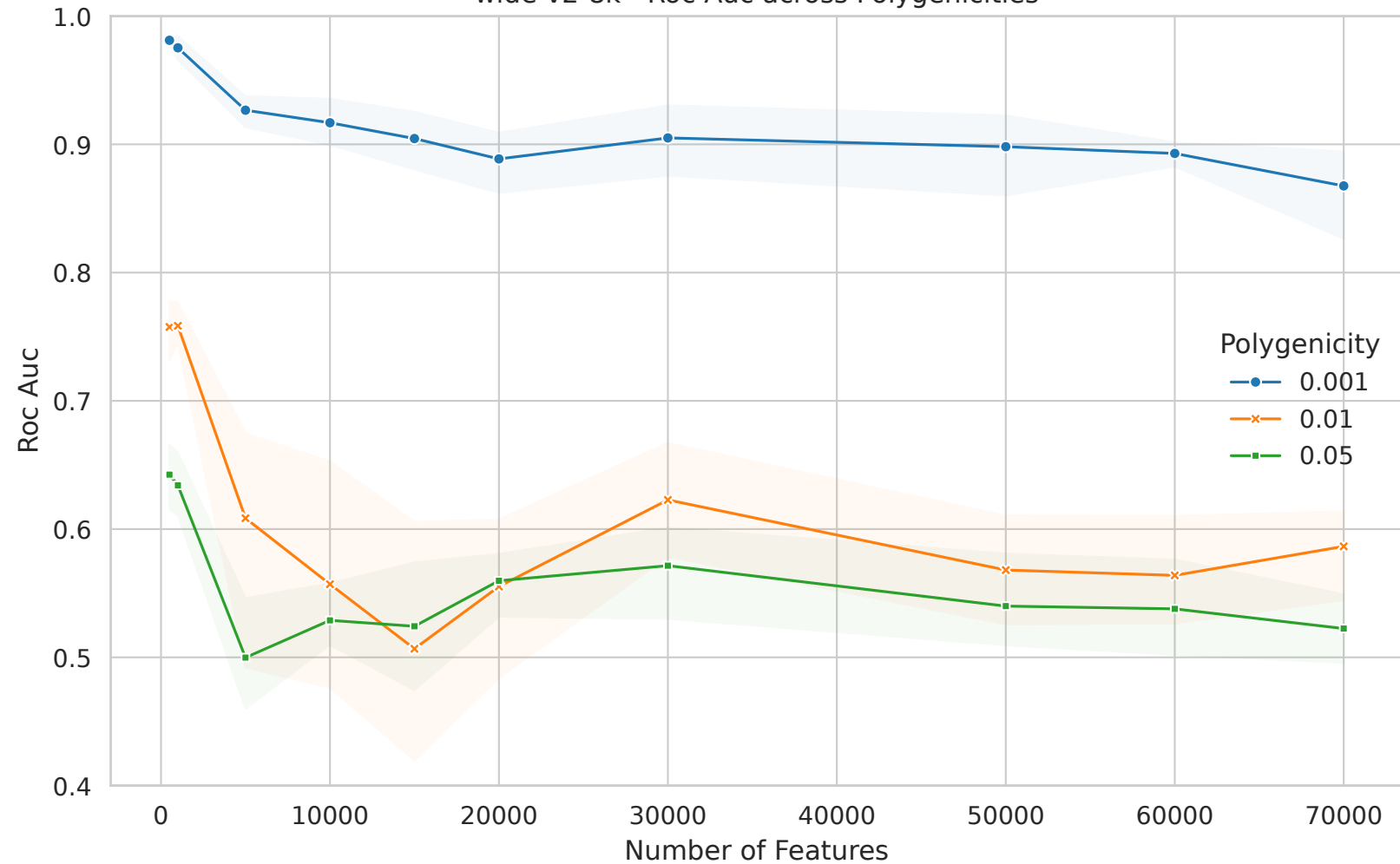
wide-v2-8k - Roc Auc across Polygenicities
