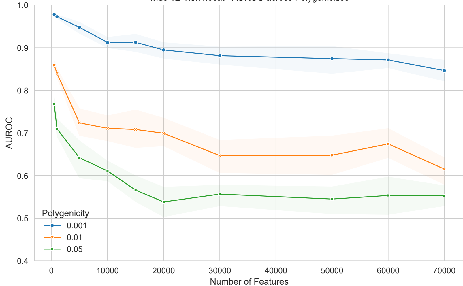
wide-v2-1.5k-nocat - AUROC across Polygenicitities
