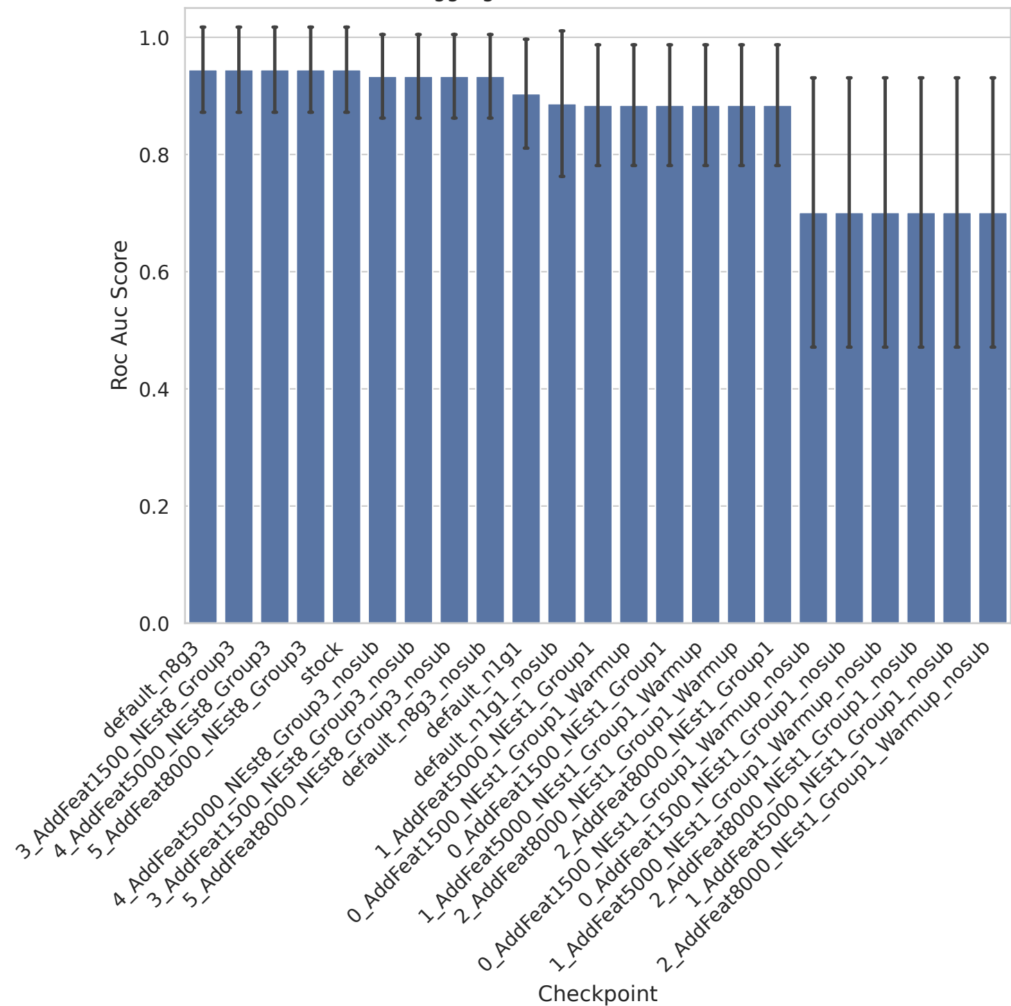
Aggregated Roc Auc Score - hdlss
