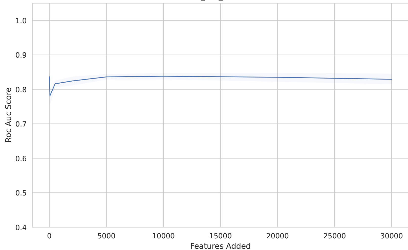
Dataset 46921 - roc_auc_score vs Features Added
