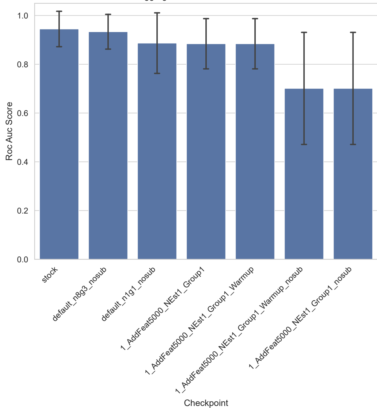
Aggregated Roc Auc Score - hdls
