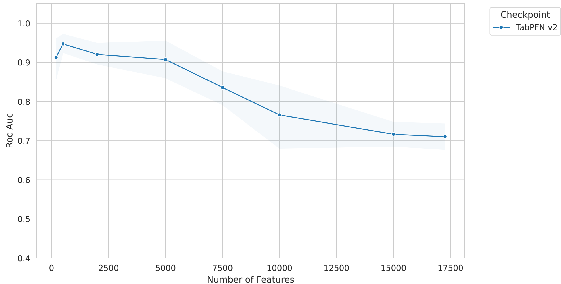
COAD - Roc Auc vs Feature Count
