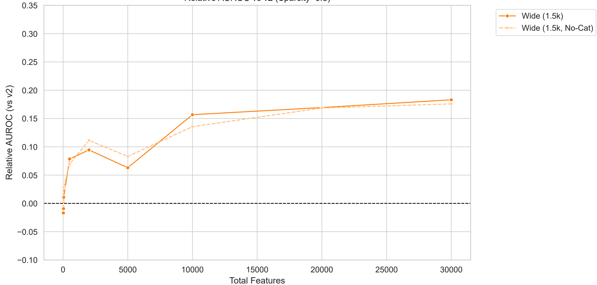
Relative AUROC vs v2 (Sparsity=0.5)
