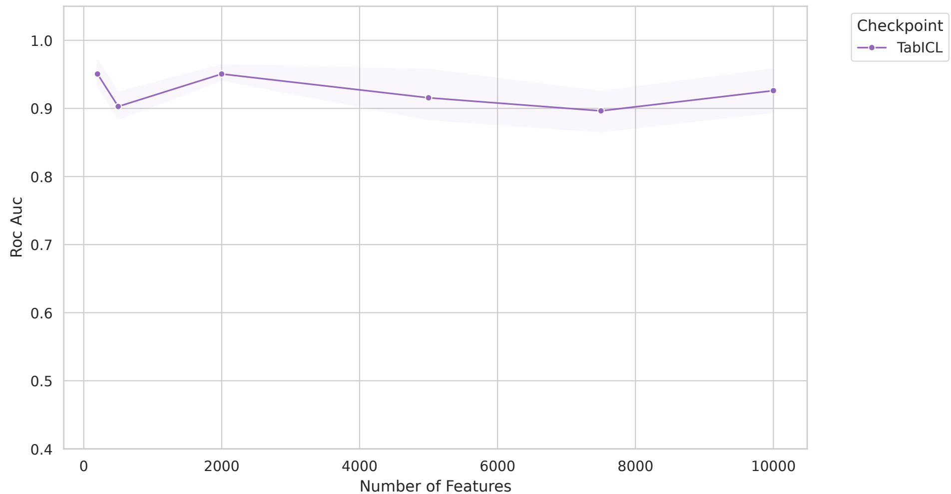
OV - Roc Auc vs Feature Count
