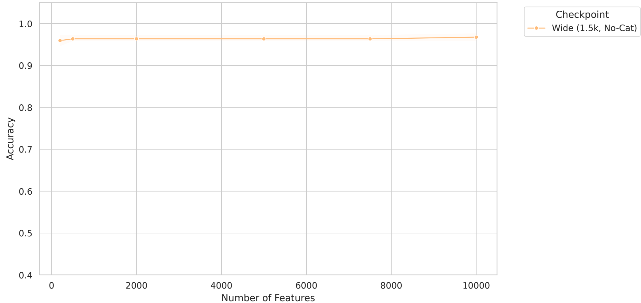
LGG - Accuracy vs Feature Count
