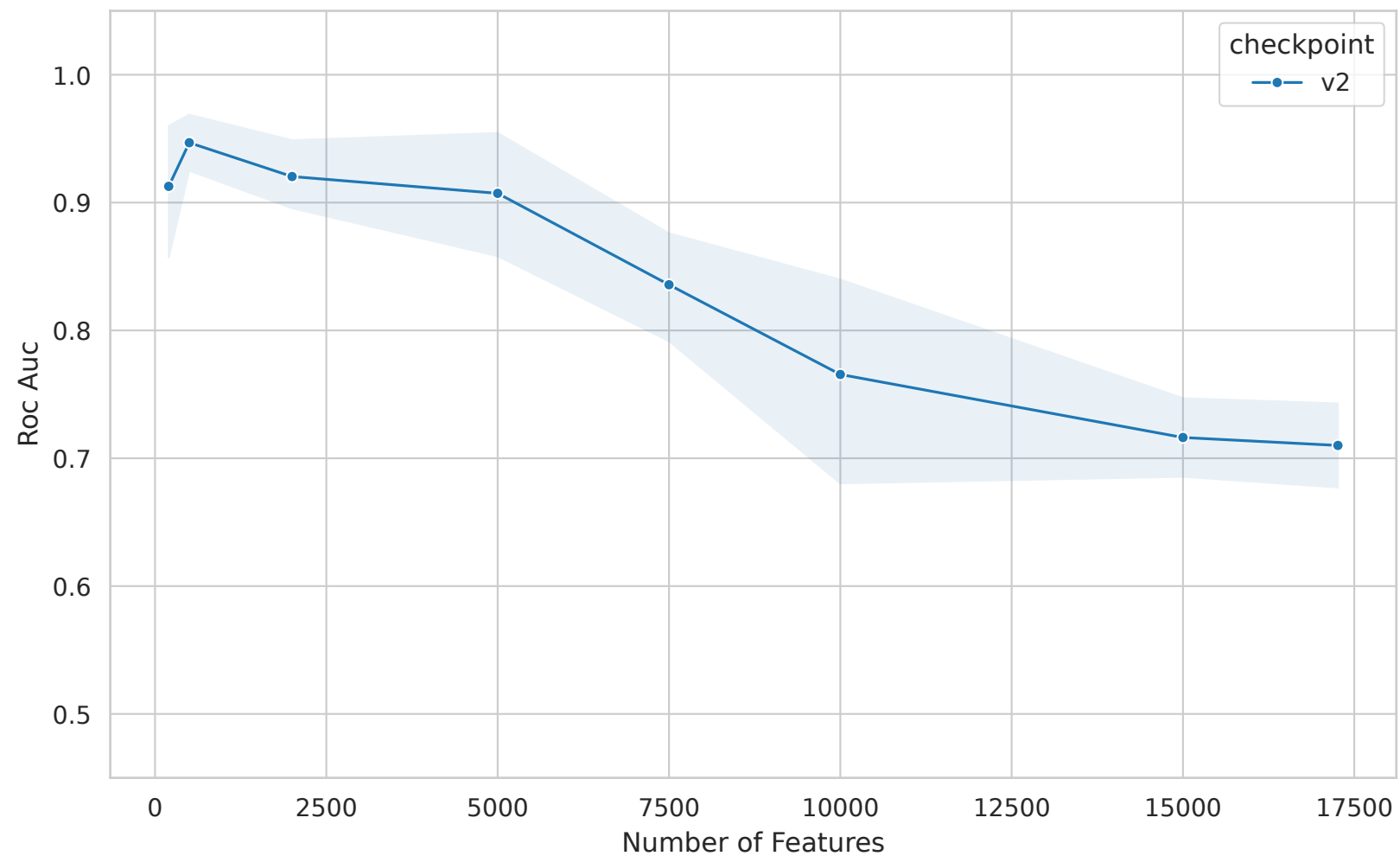
COAD - Roc Auc vs Feature Count
