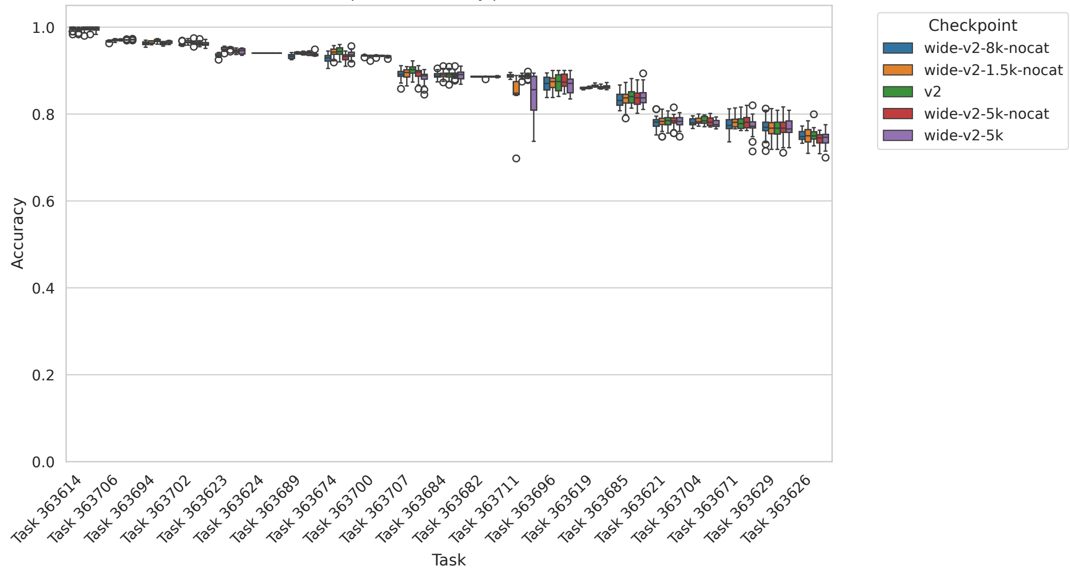
openml - accuracy per Task
