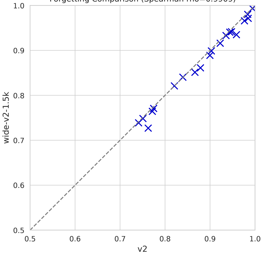
Forgetting Comparison (Spearman rho=0.9909)
