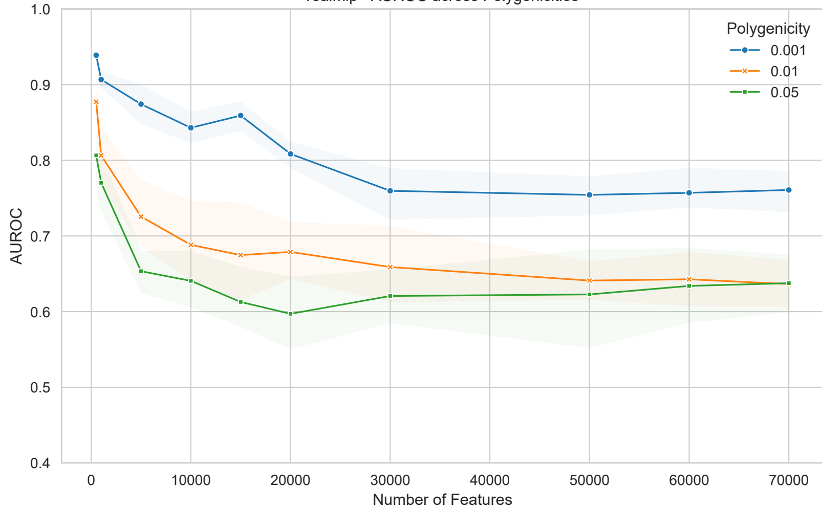
realmlp - AUROC across Polygenicities
