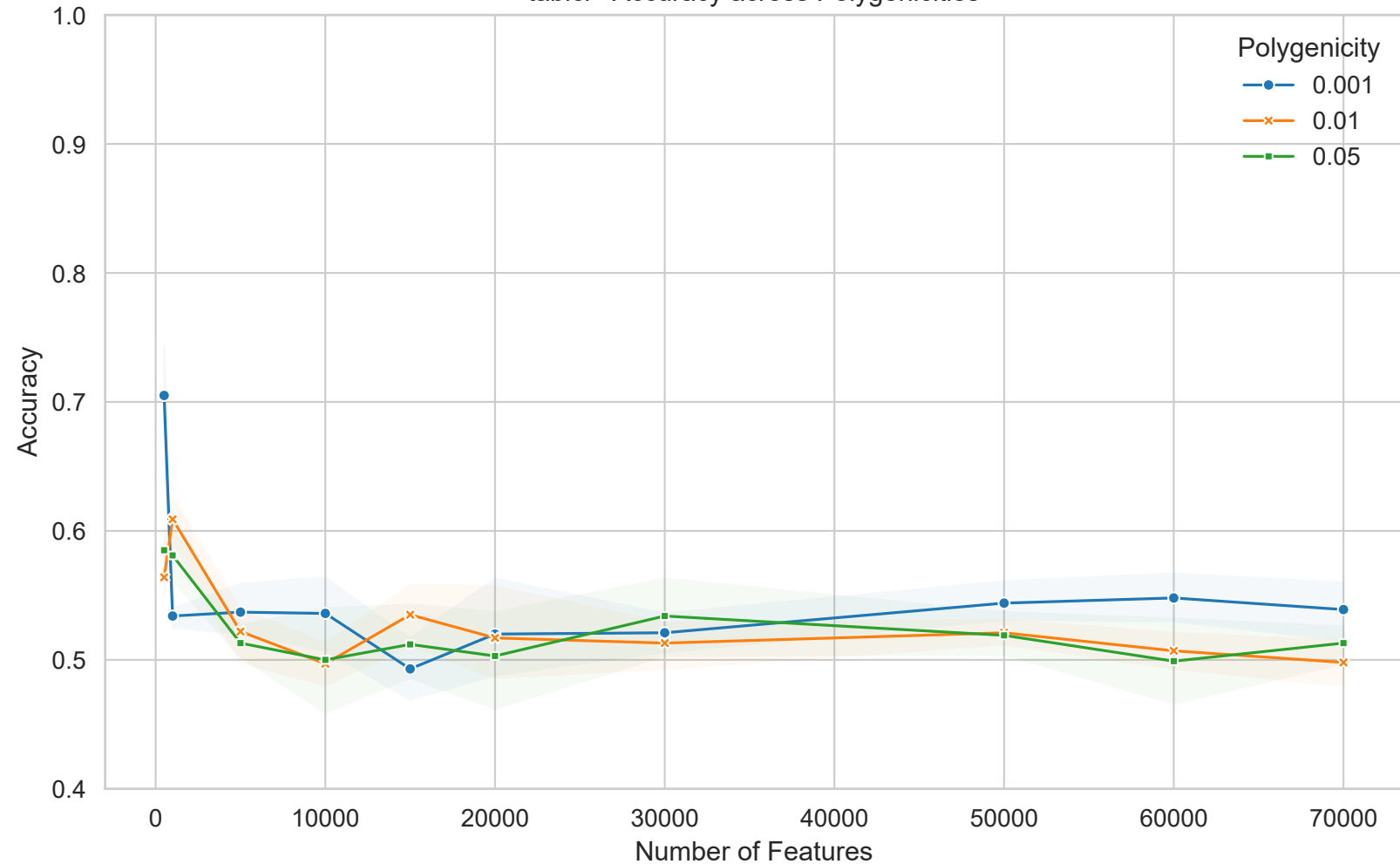
tab1c1 - Accuracy across Polygenicities
