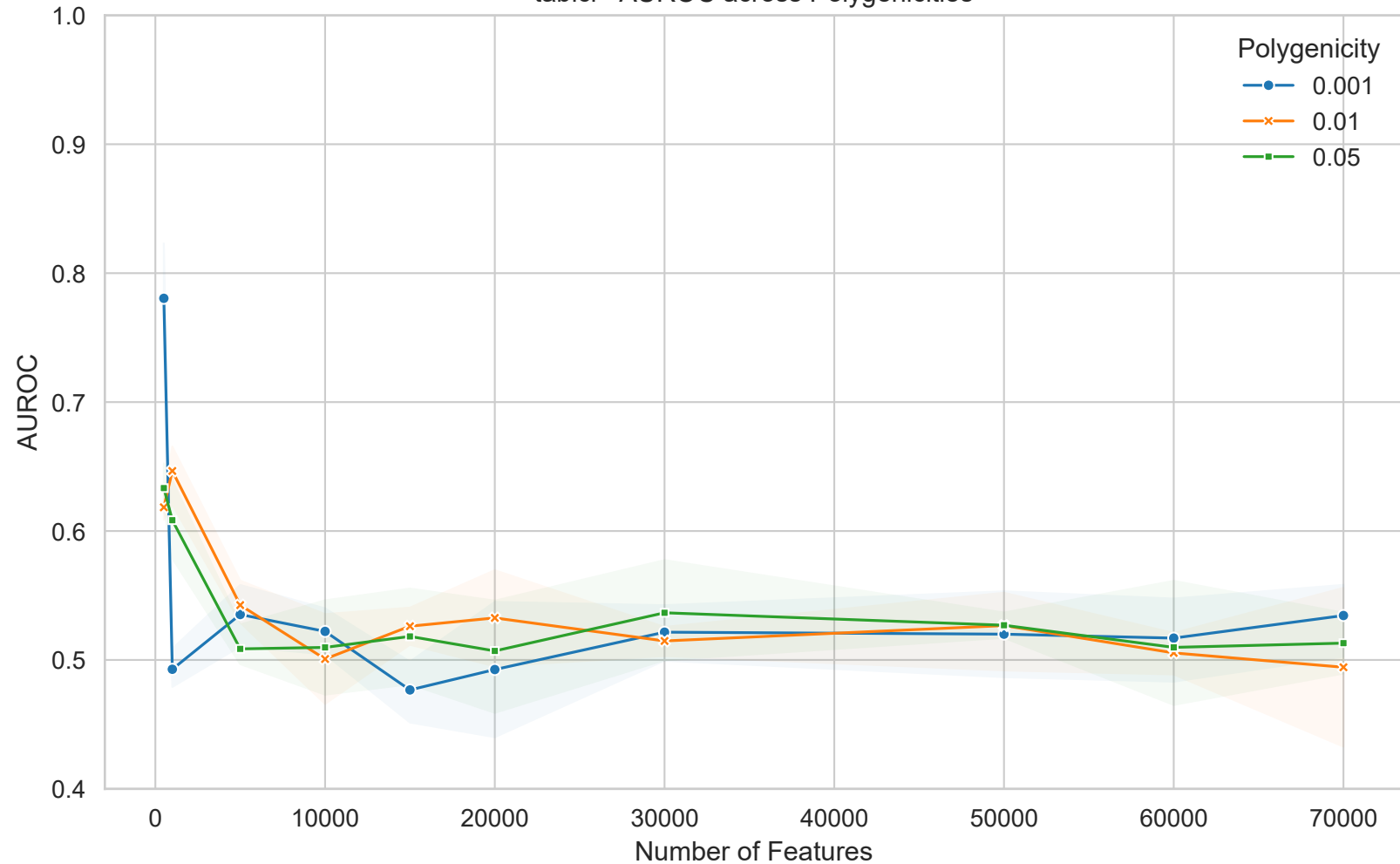
tabicl - AUROC across Polygenicities
