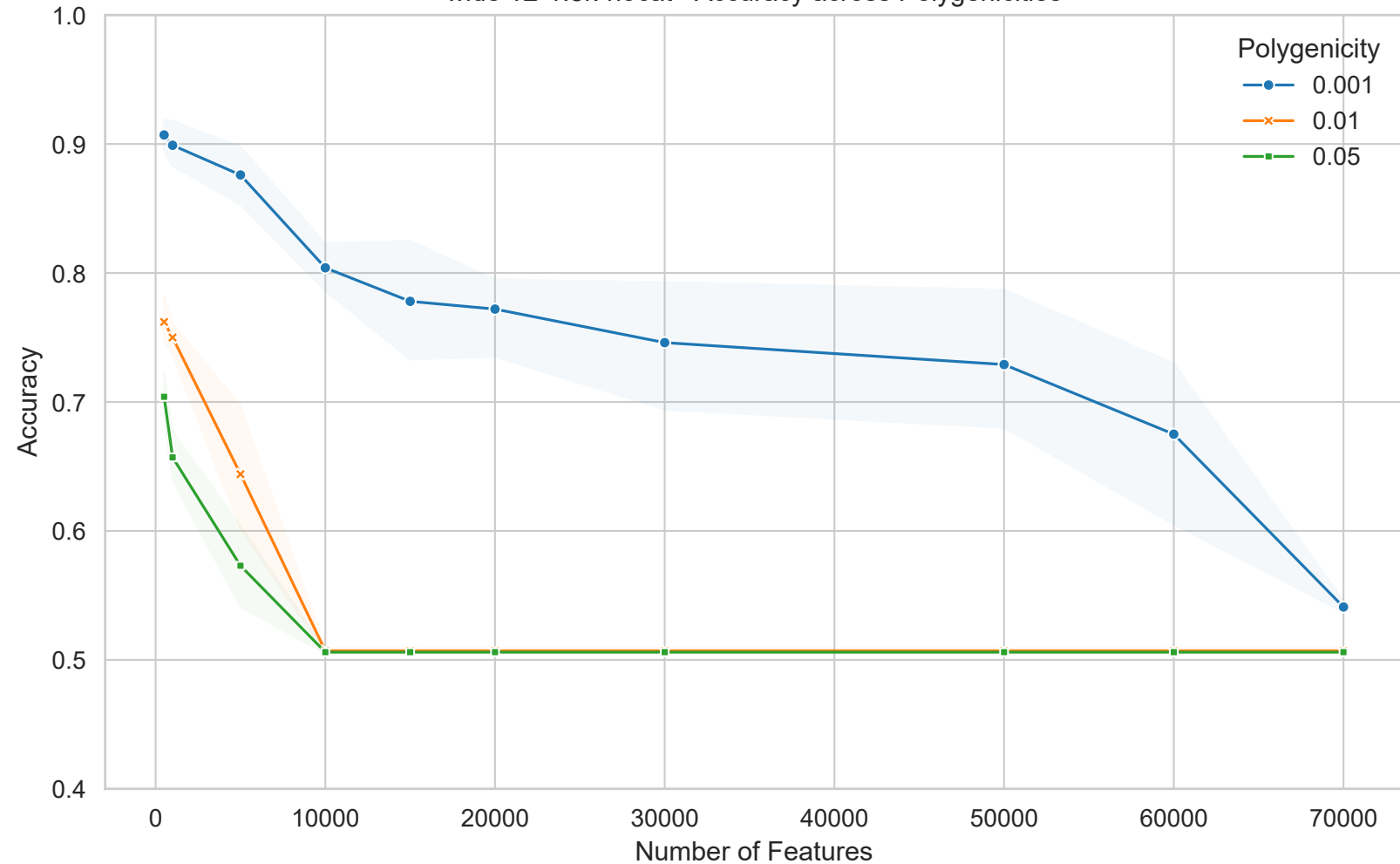
wide-v2-1.5k-nocat - Accuracy across Polygenicities
