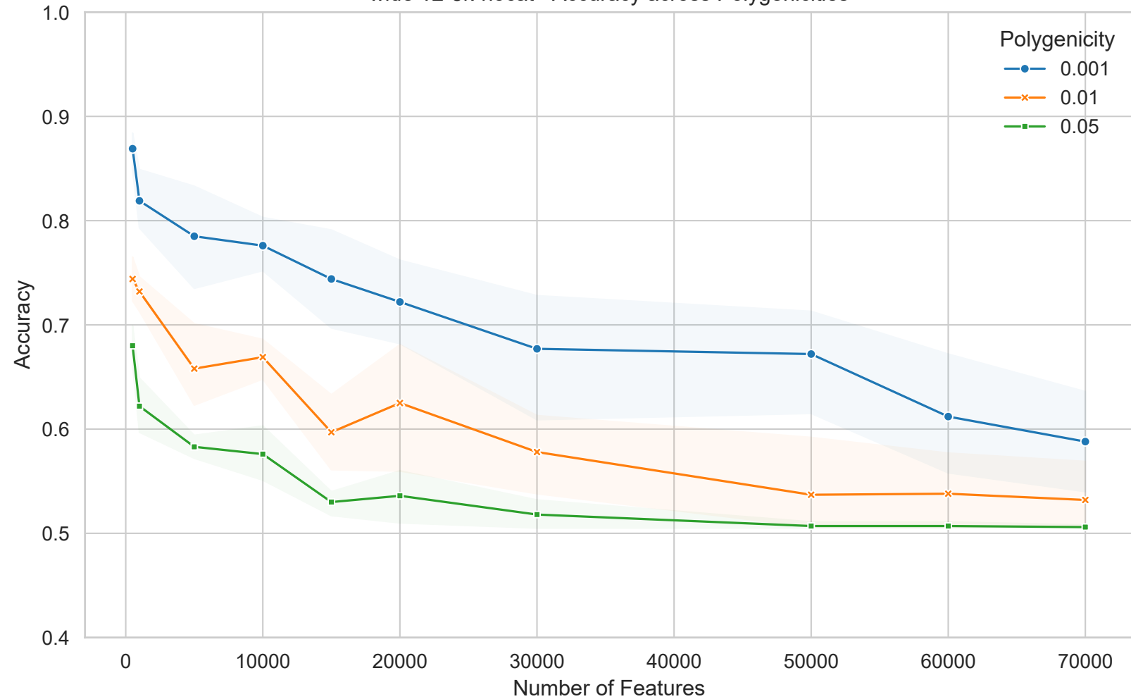
wide-v2-5k-nocat - Accuracy across Polygenicities
