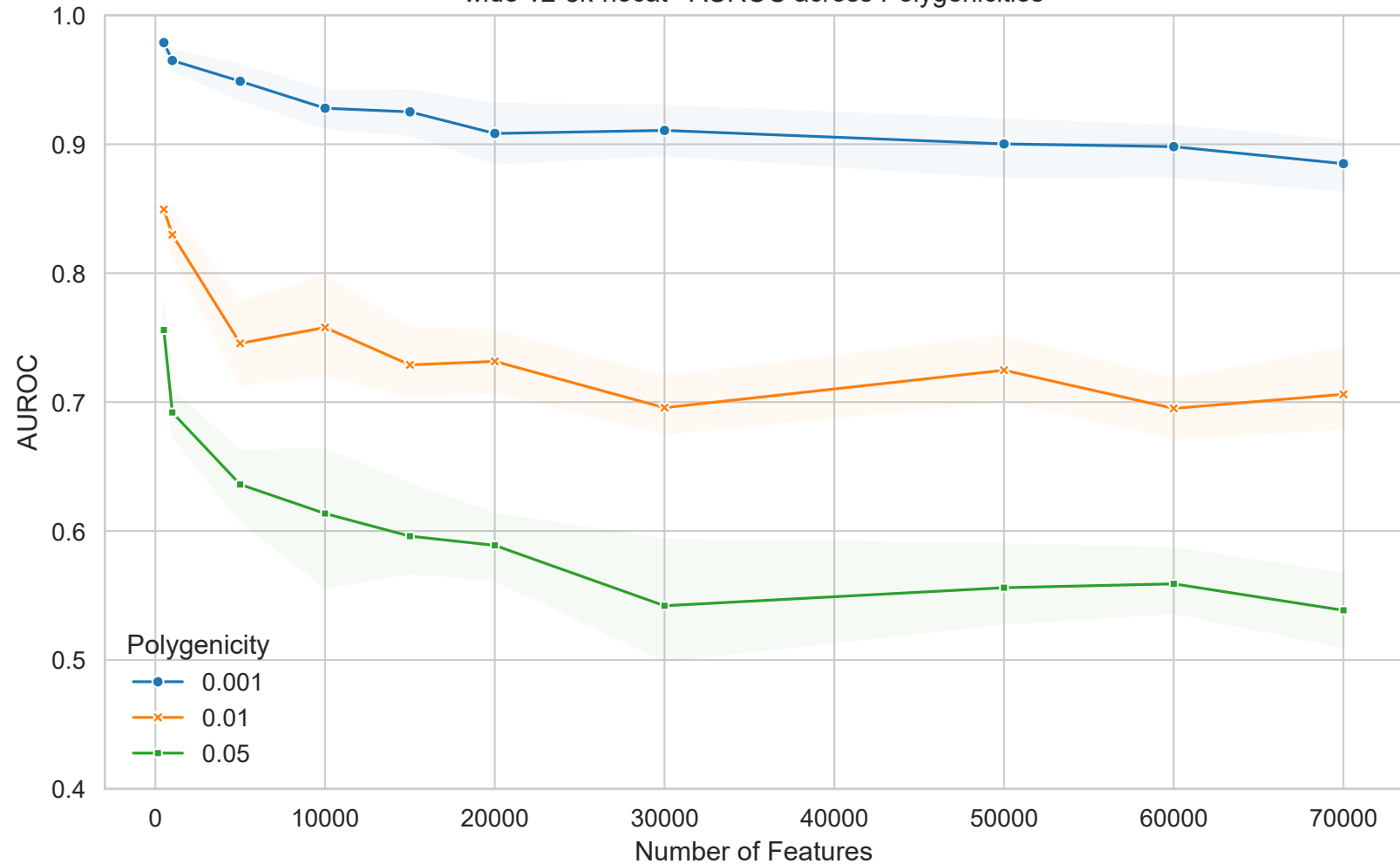
wide-v2-8k-nocat - AUROC across Polygenicities
