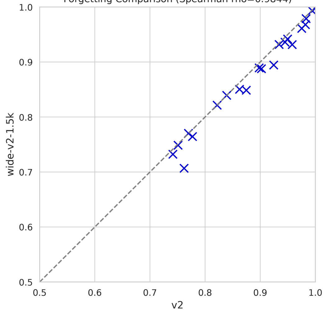
Forgetting Comparison (Spearman rho=0.9844)
