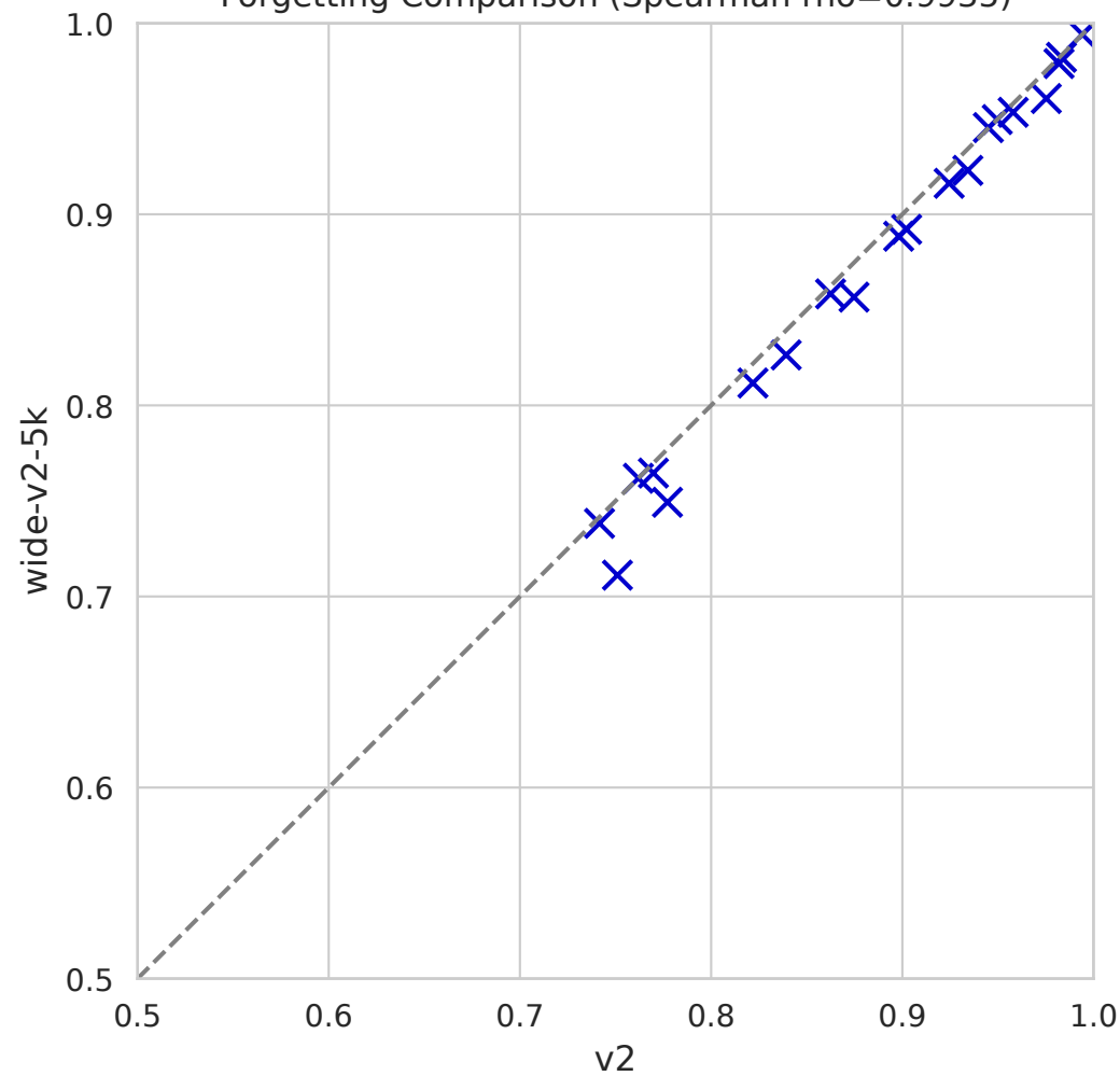
Forgetting Comparison (Spearman rho=0.9935)
