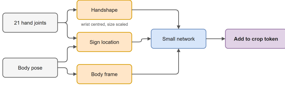
Fig. 5 Landmark features. Joints are centred on the wrist and scaled by hand size before a small network adds them to the crop token.
