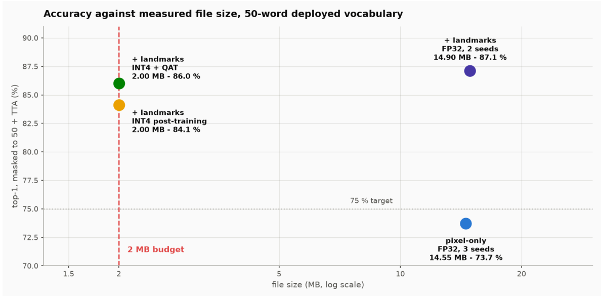
Fig. 11 Accuracy against measured file size. The dashed line marks the 2 MB budget and the dotted line the 75 % target.
