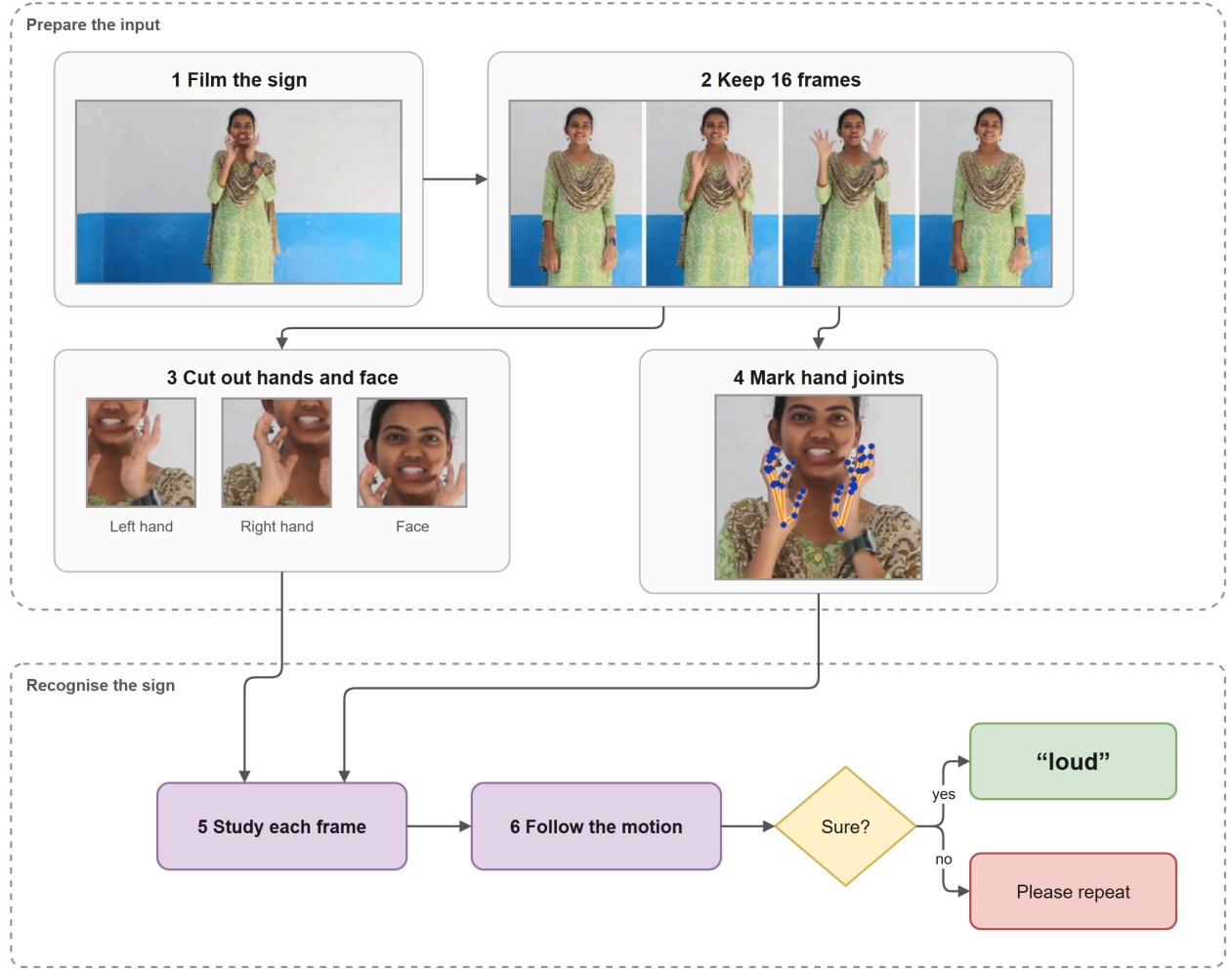
Fig. 2 How ISL-ViT-Tiny reads a sign. Images are real frames, crops and detected hand joints from a held-out test clip of “loud”.
