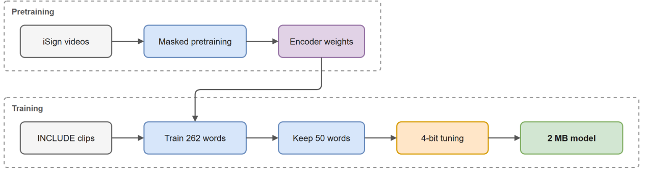
Fig. 7 Training pipeline, from unlabelled pretraining to the 2 MB deployed model.
