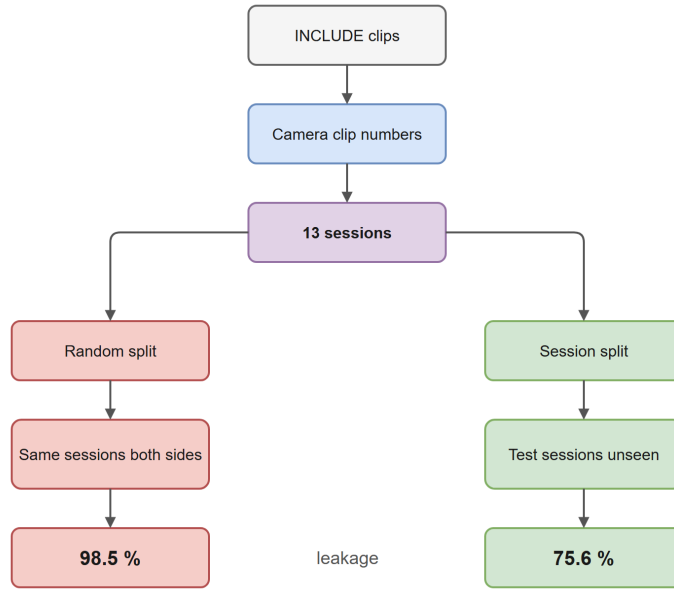
Fig. 4 Building the evaluation split. The same model scores 98.5 % when sessions are shared and 75.6 % when test sessions are unseen.
