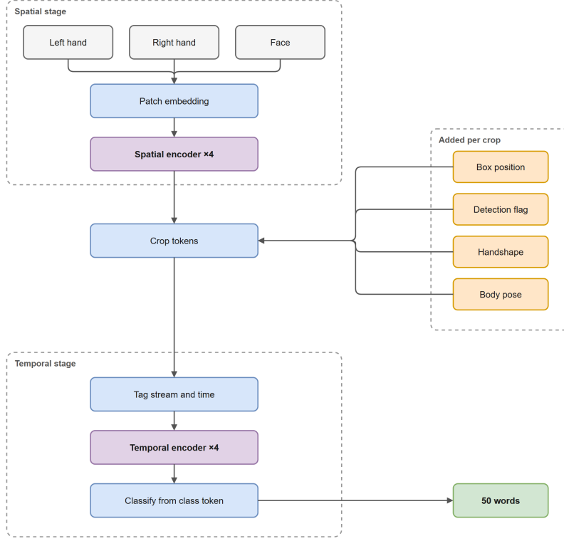
Fig. 6 ISL-ViT-Tiny. The spatial stage runs once per crop with shared weights; the orange inputs are added to every crop token before the temporal stage.
