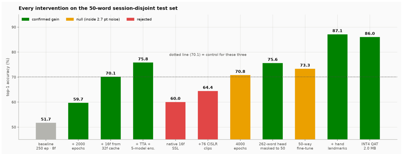
Fig. 10 Every intervention on the 50-word session-disjoint test set. Green: confirmed gain. Amber: inside the 2.7-point noise floor. Red: rejected.
