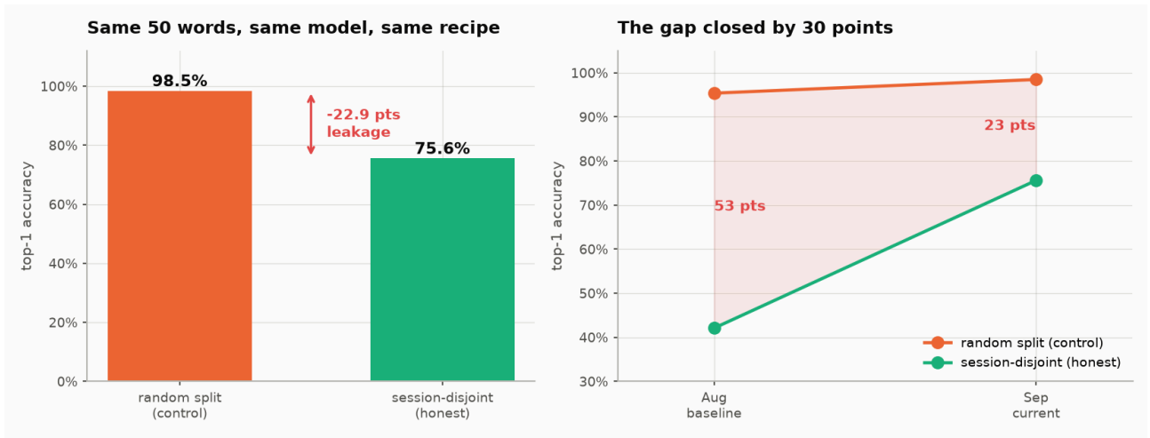
Fig. 9 Left: one model, two splits. Right: the gap between them at the start and end of the project.
