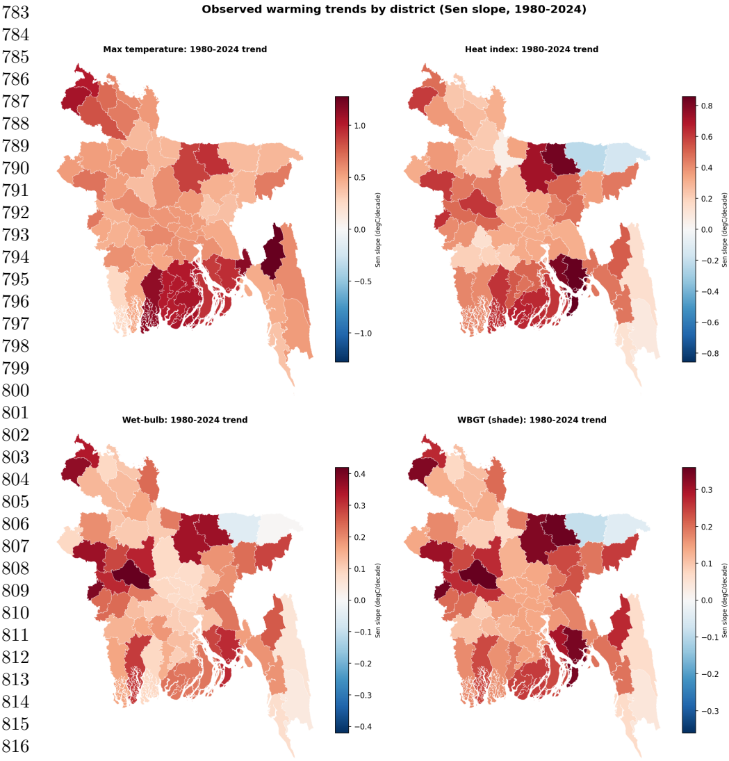
Fig. 2 Observed 1980–2024 warming by district (Theil–Sen slope, °C per decade) for maximum temperature, heat index, wet-bulb temperature, and shade WBGT. Red indicates warming, blue cooling. Values are computed after masking missing-as-zero early-record days (Section 3.12).
