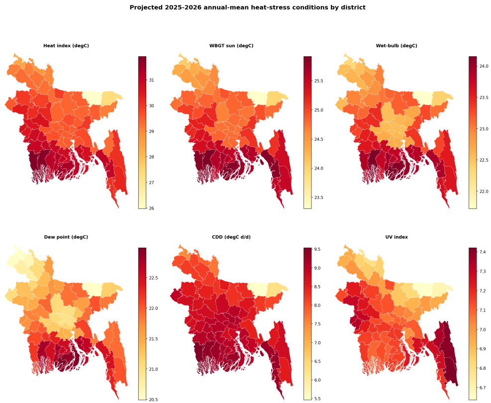
Fig. 6 Projected 2025-2026 annual-mean heat-stress conditions by district: heat index, sun WBGT, wet-bulb temperature, dew point, cooling degree-days, and UV index. Every condition is shown at full district resolution rather than aggregated to zones.
