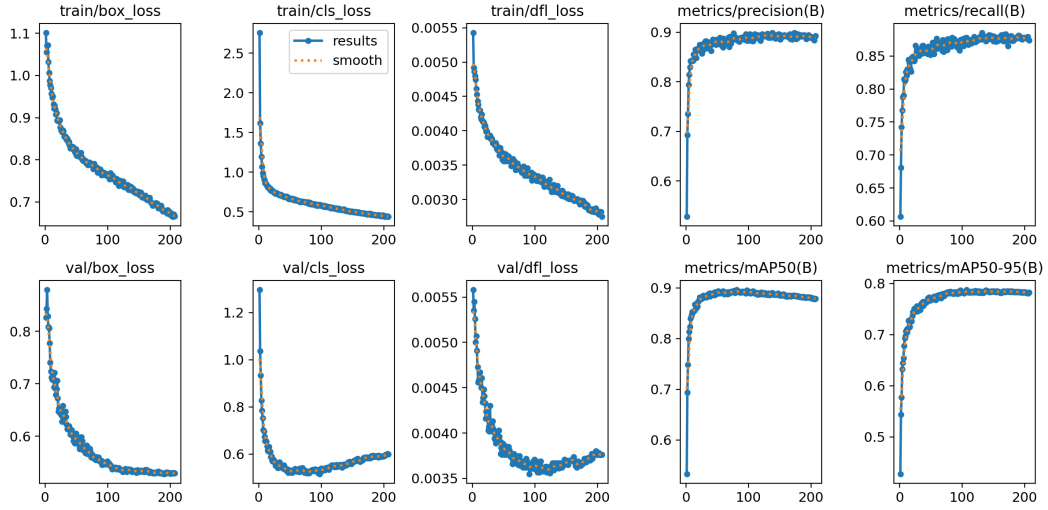
Figure 1: Training results from the YOLO model.
