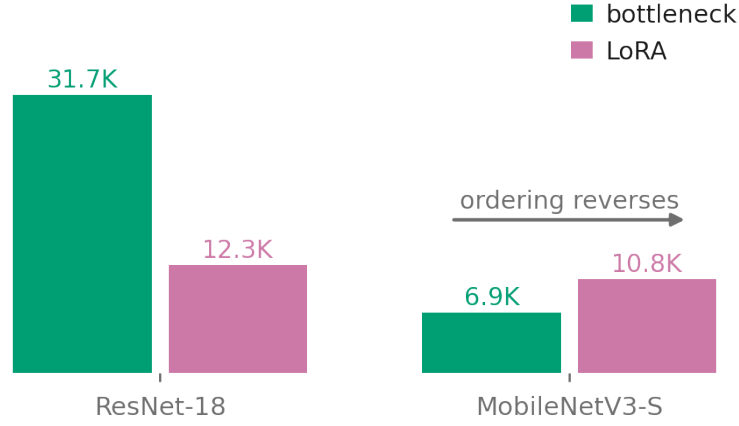
Figure 5.5: The trainable-parameter-count reversal behind ??: bottleneck is the larger adapter on ResNet-18, LoRA is the larger adapter on MobileNetV3-Small.
