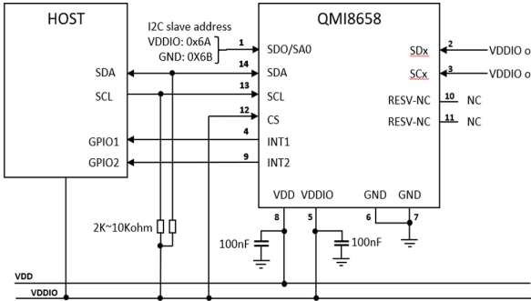
Figure 6. I3C/I2C-UI mode
