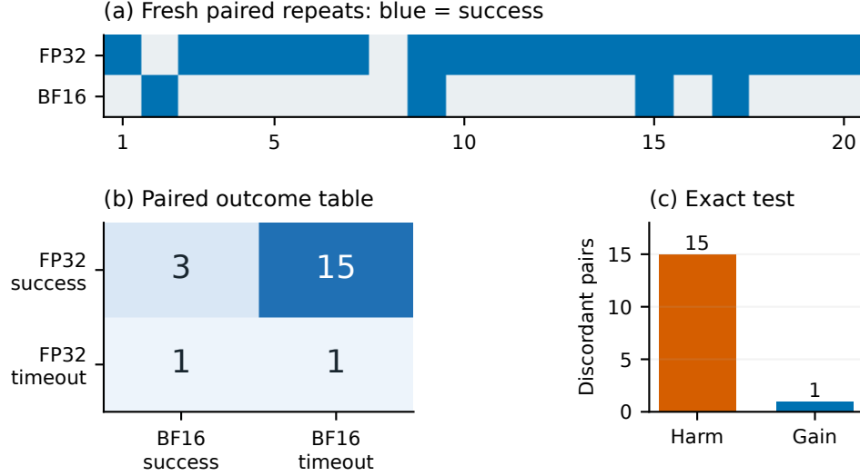
Figure 5: Fresh BF16 follow-up at one selected state. (a) All 20 paired binary outcomes in repeat order; light grey denotes timeout. (b) The full paired table. (c) Fifteen harmful versus one beneficial discordance yield exact one-sided p = 0.0002593994 . The state was selected from the pilot, but only new outcomes enter this single confirmation test.
