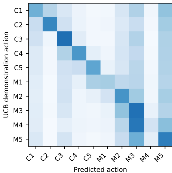
(c) Padded-state confusion
