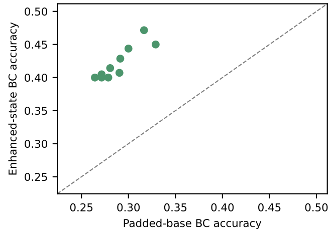
(c) In-sample imitation fit
