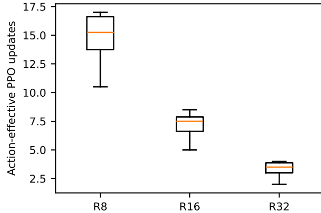
(b) Updates before later actions
