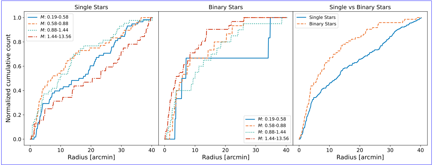
Fig. 9. Left panel: The cumulative distributions of single stars within NGC 6383 are segmented into four mass quartiles ranging from 0.19 – 0.58 M_{\odot} to 1.44 – 13.56 M_{\odot} , illustrating the spatial distribution across different mass ranges and highlighting the potential influences of mass on the distribution of stars within the cluster. Middle panel: The same distributions as in the left panel for binary stars only, where binaries are defined as sources with a binary probability of at least 0.6 . Right panel: The normalized cumulative distributions compare single stars with binary stars, with masses between 0.19 M_{\odot} and 13.56 M_{\odot} . All plots are based on stars with a membership pseudo-probability of at least 0.6 . The corresponding KS test results are given in Sect. 7.
