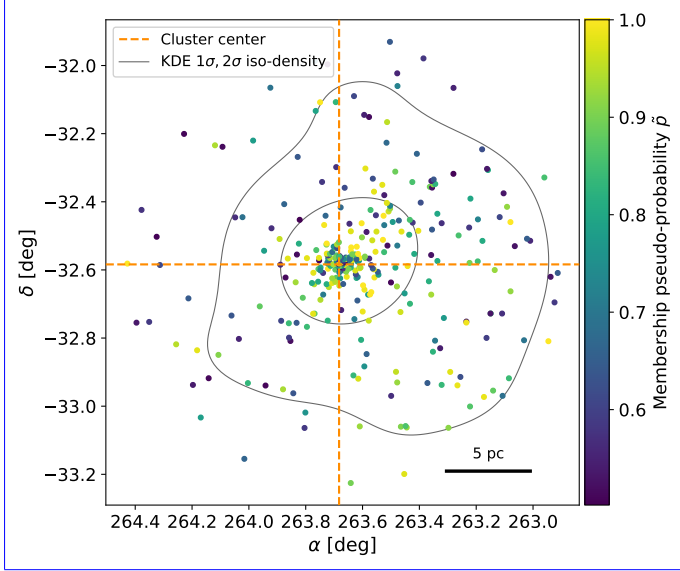
Fig. 4. Spatial distribution of the likely cluster candidates ( \bar{p} > 0.5 ) of NGC 6383 in right ascension ( \alpha ) and declination ( \delta ), color-coded according to their membership pseudo-probability \bar{p} . The gray solid contours are the 1\sigma and 2\sigma iso-density contours (enclosing 39% and 86%) of a kernel density estimate of the candidate positions, revealing the density gradient of the points. The central coordinates of the cluster are marked by dark-orange dashed lines, which approximately coincide with the density peak within the plotted area.
