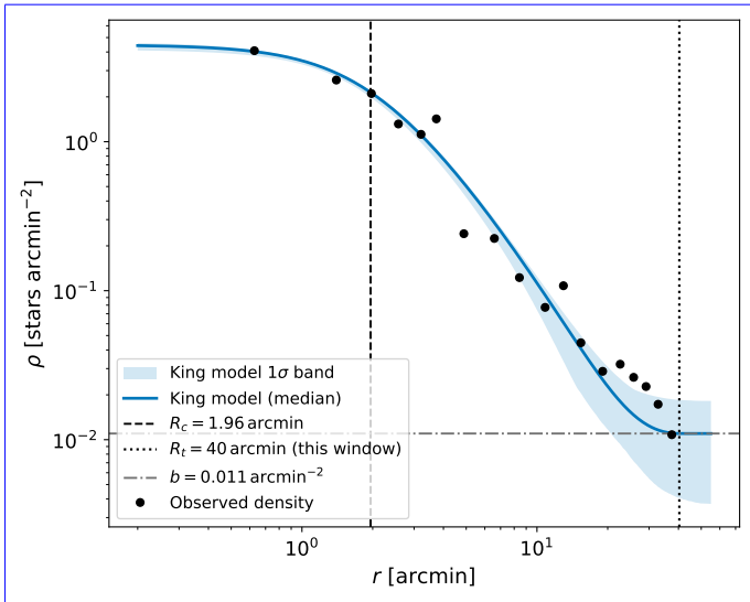
Fig. 5. Radial density profile of NGC 6383 in logarithmic scale: annular number densities of the reference sample with the King model at the posterior median and its 16–84% posterior band. The vertical lines mark the core radius and the outer radius preferred by this 40 arcmin-window fit, and the horizontal line the fitted background level b . The posterior band is narrow near the core, where the profile is set by the well-constrained central density, and broadens markedly at large radii, where this window contains almost no background annulus; the adopted outer radius, R_t = 54^{+7}_{-11} arcmin, is measured on the 70 arcmin extraction (Appendix D, Fig. D.1).
