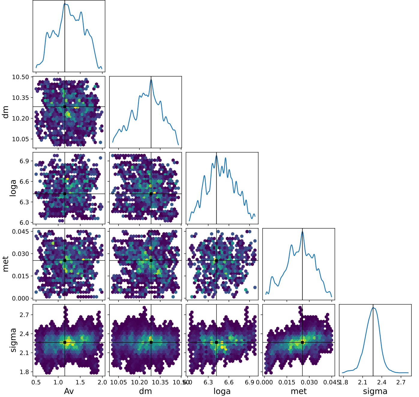
Fig. B.4. Posterior Marginal and joint distributions of the parameters A_V (visual extinction), dm (distance modulus), \log a (logarithmic age), met (metallicity), and the nuisance likelihood-scatter parameter \sigma , sampled with the DEMetropolis ensemble. The ensemble does not meet the convergence criteria of Sect. 3.1, so these are a consistency check, not sampled posteriors. The \sigma parameter is the likelihood-scatter term used in the PyMC diagnostic implementation that generated this figure and should not be interpreted as a physical cluster dispersion. The diagonals display the marginal distributions for each parameter (blue curves). The off-diagonal hexbin plots illustrate the joint distributions, highlighting correlations between parameters. Black lines mark the mode of each distribution in all panels; in the off-diagonal panels, the joint mode is additionally marked by a black square.
