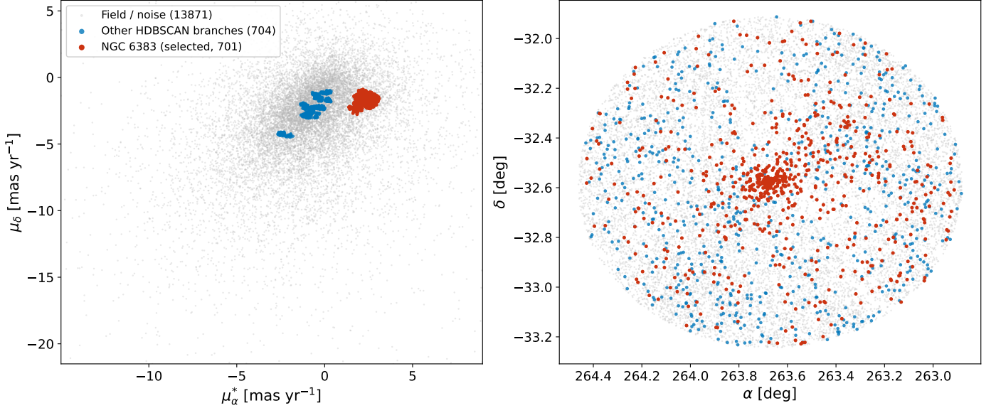
Fig. B.3. Full HDBSCAN clustering panorama of the 40 arcmin preprocessed sample (15276 sources). Left: proper-motion plane ( \mu_{\alpha}^*, \mu_{\delta} ); Right: on-sky distribution in right ascension and declination. Sources are color-coded by their HDBSCAN label: the selected NGC 6383 branch (red), the other HDBSCAN branches (blue), and the field/noise (gray); the legend lists the number of sources in each group. The proper-motion axes are clipped to the 0.5–99.5 percentile range so that the cluster over-density is visible against the broad field distribution. NGC 6383 is a compact, isolated clump in proper motion but overlaps the field on the sky, illustrating that the membership separation is driven by proper motion.
