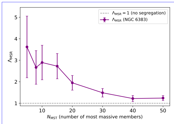
Fig. 10. Mass-segregation ratio \Delta_{\text{MSR}} (Allison et al. 2009b) of NGC 6383 as a function of the number of most-massive members N_{\text{MST}} . Following Allison et al. (2009b), \Delta_{\text{MSR}} = \langle l_{\text{norm}} \rangle / l_{\text{massive}} is the ratio of the mean minimum-spanning-tree length of 500 random N_{\text{MST}} -star sets to that of the N_{\text{MST}} most massive members (purple circles connected by a solid line); error bars are \sigma_{\text{norm}} / l_{\text{massive}} , following the convention of Allison et al. (2009b). They describe the spread of the random reference sets and are not the quantity from which the significance quoted in Sect. 7 is derived; that significance comes from the exact permutation null on the observed member positions. Values \Delta_{\text{MSR}} > 1 indicate that the most massive stars are more centrally concentrated than random members; the gray dashed line marks \Delta_{\text{MSR}} = 1 (no segregation).
