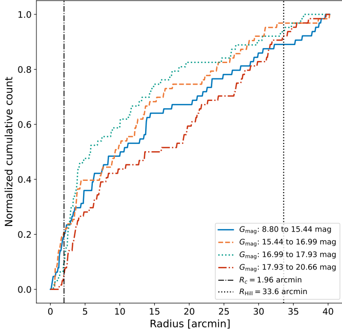
Fig. 8. Normalized cumulative counts of reference-sample stars ( \tilde{p} \geq 0.6 ) within NGC 6383 are plotted against radial distance from the cluster center for different brightness ranges, segmented into quartiles of G_{\text{mag}} , whose ranges are given in the legend. The black dash-dotted and black dotted vertical lines mark the core radius R_c = 1.96 arcmin and the Hill radius R_{\text{Hill}} = 33.6 arcmin; the adopted King outer radius, R_t = 54^{+7}_{-11} arcmin (Appendix D), lies beyond the plotted range of this 40 arcmin sample.
