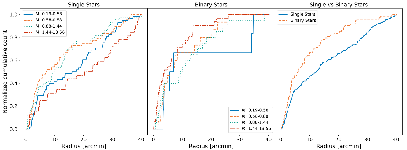
Fig. 9. Left panel: The cumulative distributions of single stars within NGC 6383 are segmented into four mass quartiles ranging from 0.19-0.58 M_{\odot} to 1.44-13.56 M_{\odot} , illustrating the spatial distribution across different mass ranges and highlighting the potential influences of mass on the distribution of stars within the cluster. Middle panel: The same distributions as in the left panel for binary stars only, where binaries are defined as sources with a binary probability of at least 0.6. Right panel: The normalized cumulative distributions compare single stars with binary stars, with masses between 0.19 M_{\odot} and 13.56 M_{\odot} . All plots are based on stars with a membership pseudo-probability of at least 0.6. The corresponding KS test results are given in Sect. 7.
