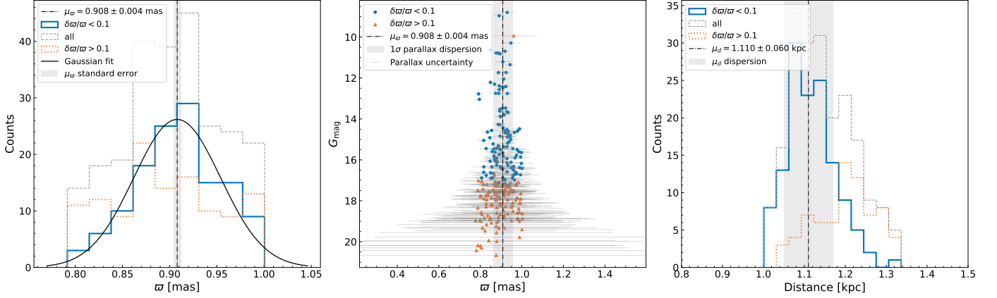
Fig. 2. Left panel: Parallax distribution of the 254-source reference sample, split by fractional parallax error into the subsample used for the estimate ( \delta\varpi/\varpi < 0.1 ), all sources, and the discarded \delta\varpi/\varpi > 0.1 sources; the smooth curve is a Gaussian fit, and the dash-dotted line and shaded band mark the mean parallax and its standard error. Middle panel: G magnitude versus parallax with the same split; horizontal bars are the individual parallax uncertainties and the shaded band the 1\sigma parallax dispersion. Right panel: Bailer-Jones geometric distances (Bailer-Jones et al. 2021) with the same split; the dash-dotted line and shaded band mark the adopted distance (the mode of the sampled distances) and its dispersion. Values are given in the panel legends. For convenience, only the portion of the histogram corresponding to distances within 0.8 to 1.2 times the minimum and maximum used distances is displayed.
