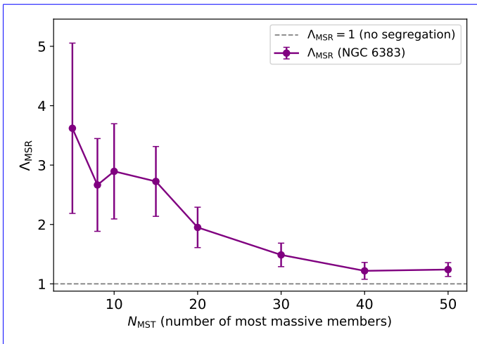
Fig. 10. Mass-segregation ratio \Delta_{\text{MSR}} (Allison et al. 2009b) of NGC 6383 as a function of the number of most-massive members N_{\text{MST}} . Following Allison et al. (2009b), \Delta_{\text{MSR}} = \langle l_{\text{norm}} \rangle / l_{\text{massive}} is the ratio of the mean minimum-spanning-tree length of 500 random N_{\text{MST}} -star sets to that of the N_{\text{MST}} most massive members (purple circles connected by a solid line); error bars are \sigma_{\text{norm}} / l_{\text{massive}} , following the convention of Allison et al. (2009b). They describe the spread of the random reference sets and are not the quantity from which the significance quoted in Sect. 7 is derived; that significance comes from the exact permutation null on the observed member positions. Values \Delta_{\text{MSR}} > 1 indicate that the most massive stars are more centrally concentrated than random members; the gray dashed line marks \Delta_{\text{MSR}} = 1 (no segregation).
