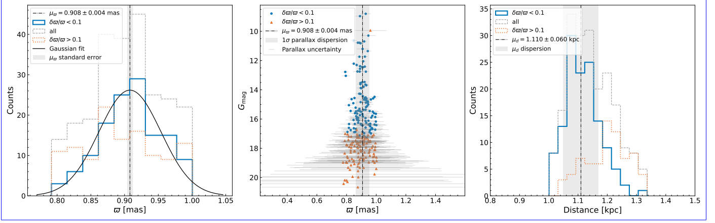
Fig. 2. Left panel: Parallax distribution of the 254-source reference sample, split by fractional parallax error into the subsample used for the estimate ( \delta\pi/\pi < 0.1 ), all sources, and the discarded \delta\pi/\pi > 0.1 sources; the smooth curve is a Gaussian fit, and the dash-dotted line and shaded band mark the mean parallax and its standard error. Middle panel: G magnitude versus parallax with the same split; horizontal bars are the individual parallax uncertainties and the shaded band the 1\sigma parallax dispersion. Right panel: Bailer-Jones geometric distances (Bailer-Jones et al. 2021) with the same split; the dash-dotted line and shaded band mark the adopted distance (the mode of the sampled distances) and its dispersion. Values are given in the panel legends. For convenience, only the portion of the histogram corresponding to distances within 0.8 to 1.2 times the minimum and maximum used distances is displayed.
