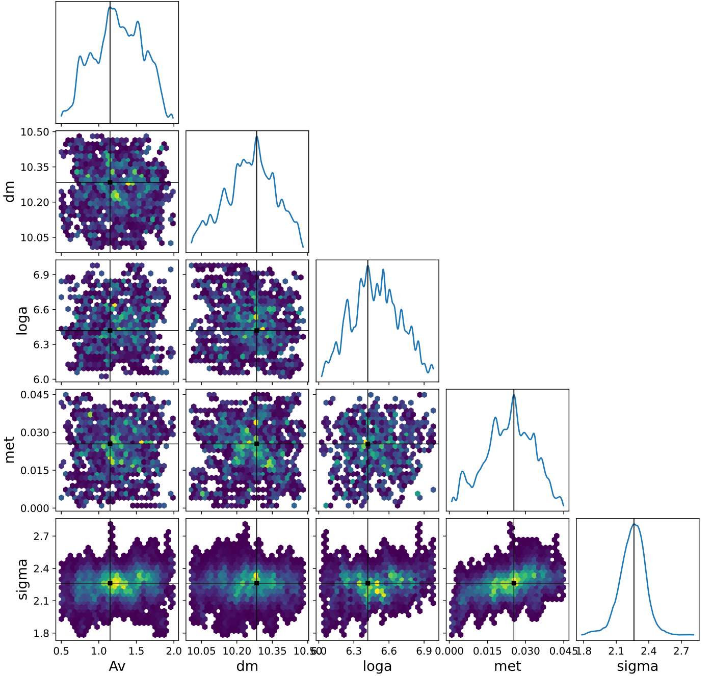
Fig. B.4. Posterior distributions of the parameters A_V (visual extinction), dm (distance modulus), \log a (logarithmic age), met (metallicity), and the nuisance likelihood-scatter parameter \sigma . The \sigma parameter is the likelihood-scatter term used in the PyMC diagnostic implementation that generated this figure and should not be interpreted as a physical cluster dispersion. The diagonals display the marginal distributions for each parameter (blue curves). The off-diagonal hexbin plots illustrate the joint distributions, highlighting correlations between parameters. Black lines mark the mode of each distribution in all panels; in the off-diagonal panels, the joint mode is additionally marked by a black square.
