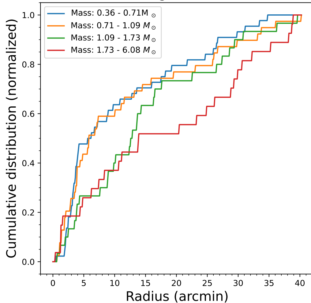
Single Stars
