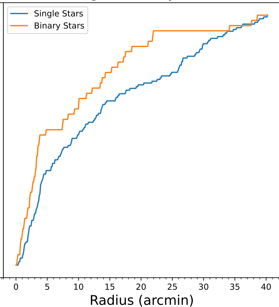
Single vs Binary Stars
