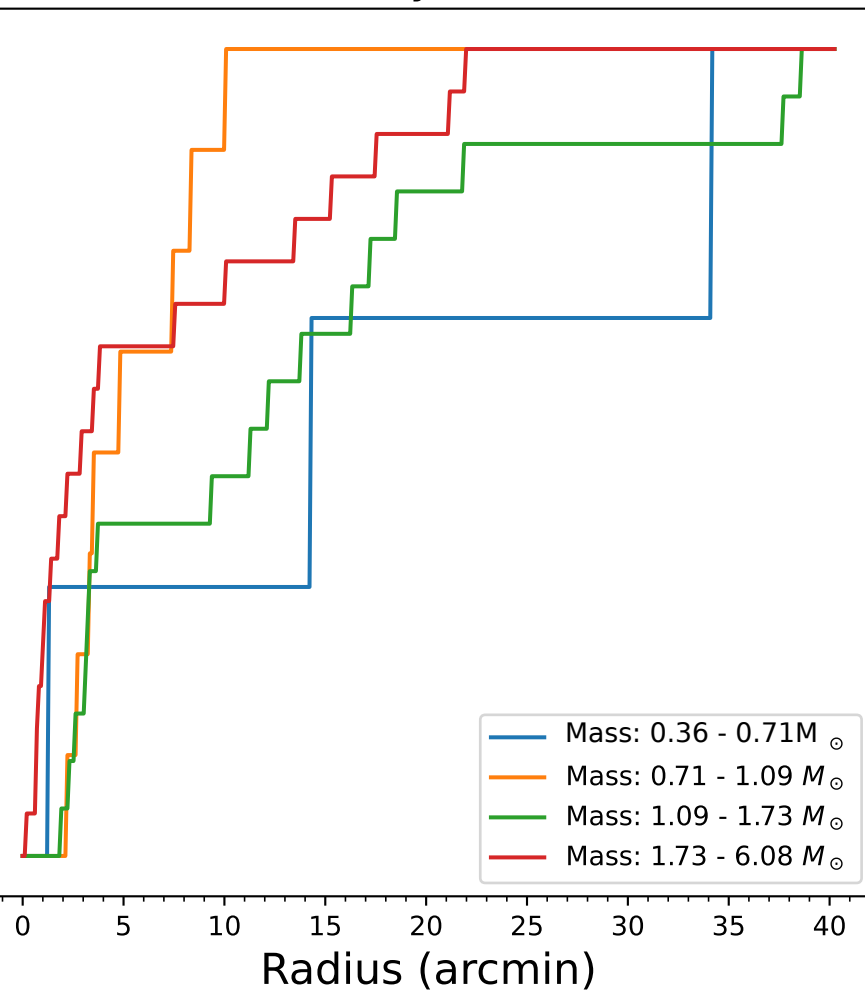
Binary Stars
