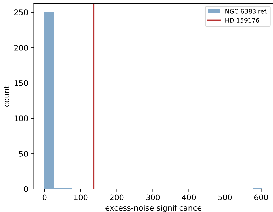
HD 159176 vs NGC 6383 Gaia DR3 astrometric-quality metrics
