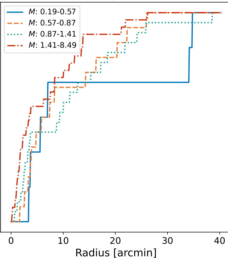
Binary Stars
