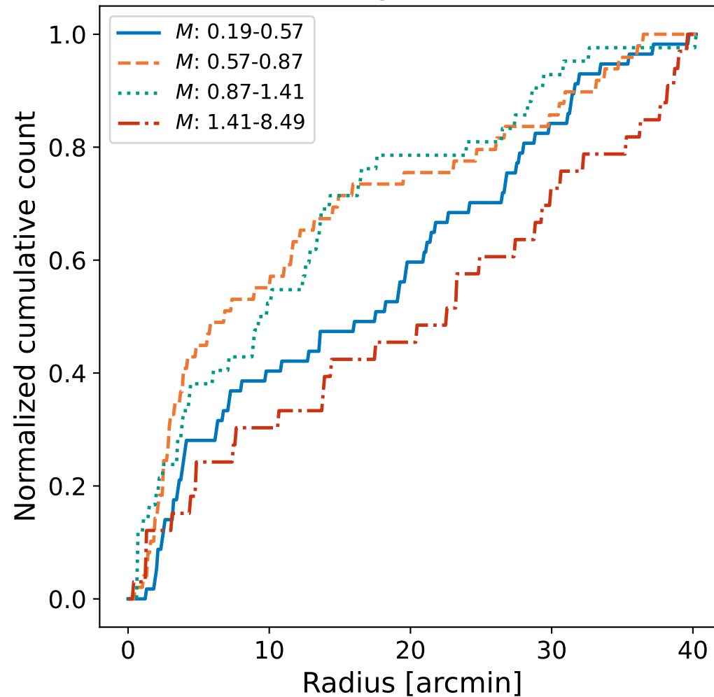
Single Stars
