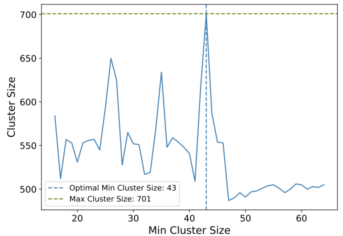
Fig. B.1. Cluster size variation as a function of minimum cluster size, determined through HDBSCAN clustering on the proper-motion data of the sources. The blue line represents the recovered cluster sizes achieved at various minimum cluster sizes. The size; the dashed blue line highlights marks the optimal-adopted minimum cluster size of 43, where the cluster size reaches a peak. The peaks, and the dashed green line indicates the maximum observed cluster size of 701. Only sweep runs passing in the branch-stability criteria stable regime (condensed-tree \lambda_{max} \geq 8 and recovered branch size between 200 and 701 of 200–701 sources) are shown, which is why the axis does not span the full m_{cl} = 10 –299 grid; this display cut does not enter the selection of m_{cl} .
