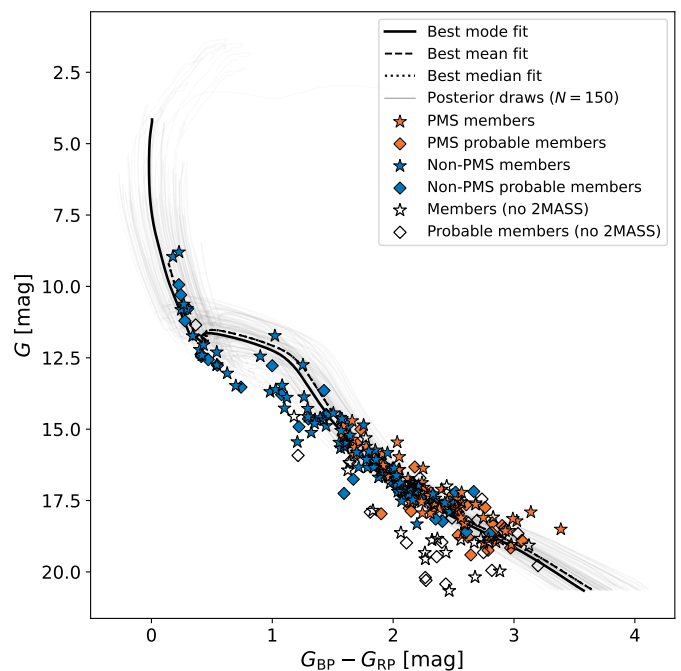
Fig. 6. CMD of NGC 6383 ( G_{\text{mag}} versus G_{BP} - G_{RP} ) with the Sagitta-based PMS classification: orange filled symbols are PMS candidates (Sagitta PMS probability \geq 0.6 ), blue filled symbols are non-PMS sources, and open black symbols are sources without 2MASS photometry, which are left unclassified; stars denote members ( \bar{p} \geq 0.8 ) and diamonds probable members ( 0.6 \leq \bar{p} < 0.8 ). The black solid, dashed, and dotted curves are the synthetic single-star sequences at the mode, mean, and median of the isochrone-fit ensemble, and the light-gray curves are 150 single-star sequences drawn from that ensemble.
